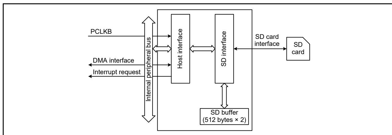
Figure 43.1 Block Diagram of the SDHI
