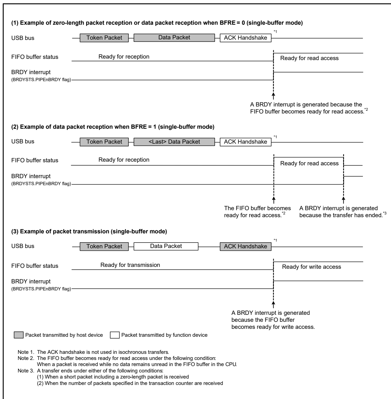
Figure 36.11 Timing of BRDY Interrupt Generation
