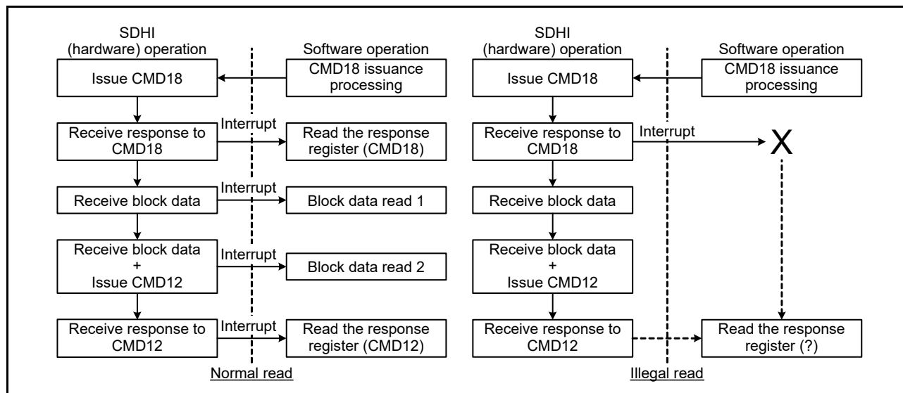
Figure 43.23 Multi-Block Read Processing When Reading Two Blocks
