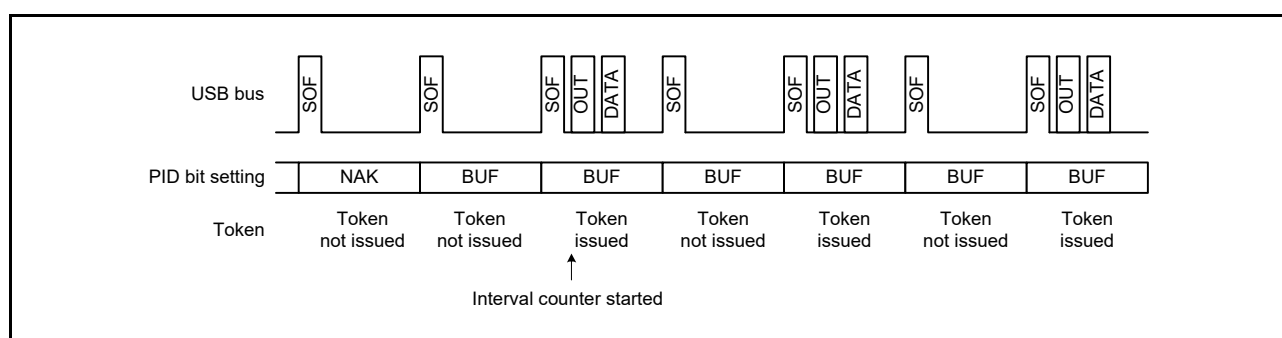
Figure 36.17 Token Issuance When IITV[2:0] = 001b
