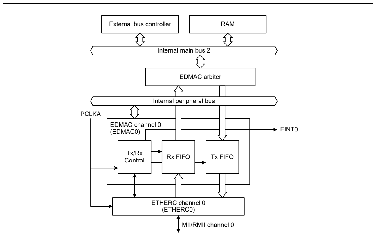
Figure 35.1 EDMAC Configuration
