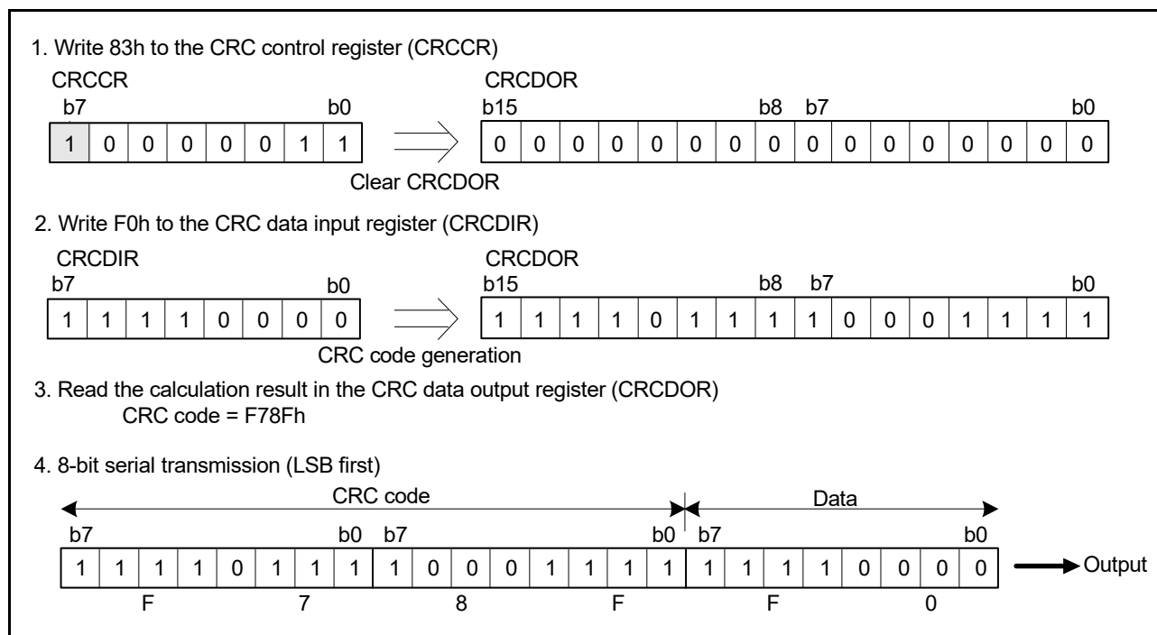
Figure 42.2 LSB First Data Transmission
