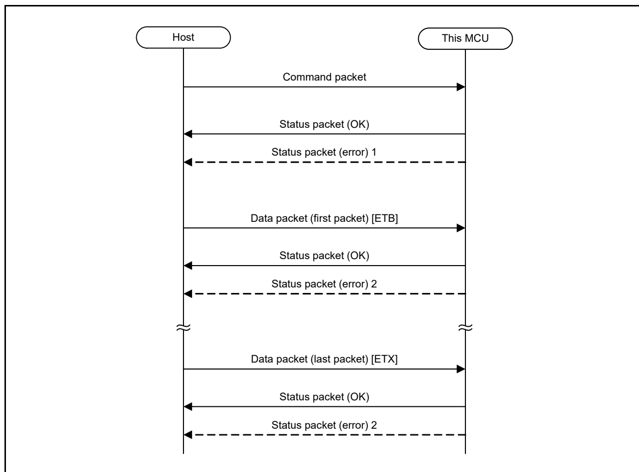
Figure 59.22 Configuration Program Command Transfer Sequence
