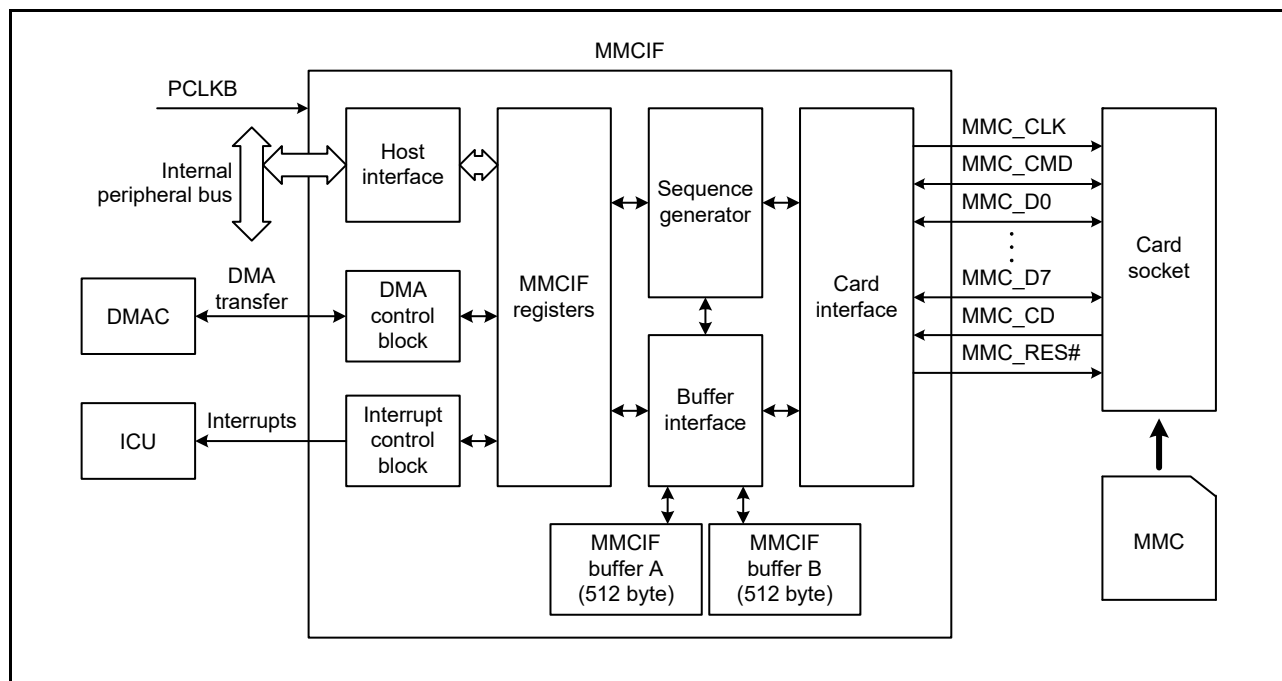
Figure 45.1 Block Diagram of the MMCIF
