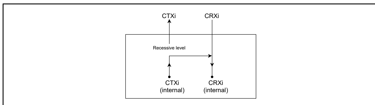
Figure 39.6 Connection when Listen-Only Mode is Selected ( i = 0, 1 )
