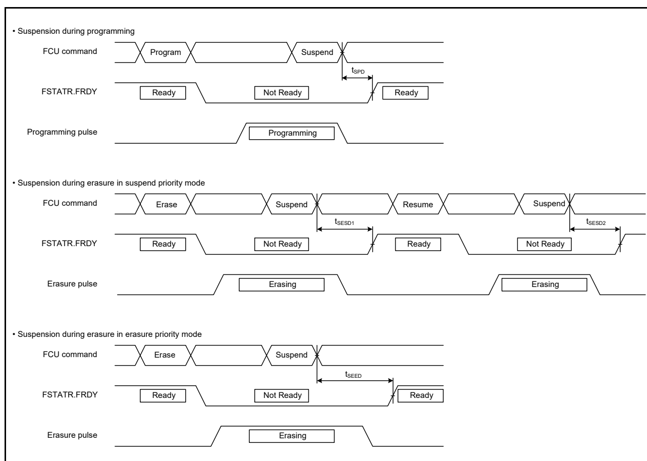
Figure 60.96 Flash Memory Programming/Erasure Suspension Timing
