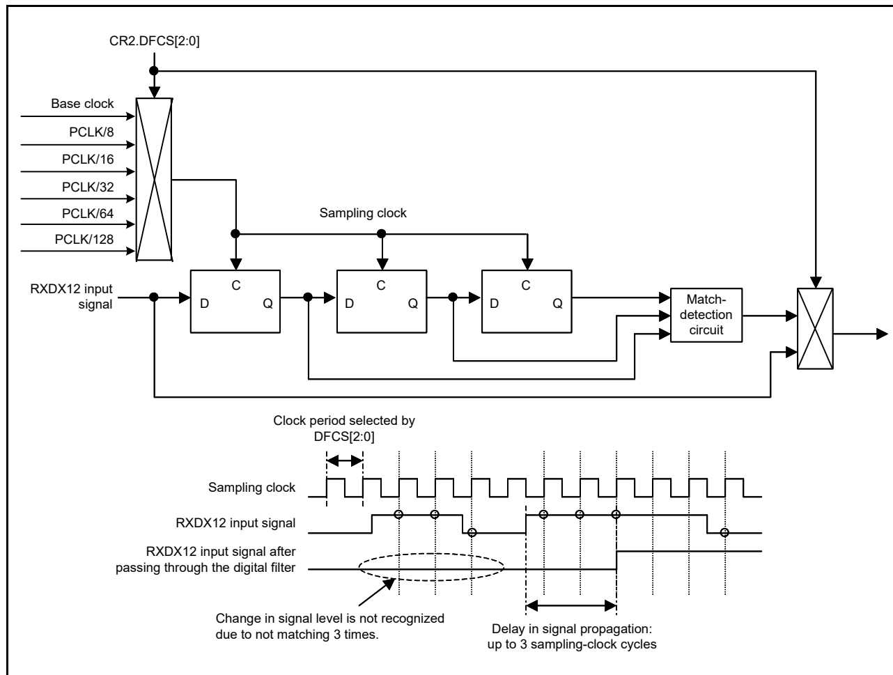
Figure 37.74 Example of Operations with the Digital Filter
