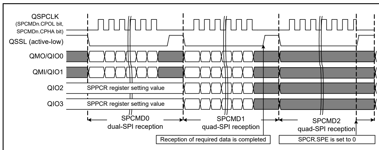
Figure 41.19 Example of Sequence Configuration with Transfer Mode Switching (Termination Method 1 When All the Commands Configuring a Sequence Are Dual-/Quad-SPI Read Operations) (n = 0 to 3)
