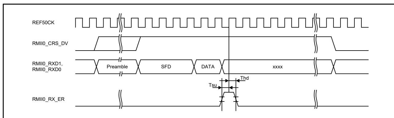
Figure 60.69 RMII Reception Timing (Error Occurrence)
