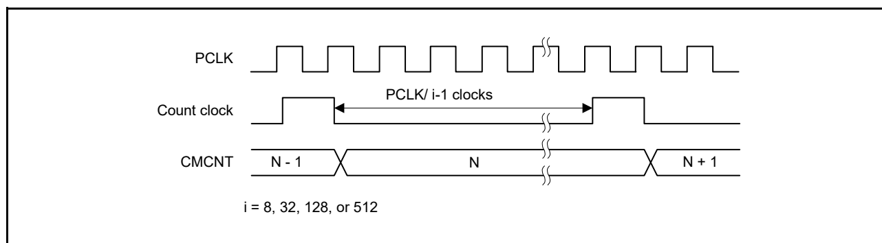
Figure 29.3 CMCNT Count Timing
