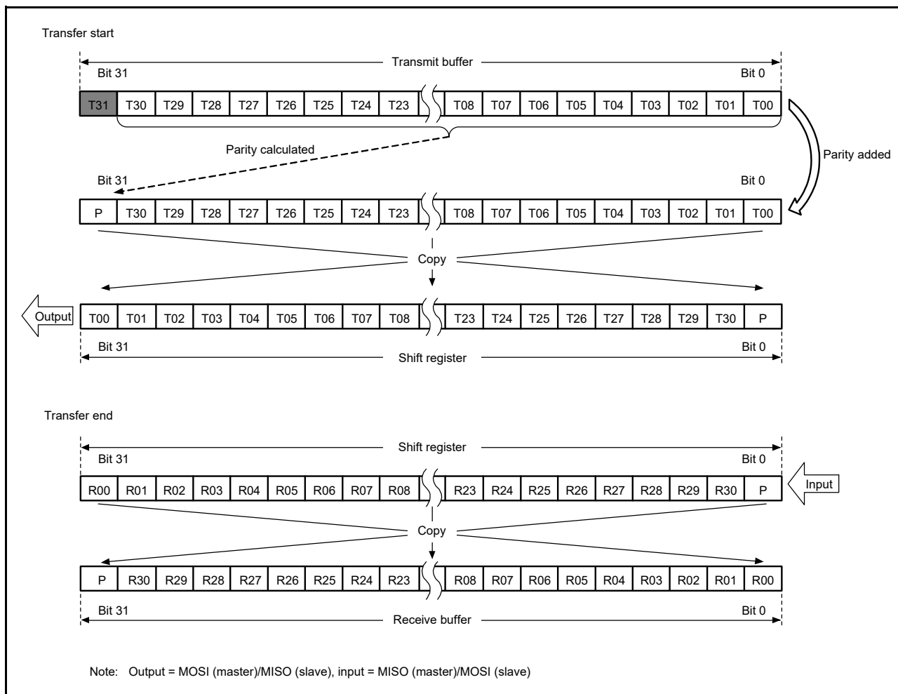
Figure 40.20 LSB First Transfer (32-Bit Data, Parity Enabled)
