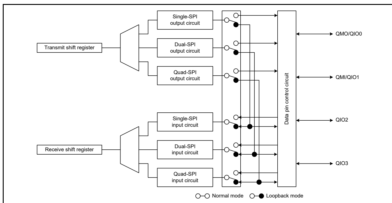
Figure 41.26 Schematic Internal Connection in Loopback Mode
