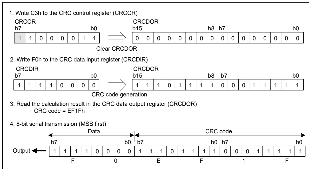
Figure 42.3 MSB First Data Transmission
