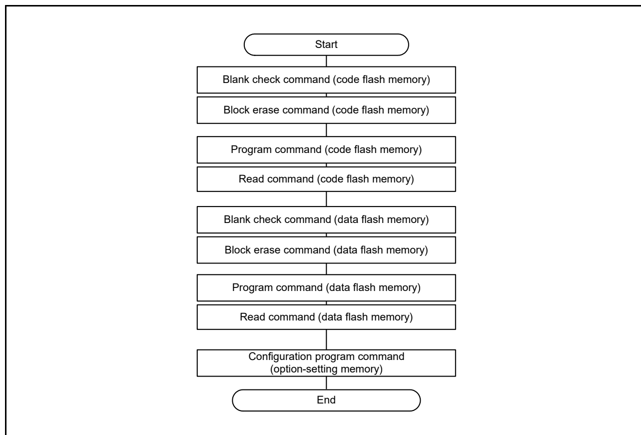
Figure 59.23 Example of Reprogramming Procedure
