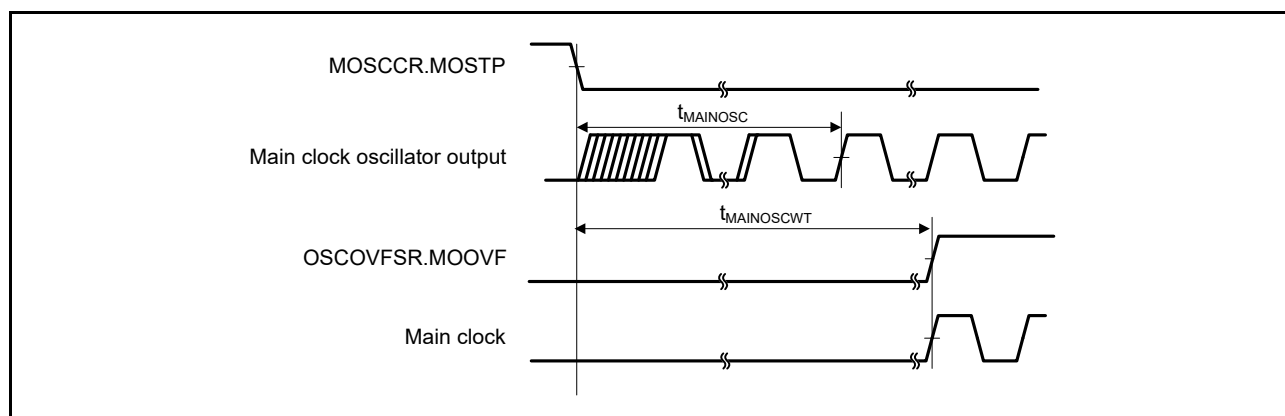
Figure 60.5 Main Clock Oscillation Start Timing
