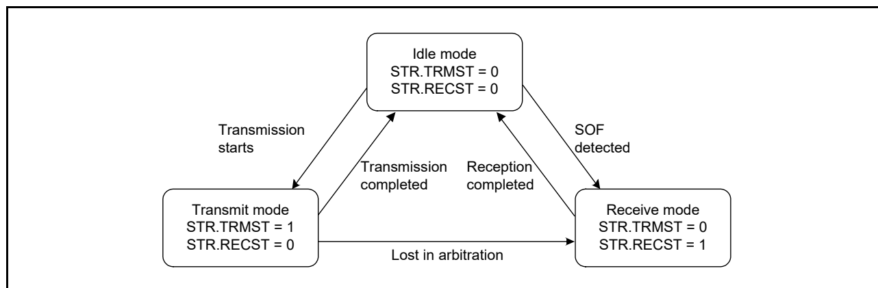
Figure 39.10 Sub-Modes of CAN Operation Mode
