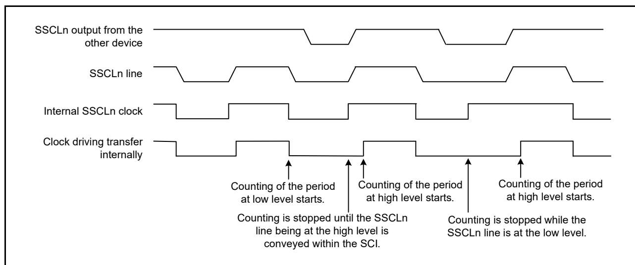
Figure 37.53 Example of Operations for Clock Synchronization
