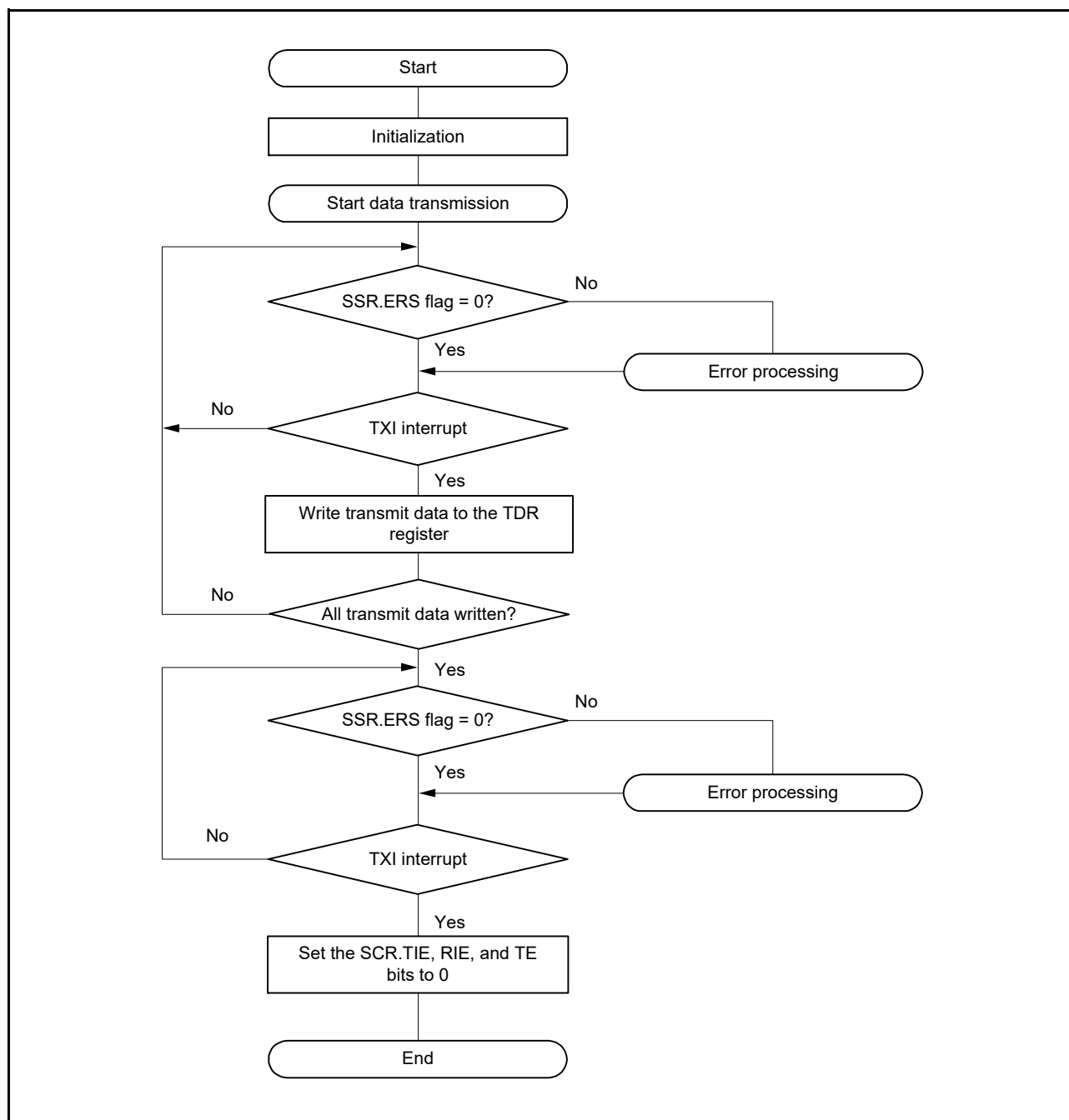
Figure 37.45 Sample Smart Card Interface Transmission Flowchart
