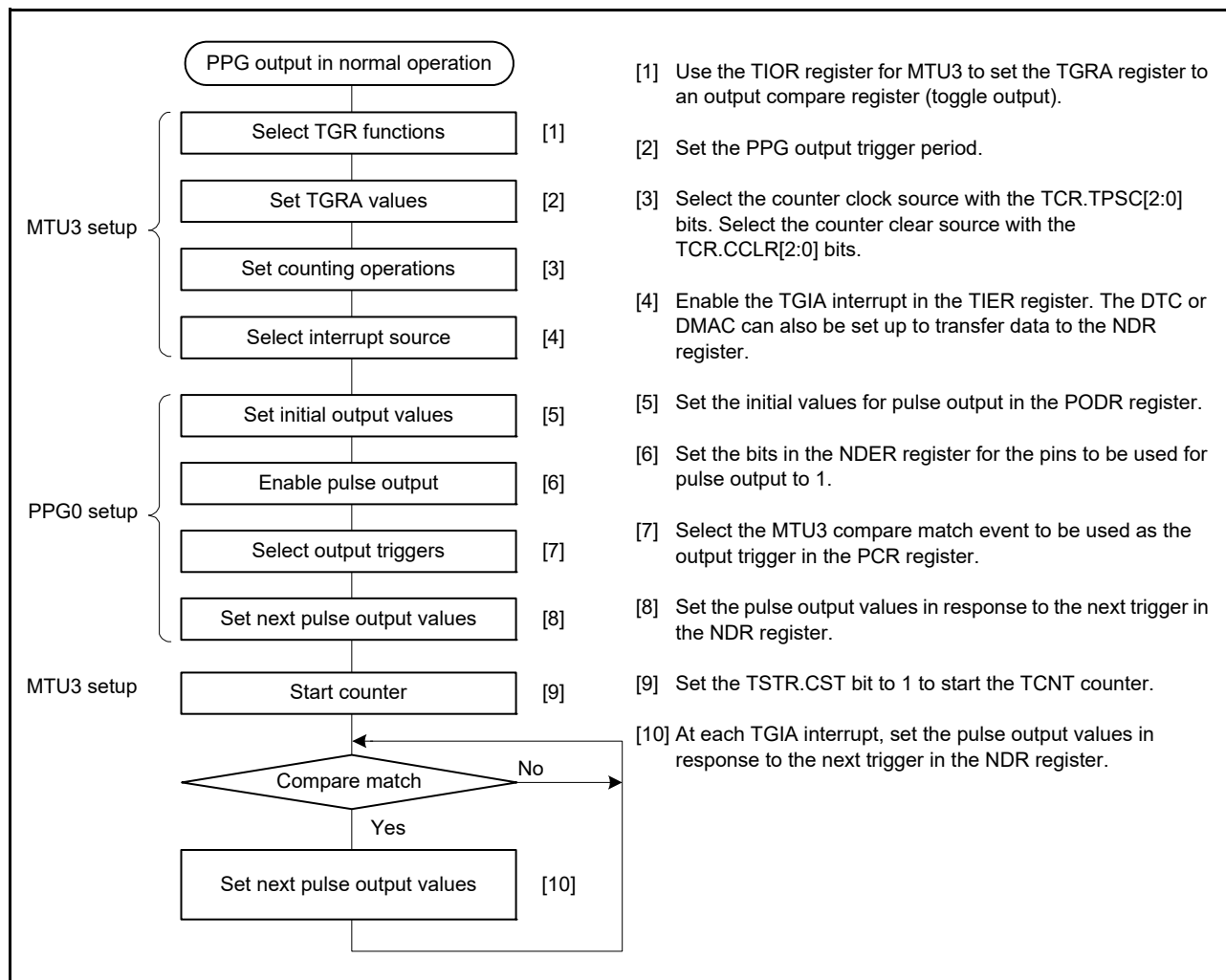
Figure 27.6 Example of Setup Procedure for Pulse Output in Normal Operation (PPG0 Setting)
