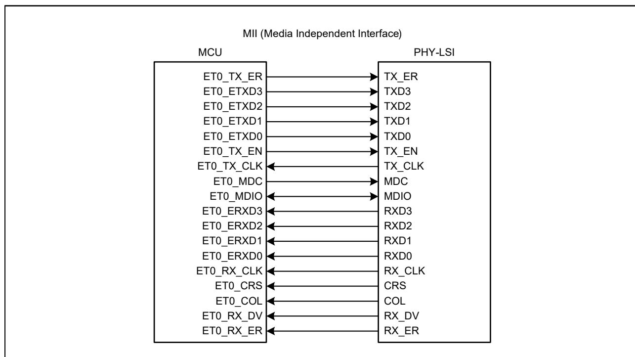
Figure 34.2 Example of Connection with the PHY-LSI for the MII
