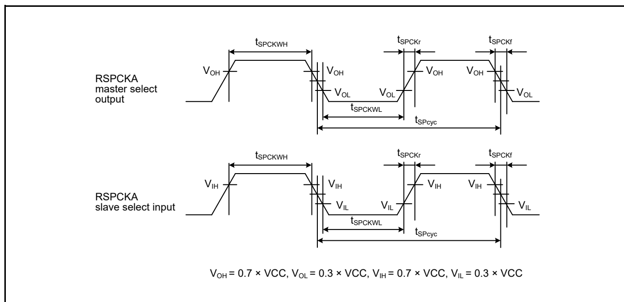
Figure 60.54 RSPI Clock Timing
