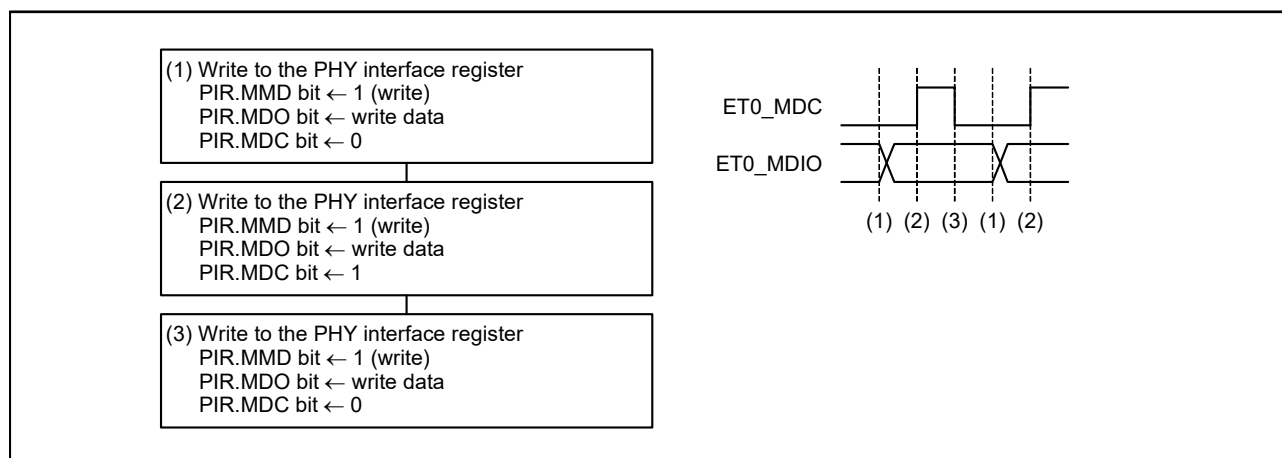
Figure 34.14 1-Bit Data Write Flow
