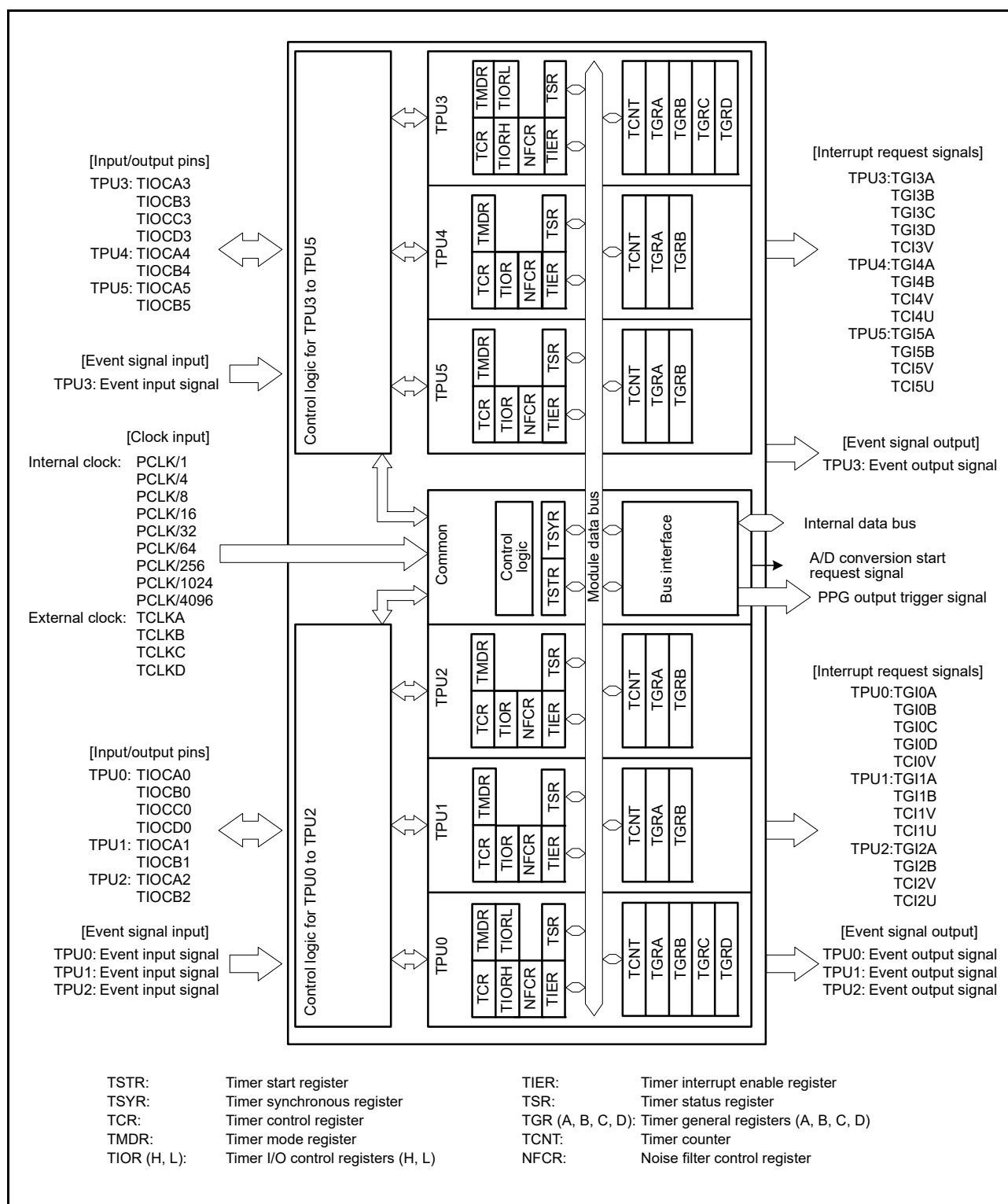
Figure 26.1 Block Diagram of TPU
