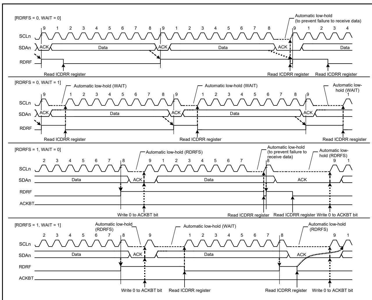
Figure 38.31 Automatic Low-Hold Operation in Receive Mode (Using RDRFS and WAIT Bits)
