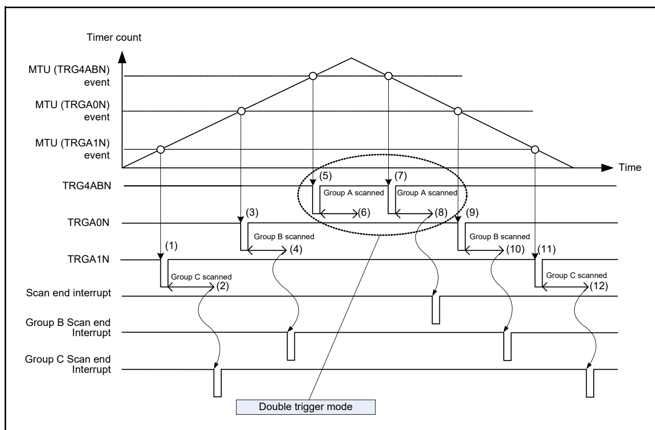
Figure 53.23 Example of Operation in Group Scan Mode with Double Trigger Mode (Basic Operation: Synchronous Triggers from MTU Used)
