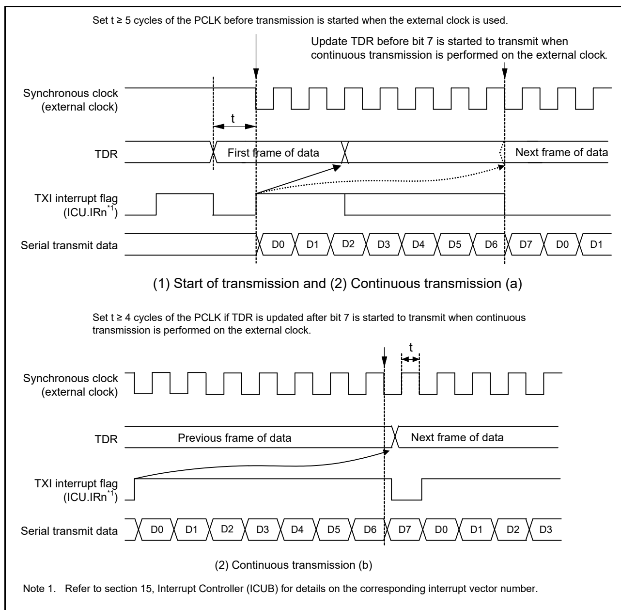
Figure 37.80 Restrictions on Use of External Clock in Clock Synchronous Transmission
