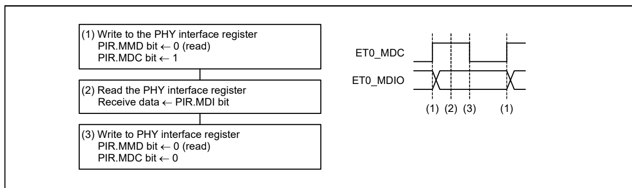
Figure 34.16 1-Bit Data Read Flow
