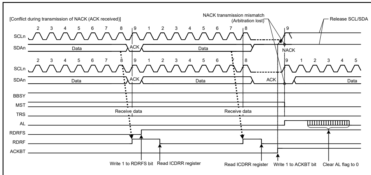
Figure 38.34 Example of NACK transmission arbitration-lost Detection (NALE = 1)
