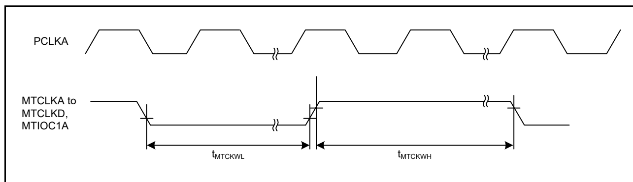
Figure 60.39 MTU3 Clock Input Timing
