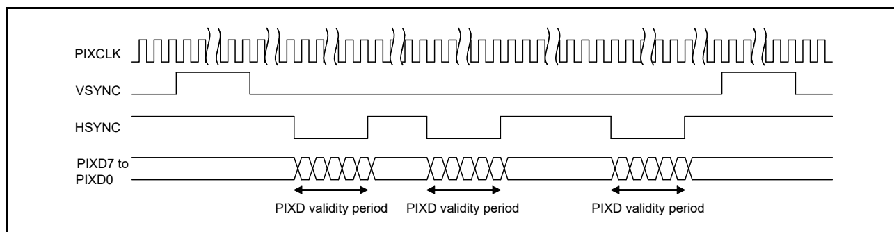
Figure 46.7 PDC Transfer Format (for VPS = 1, HPS = 1)
