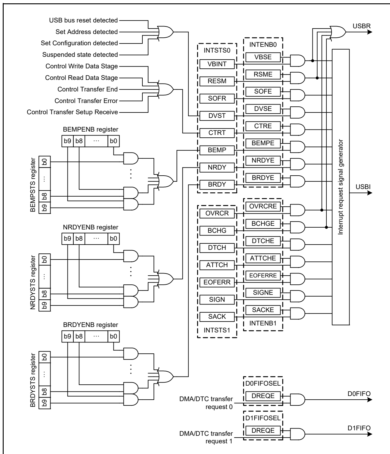
Figure 36.10 Circuits Related to Interrupts in USB
