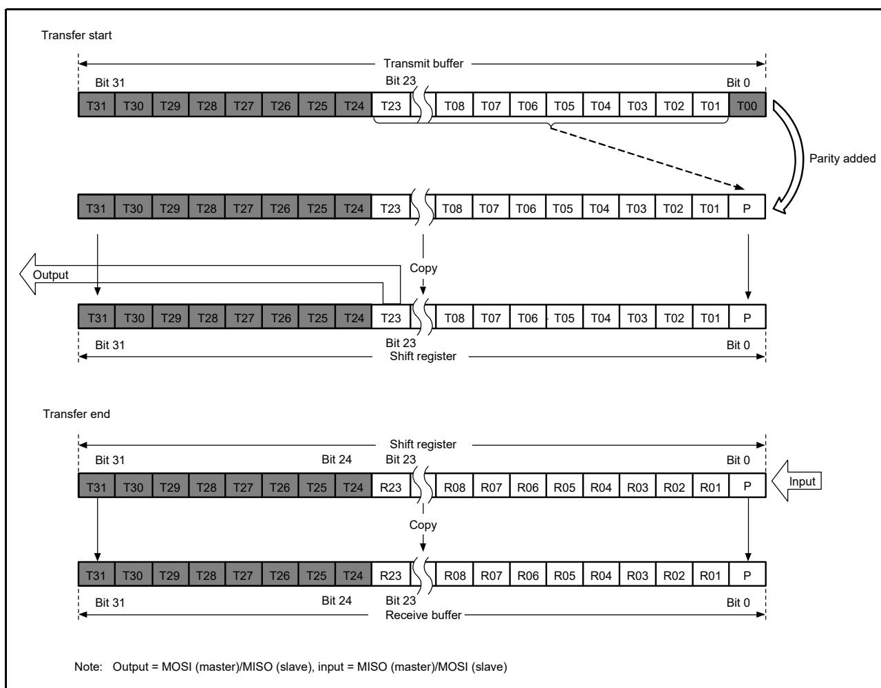
Figure 40.19 MSB First Transfer (24-Bit Data, Parity Enabled)
