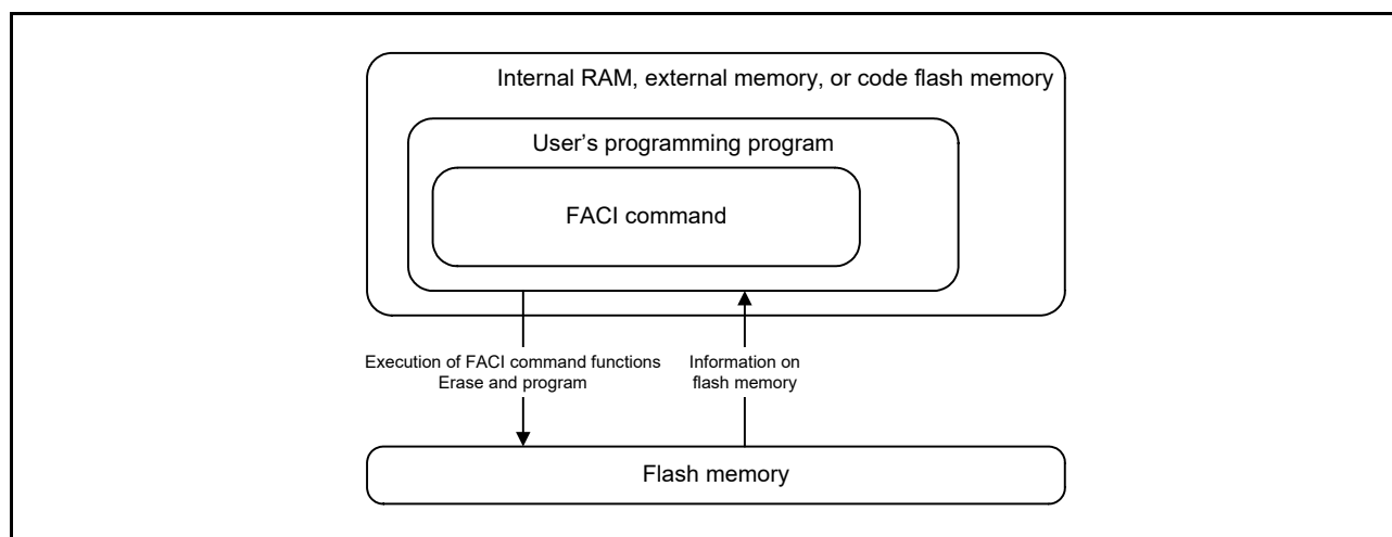
Figure 59.28 Schematic View of Self-Programming
