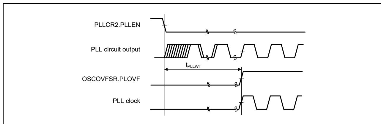
Figure 60.10 PLL Clock Oscillation Start Timing
