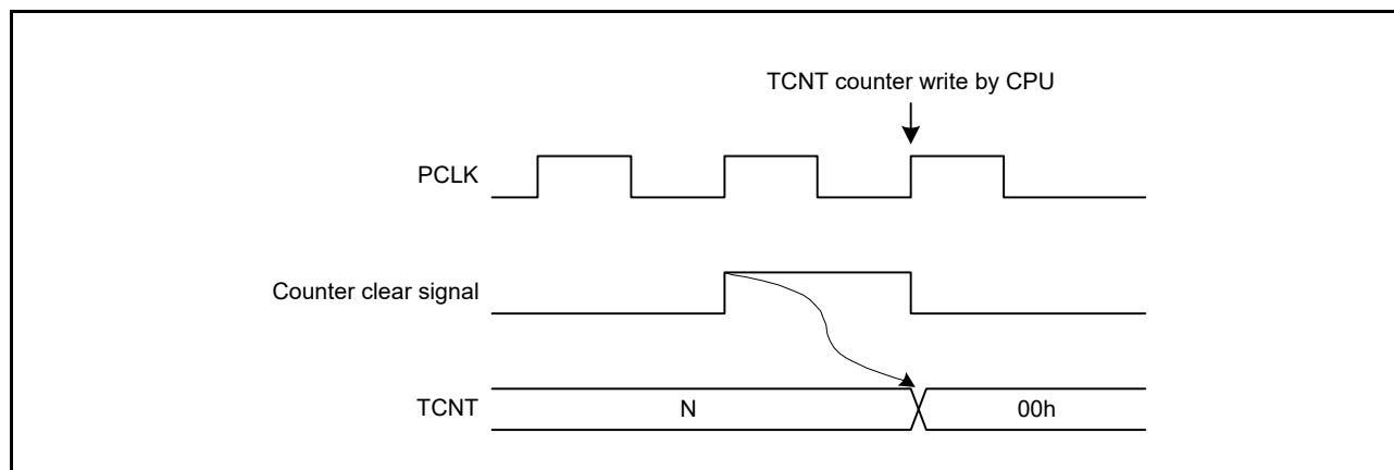
Figure 28.13 Conflict between TCNT Write and Counter Clear
