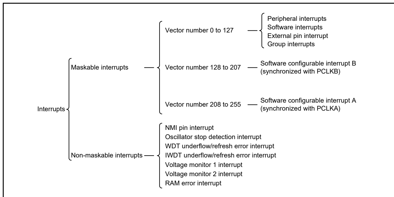
Figure 15.2 Types of Interrupts
