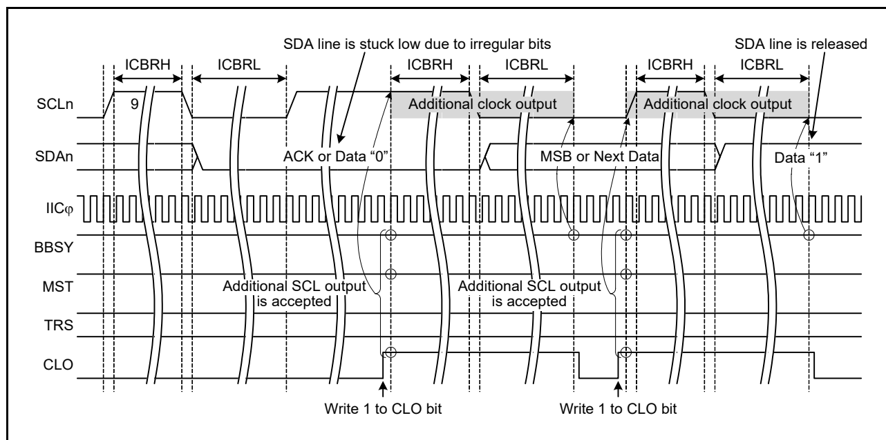
Figure 38.39 Additional SCL Output Function (CLO Bit)
