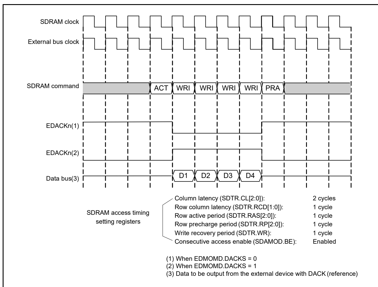
Figure 19.34 Operation Example in Block-Transfer (SDRAM Area Write: Consecutive Access Enabled, EXDMACn.EDMOMD.DACKSEL = 0) Single Address Mode
