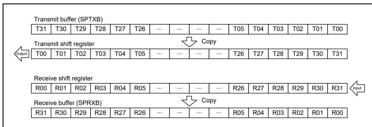
Figure 41.9 LSB First Transfer (32-Bit Data)
