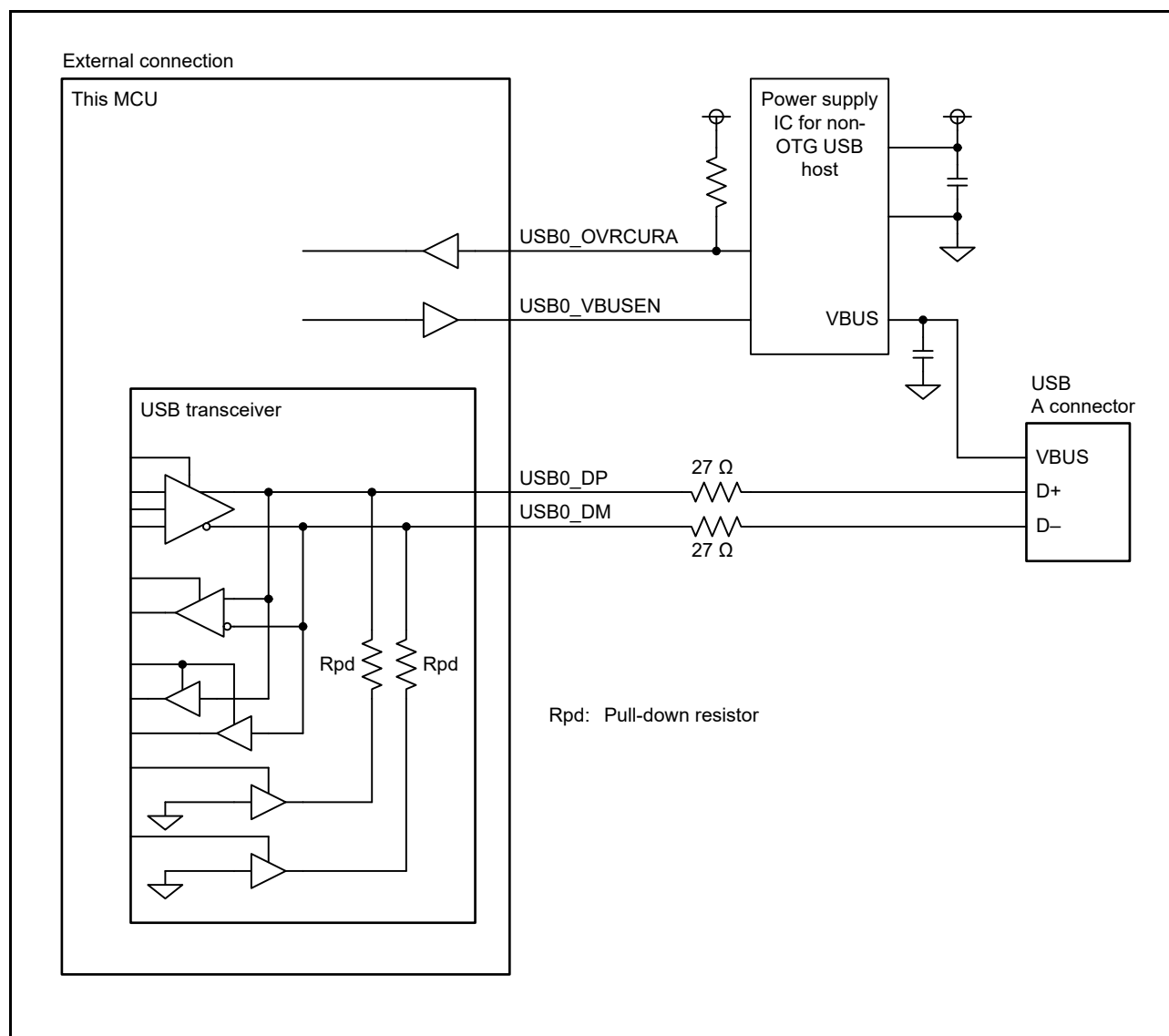
Figure 36.4 Example of Connection between Host and USB Connector
