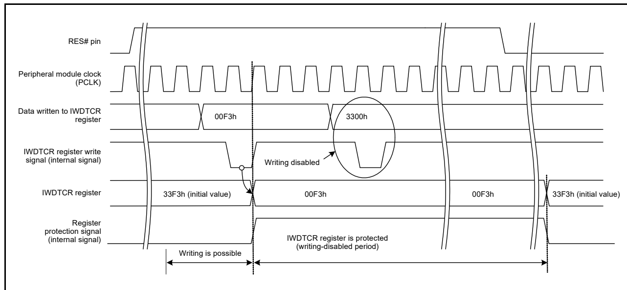
Figure 33.5 Control Waveforms Produced in Response to Writing to the IWDTCR Register
