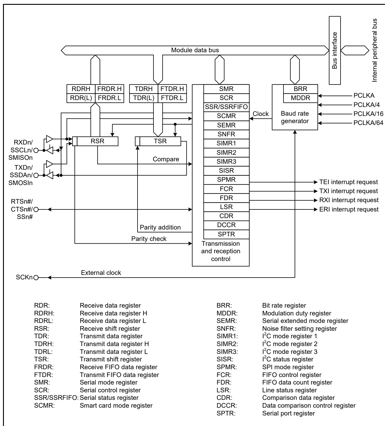
Figure 37.3 Block Diagram of SCli (SCI10 and SCI11)
