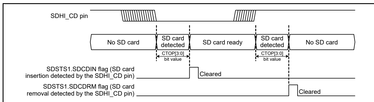
Figure 43.6 SD Card Detection Using the SDHI_CD Pin
