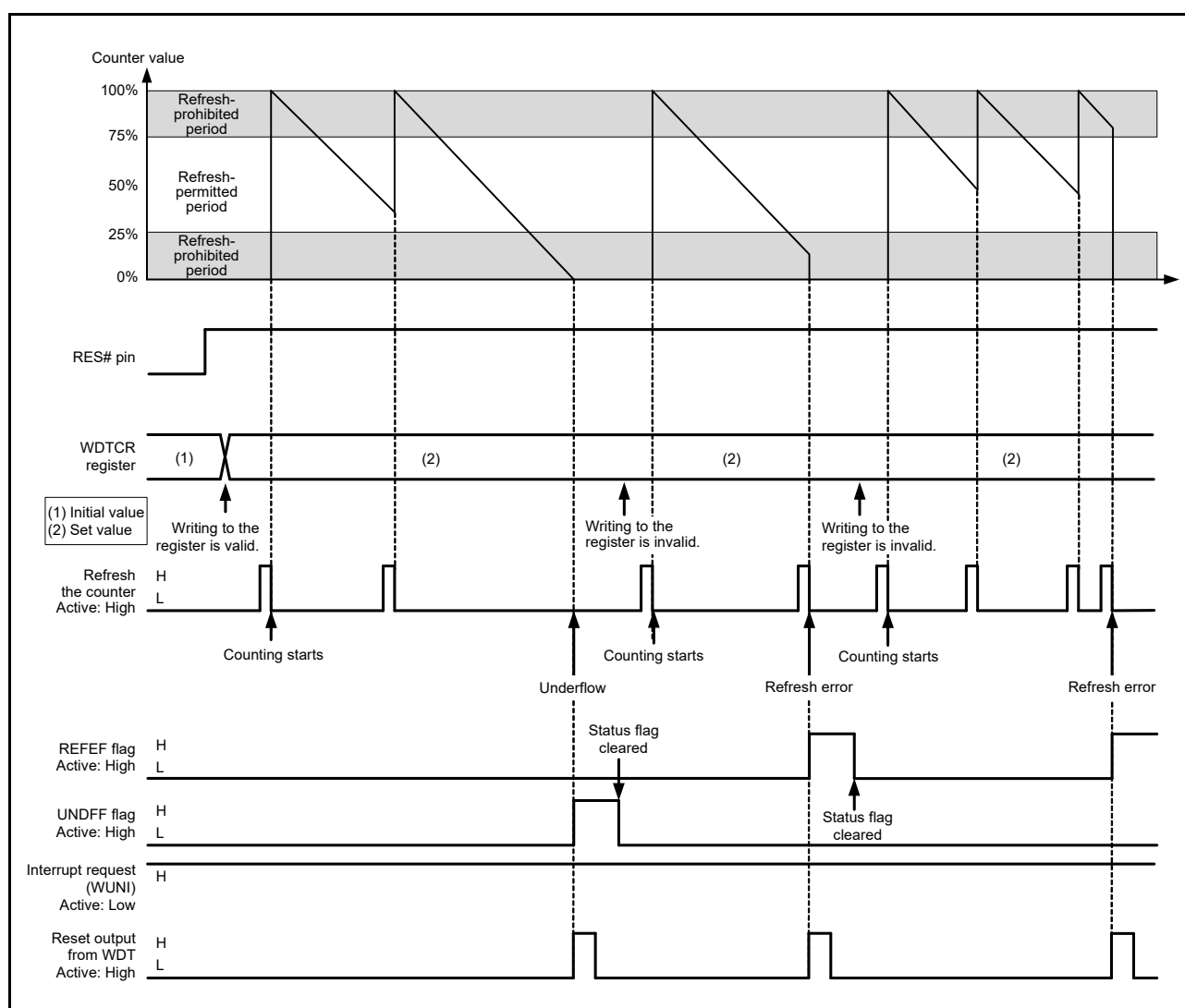
Figure 32.3 Operation Example in Register Start Mode
