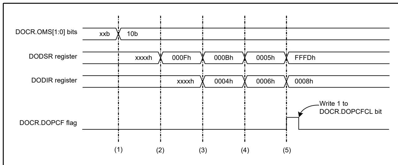
Figure 56.4 Example of Operation in Data Subtraction Mode
