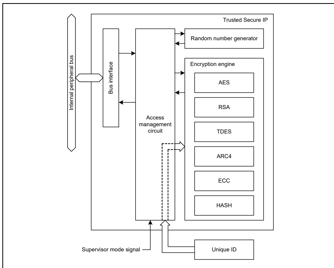
Figure 52.1 Trusted Secure IP Block Diagram
