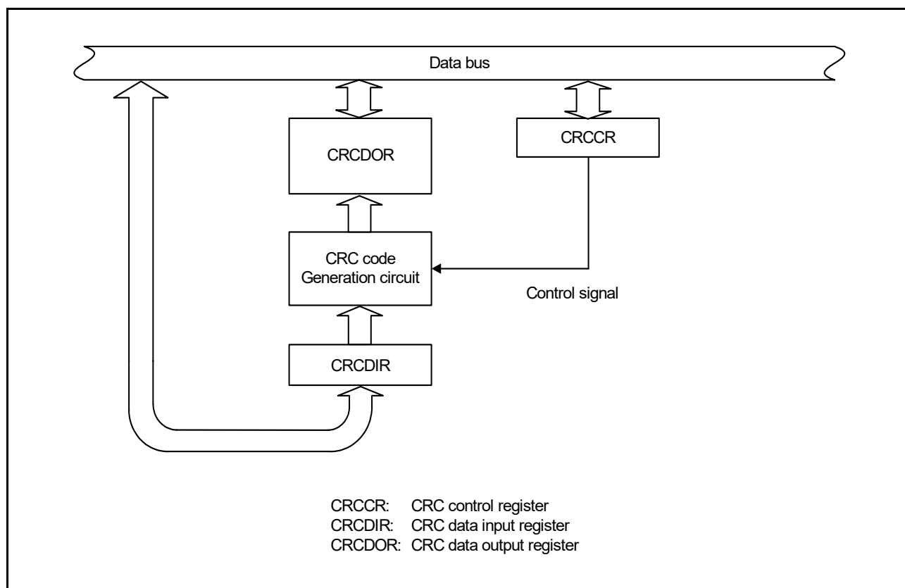
Figure 42.1 CRC Block Diagram
