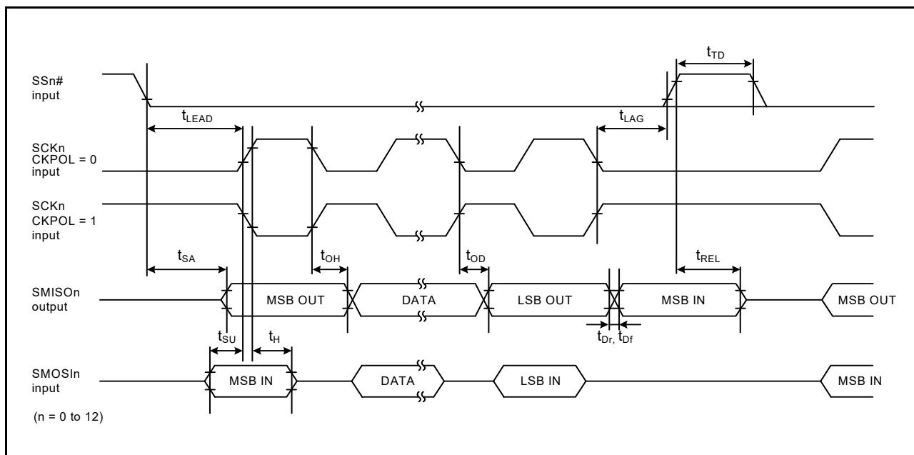
Figure 60.52 Simple SPI Timing (Slave, CKPH = 1)
