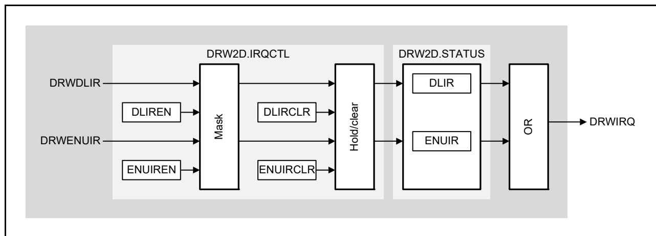
Figure 48.3 Interrupt Controller Unit
