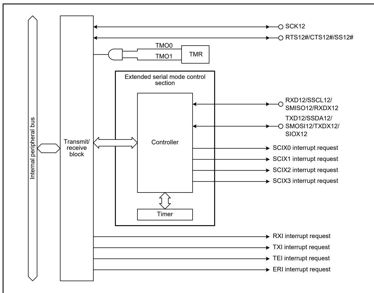
Figure 37.4 Block Diagram of SC1h (SCI12)
