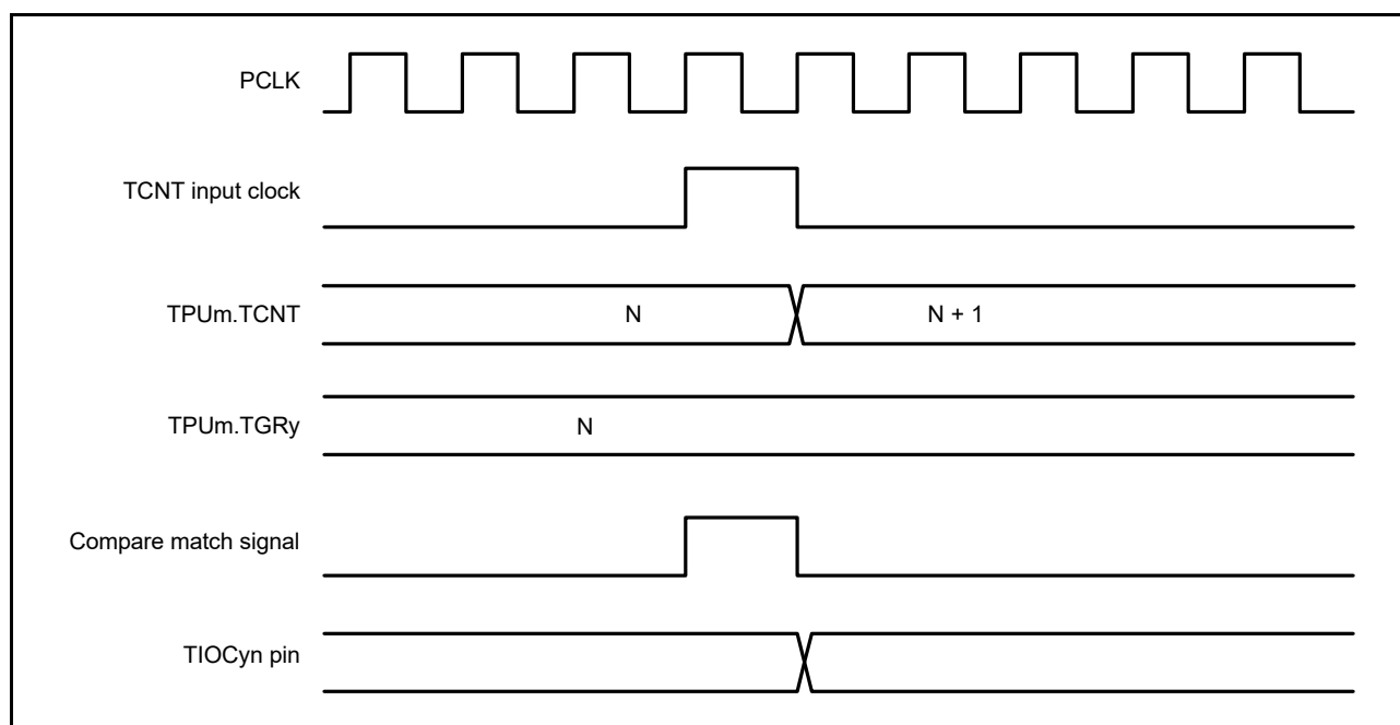
Figure 26.33 Output Compare Output Timing
