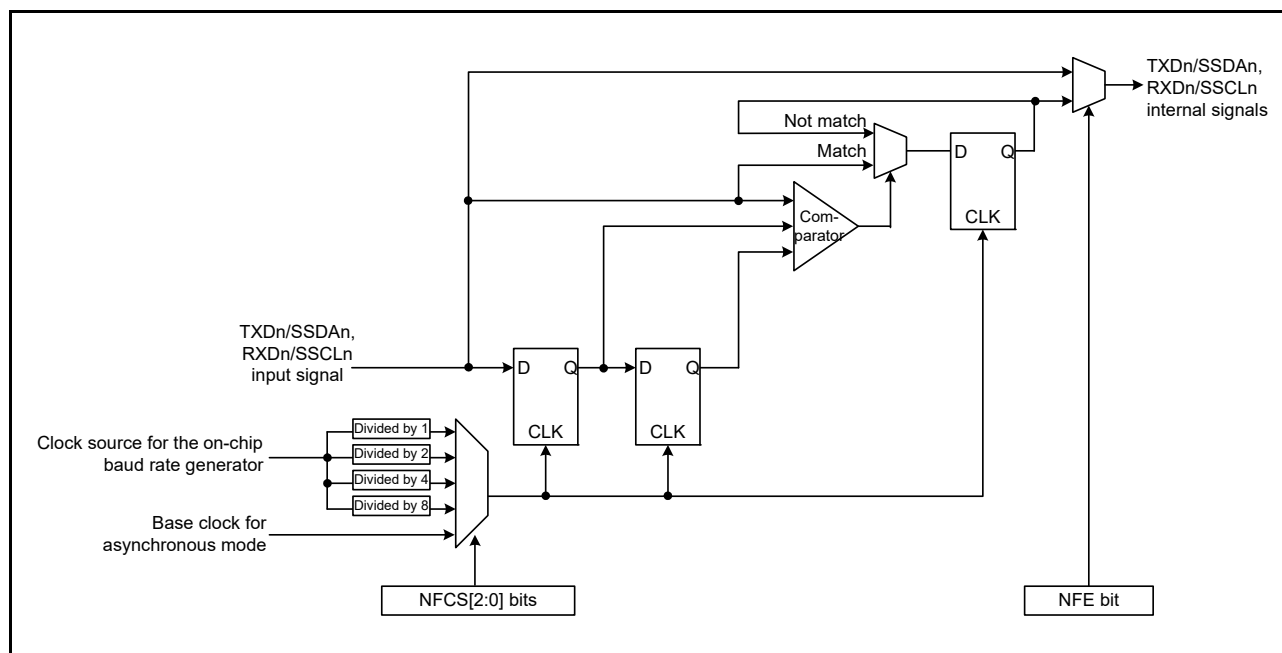
Figure 37.79 Block Diagram of Digital Noise Filter
