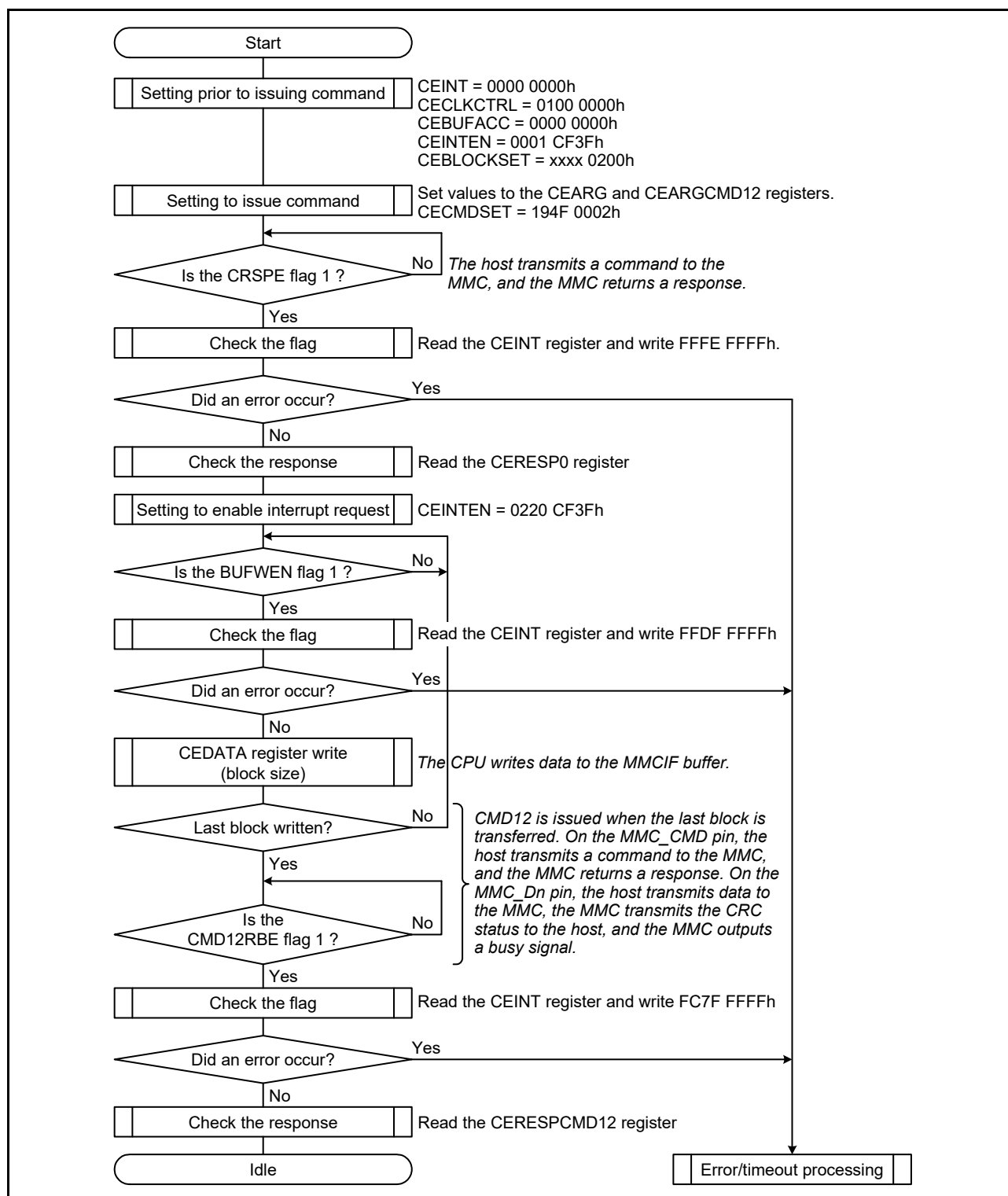
Figure 45.20 Issuing a Multi-Block Write Command (CMD25 Open-Ended)
