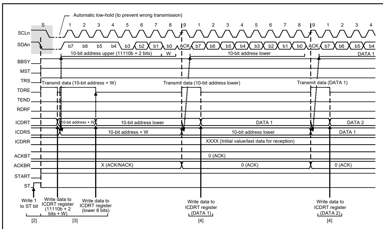
Figure 38.7 Master Transmit Operation Timing (2) (10-Bit Address Format)
