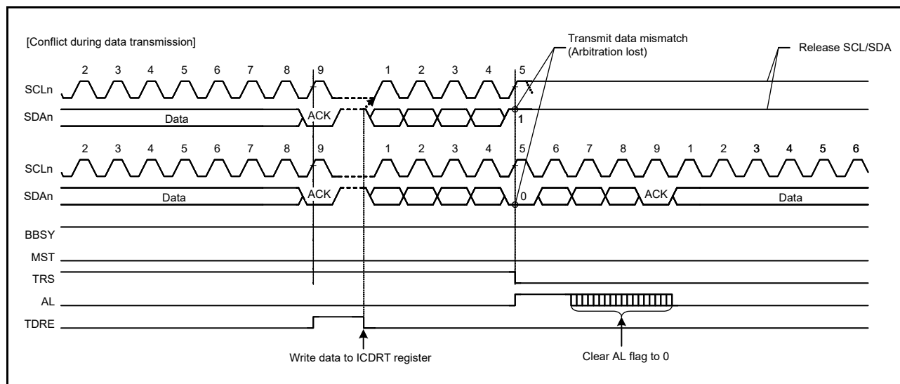
Figure 38.35 Example of Slave Arbitration-Lost Detection (SALE = 1)
