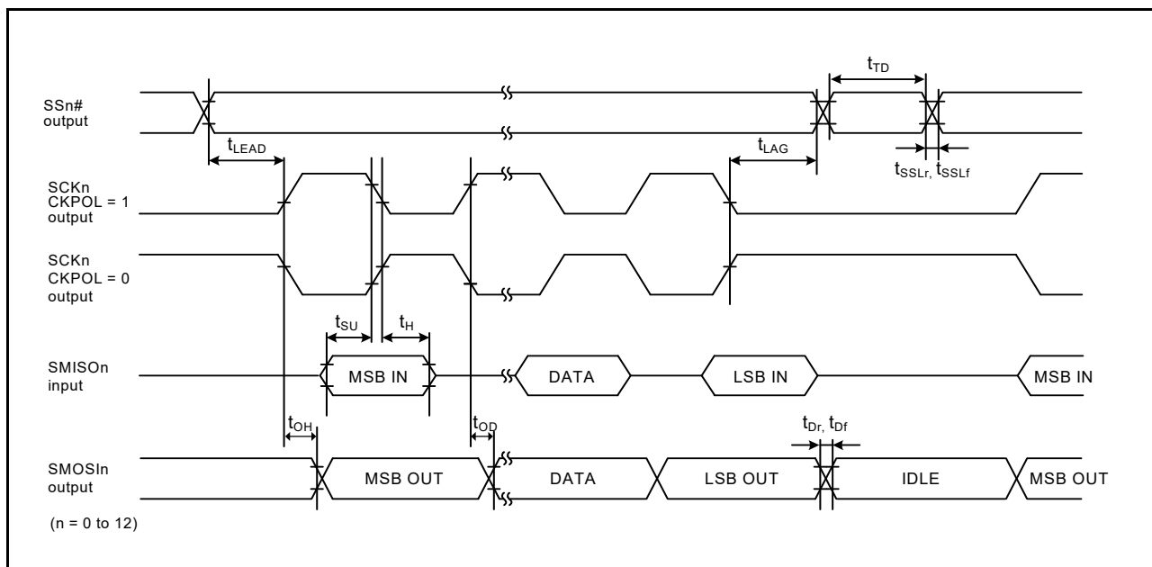
Figure 60.51 Simple SPI Timing (Master, CKPH = 0)
