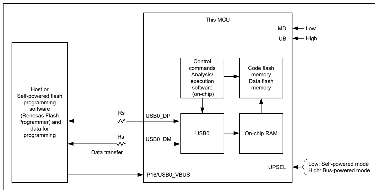
Figure 59.9 System Configuration in Boot Mode (USB Interface)
