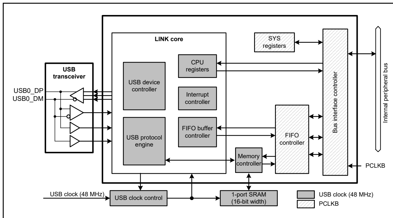
Figure 36.1 USB Block Diagram
