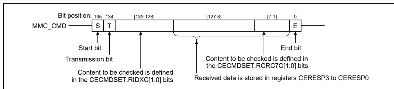
Figure 45.4 17-Byte Response Format (R2 Response)
