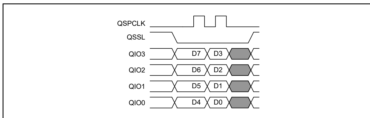
Figure 41.5 Transfer Format in Quad-SPI Format
