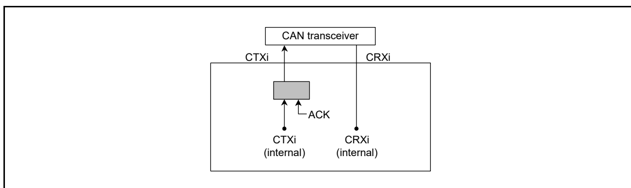
Figure 39.7 Connection when Self-Test Mode 0 is Selected ( i = 0, 1 )
