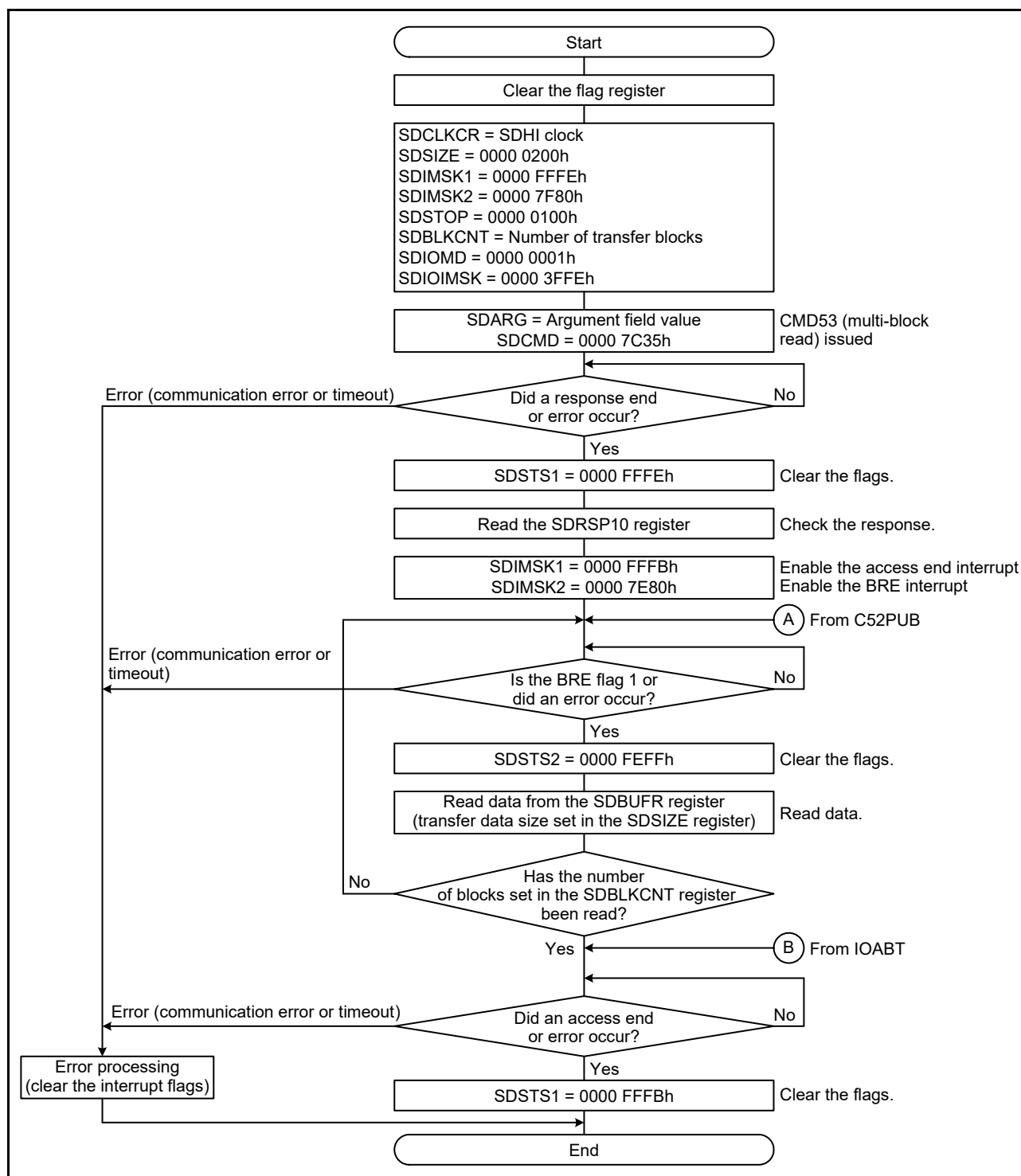
Figure 43.15 Issuing the IO_RW_EXTENDED Command (CMD53/Multi-Block Read)
