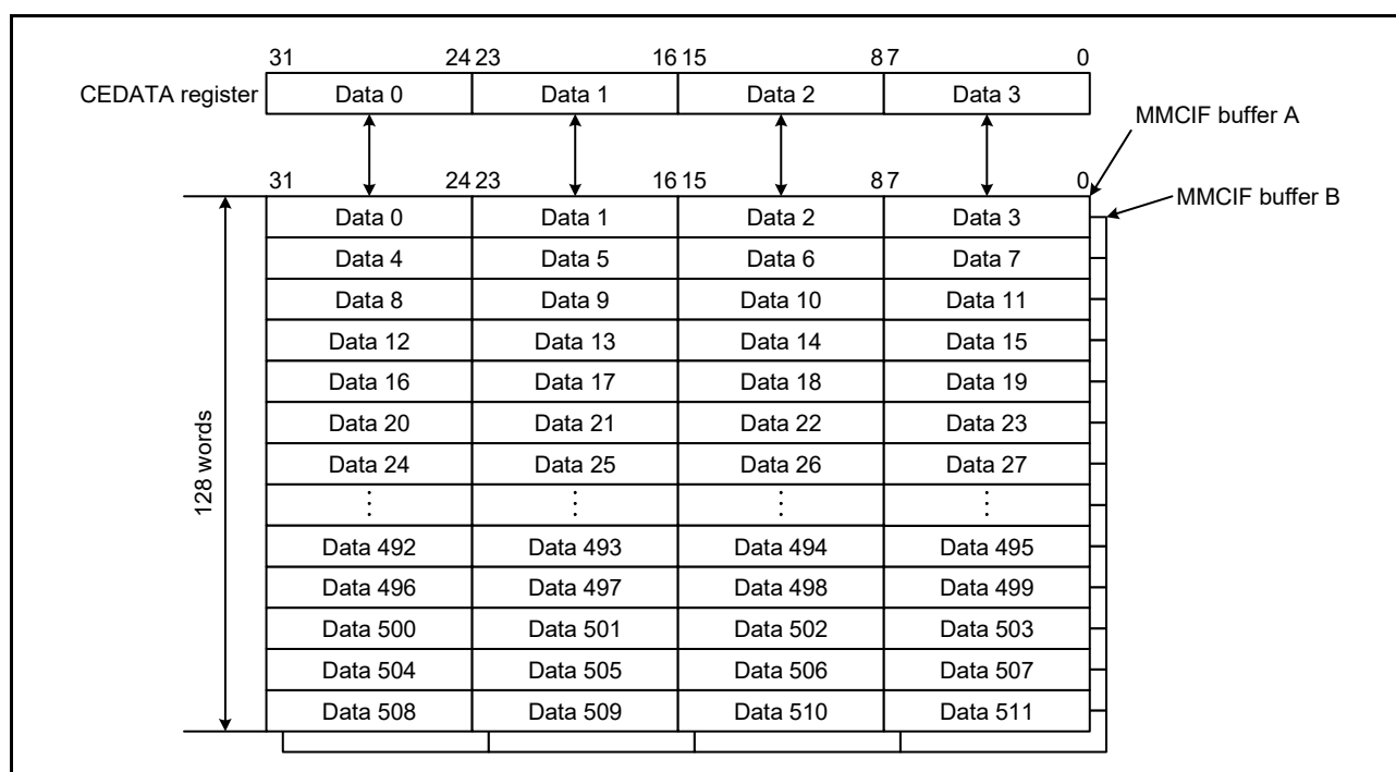
Figure 45.6 MMCIF Buffer Structure (32-Bit Access)
