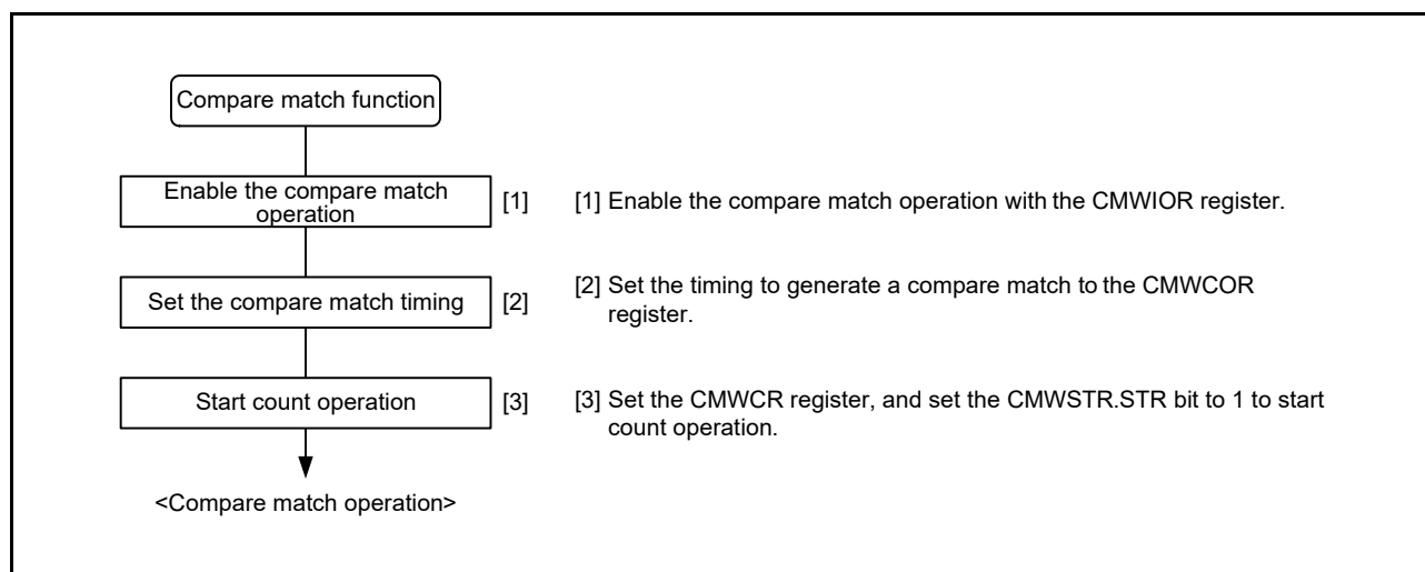
Figure 30.3 Procedure for Setting Compare Match Operation
