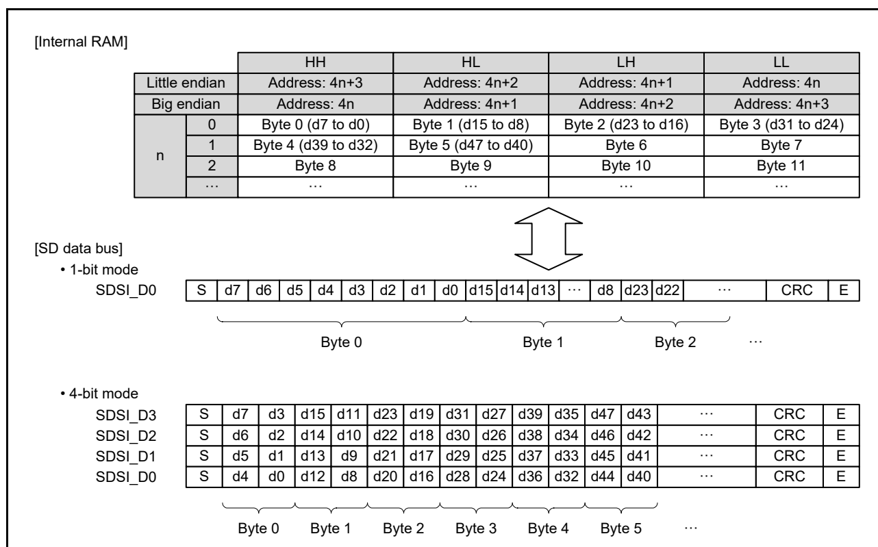
Figure 44.5 Data Format (Without Data Swapping)
