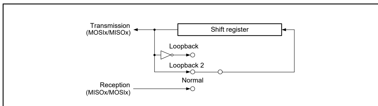
Figure 40.50 Configuration of Shift Register I/O Paths in Loopback Mode (Master Mode)
