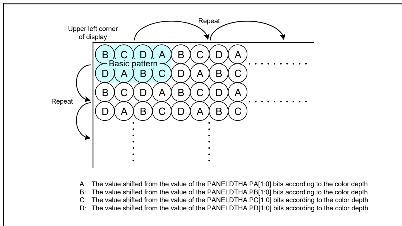
Figure 47.13 Addition Value Selection Method for 2×2 Pattern Dither
