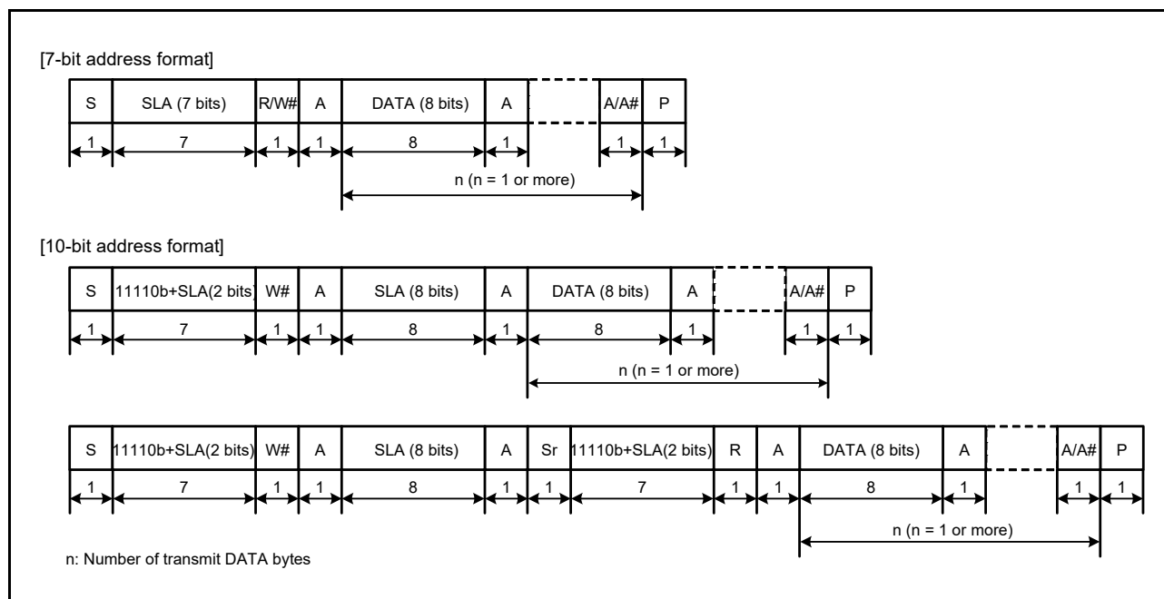
Figure 38.2 I 2 C-bus Format
