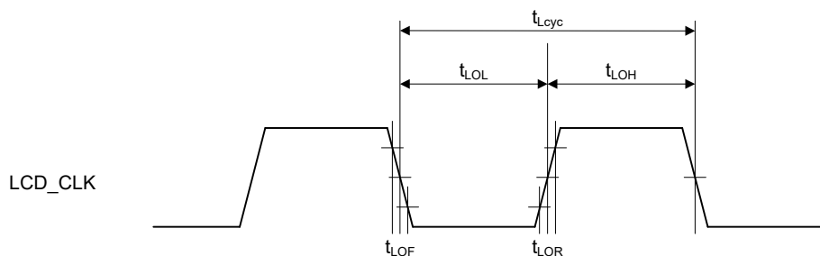
Figure 60.80 LCD_CLK Clock Output Timing
