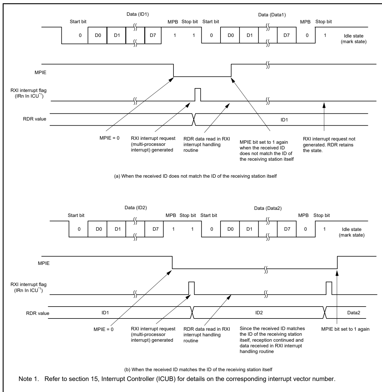
Figure 37.24 Example of SCI Reception (8-Bit Data/Multi-Processor Bit/1 Stop Bit)
