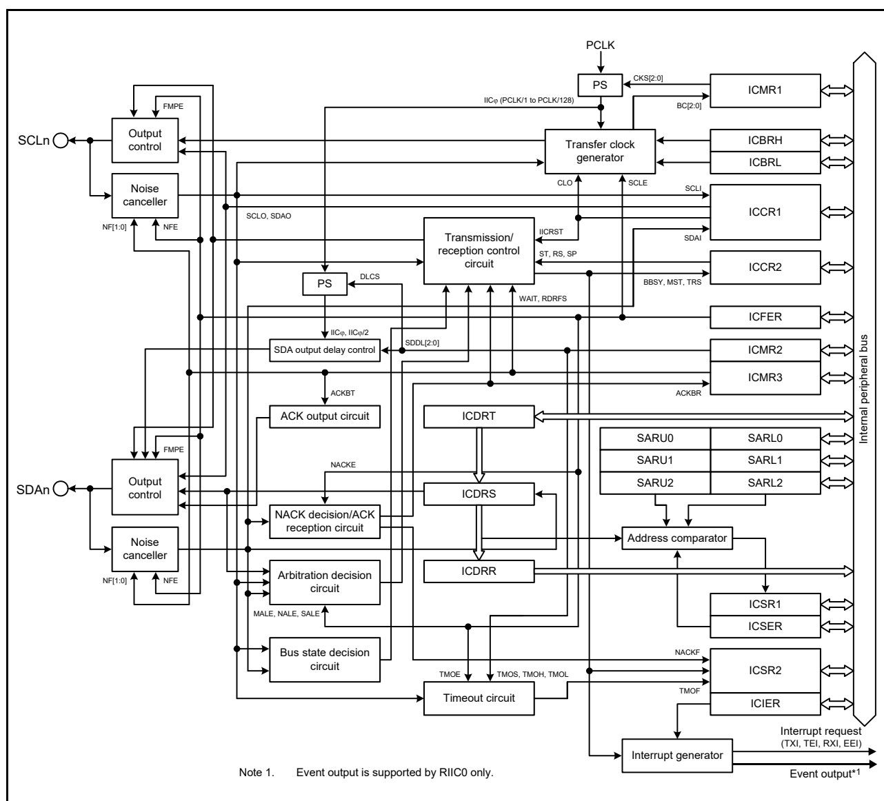
Figure 38.1 RIIC Block Diagram (n = 0 to 2)
