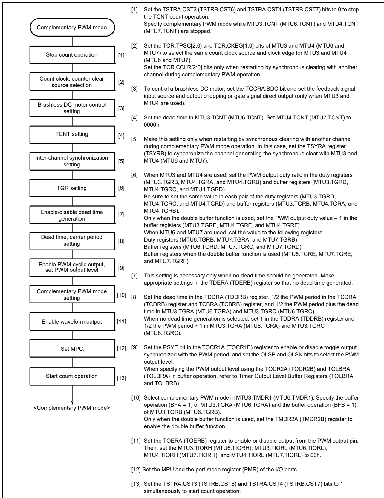
Figure 24.48 Example of Complementary PWM Mode Setting Procedure
