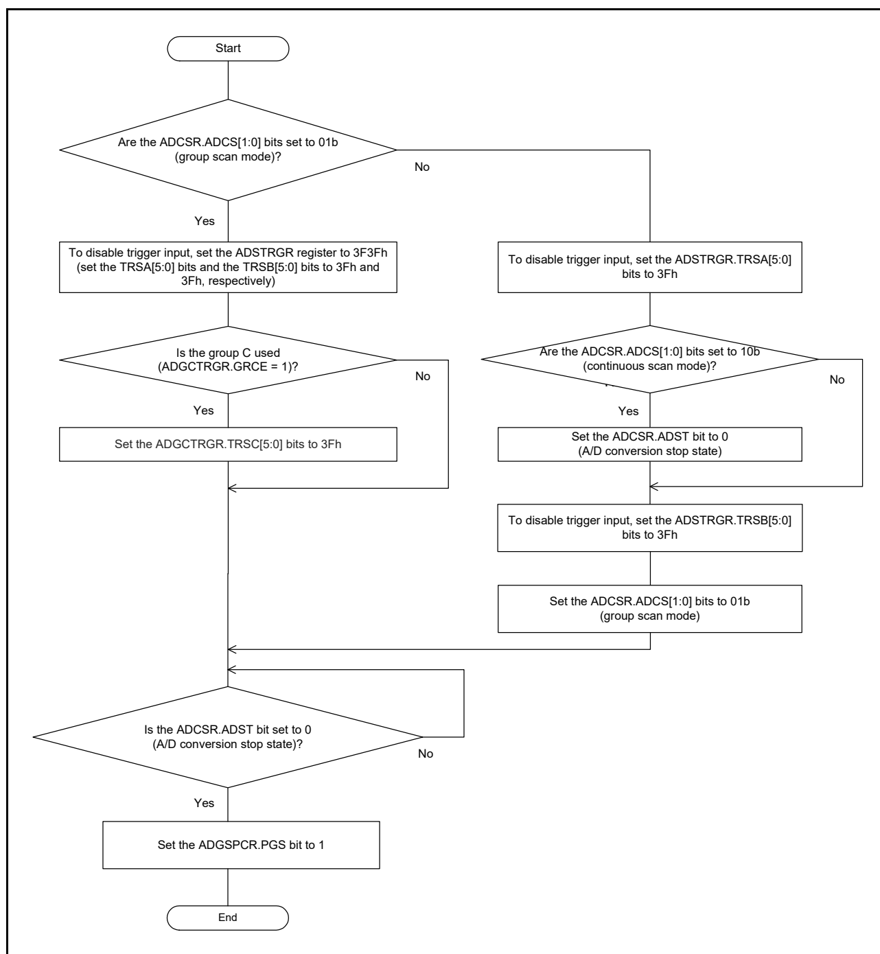
Figure 53.24 Flow of Setting the ADGSPCR.PGS Bit
