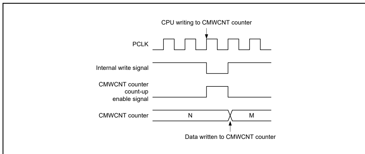
Figure 30.24 Conflict between CMWCNT Counter Writing and Incrementing
