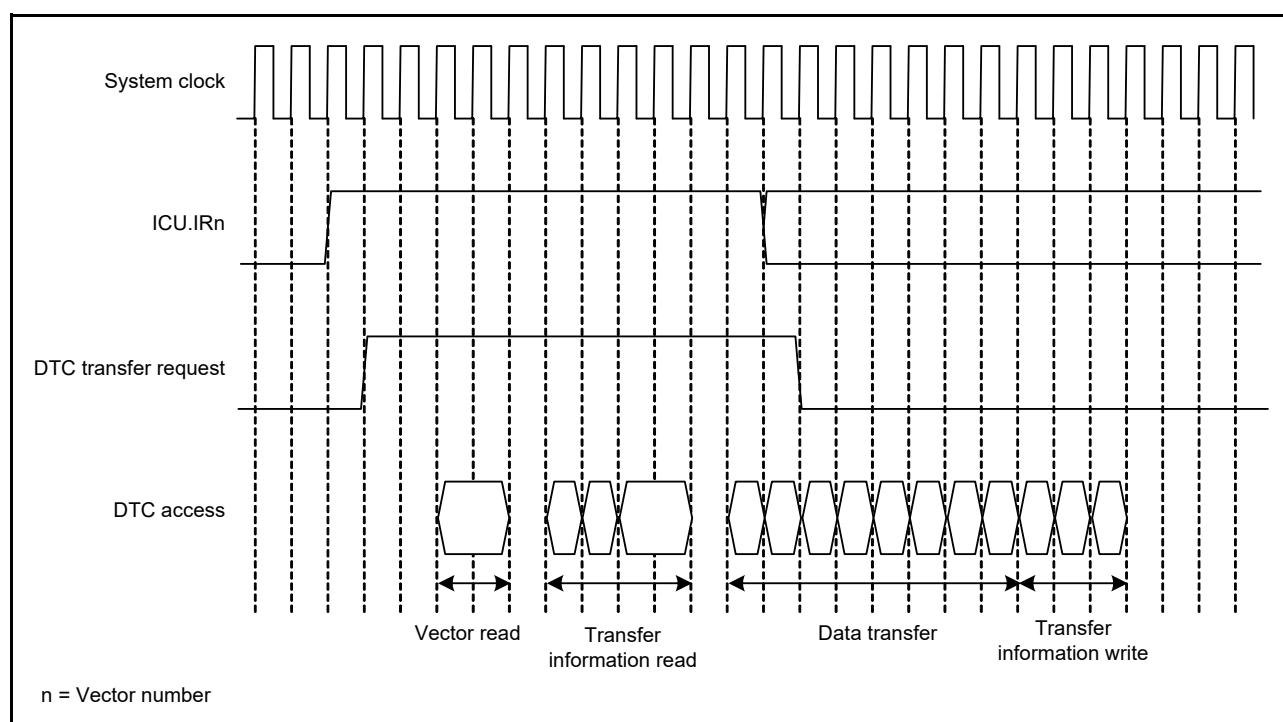
Figure 20.11 Example (2) of DTC Operation Timing (Short-Address Mode, Block Transfer Mode, Block Size = 4)
