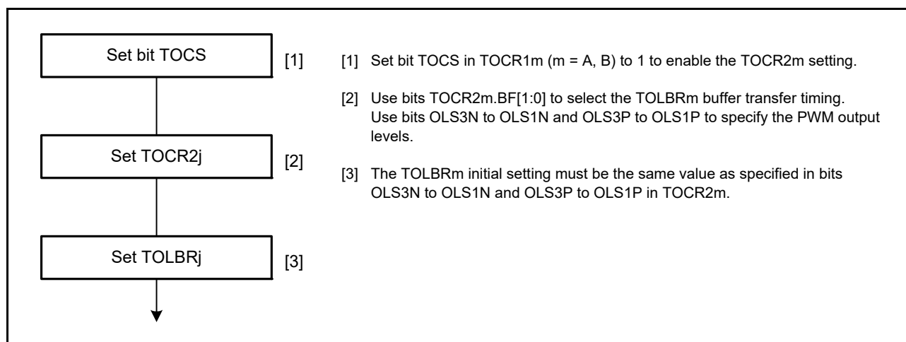
Figure 24.4 Example of PWM Output Level Setting Procedure in Buffer Operation
