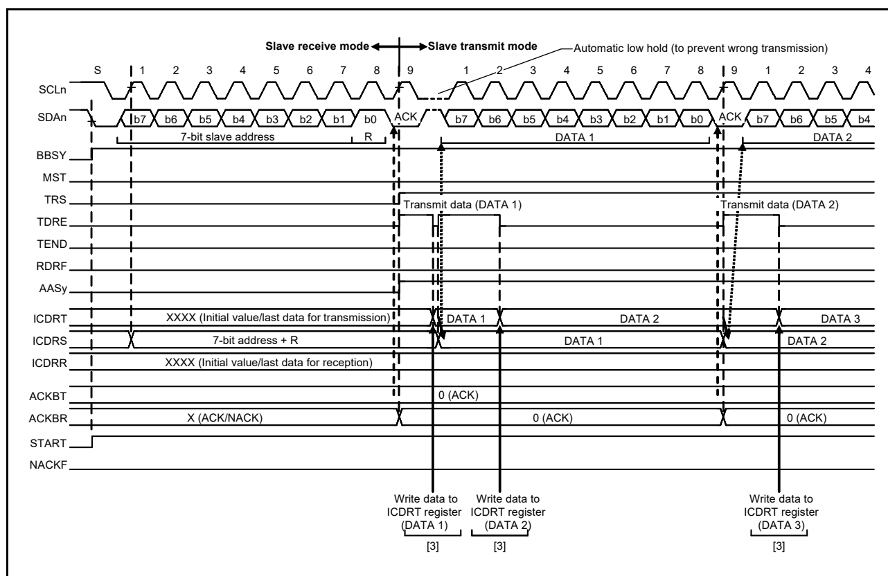
Figure 38.15 Slave Transmit Operation Timing (1) (7-Bit Address Format)
