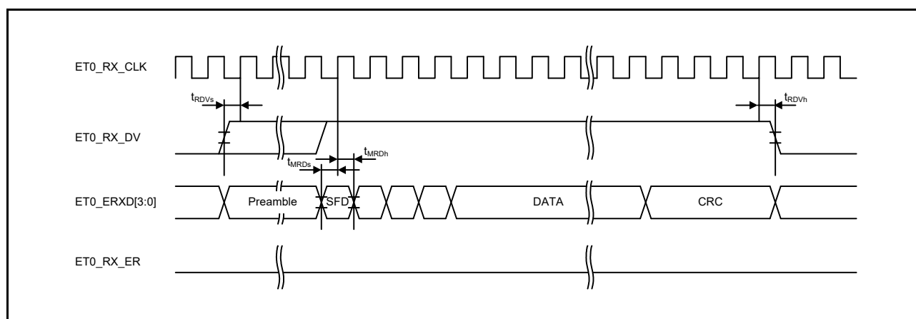
Figure 60.73 MII Reception Timing (Normal Operation)
