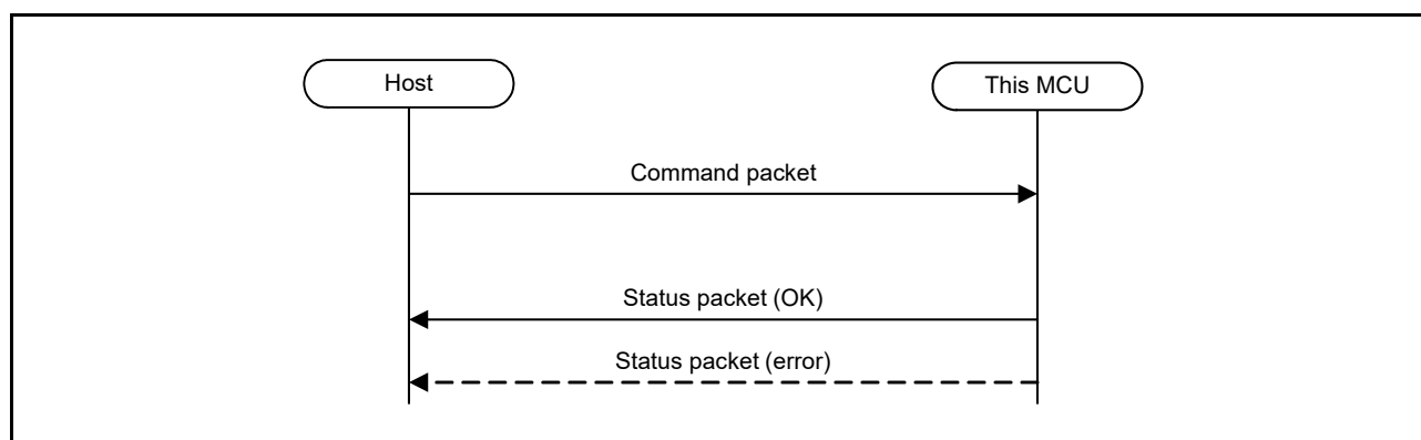
Figure 59.17 Common Transfer Sequence for the Commands that Only Make Settings
