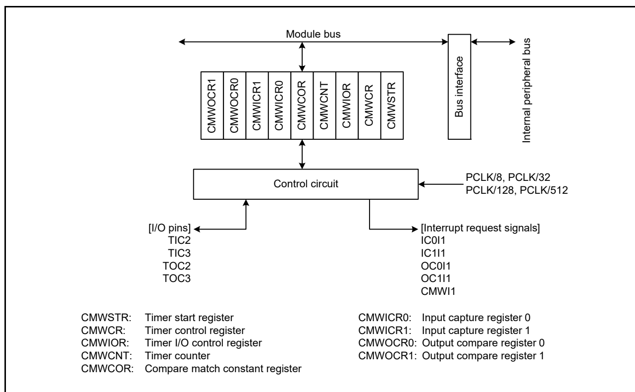
Figure 30.2 CMTW1 Block Diagram
