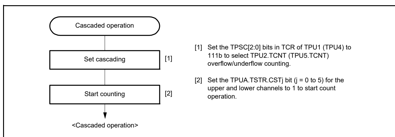
Figure 26.17 Cascaded Operation Setting Procedure
