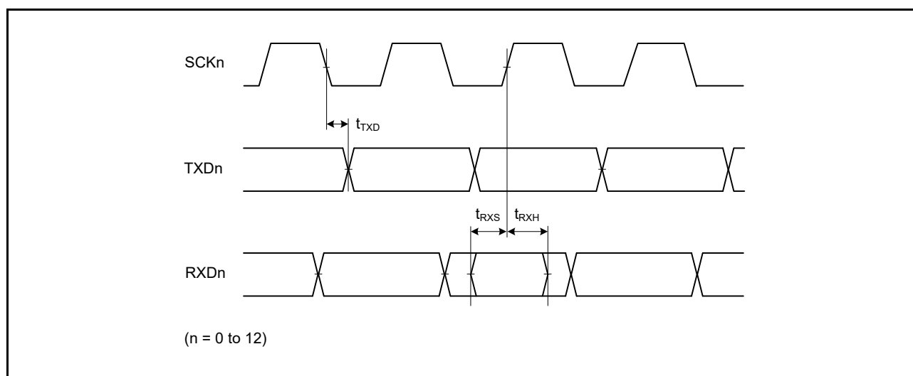
Figure 60.47 SCI Input/Output Timing: Clock Synchronous Mode
