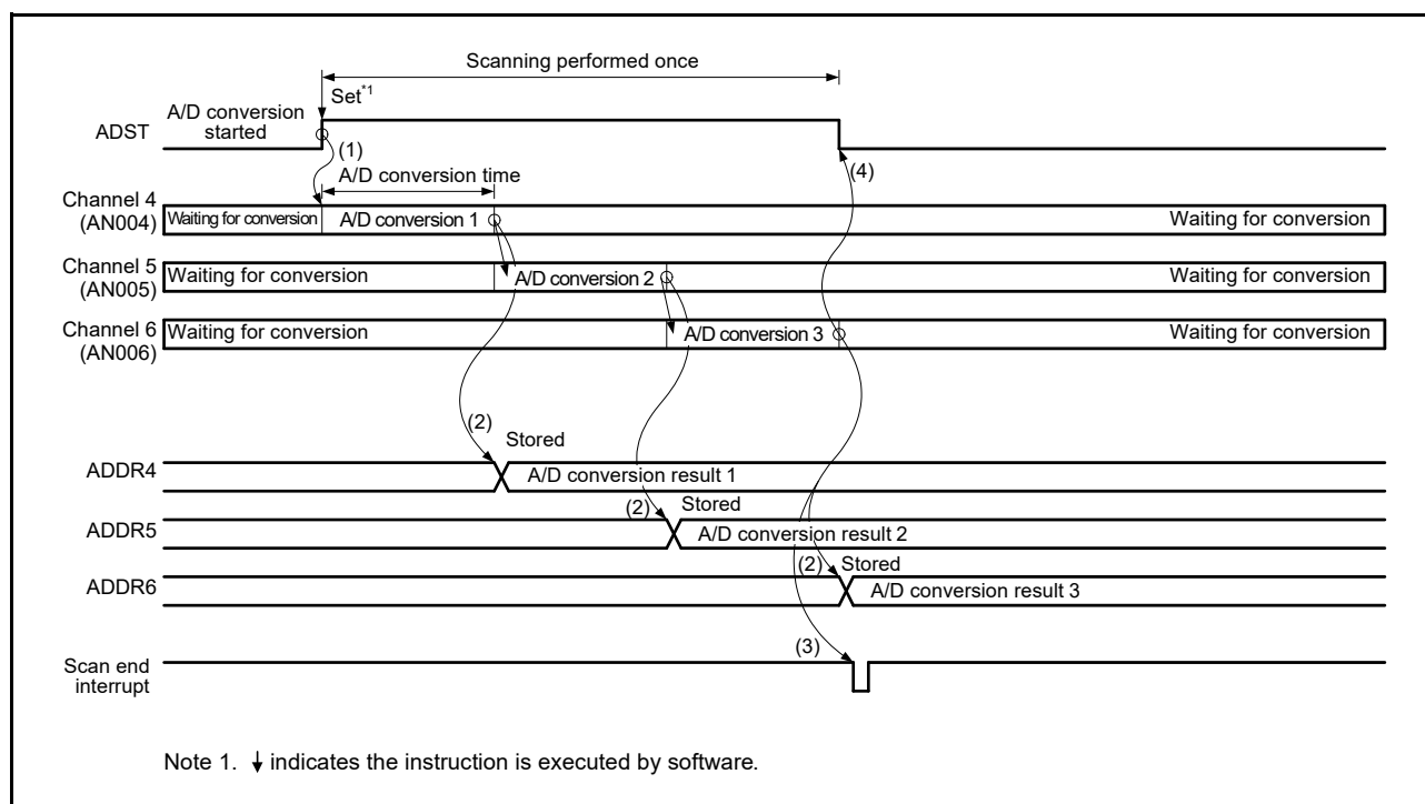
Figure 53.6 Example of Operation in Single Scan Mode (Basic Operation: AN004, AN005, AN006 Selected)
