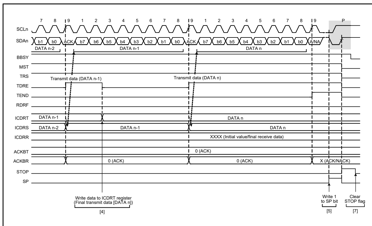
Figure 38.8 Master Transmit Operation Timing (3)
