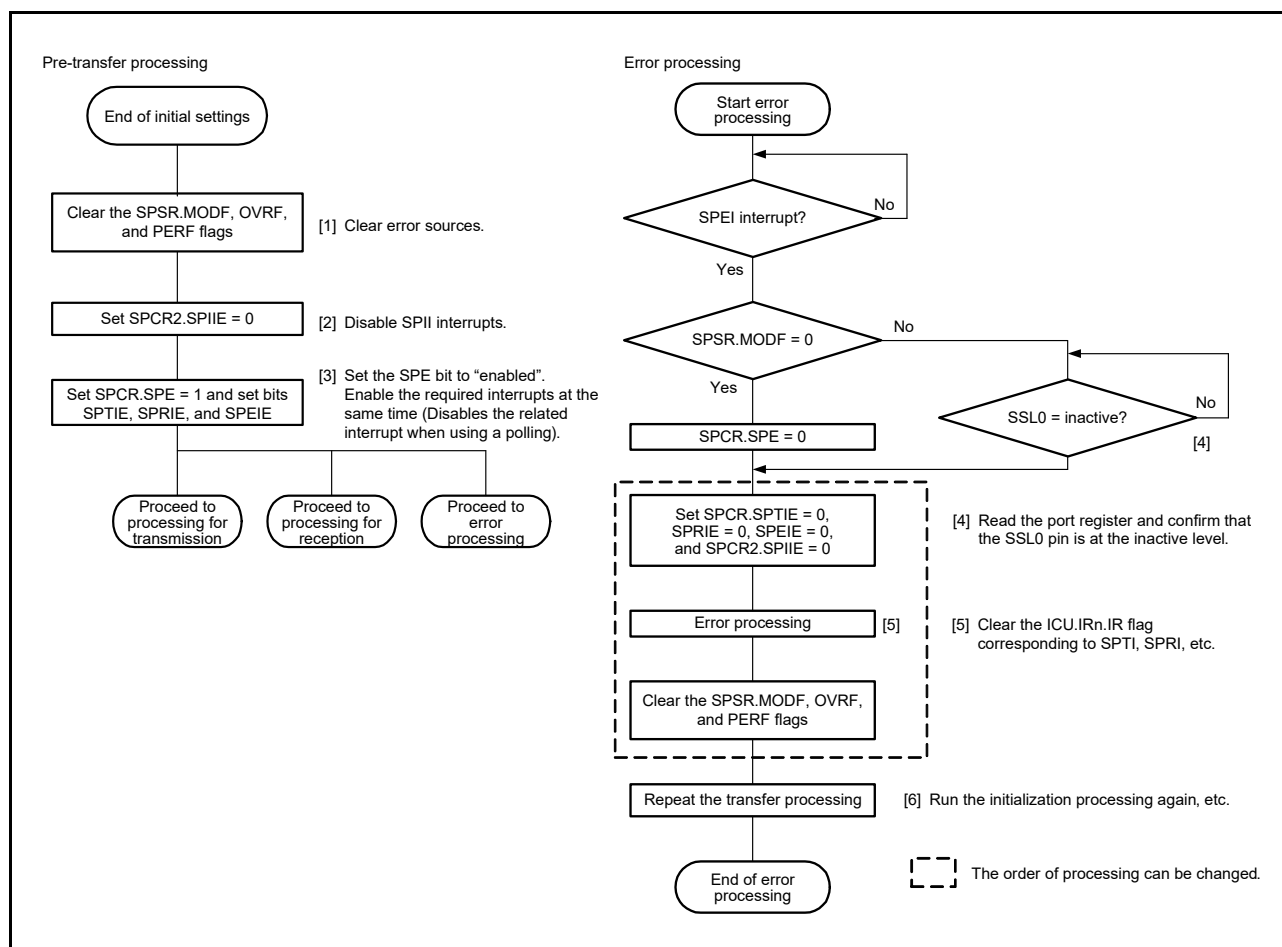
Figure 40.40 Flowchart for Master Mode (Error Processing)
