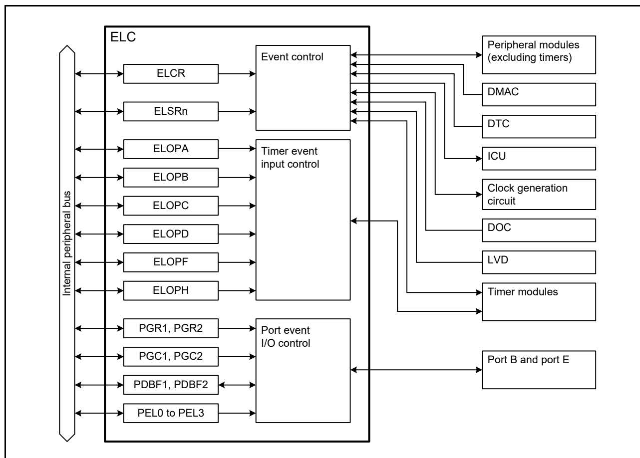
Figure 21.1 ELC Block Diagram (n = 0, 3, 4, 7, 10 to 13, 15, 16, 18 to 28, 33, 35 to 38, 45)
