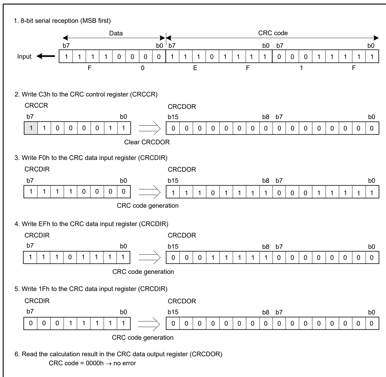
Figure 42.5 MSB First Data Reception
