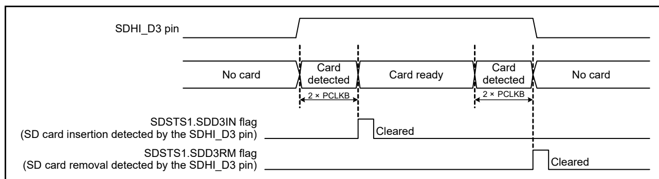
Figure 43.7 SD Card Detection Using the SDHI_D3 Pin
