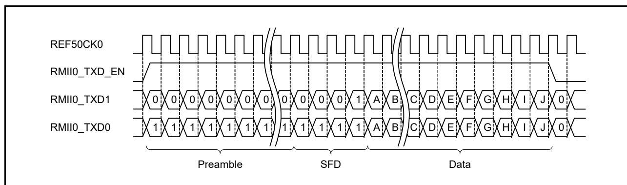
Figure 34.11 RMII Frame Transmit Timing During Normal Transmission
