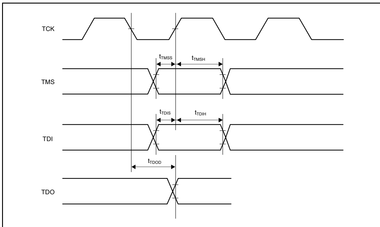
Figure 60.99 Boundary Scan Input/Output Timing
