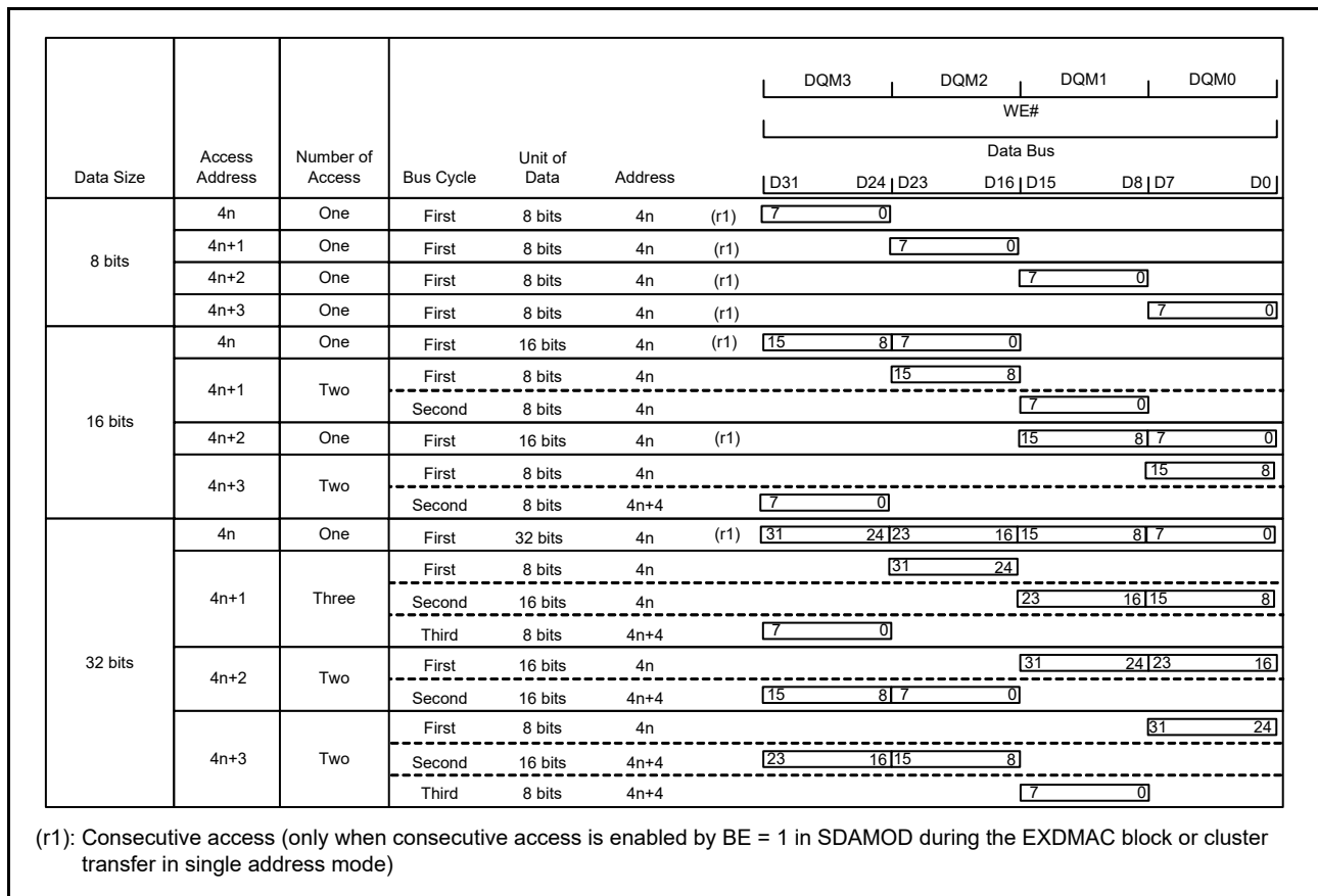
Figure 16.13 Data Alignment (Big Endian) in 32-Bit Bus Space
