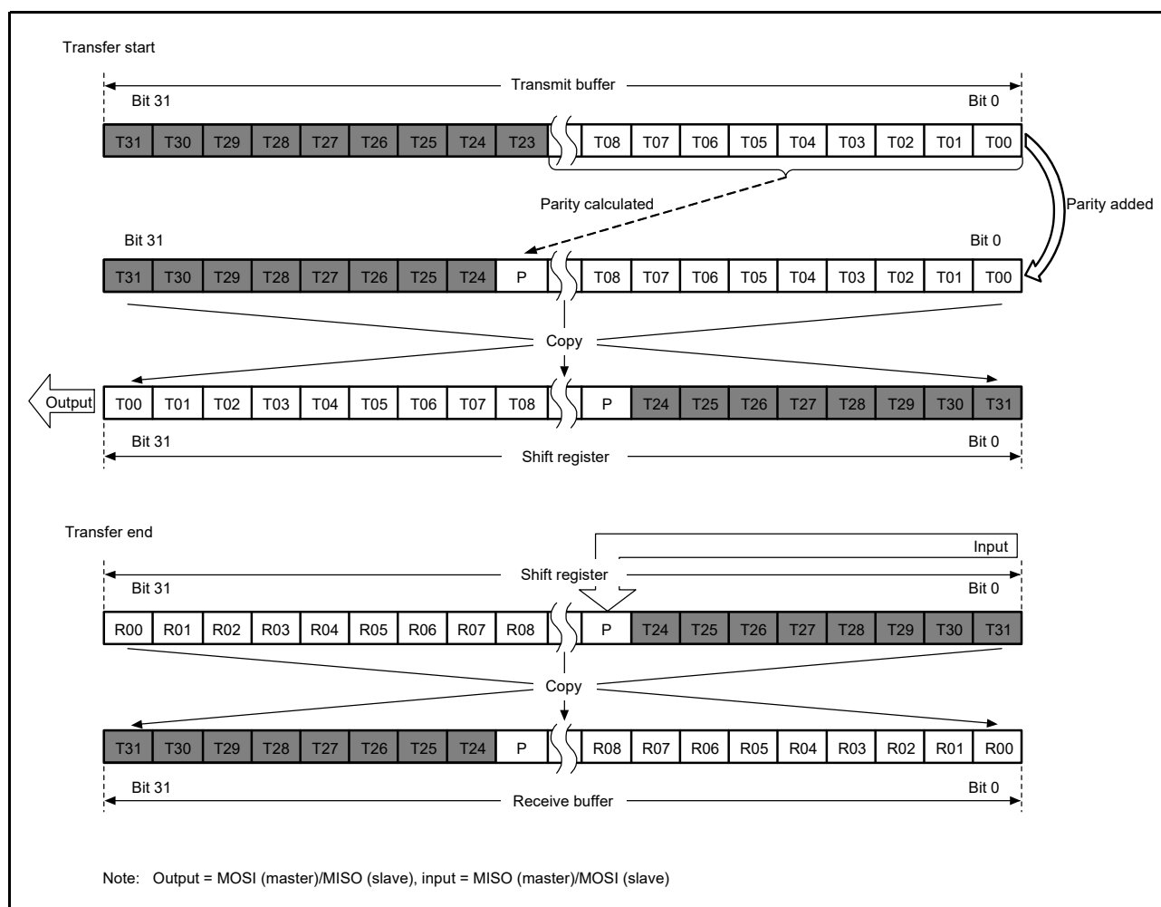
Figure 40.21 LSB First Transfer (24-Bit Data, Parity Enabled)
