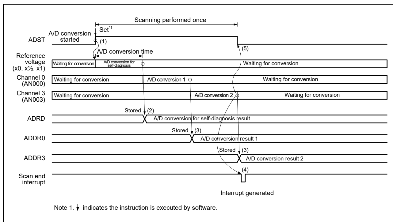
Figure 53.9 Example of Operation in Single Scan Mode (Basic Operation: AN000, AN003 Selected + Self-Diagnosis)
