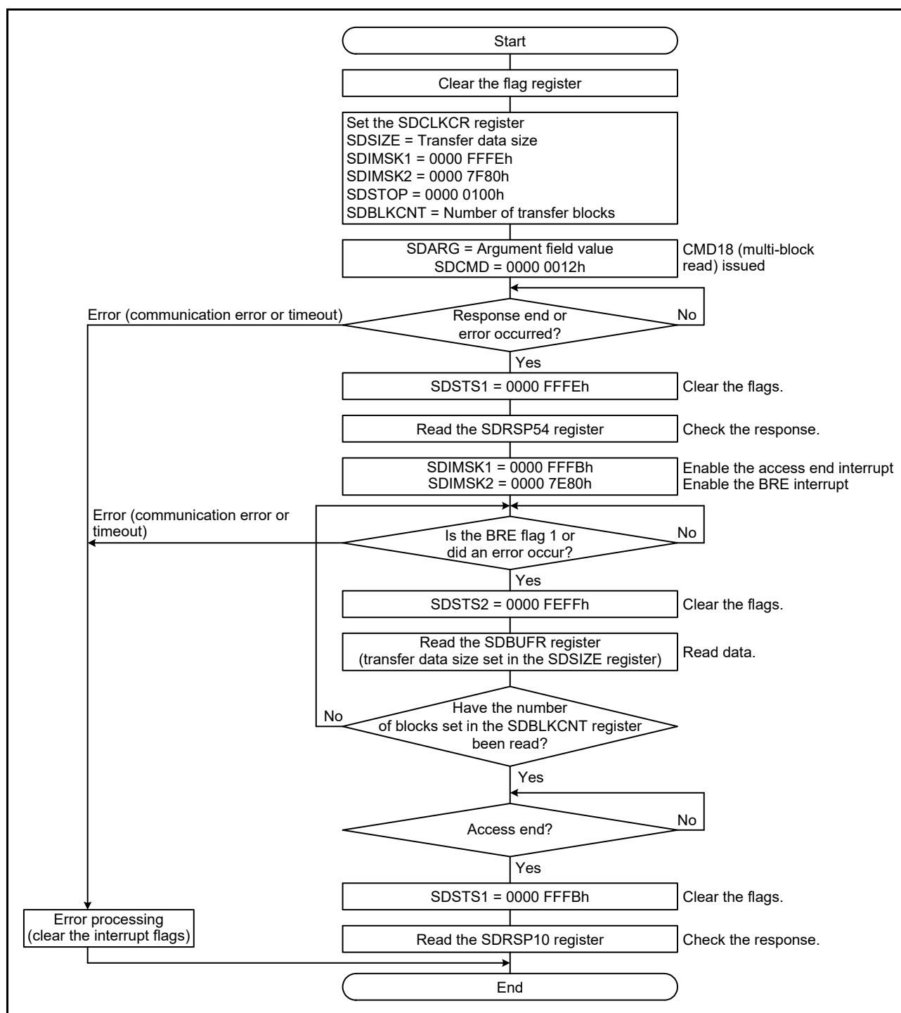
Figure 43.12 Issuing the Multi-Block Read Command
