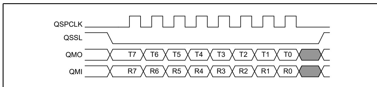
Figure 41.3 Transfer Format in Single-SPI Format
