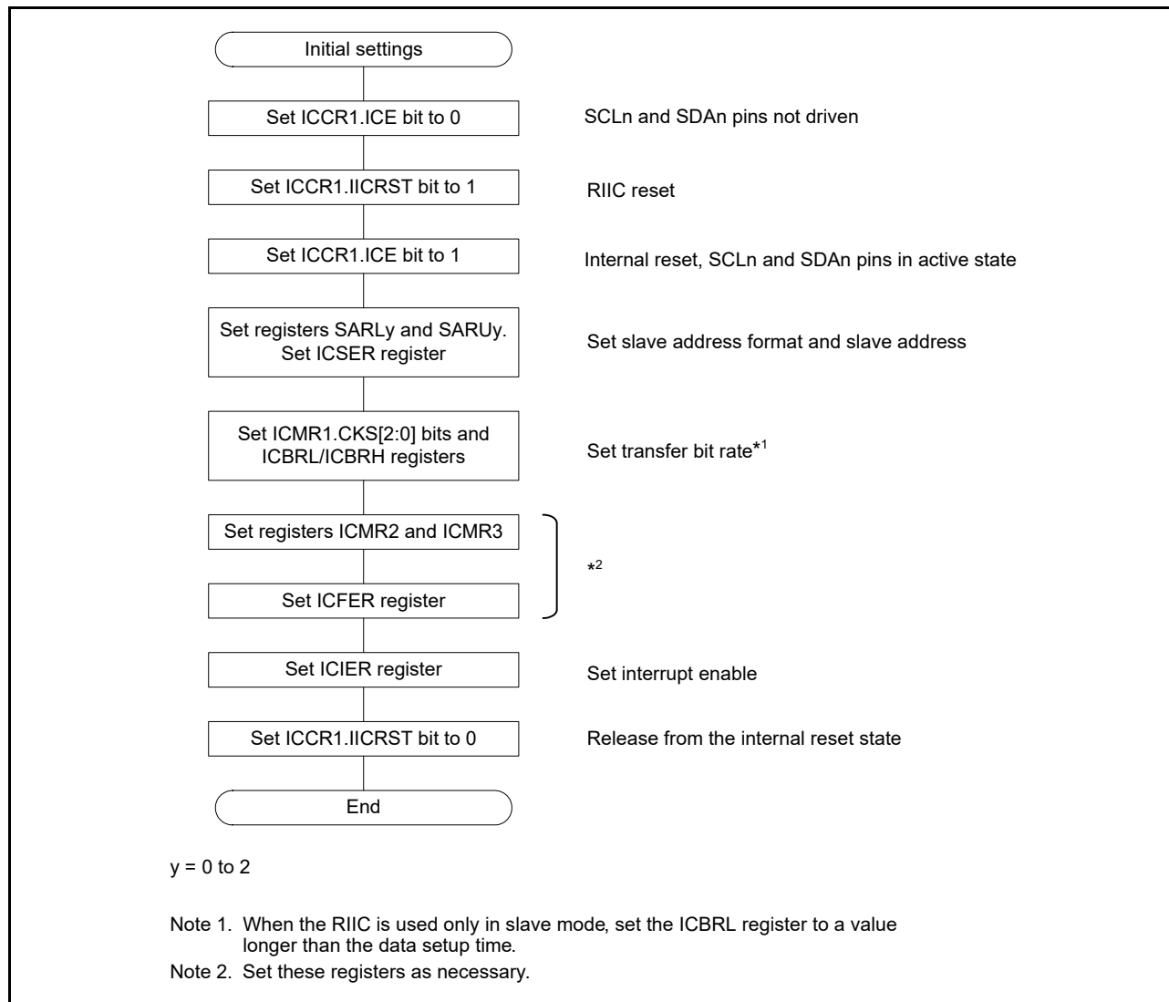
Figure 38.4 Example of RIIC Initialization Flowchart
