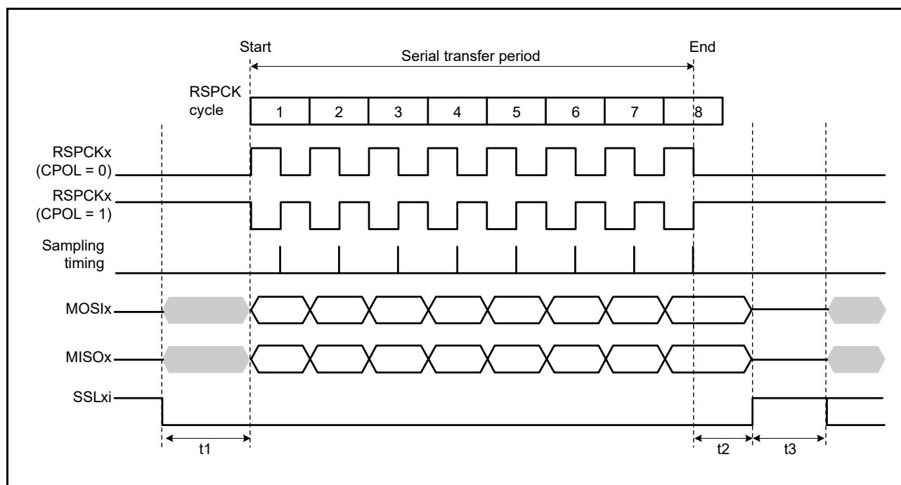
Figure 40.25 RSPI Transfer Format (CPHA = 1)
