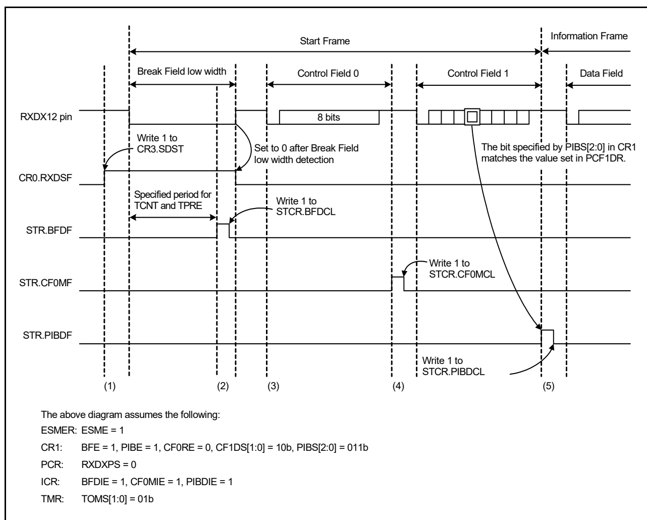
Figure 37.72 Example of Operations When Receiving a Start Frame While the CR1.PIBE Bit is 1
