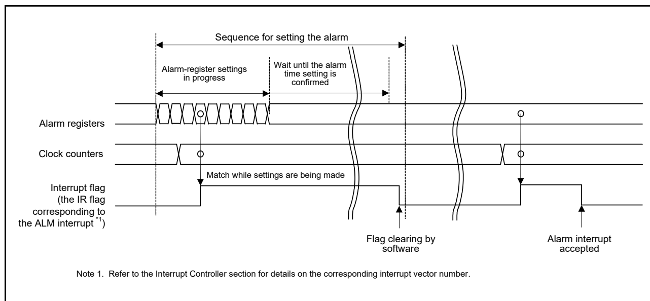
Figure 31.11 Timing Chart for the Alarm Interrupt (ALM)
