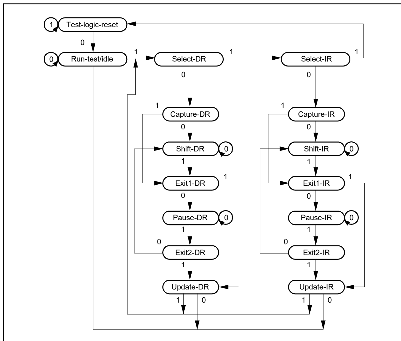
Figure 49.2 State Transition Diagram of TAP Controller
