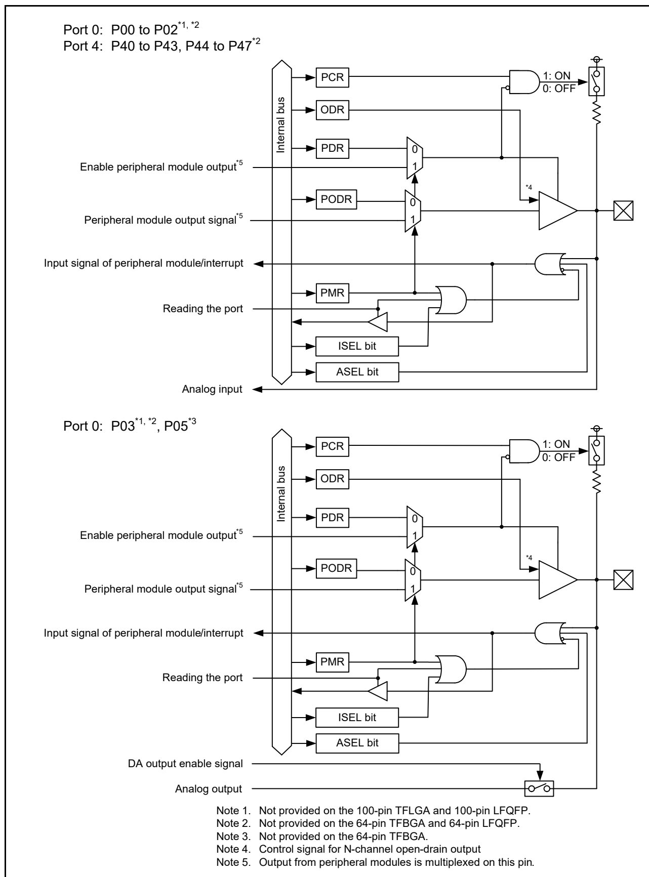
Figure 22.1 I/O Port Configuration (1)
