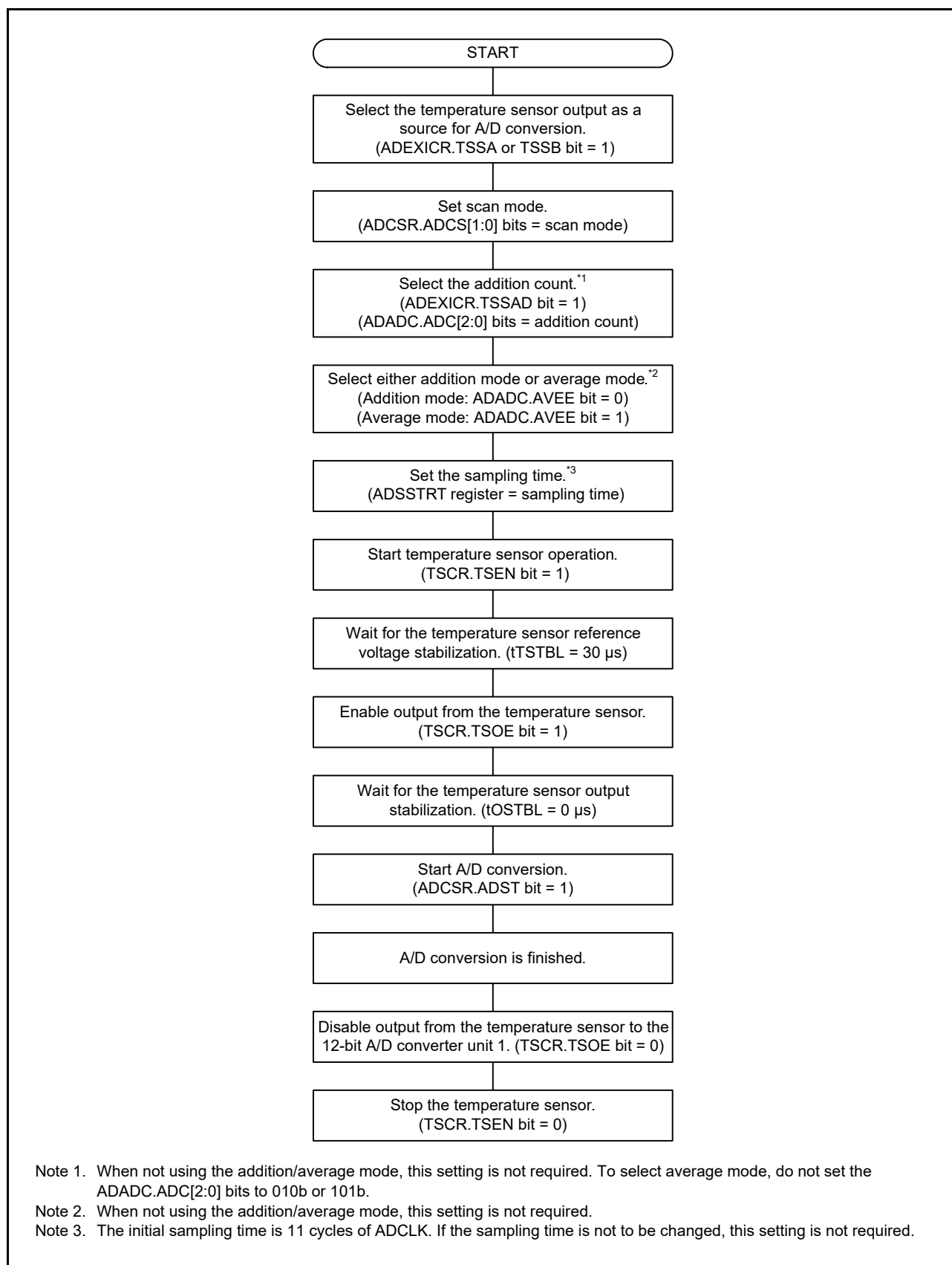
Figure 55.3 Procedure for Using the Temperature Sensor
