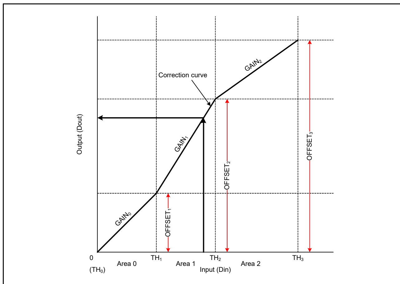
Figure 47.11 Calculation of Gamma Correction Value
