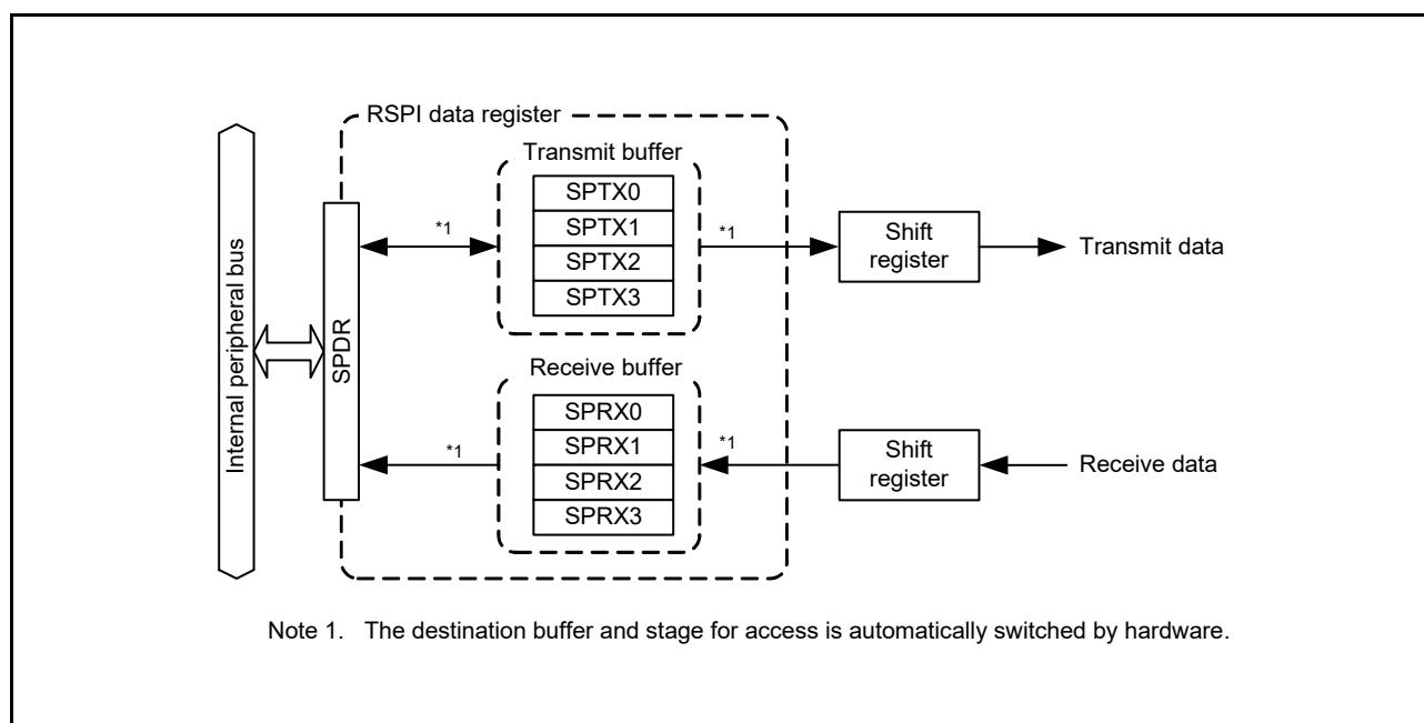
Figure 40.2 Configuration of the SPDR Register
