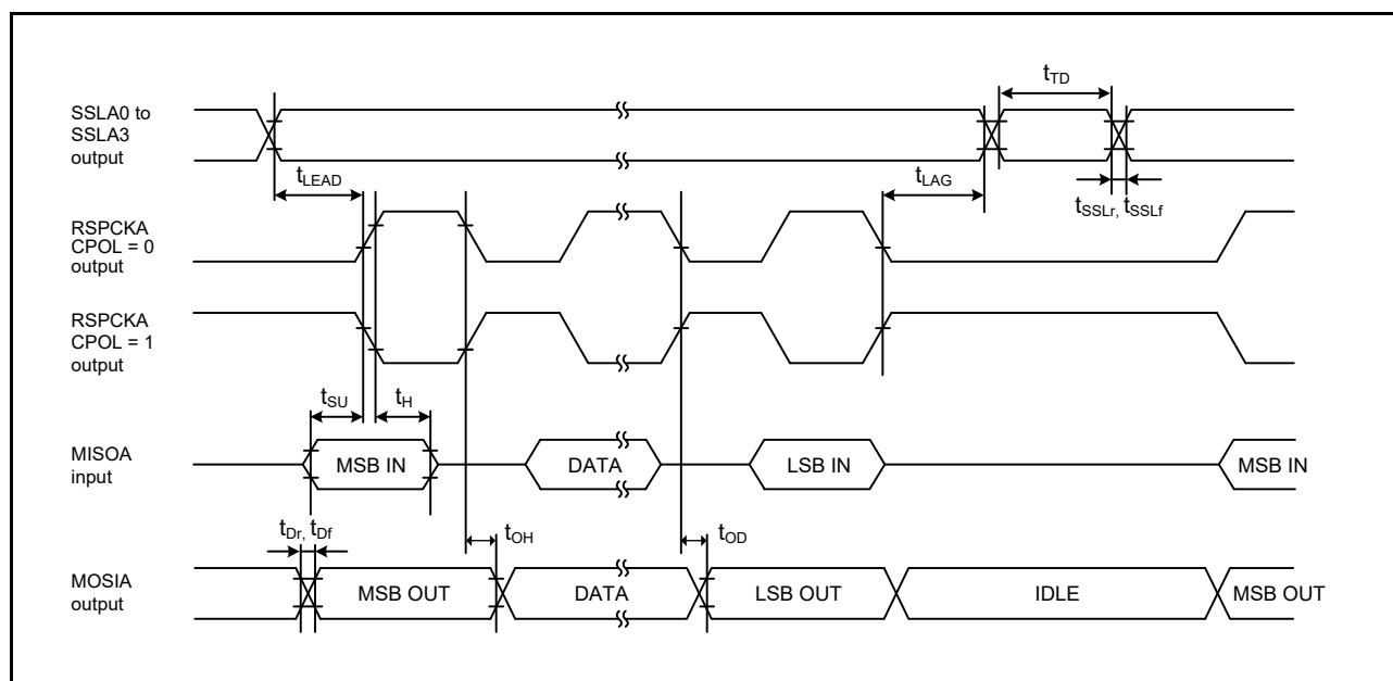
Figure 60.55 RSPI Timing (Master, CPHA = 0) (Bit Rate: PCLKA Division Ratio Set to a Value Other Than 1/2)
