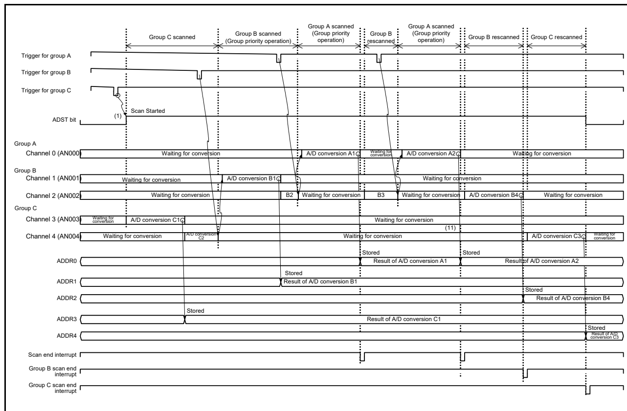
Figure 53.31 Example 2 of Group Priority Operation: Priority Group Trigger Input during Low-Priority Group Rescan, With Rescan Setting (ADGSPCR.GBRSCN = 1, ADGSPCR.GBRP = 0, ADGSPCR.LGRRS = 1)
