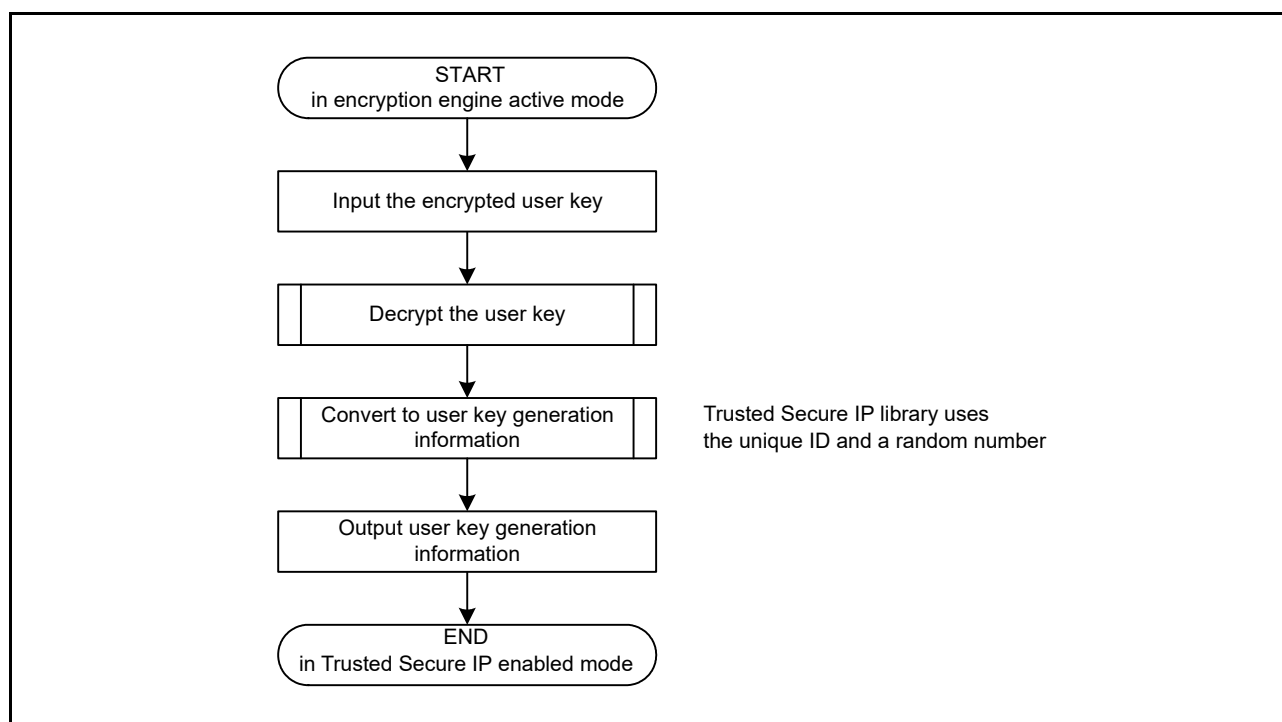
Figure 52.5 Key Installation Flow Chart
