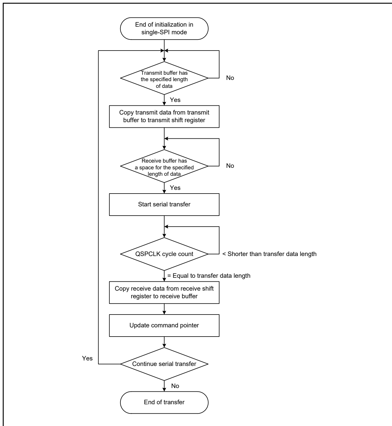
Figure 41.16 Transfer Operation Flowchart in Single-SPI Mode
