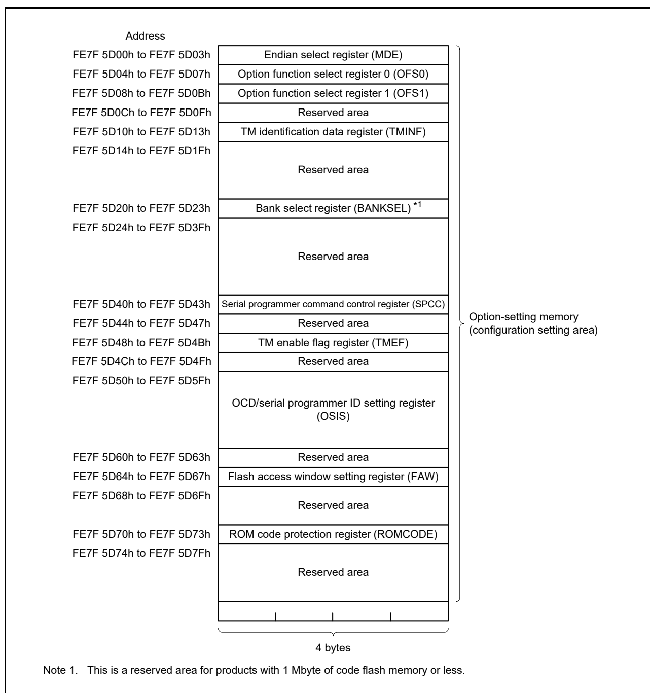
Figure 7.1 Option-Setting Memory
