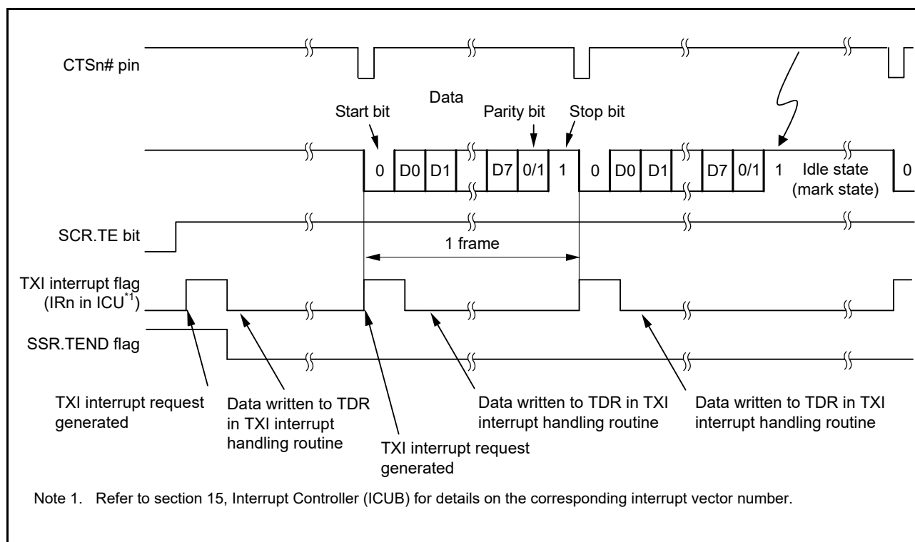
Figure 37.15 Example of Operation for Serial Transmission in Asynchronous Mode (2) (with 8-Bit Data, Parity, 1 Stop Bit, CTS Function Used, at the Beginning of Transmission)
