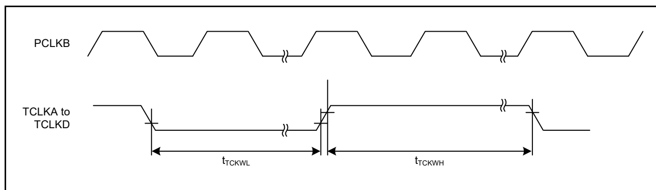
Figure 60.35 TPU Clock Input Timing
