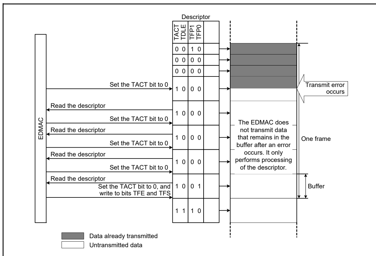
Figure 35.7 EDMAC Operation After a Transmit Error Occurs
