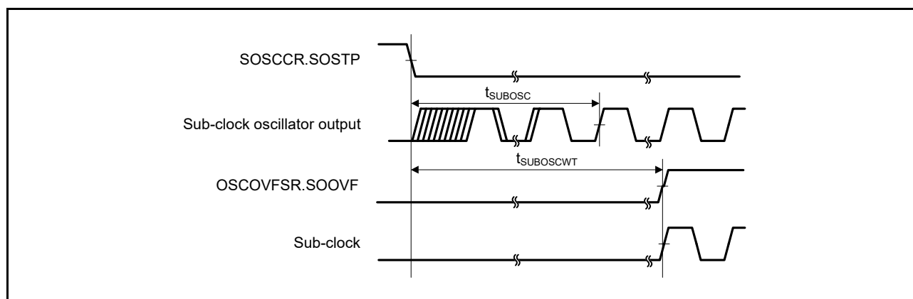
Figure 60.11 Sub-Clock Oscillation Start Timing
