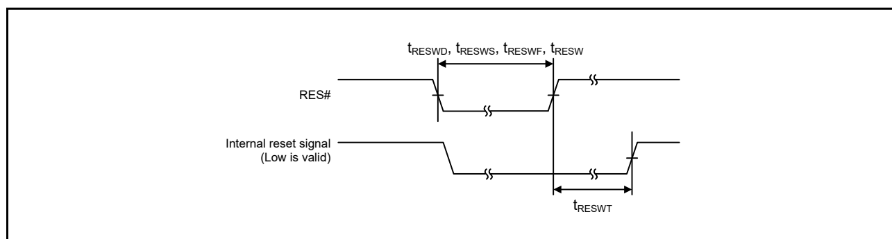
Figure 60.2 Reset Input Timing
