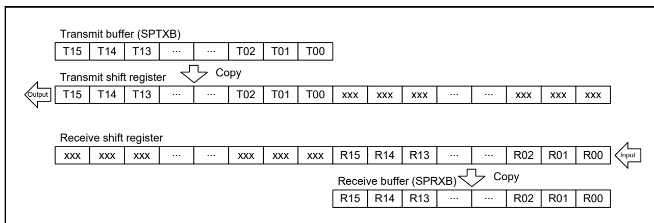
Figure 41.7 MSB First Transfer (16-Bit Data)
