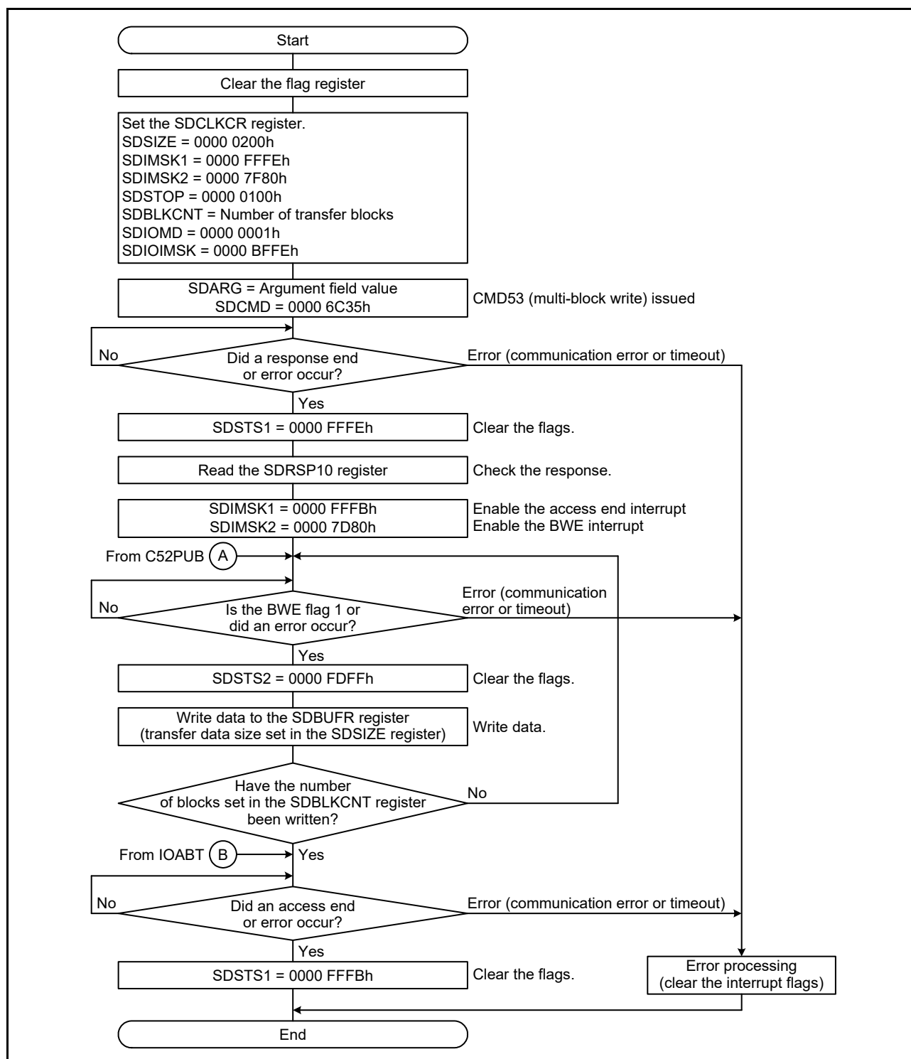
Figure 43.18 Issuing the IO_RW_EXTENDED Command (CMD53/Multi-Block Write)
