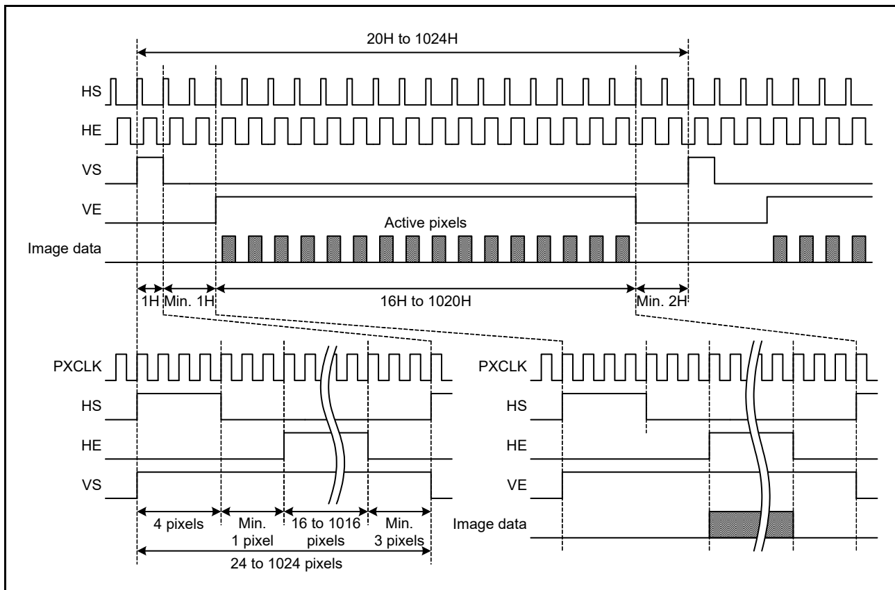
Figure 47.21 Image Data Carrier Signals in the GLCDC
