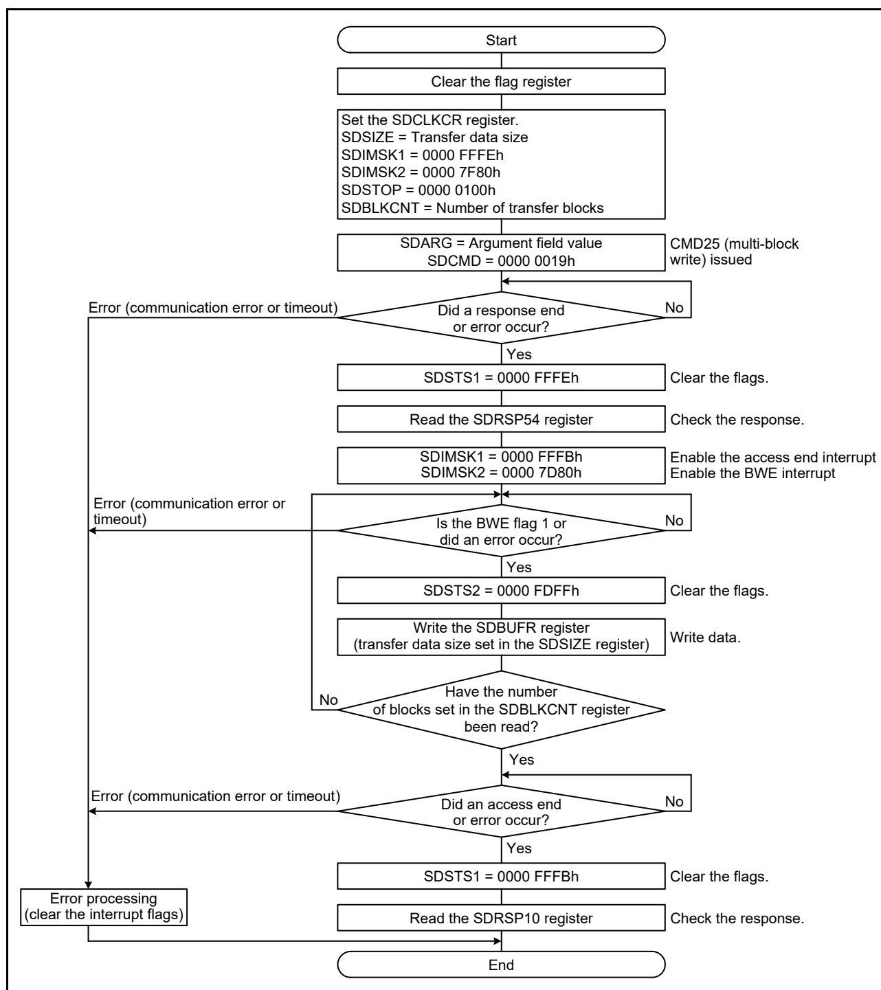
Figure 43.13 Issuing the Multi-Block Write Command
