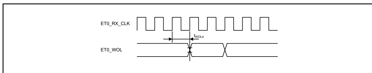
Figure 60.75 WOL Output Timing (MII)
