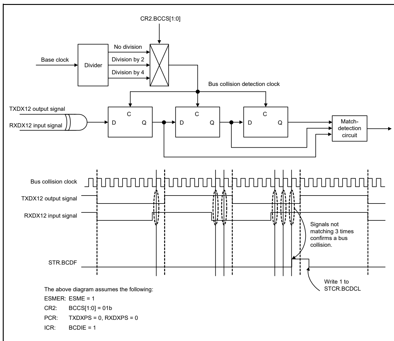
Figure 37.73 Example of Operations with Bus Collision Detection
