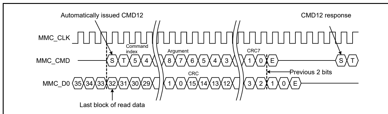
Figure 45.8 Timing for Automatically Issuing CMD12 During a Multi-Block Read Operation (1-Bit Data Bus Width)
