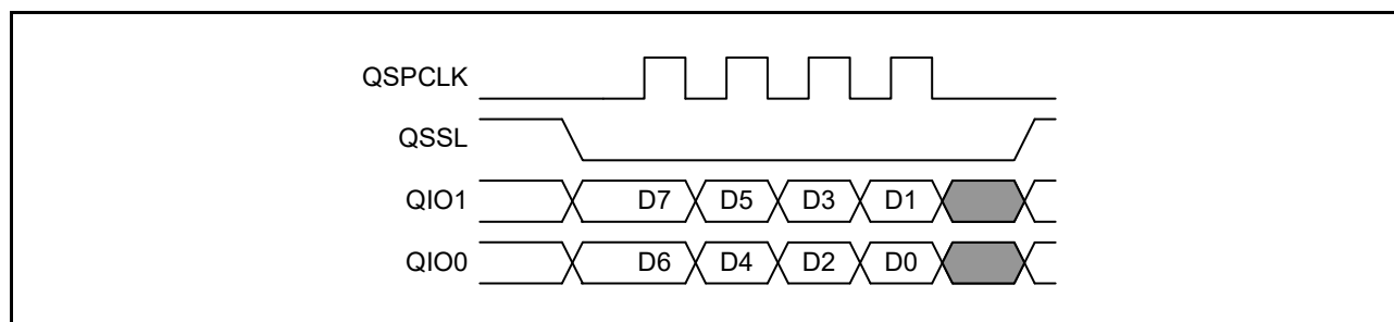
Figure 41.4 Transfer Format in Dual-SPI Format
