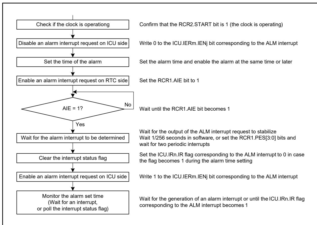
Figure 31.7 Using Alarm Function
