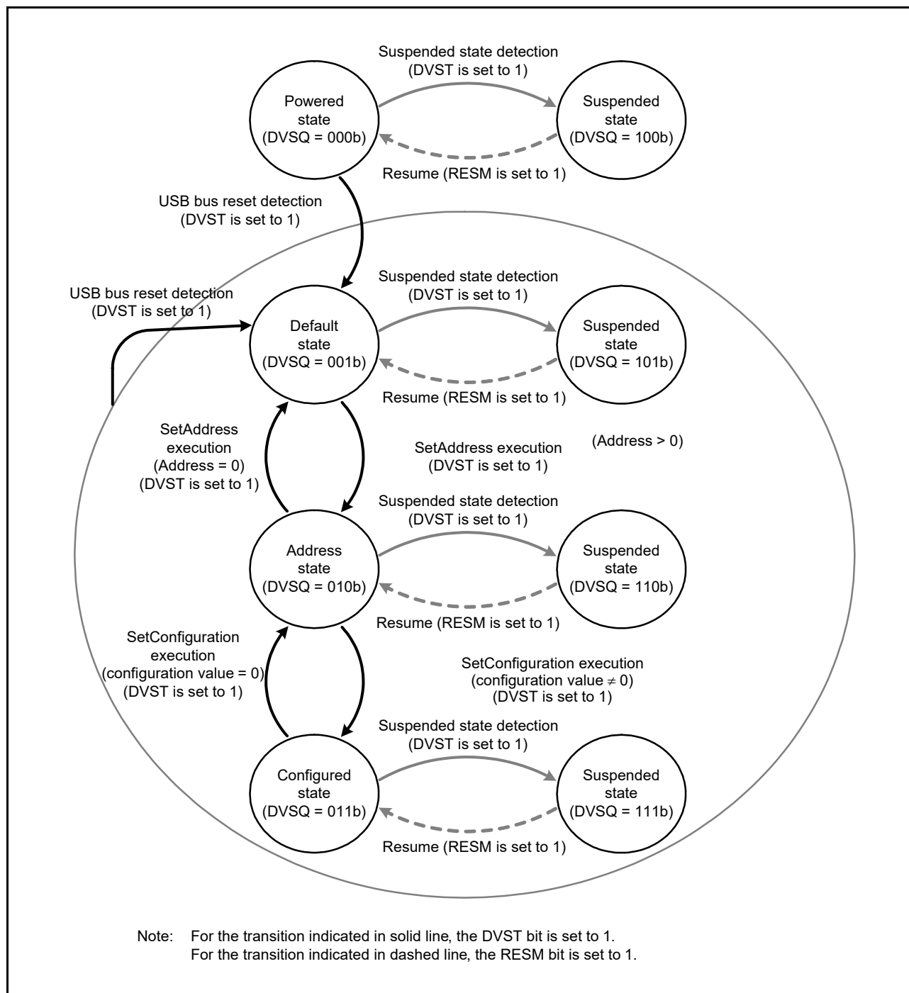
Figure 36.14 Device State Transitions
