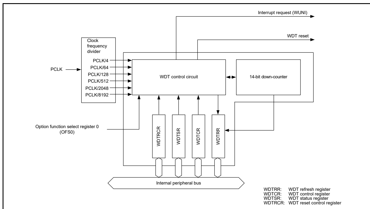
Figure 32.1 WDT Block Diagram
