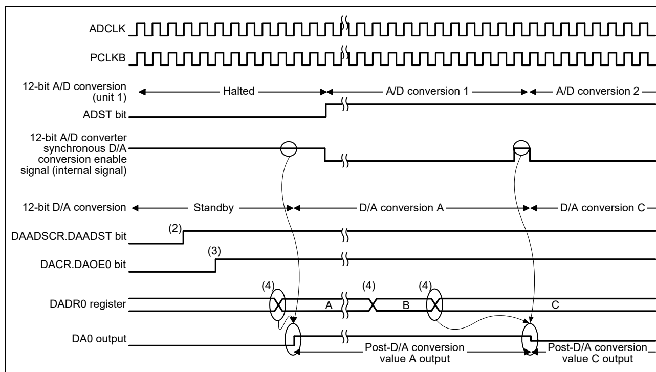
Figure 54.3 Example of Conversion When the 12-Bit D/A Converter is Synchronized with the 12-Bit A/D Converter (Unit 1)
