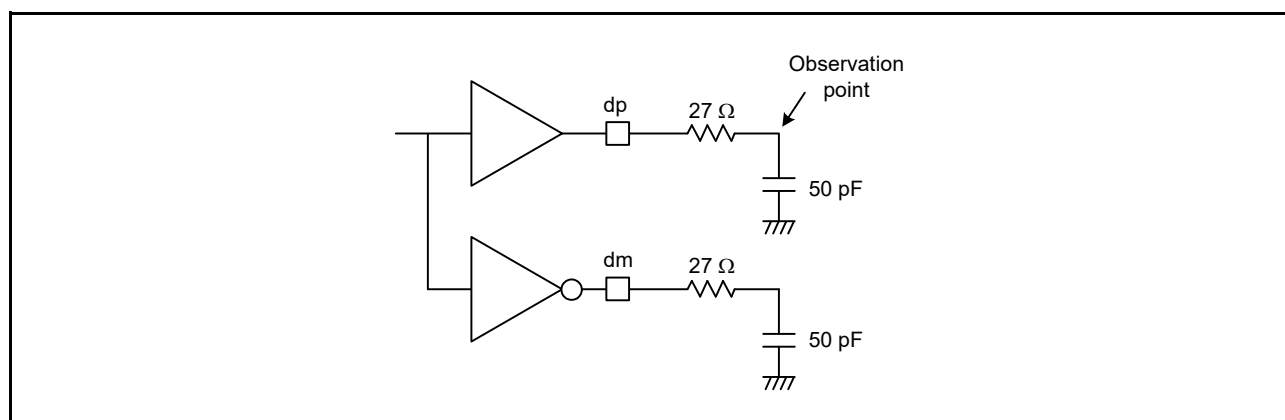
Figure 60.89 Test Circuit (Full-Speed)
