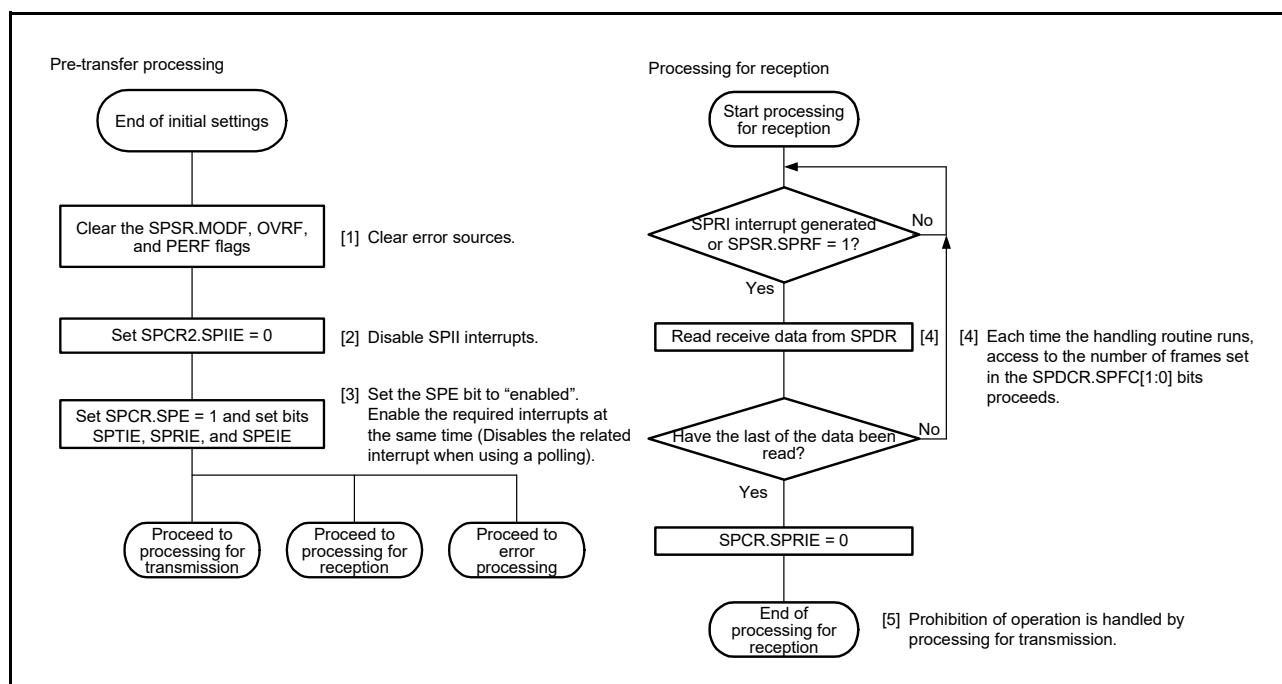
Figure 40.39 Flowchart in Master Mode (Reception)
