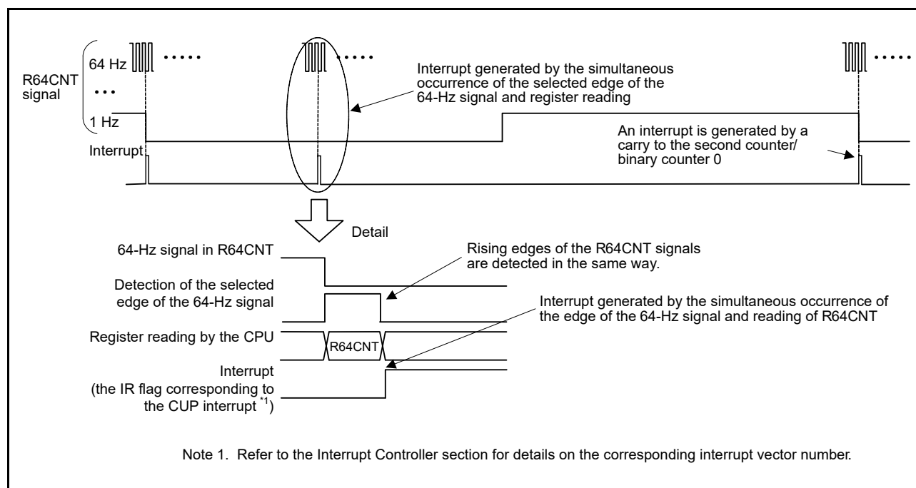
Figure 31.12 Carry Interrupt (CUP) Timing Chart
