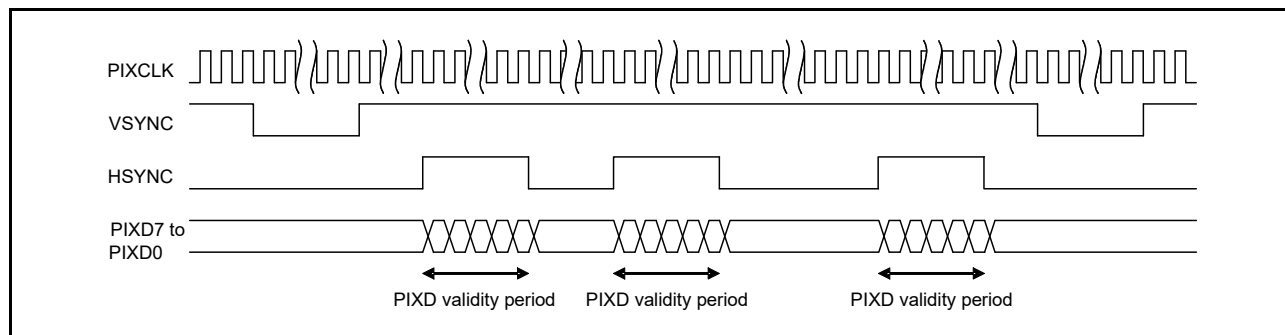
Figure 46.4 PDC Transfer Format (for VPS = 0, HPS = 0)
