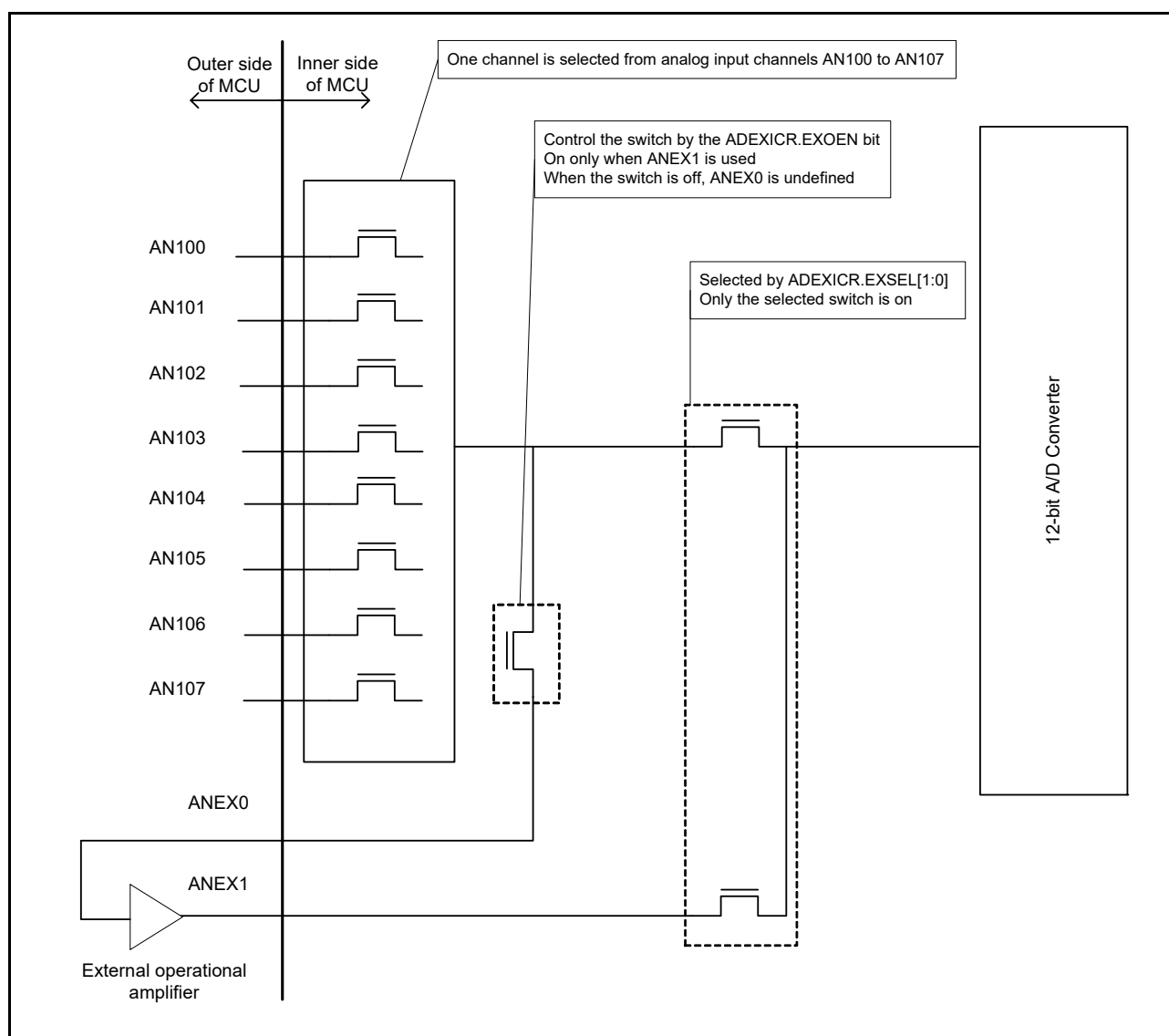
Figure 53.35 Example of Configuration of Extended Analog Input When ANEX1 is Used
