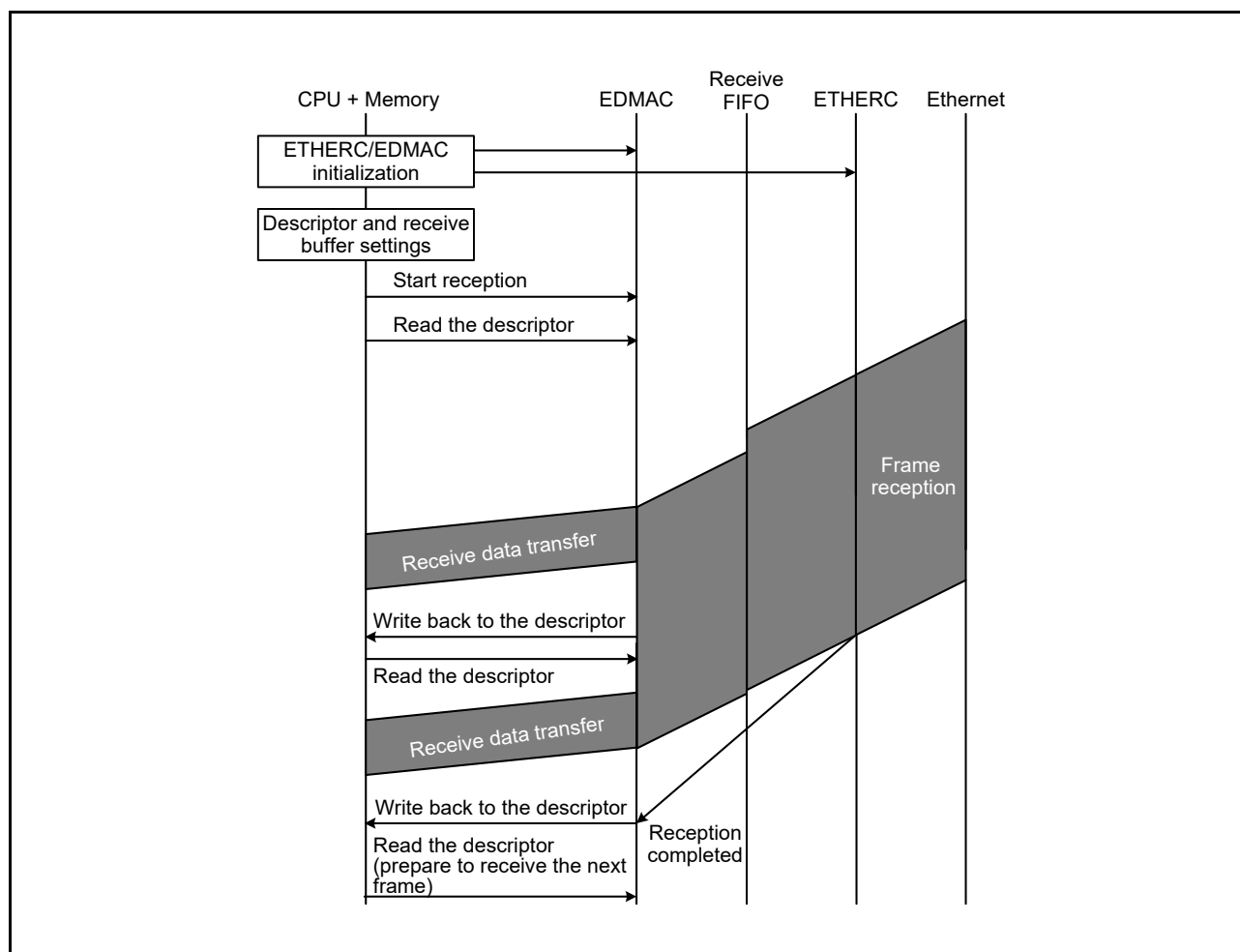
Figure 35.6 Example of Reception Flow
