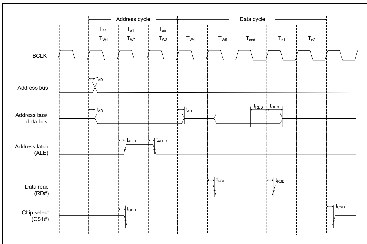
Figure 60.16 Address/Data Multiplexed Bus Read Access Timing
