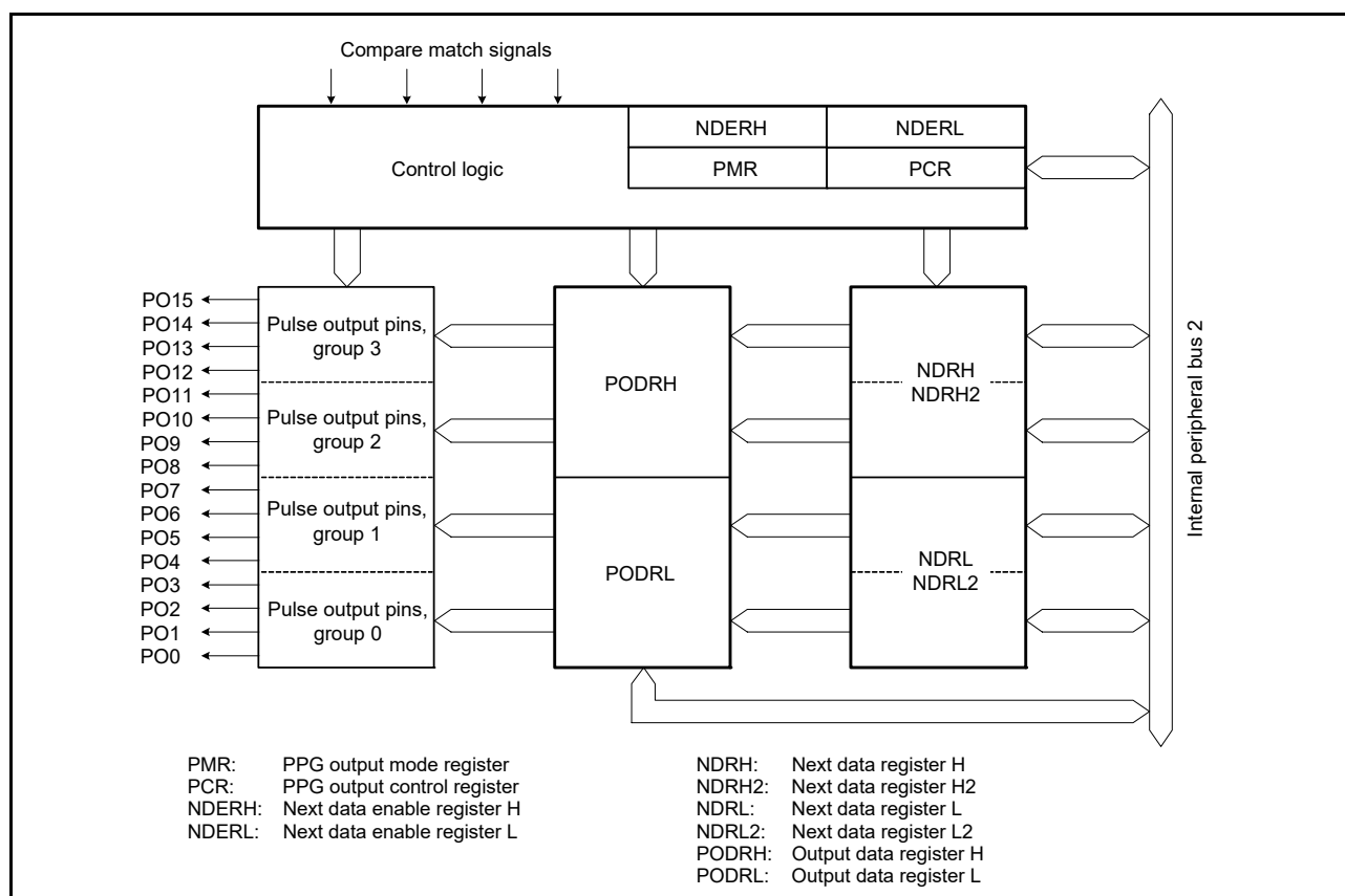
Figure 27.1 Block Diagram of PPG0
