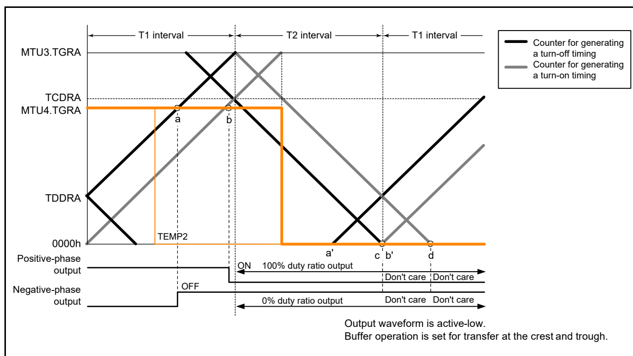
Figure 24.62 Example of 0% and 100% Waveform Output in Complementary PWM Mode (MTU3 and MTU4) (4)
