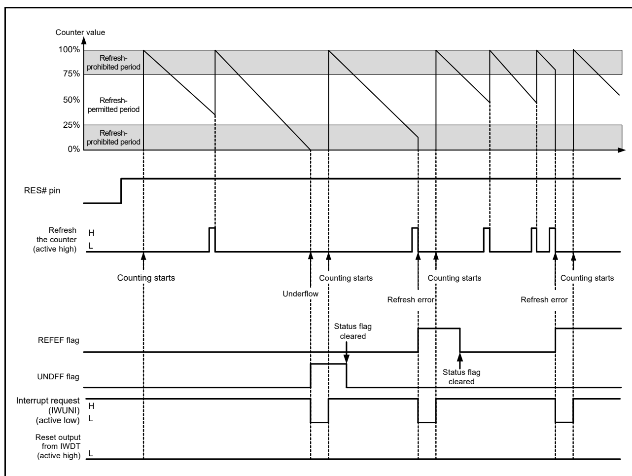
Figure 33.4 Operation Example in Auto-Start Mode
