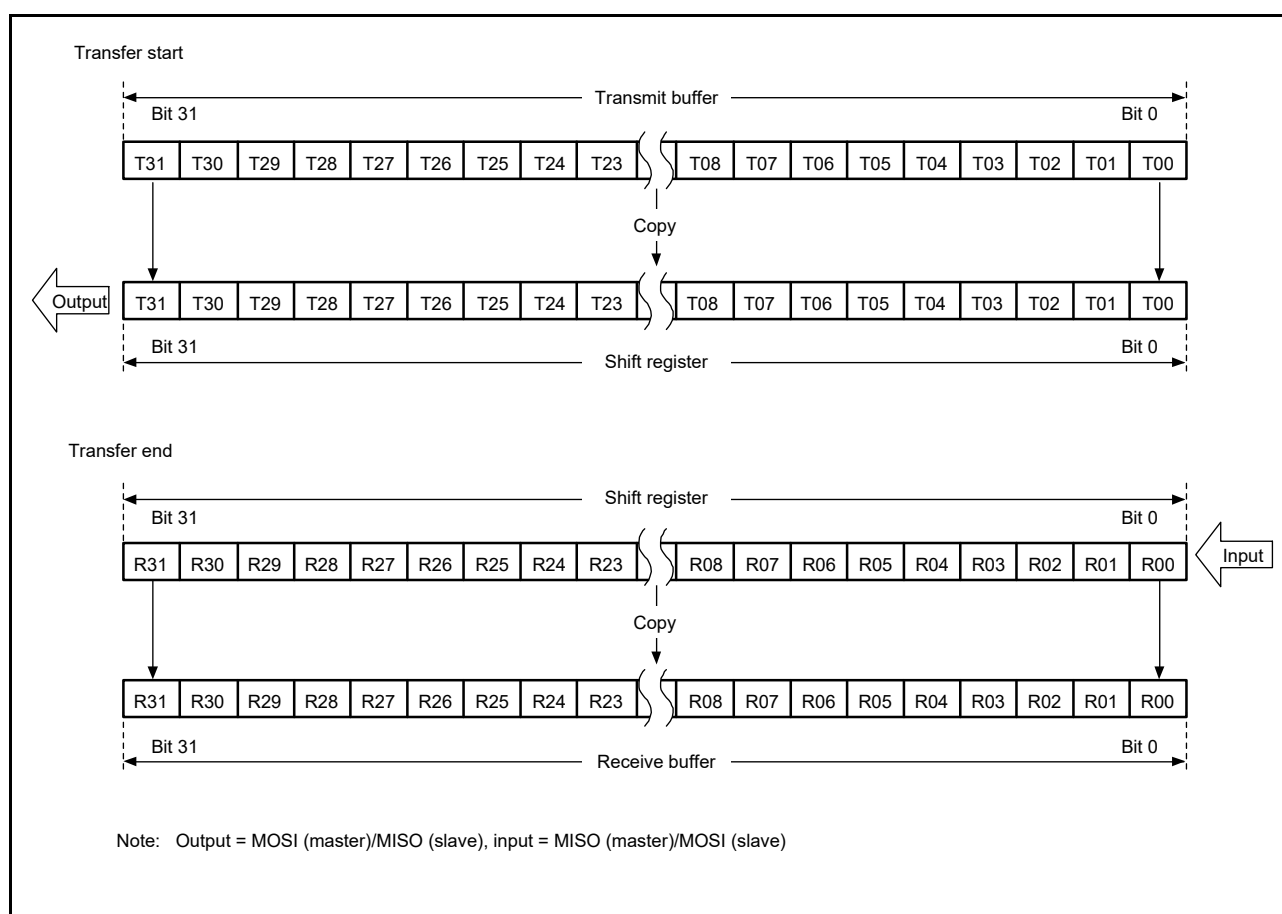
Figure 40.14 MSB First Transfer (32-Bit Data, Parity Disabled)
