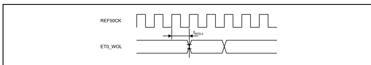
Figure 60.70 WOL Output Timing (RMII)
