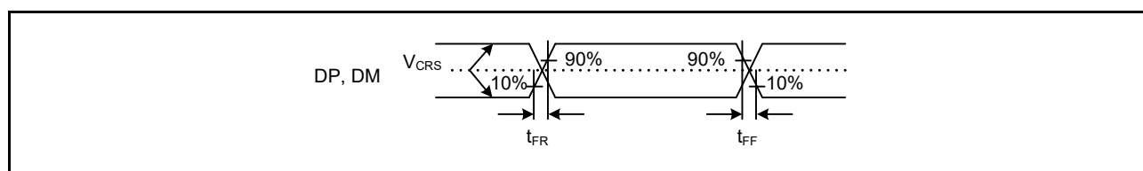
Figure 60.88 DP and DM Output Timing (Full-Speed)
