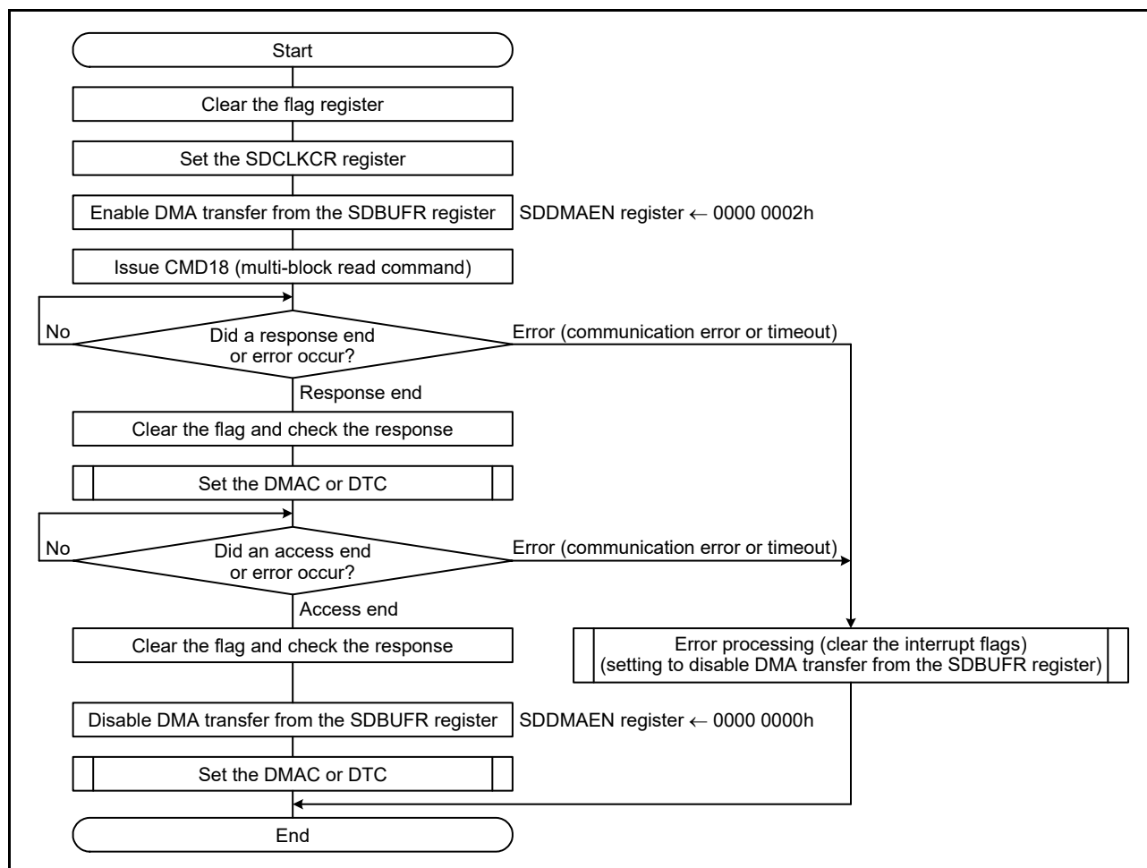
Figure 43.21 DMA Transfer After CMD18 is Issued
