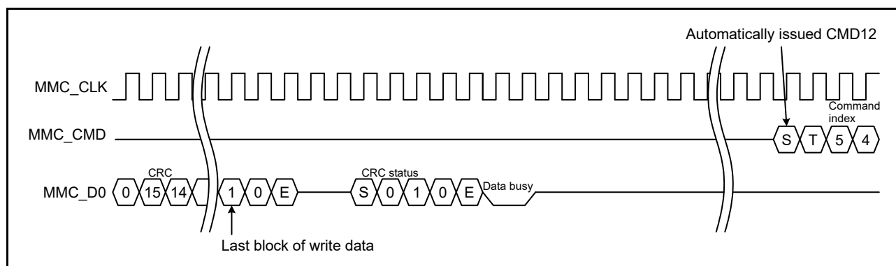
Figure 45.9 Timing for Automatically Issuing CMD12 During a Multi-Block Write Operation (1-Bit Data Bus Width)
