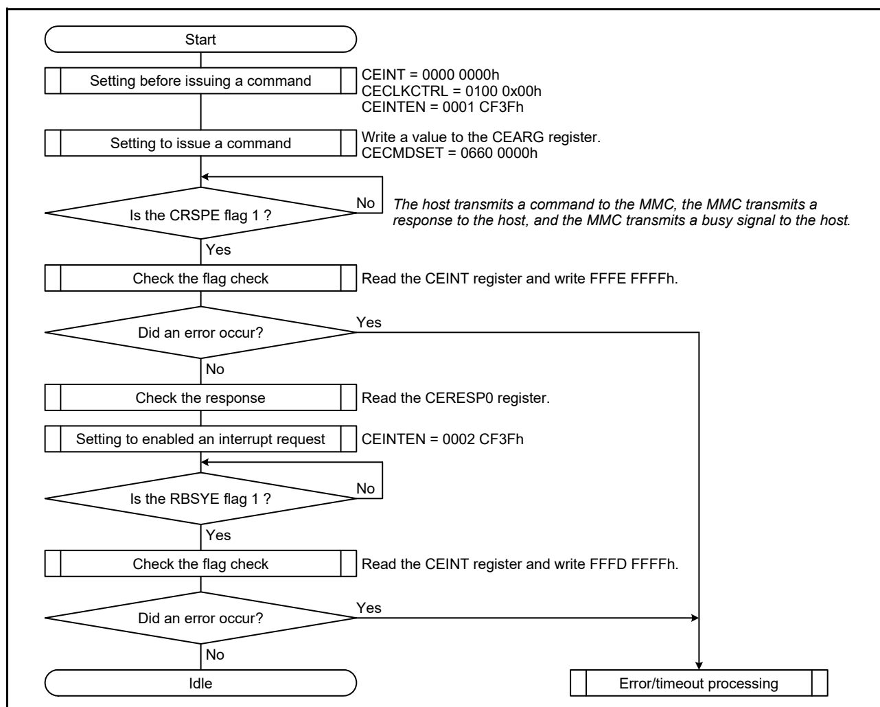
Figure 45.13 Issuing a Command Where Data is Not Transferred and the Busy Signal is Used (CMD6)
