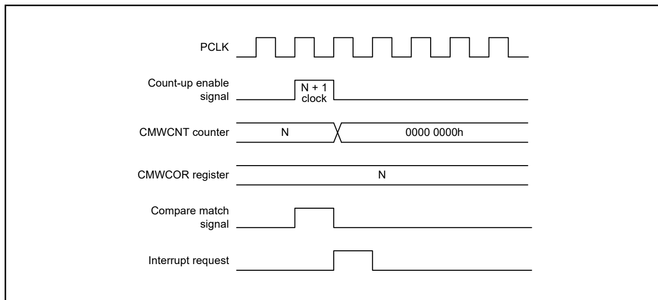
Figure 30.13 Timing of Compare Match Interrupt Generation
