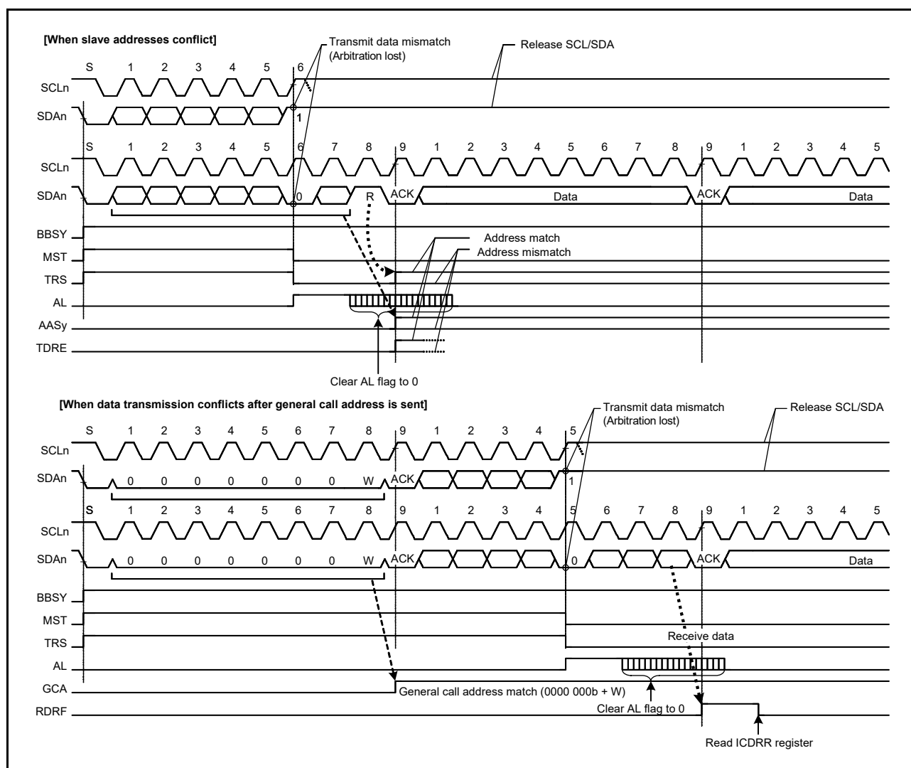
Figure 38.32 Examples of Master Arbitration-Lost Detection (MALE = 1)
