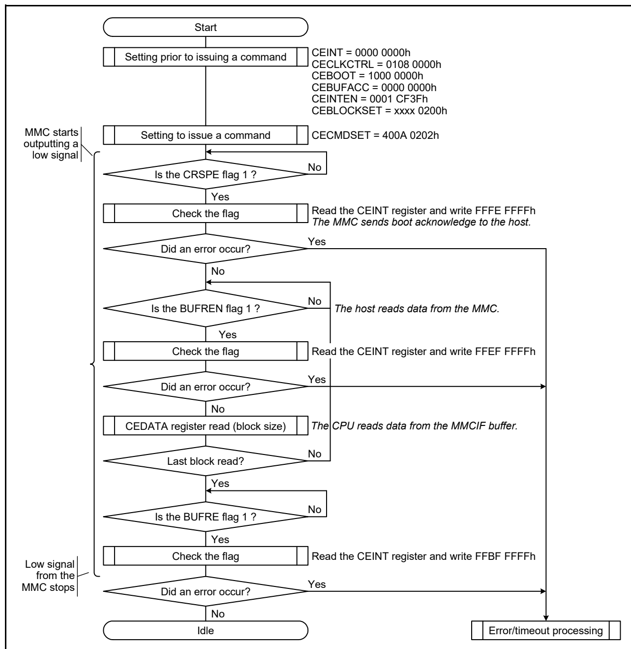
Figure 45.21 Boot Operation With Boot Acknowledge
