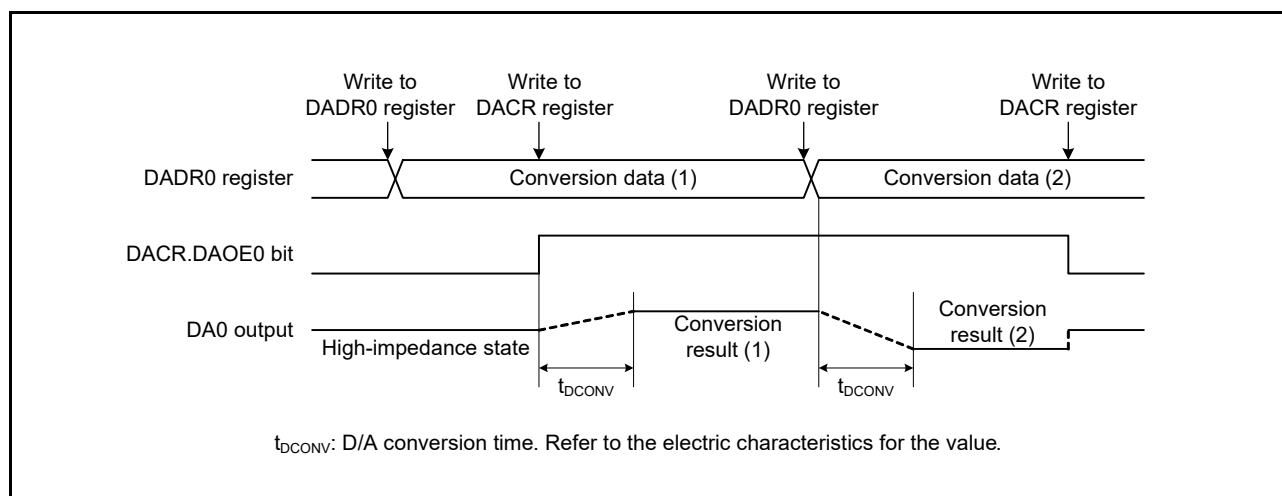
Figure 54.2 Example of 12-Bit D/A Converter Operation
