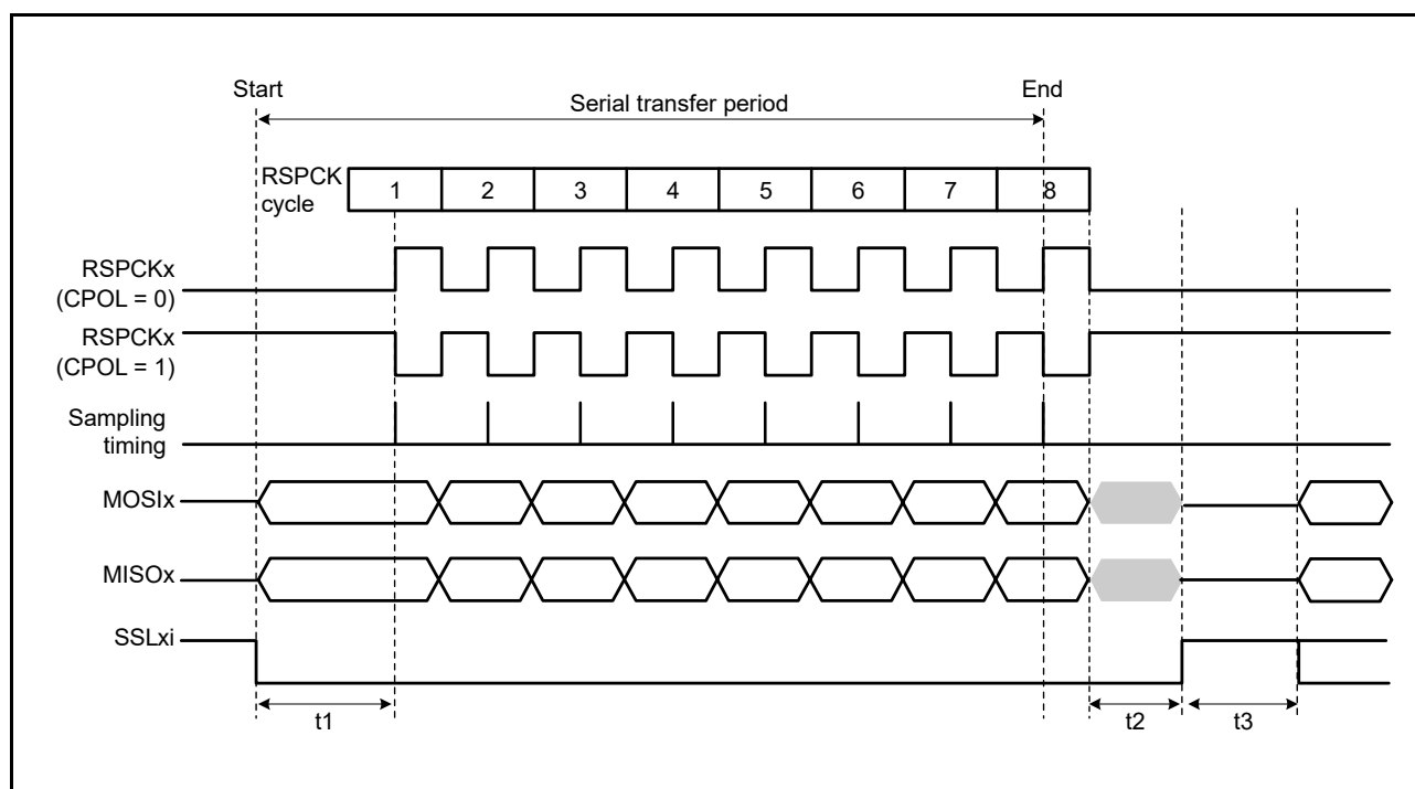
Figure 40.24 RSPI Transfer Format (CPHA = 0)
