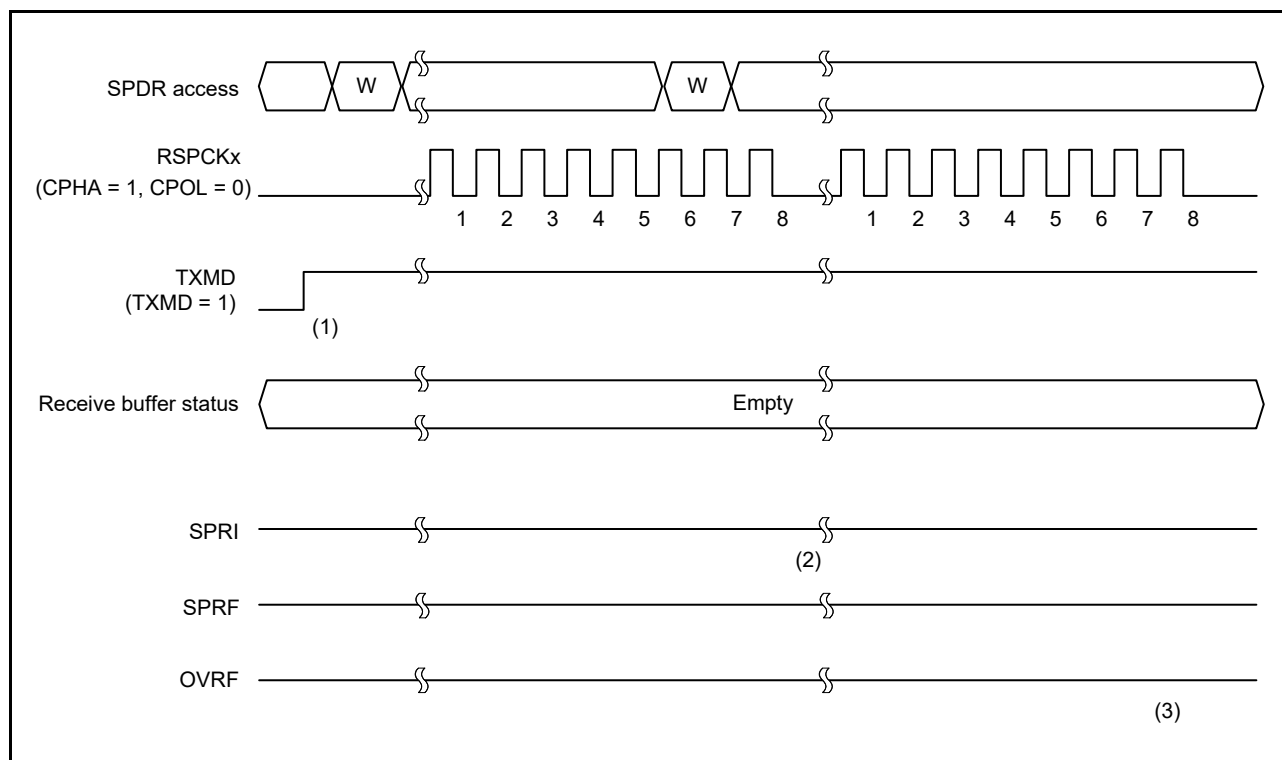
Figure 40.27 Operation Example of SPCR.TXMD = 1
