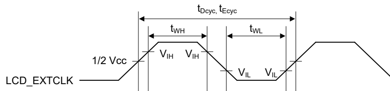
Figure 60.79 LCD_EXTCLK Clock Input Timing
