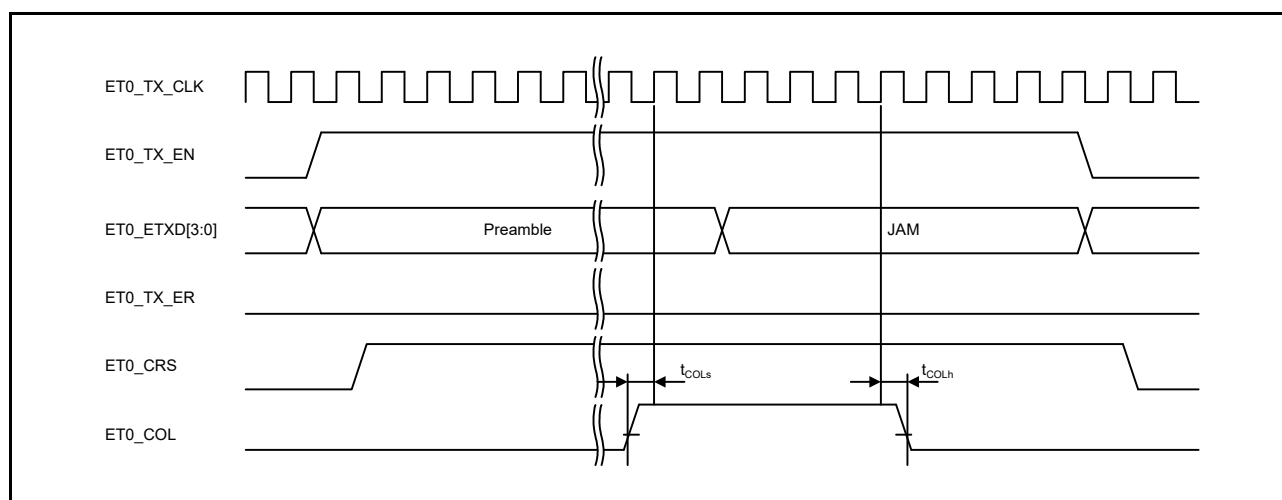
Figure 60.72 MII Transmission Timing (Conflict Occurrence)
