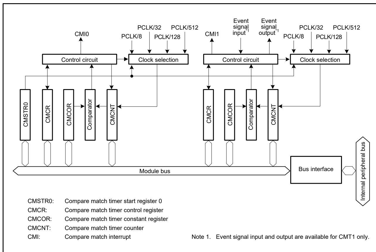
Figure 29.1 CMT (Unit 0) Block Diagram
