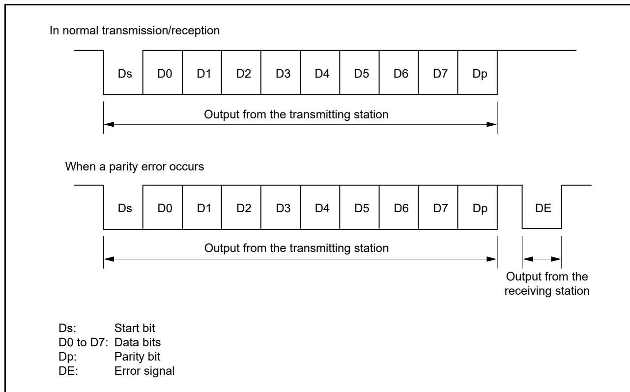
Figure 37.38 Data Formats in Smart Card Interface Mode
