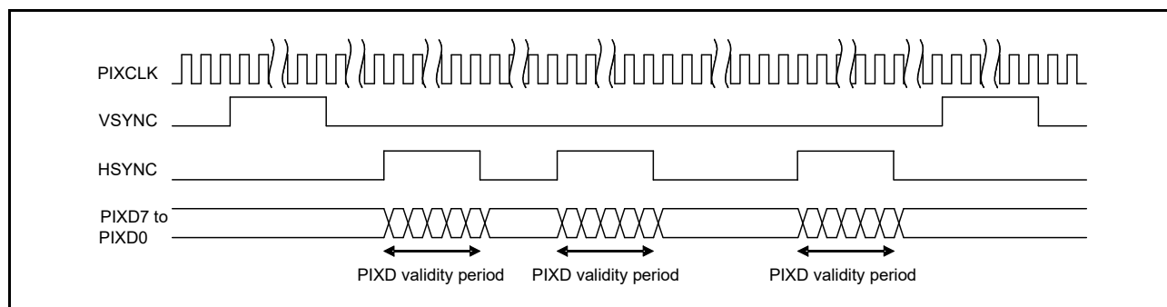
Figure 46.5 PDC Transfer Format (for VPS = 1, HPS = 0)
