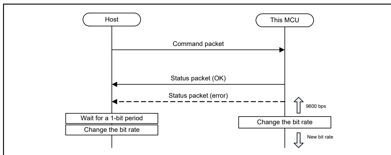
Figure 59.19 Bit-Rate Setting Command Transfer Sequence
