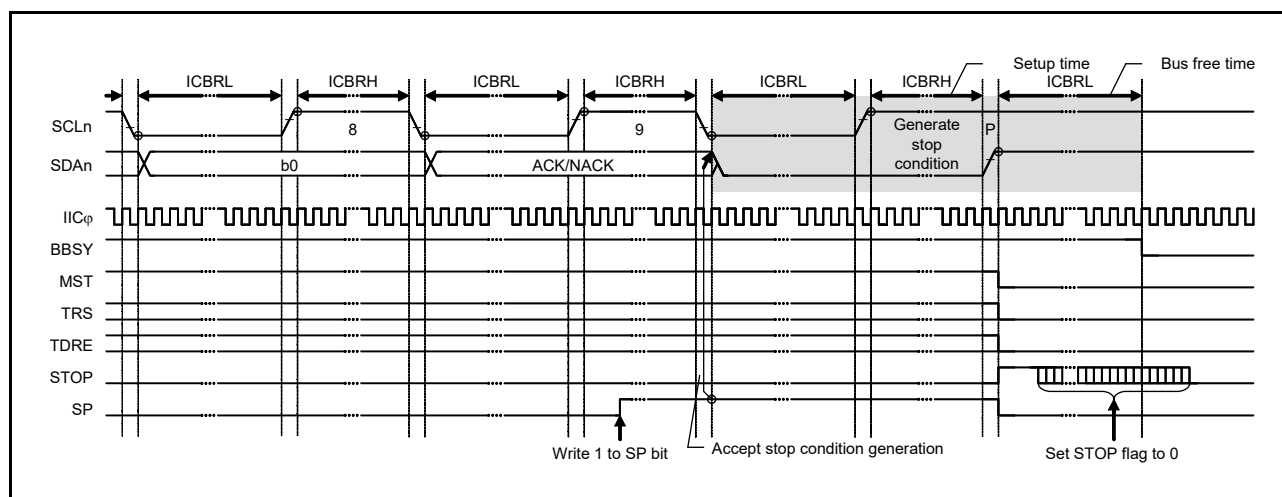
Figure 38.37 Stop Condition Generation Timing (SP Bit)
