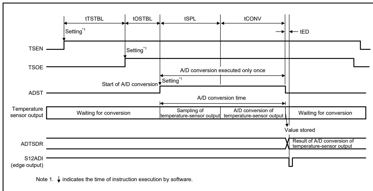
Figure 55.4 Timing from the Start of Temperature-Sensor Operation until Completion of A/D Conversion
