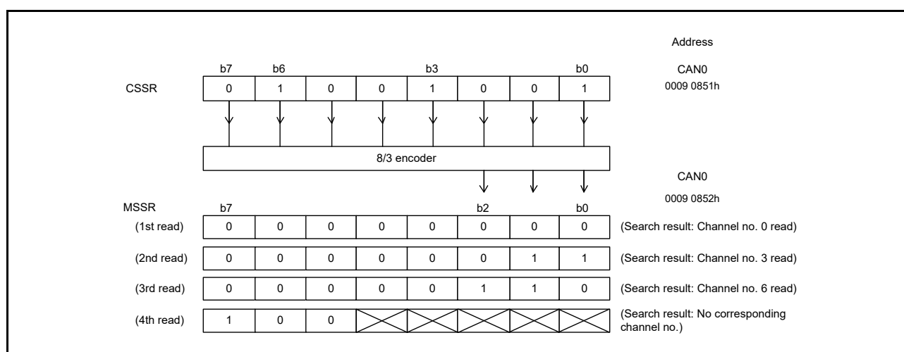
Figure 39.4 Write and Read of CSSR and MSSR
