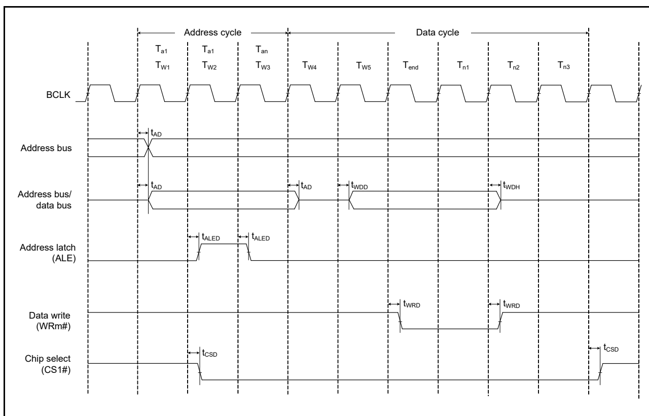
Figure 60.17 Address/Data Multiplexed Bus Write Access Timing
