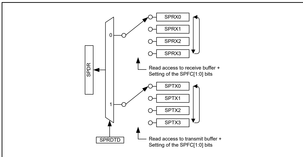
Figure 40.4 Configuration of the SPDR Register (Reading)
