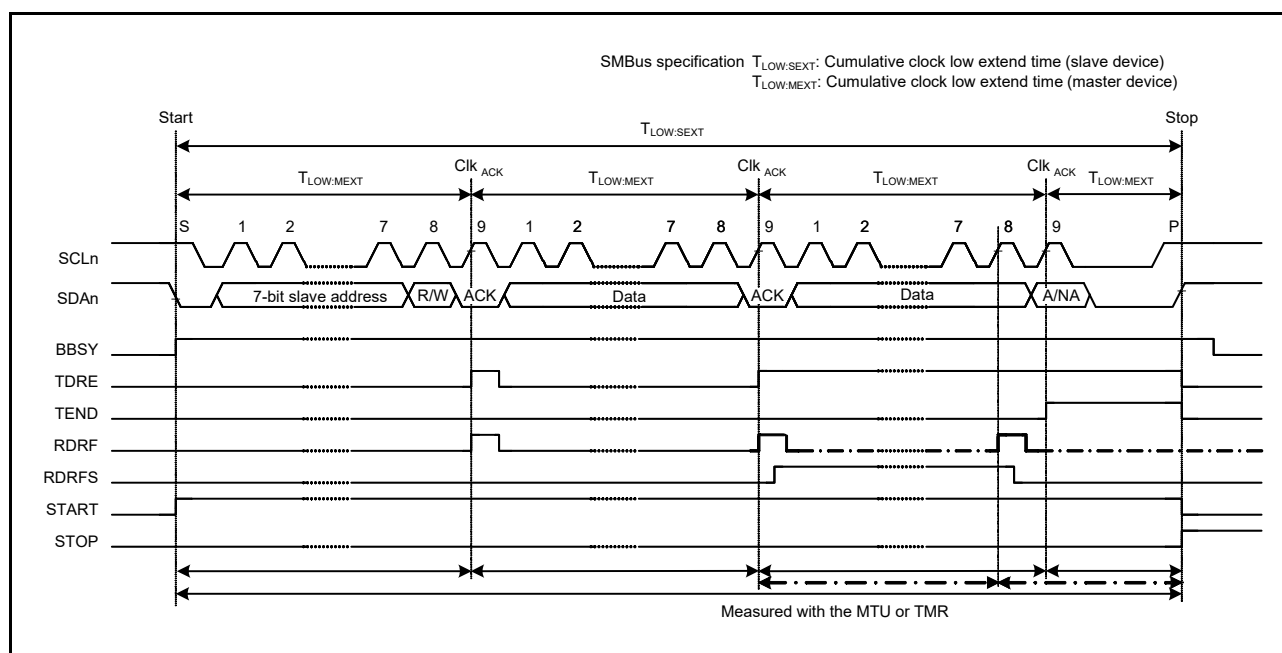
Figure 38.40 SMBus Timeout Measurement
