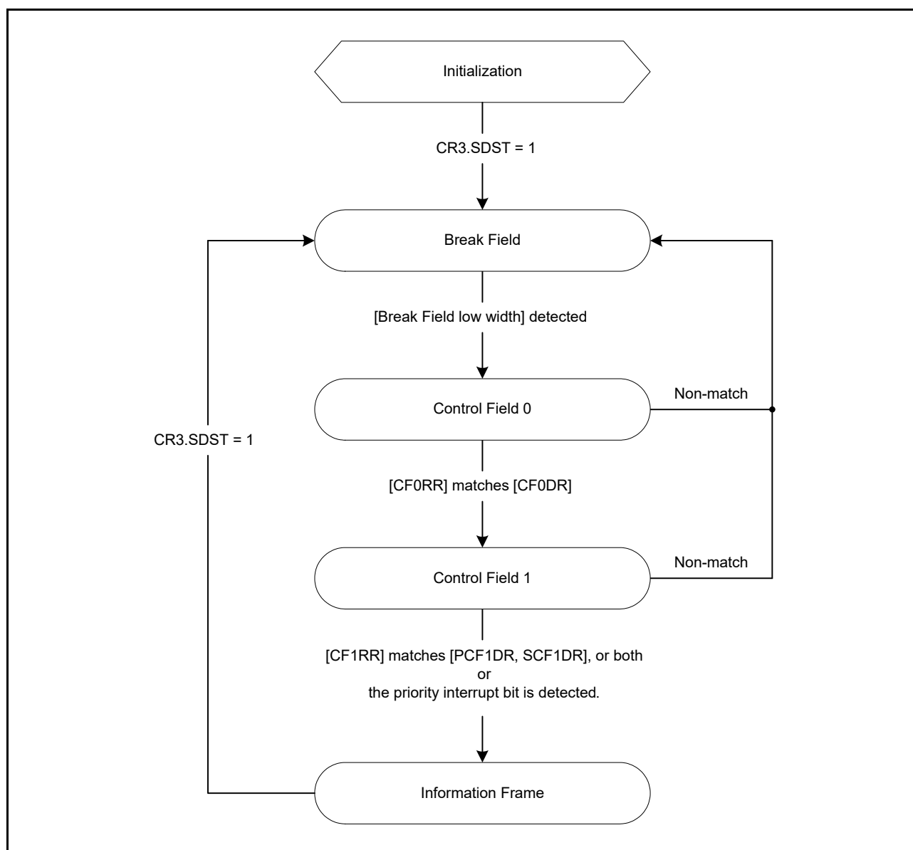
Figure 37.71 State Transitions When Receiving a Start Frame
