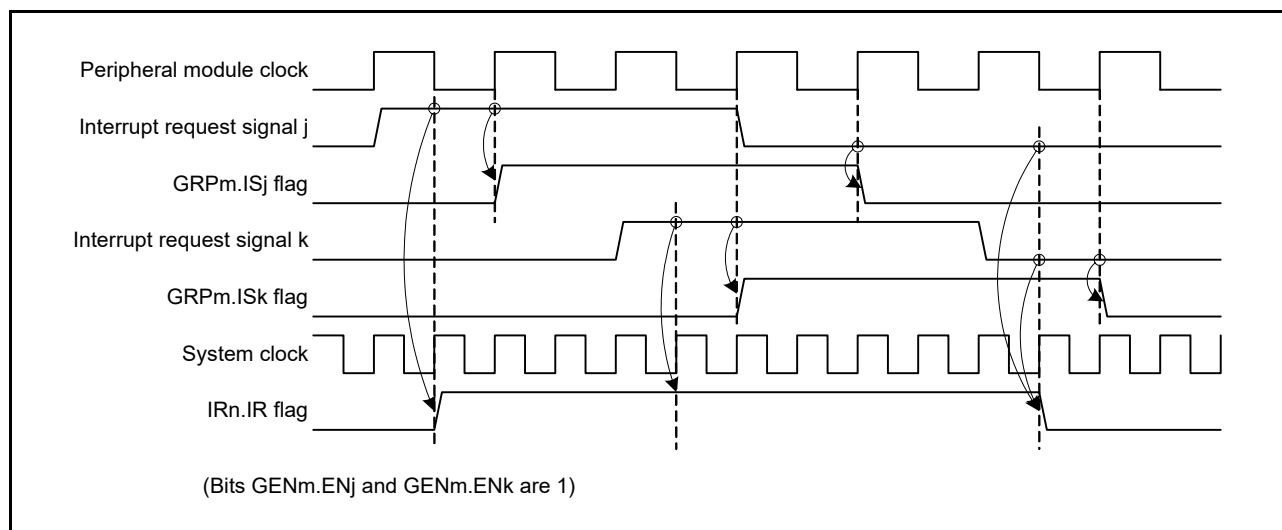
Figure 15.17 Operation Example When Multiple Interrupt Requests are Generated in the Same Group ( m = \text{BL0, BL1, BL2, AL0, AL1} )
