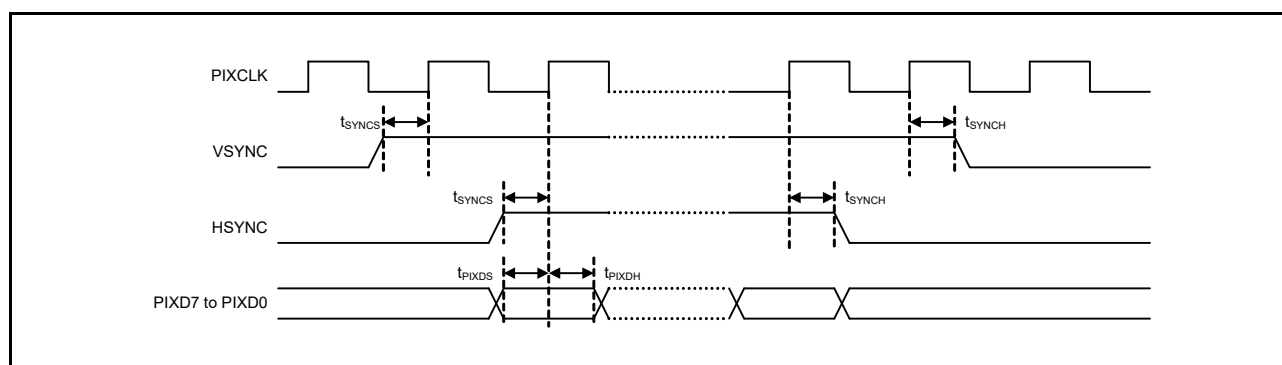
Figure 60.78 PDC AC Timing
