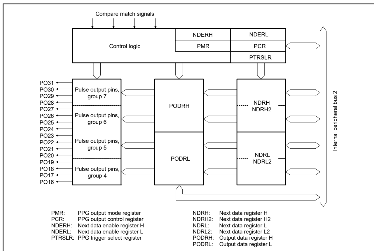
Figure 27.2 Block Diagram of PPG1
