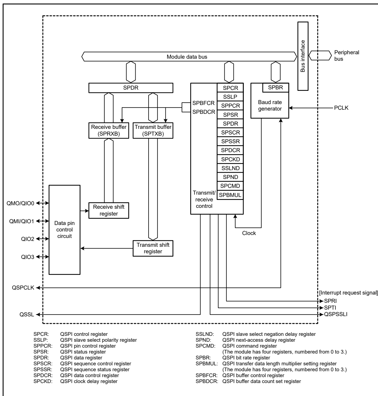
Figure 41.1 QSPI Block Diagram
