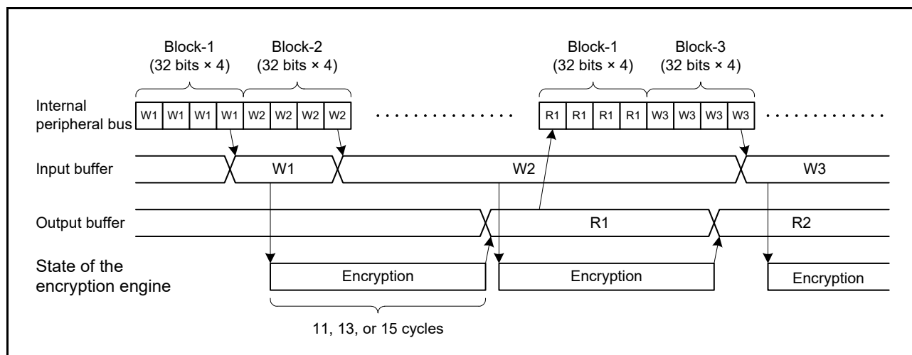
Figure 52.6 Encryption and Decryption Timing Diagram
