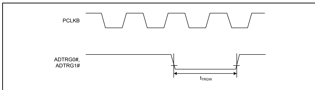
Figure 60.45 A/D Converter Trigger Input Timing
