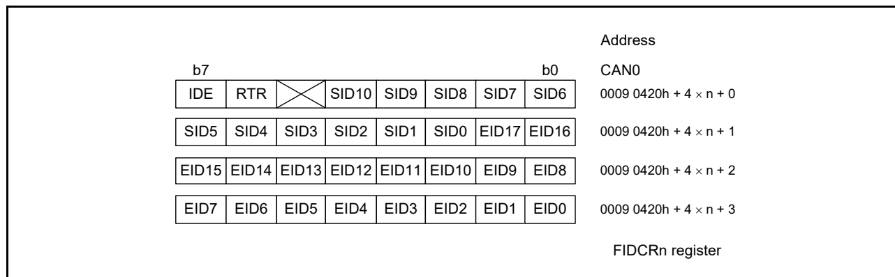
Figure 39.15 Structure of FIDCRn (n = 0, 1)
