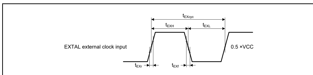
Figure 60.4 EXTAL External Clock Input Timing
