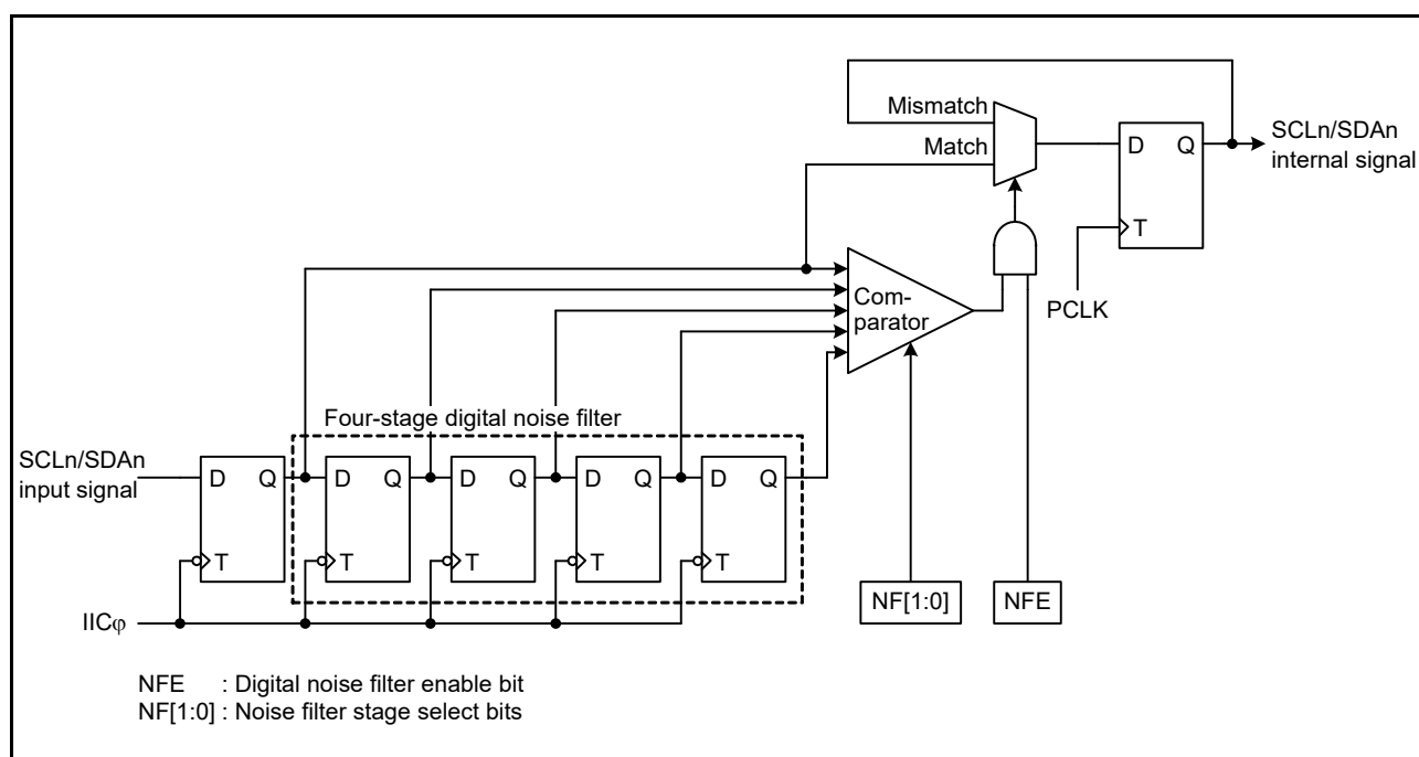
Figure 38.22 Block Diagram of the Digital Noise Filter
