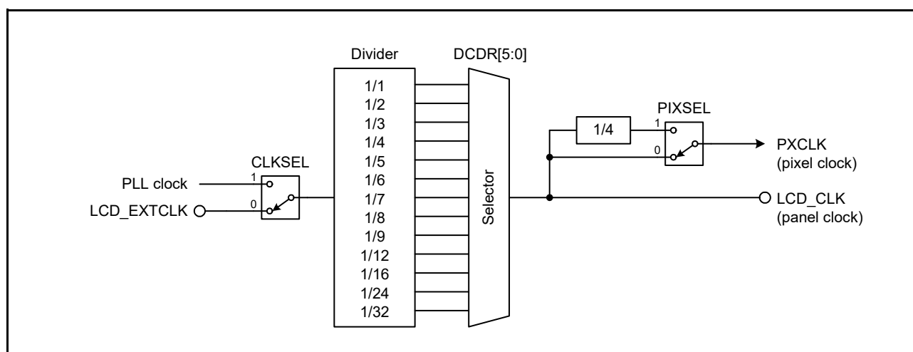
Figure 47.19 Structure of Clock Generator
