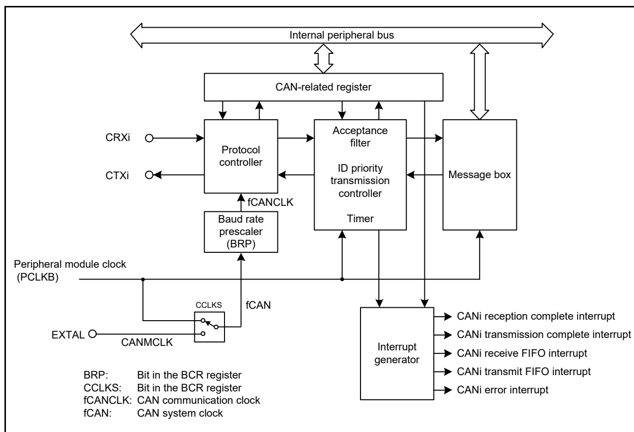
Figure 39.1 Block Diagram of CAN Module (i = 0, 1)
