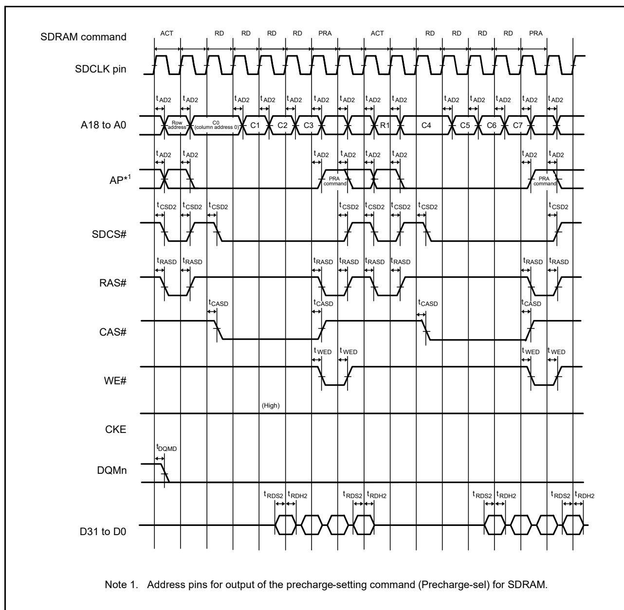
Figure 60.27 SDRAM Space Multiple Read Line Stride Bus Timing
