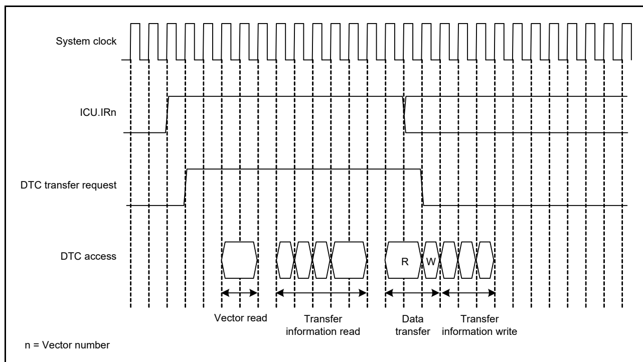
Figure 20.13 Example (4) of DTC Operation Timing (Full-Address Mode, Normal Transfer Mode, Repeat Transfer Mode)
