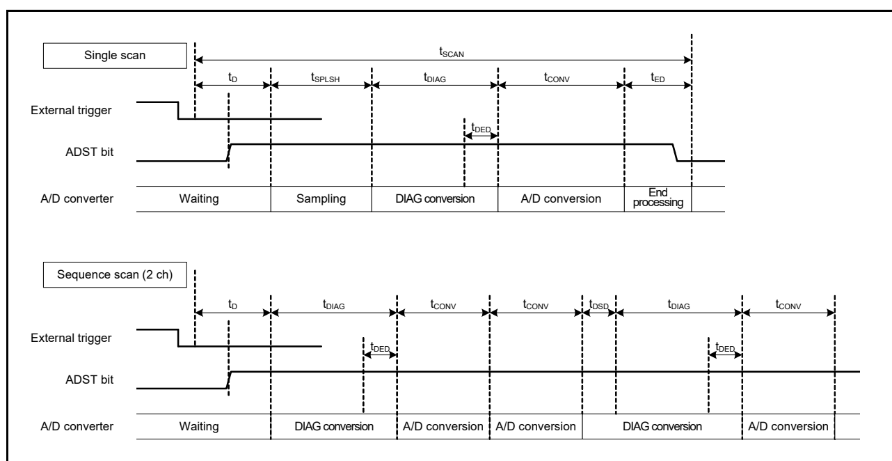
Figure 53.39 Scan Conversion Timing (Activated by Asynchronous Trigger)
