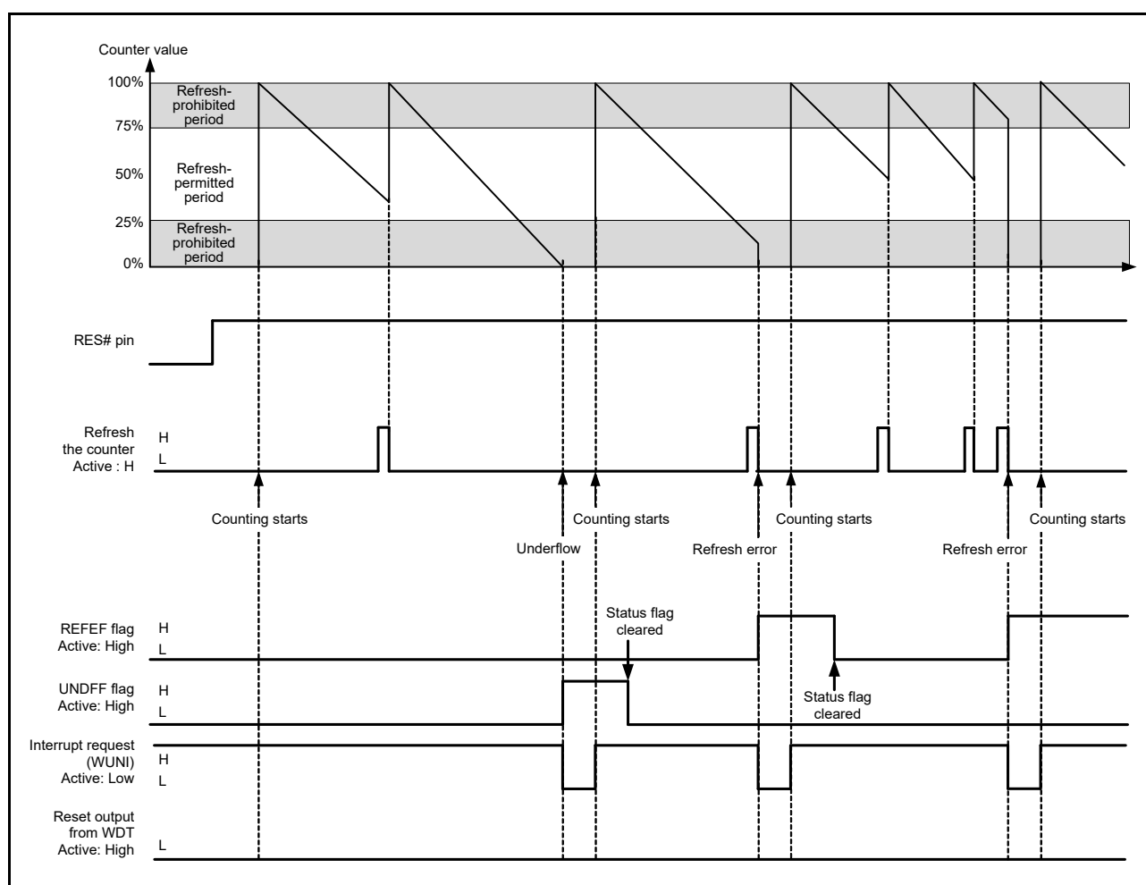
Figure 32.4 Operation Example in Auto-Start Mode
