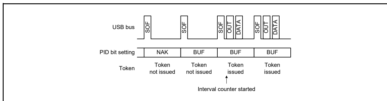
Figure 36.16 Token Issuance When IITV[2:0] = 000b
