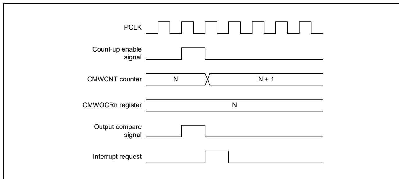
Figure 30.14 Timing of Output Compare Interrupt Generation ( n = 0, 1 )
