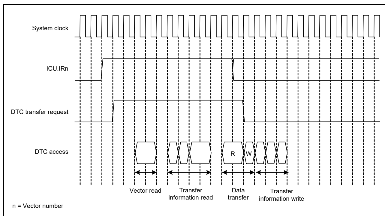
Figure 20.10 Example (1) of DTC Operation Timing (Short-Address Mode, Normal Transfer Mode, Repeat Transfer Mode)
