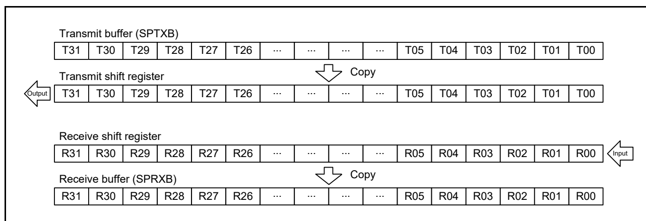
Figure 41.6 MSB First Transfer (32-Bit Data)
