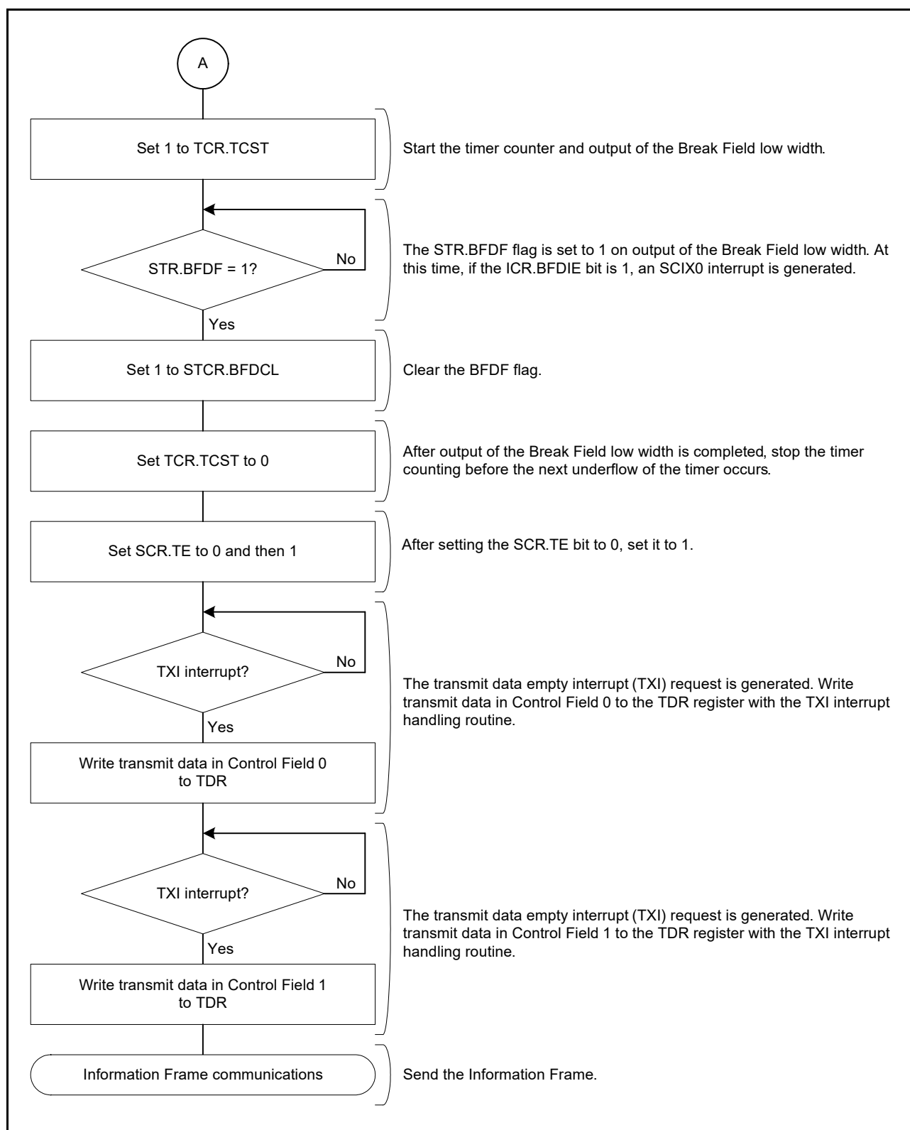
Figure 37.67 Example of Start Frame Transmission (2/2)
