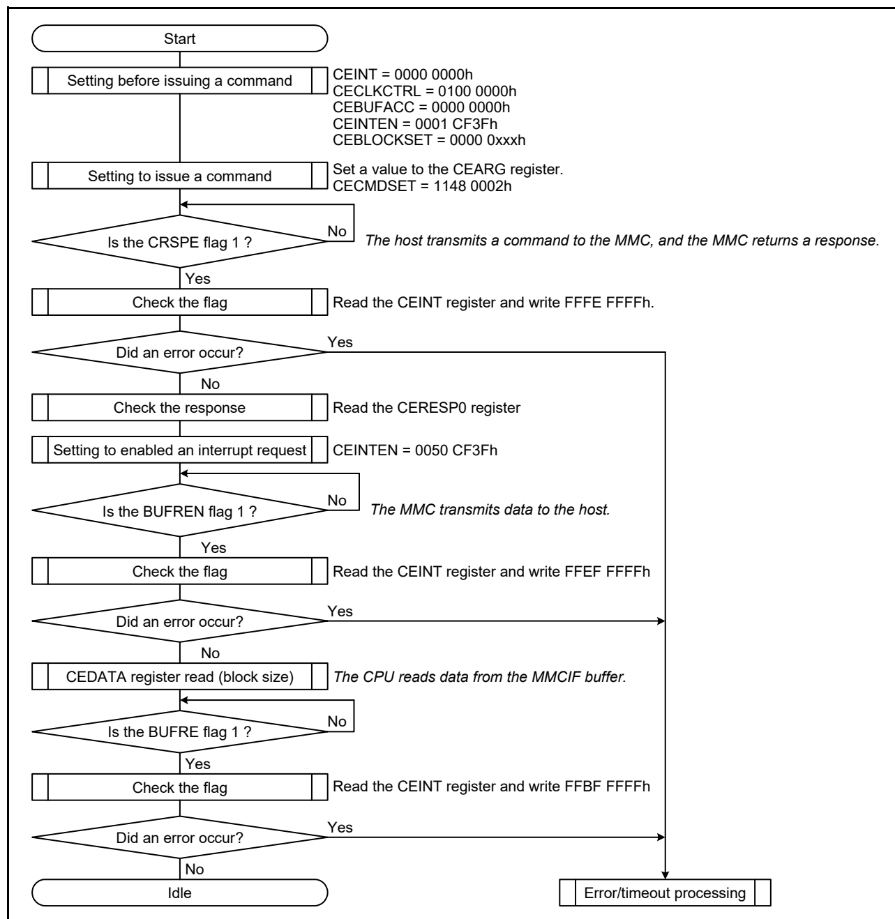
Figure 45.15 Issuing a Single Block Read Command (CMD17)
