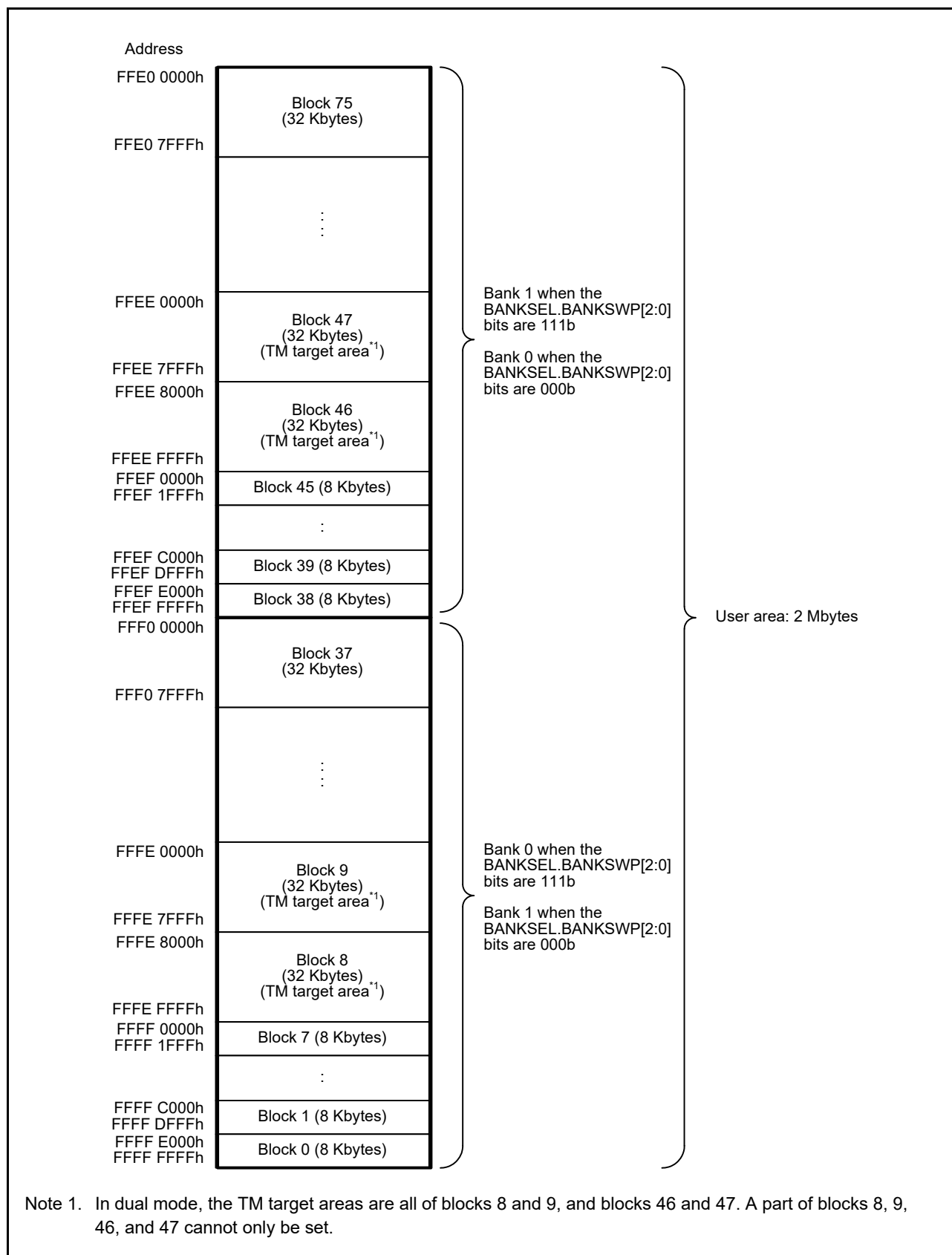
Figure 59.4 Map of the Code Flash Memory in Dual Mode (Products with 2 Mbytes of code flash memory)
