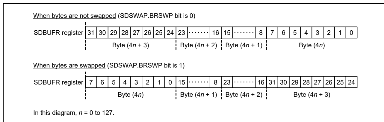
Figure 43.5 Data Alignment When Reading the SDBUFR Register
