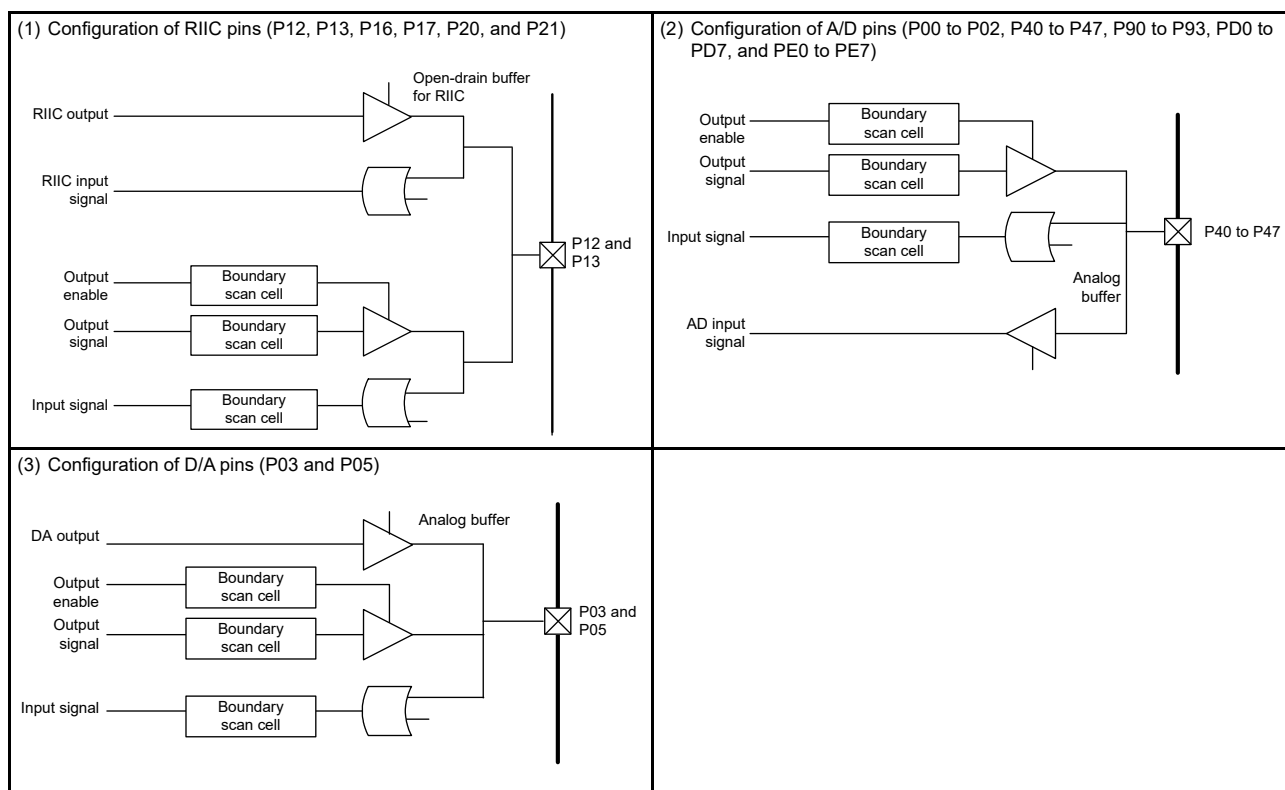
Figure 49.4 Pin Configuration
