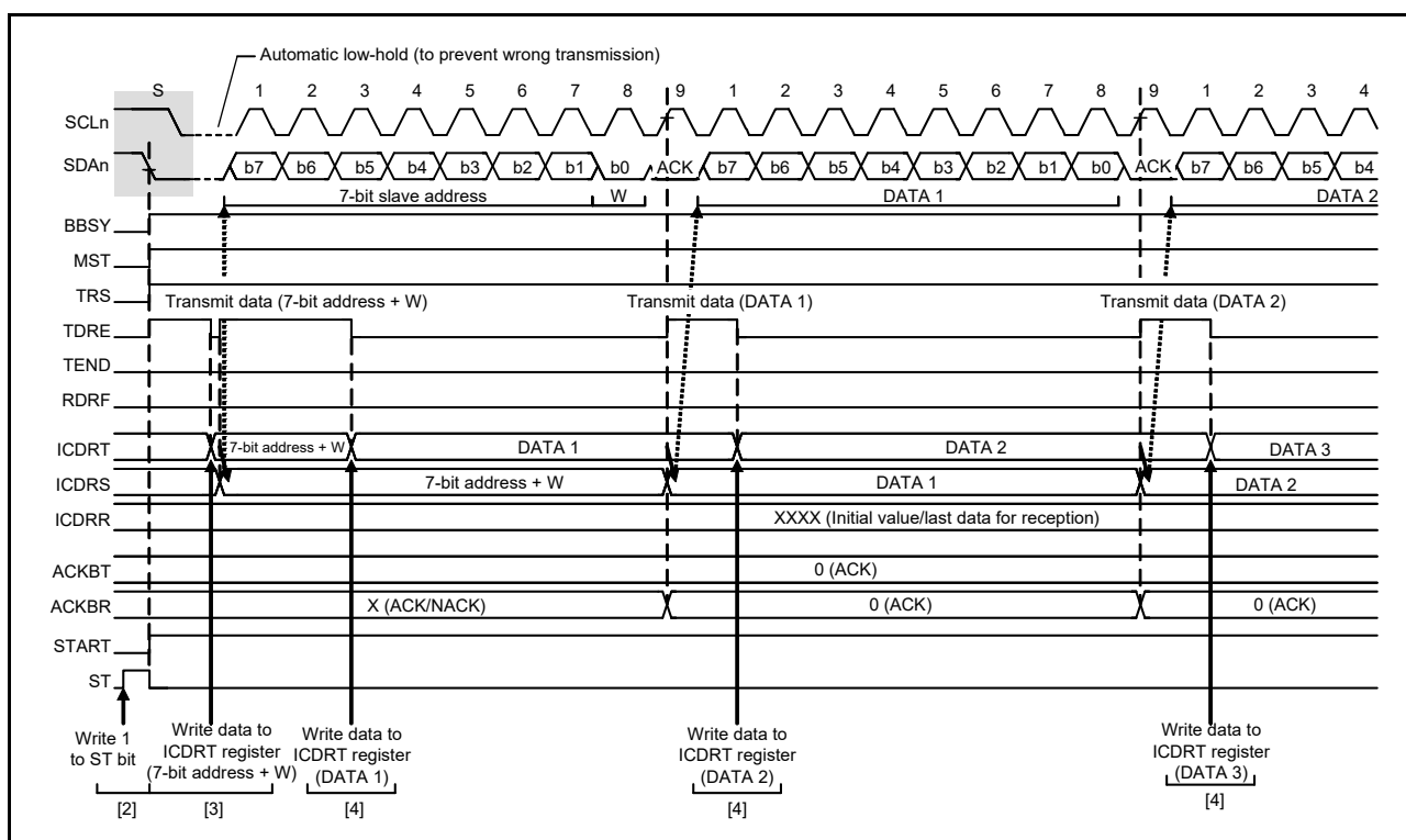
Figure 38.6 Master Transmit Operation Timing (1) (7-Bit Address Format)
