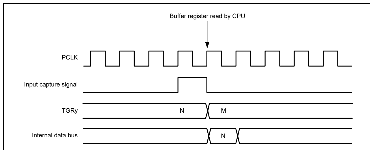
Figure 26.48 Conflict between TPUM.TGRy Read and Input Capture
