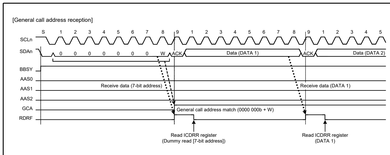
Figure 38.26 Timing of GCA Flag Setting during Reception of General Call Address
