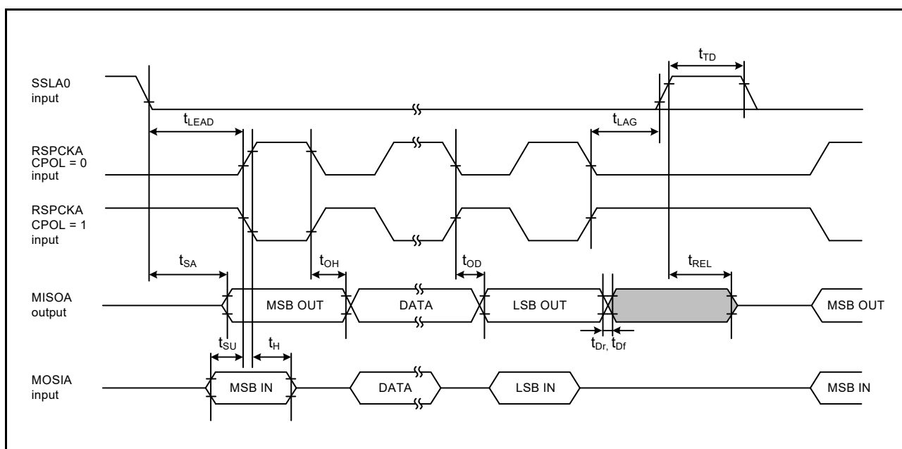
Figure 60.59 RSPI Timing (Slave, CPHA = 0)
