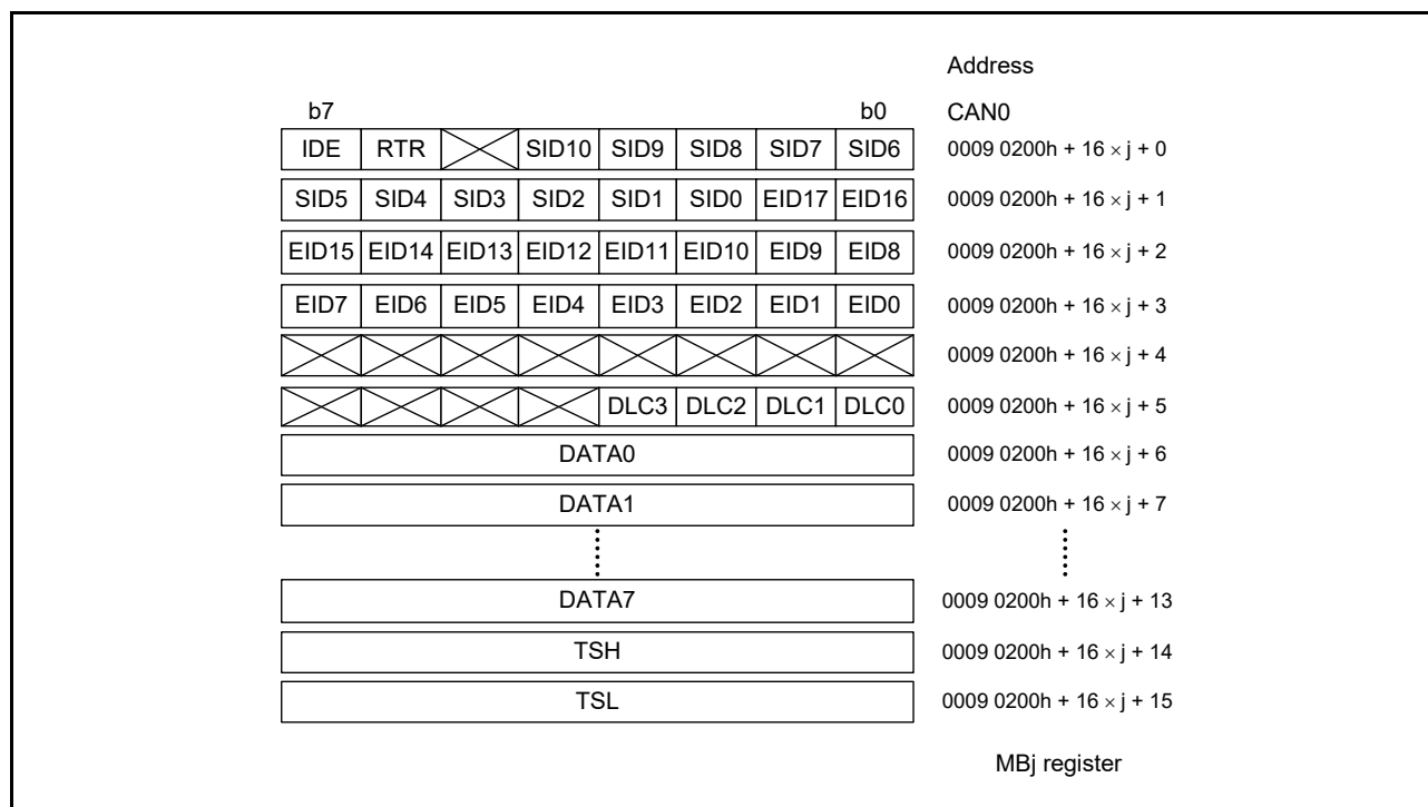
Figure 39.13 Structure of MBj (j = 0 to 31)
