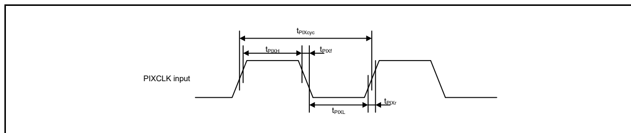
Figure 60.76 PDC Input Clock Timing
