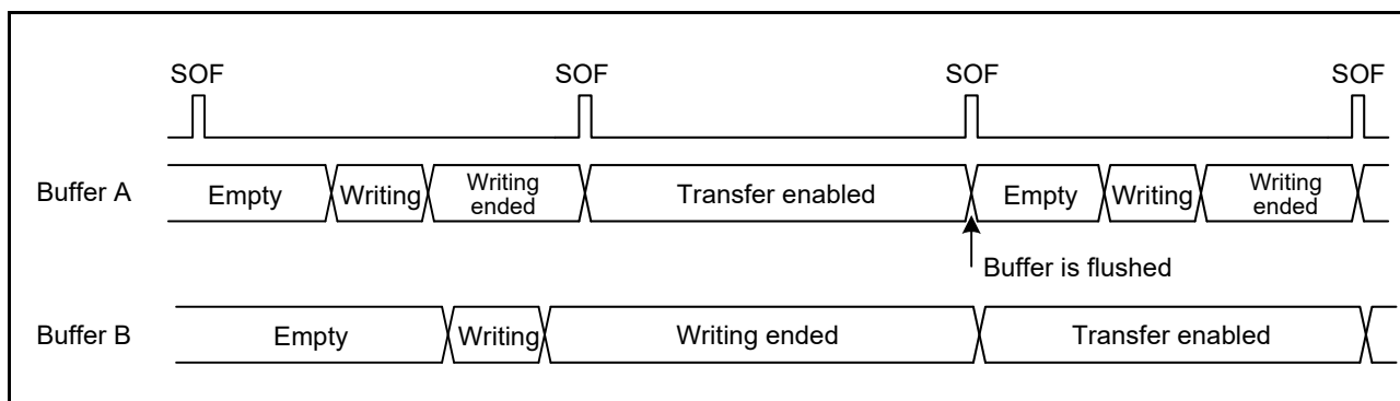
Figure 36.21 Example of Buffer Flush Operation
