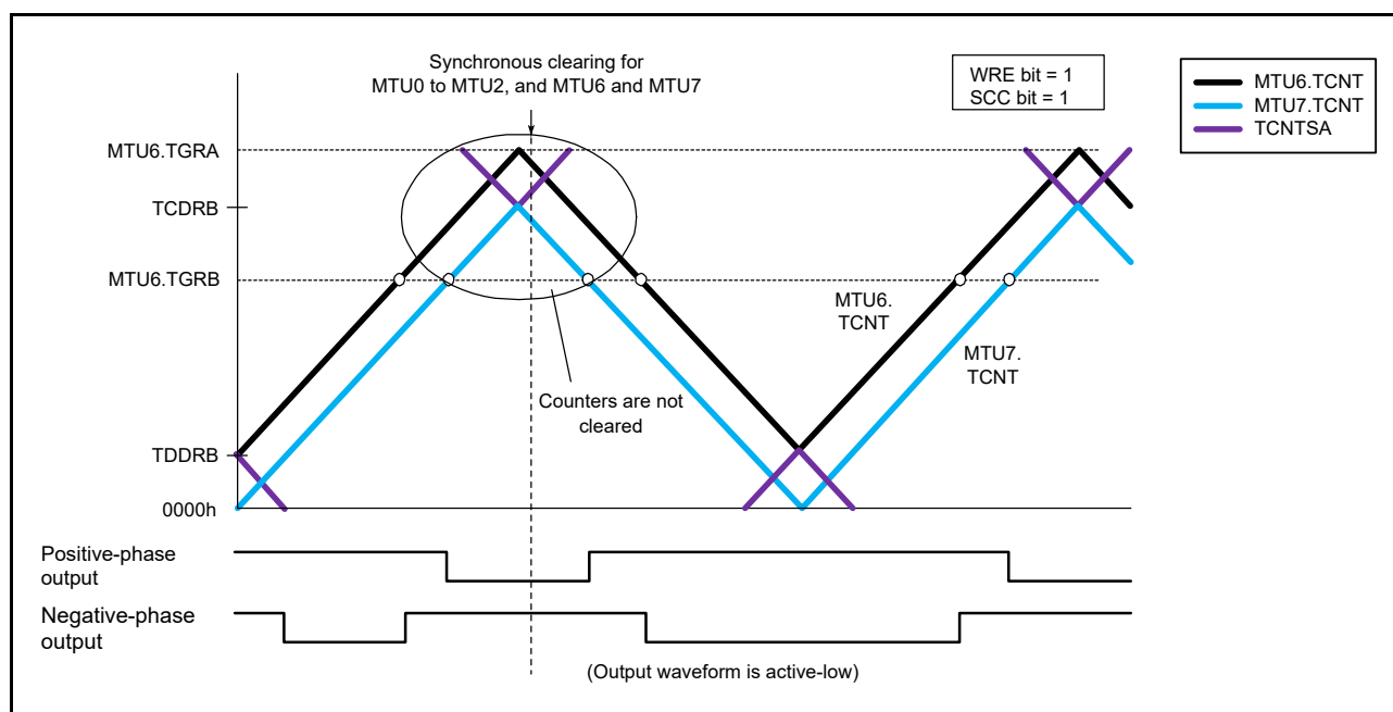
Figure 24.75 Example of Synchronous Clearing in Tb1 interval (Timing (6) in Figure 24.66; TWCRB.WRE Bit is 1 and SCC Bit is 1 in MTU6 and MTU7)
