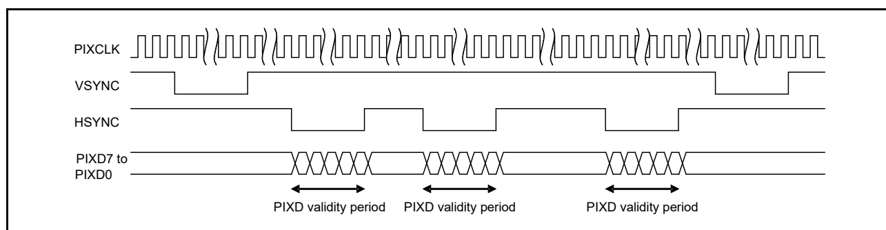
Figure 46.6 PDC Transfer Format (for VPS = 0, HPS = 1)
