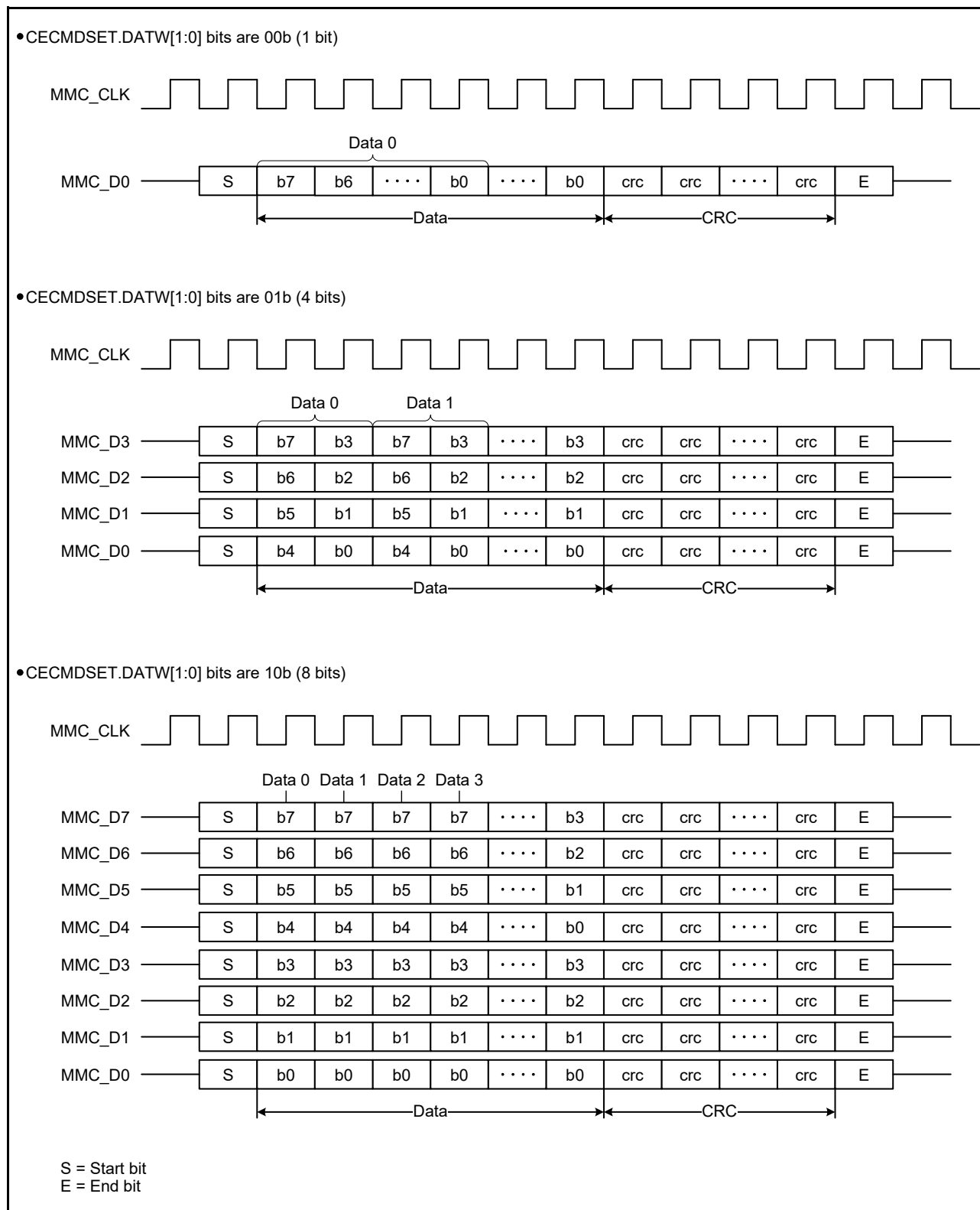
Figure 45.5 Data Block Format
