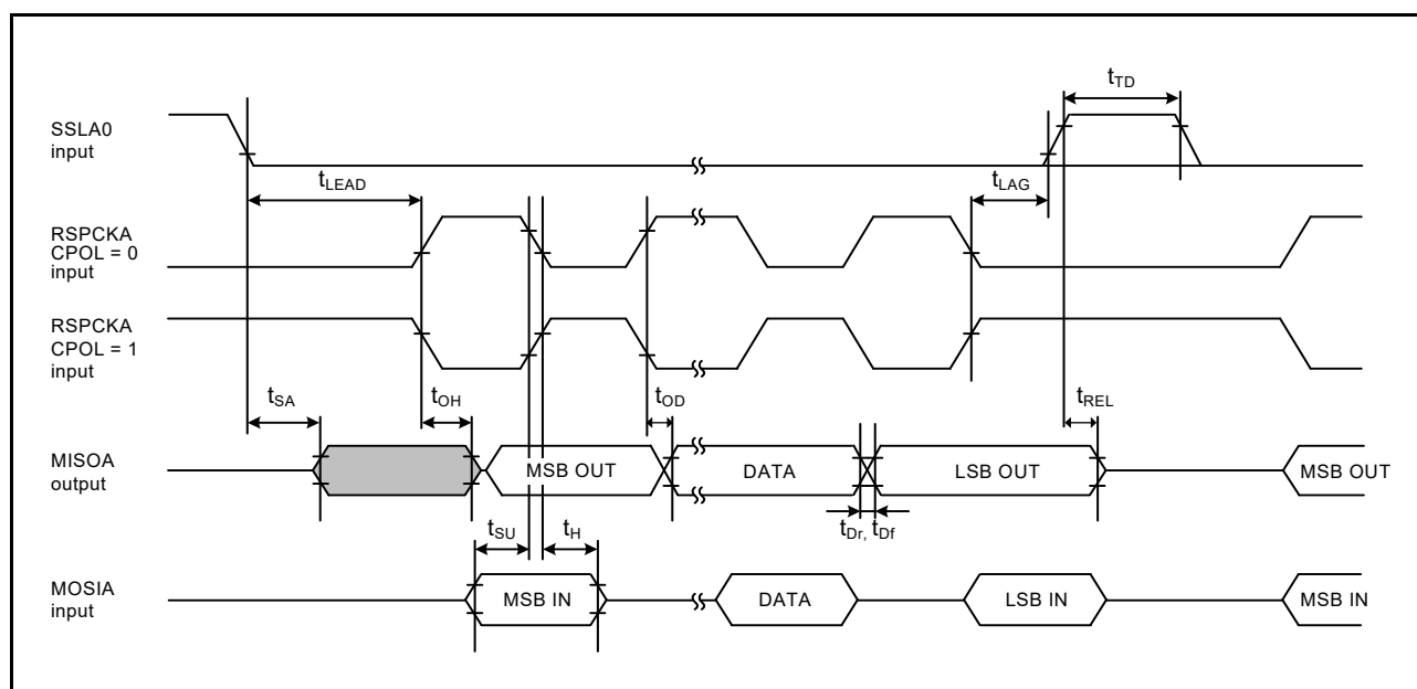
Figure 60.60 RSPI Timing (Slave, CPHA = 1)
