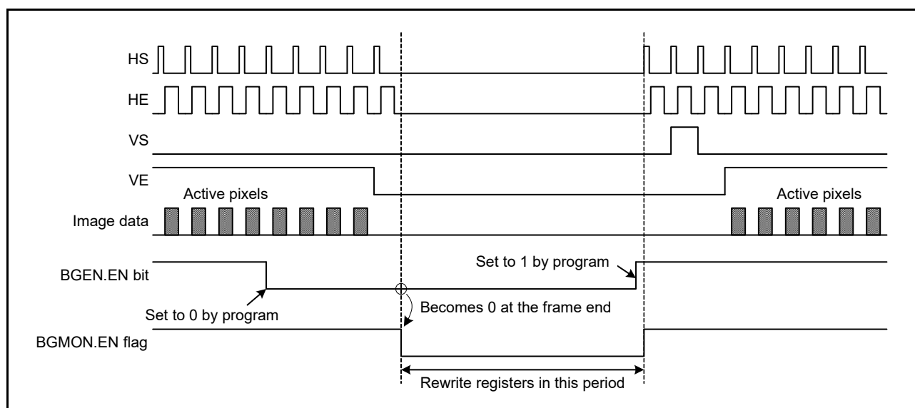
Figure 47.23 Stop and Restart in Normal Operation
