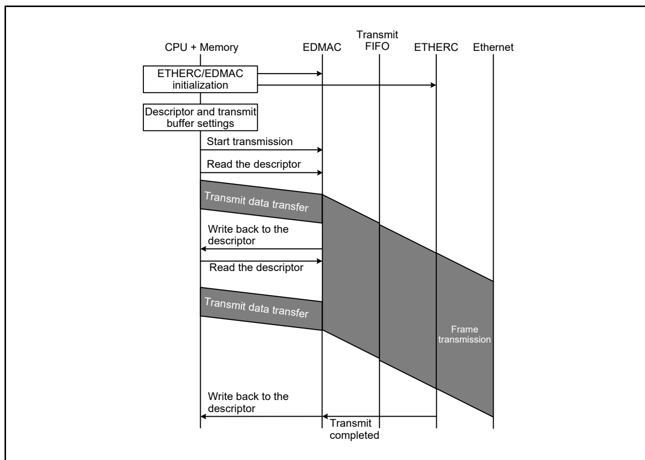
Figure 35.5 Example of Transmission Flow
