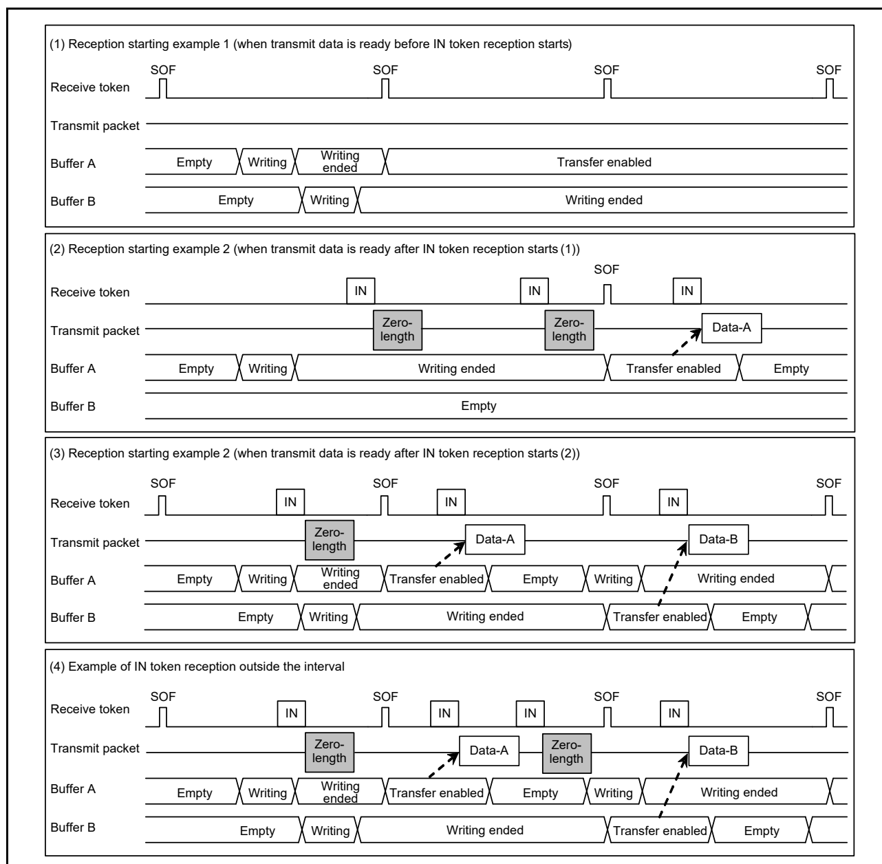
Figure 36.20 Example of Data Setup Function Operation
