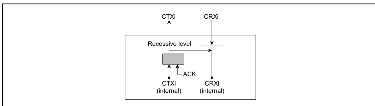
Figure 39.8 Connection when Self-Test Mode 1 is Selected ( i = 0, 1 )
