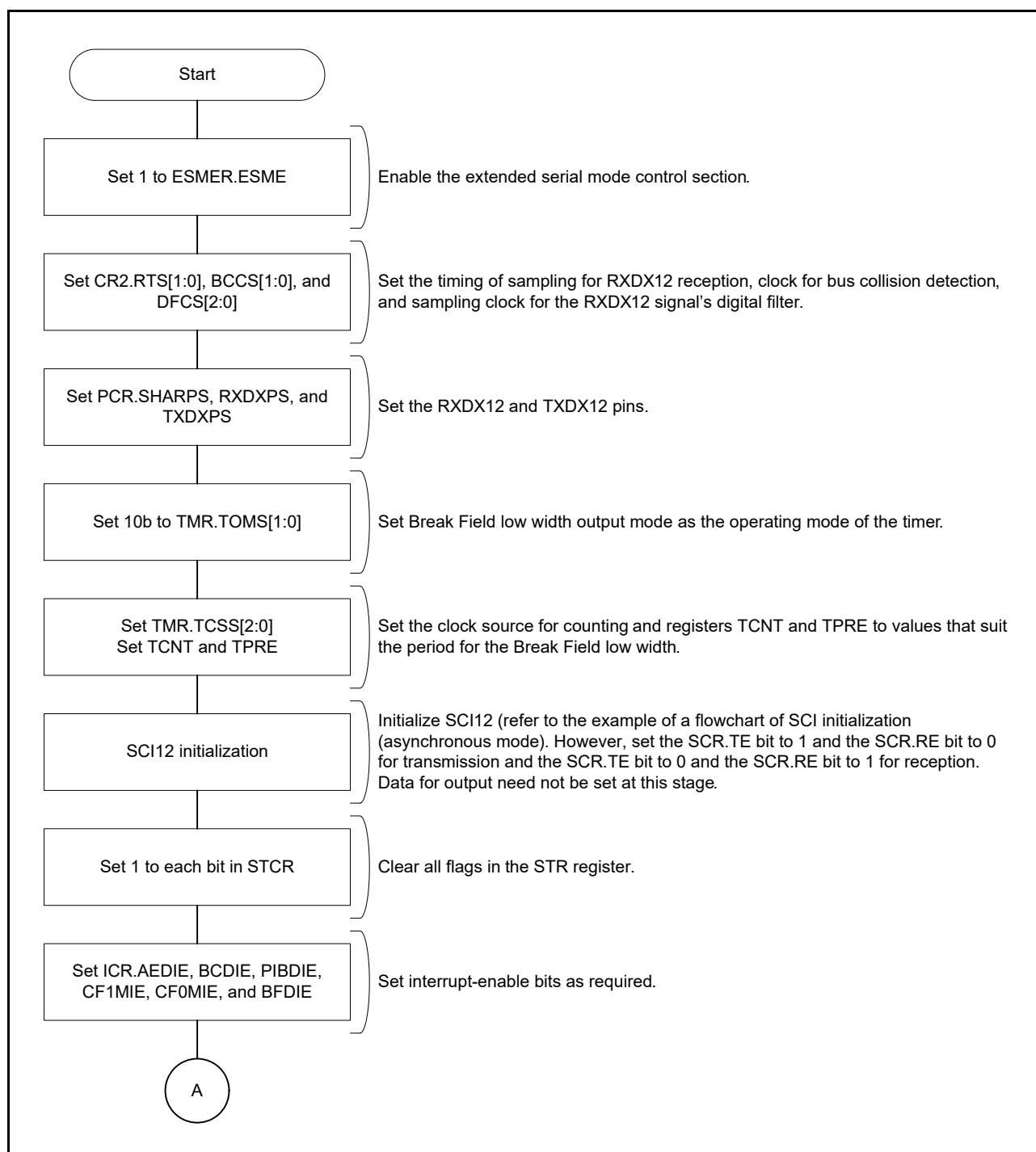
Figure 37.66 Example of Start Frame Transmission (1/2)
