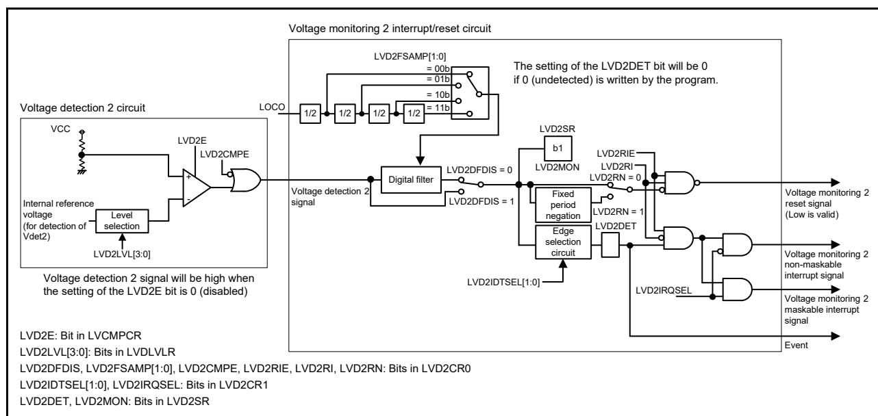
Figure 8.3 Block Diagram of Voltage Monitoring 2 Interrupt/Reset Circuit
