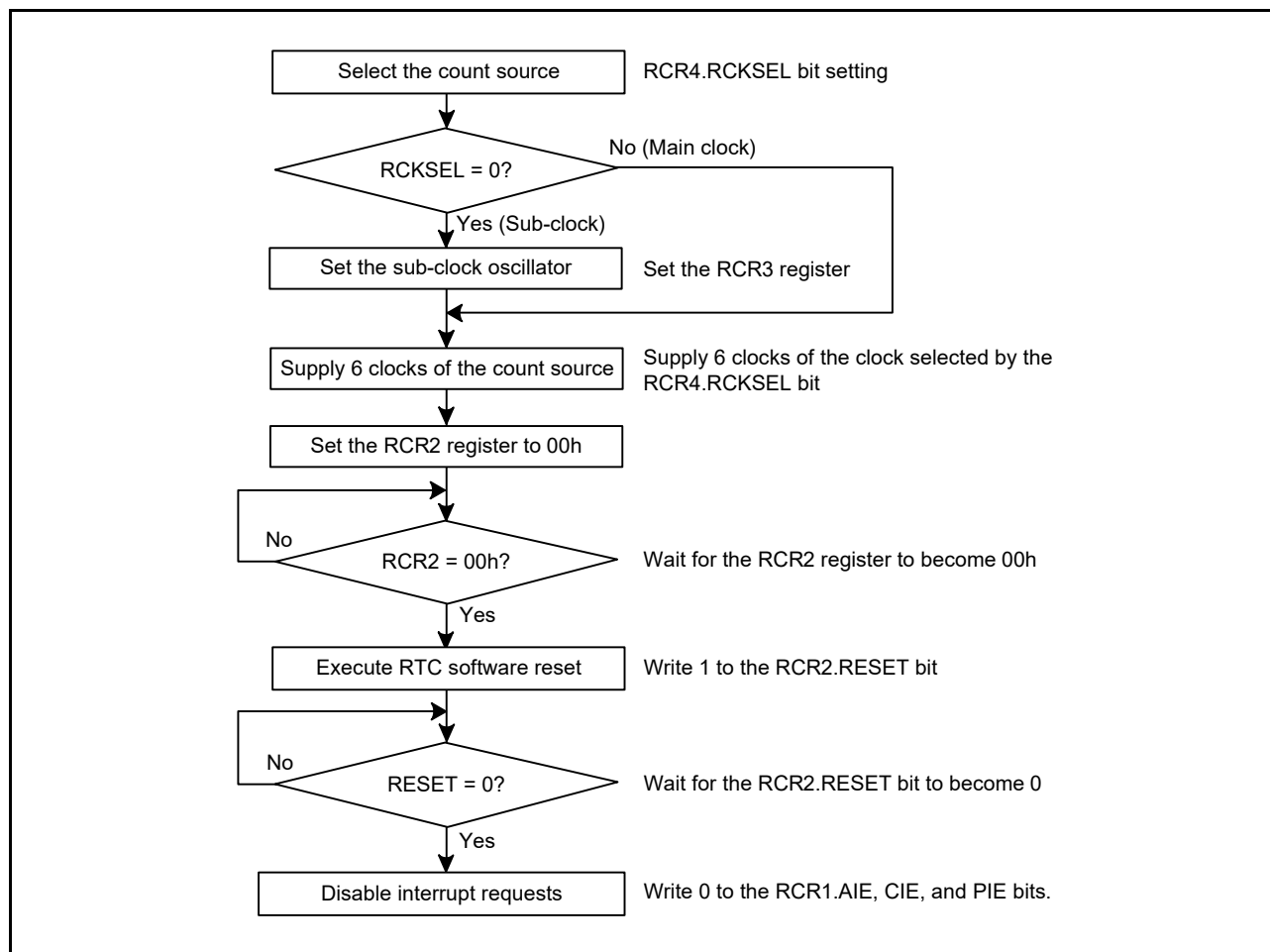
Figure 31.14 Initialization Procedure
