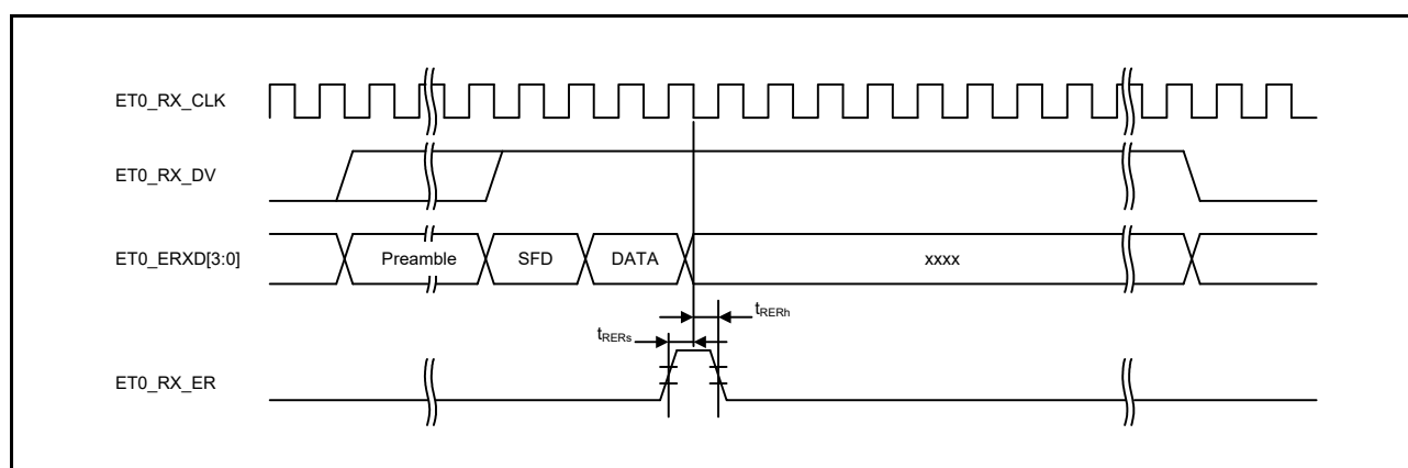
Figure 60.74 MII Reception Timing (Error Occurrence)
