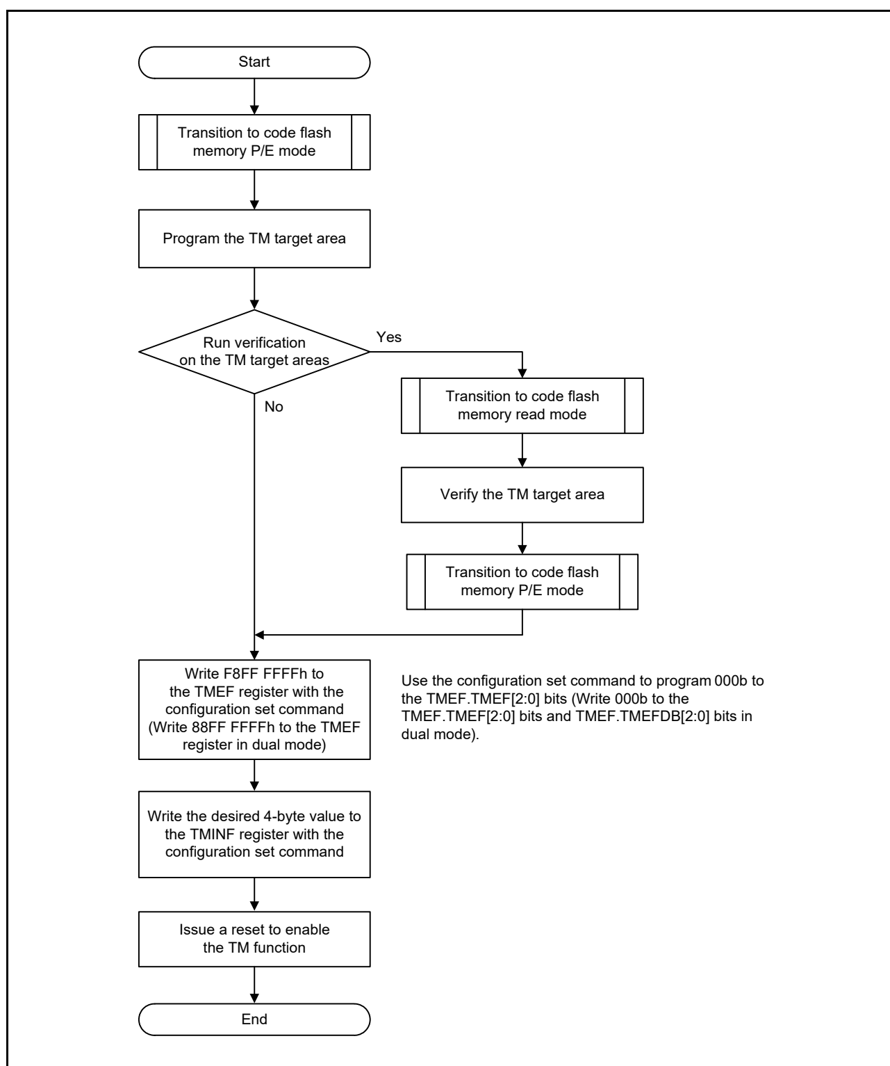
Figure 59.30 Flowchart for Enabling the TM Function by Self-Programming
