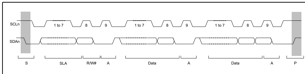
Figure 38.3 I 2 C-bus Timing (SLA = 7 Bits)
