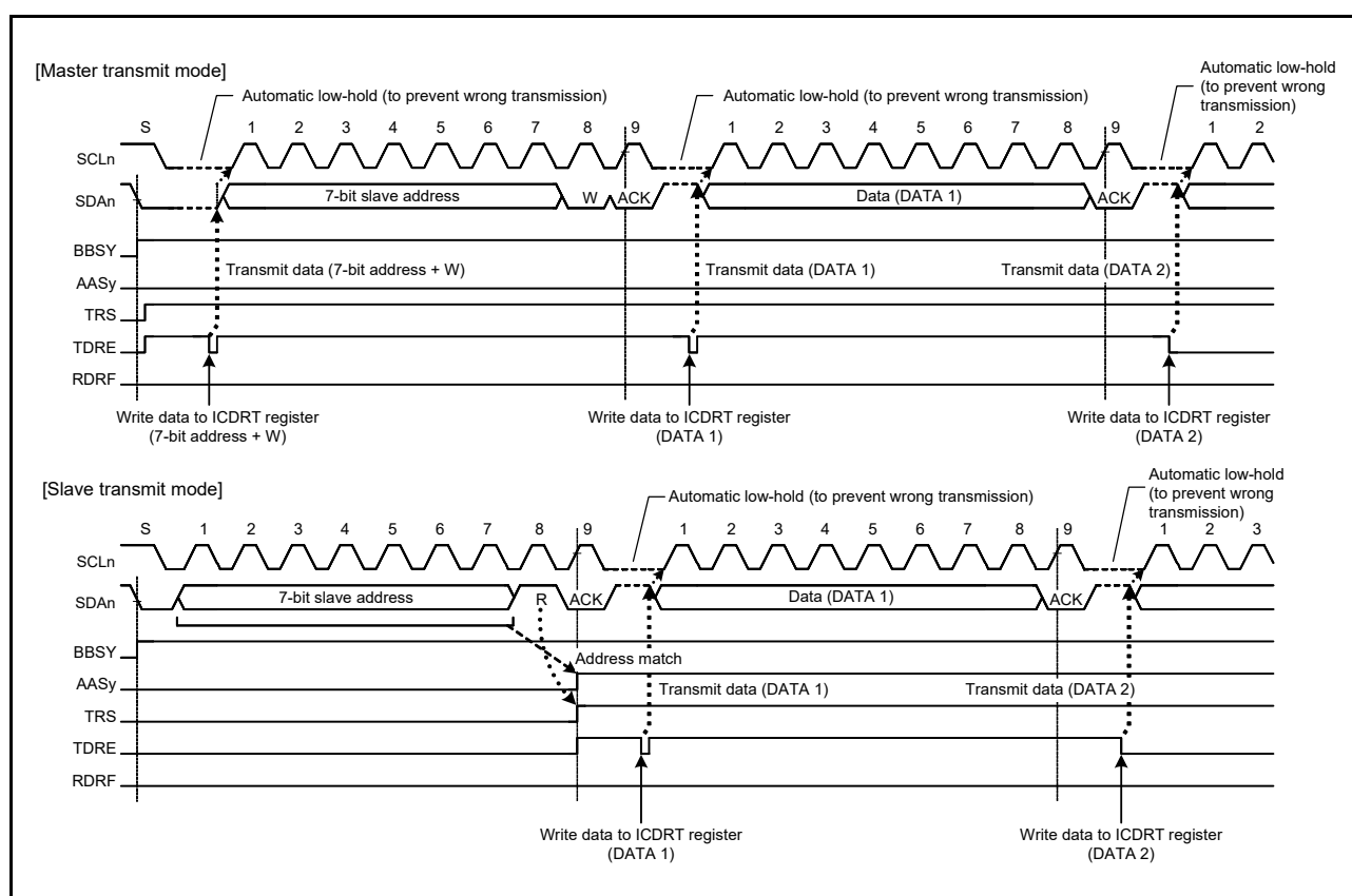
Figure 38.29 Automatic Low-Hold Operation in Transmit Mode
