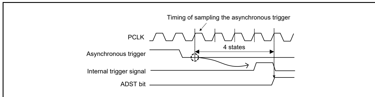
Figure 53.44 Timing of Sampling Asynchronous Trigger
