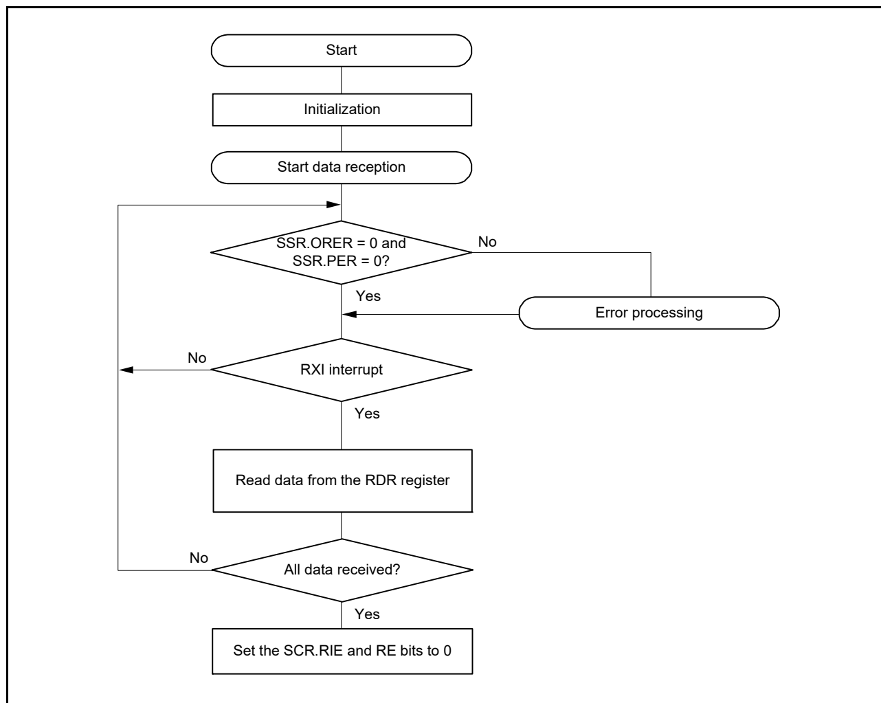
Figure 37.48 Sample Smart Card Interface Reception Flowchart
