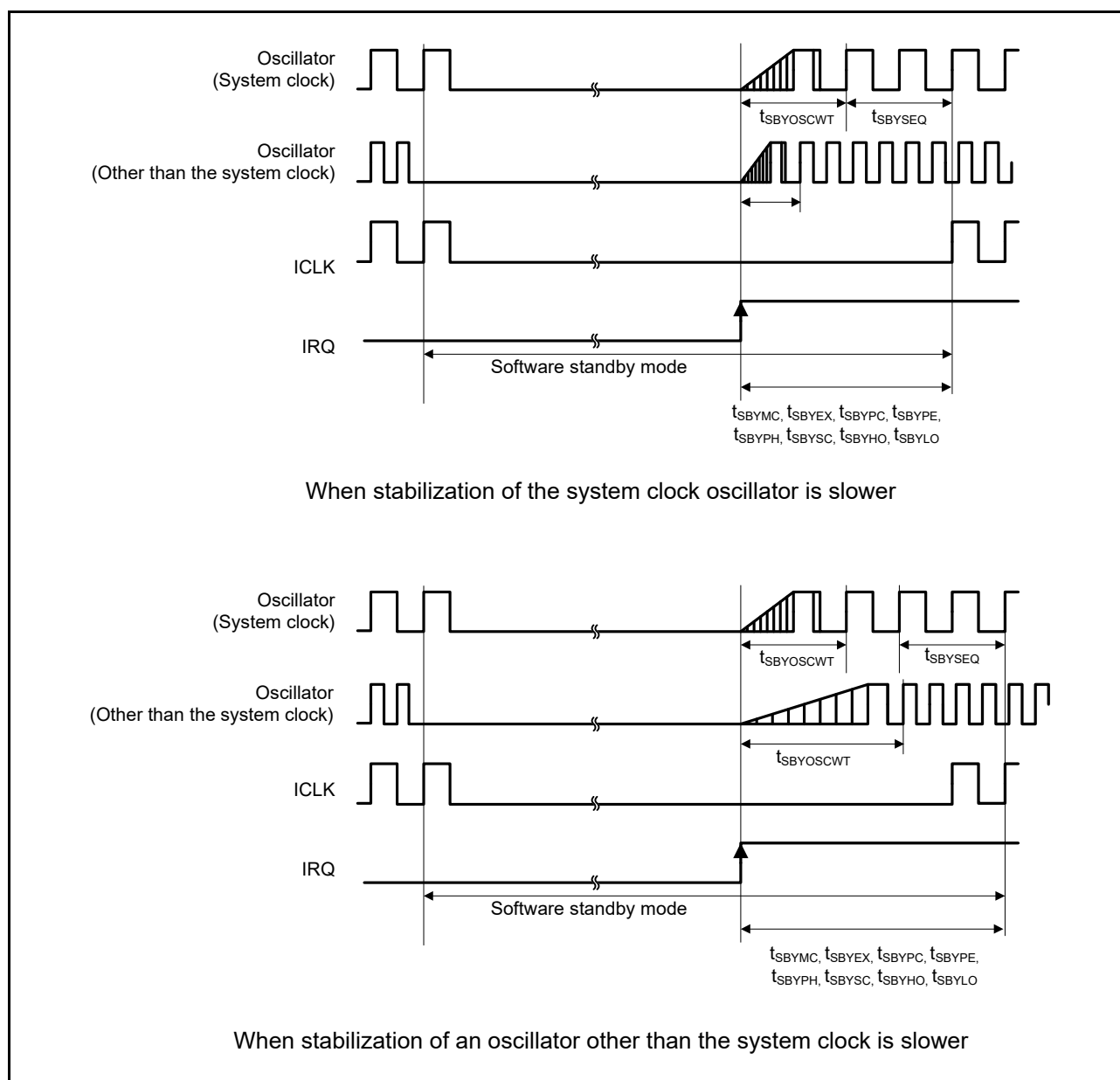
Figure 60.12 Software Standby Mode Recovery Timing
