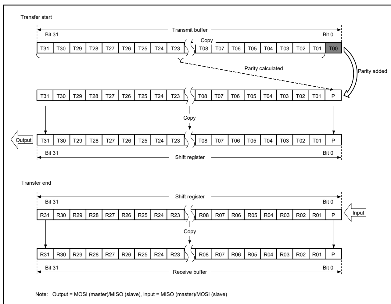
Figure 40.18 MSB First Transfer (32-Bit Data, Parity Enabled)
