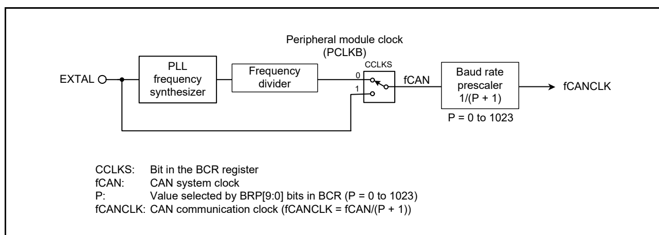
Figure 39.11 Block Diagram of CAN Clock Generator
