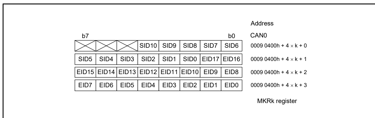
Figure 39.14 Structure of MKRk (k = 0 to 7)
