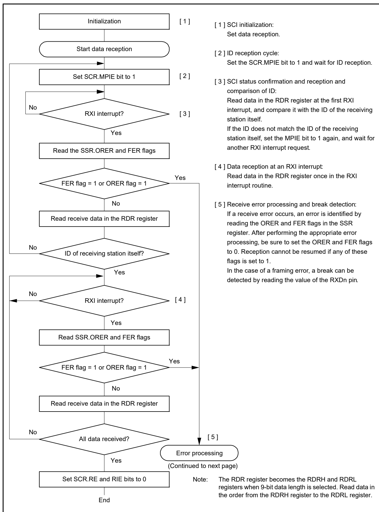
Figure 37.25 Example of Multi-Processor Serial Reception Flowchart (1)
