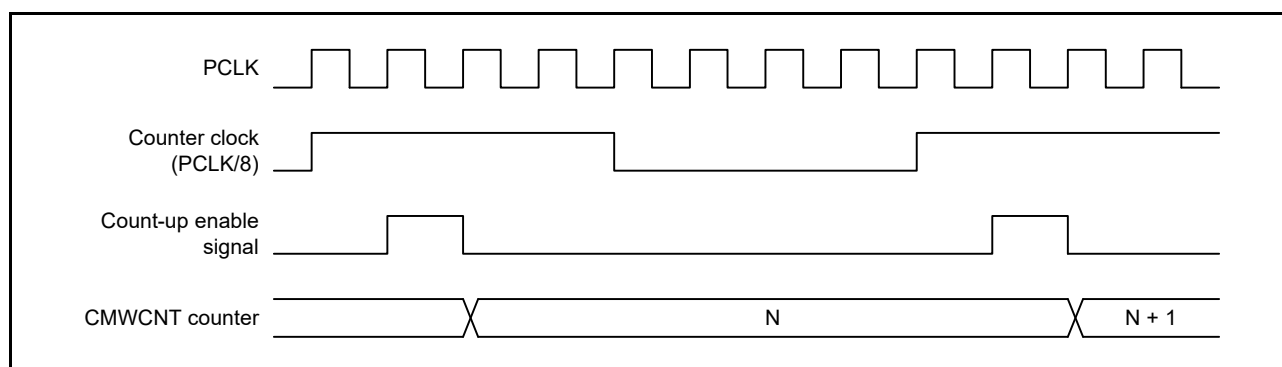
Figure 30.10 Count Timing (PCLK/8)
