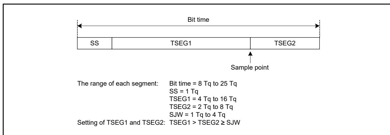
Figure 39.12 Bit Timing
