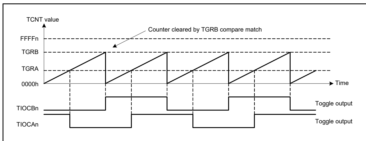
Figure 26.7 Example of Toggle Output Operation (n = 0 to 5)
