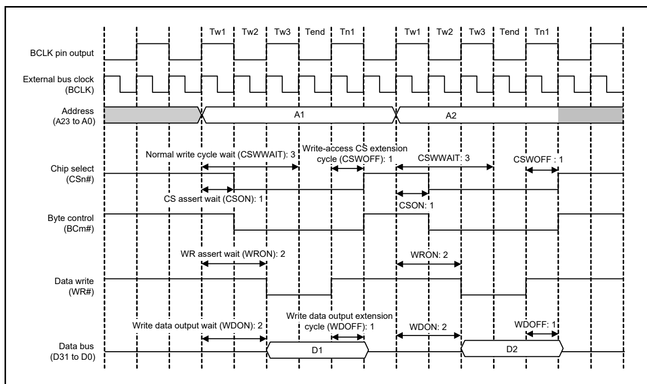
Figure 16.28 Example of Normal-Write Operation (when 1/2 BCLK is Selected with the BCLK Pin Output Select Bit) (n = 0 to 7, m = 0 to 3)
