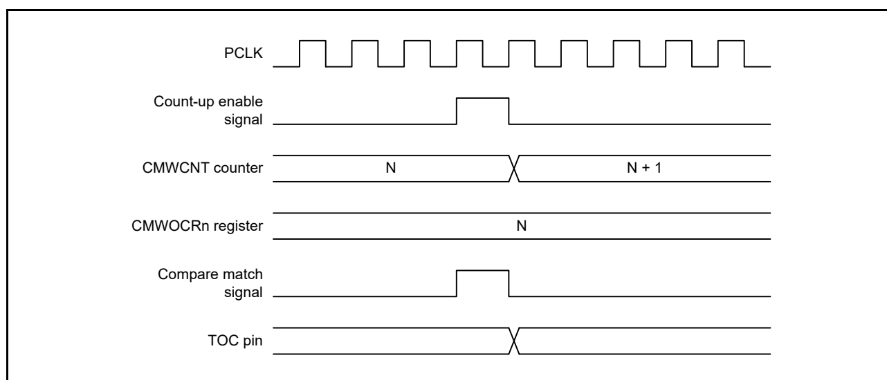
Figure 30.11 Output Compare Output Timing
