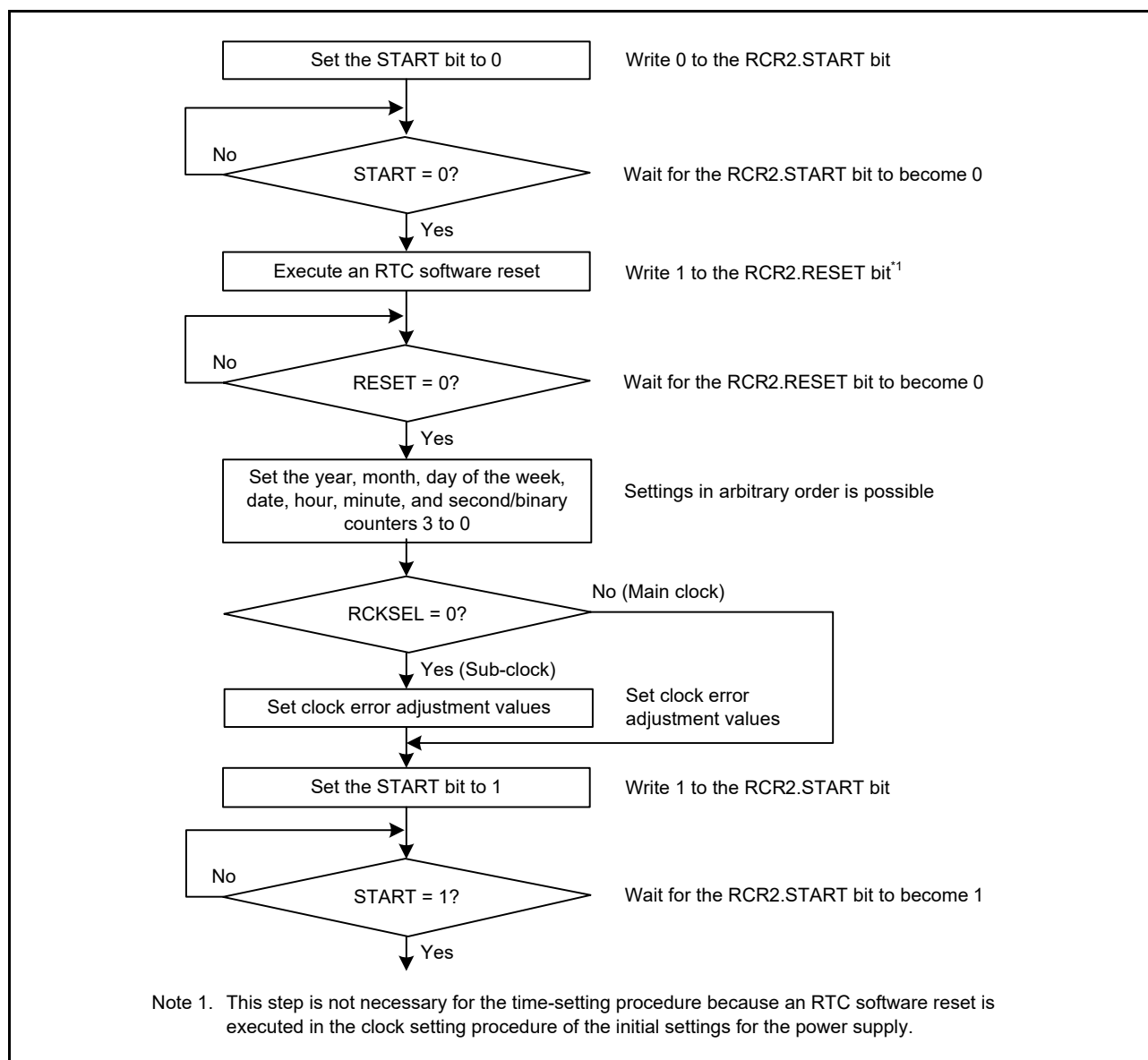
Figure 31.4 Setting the Time
