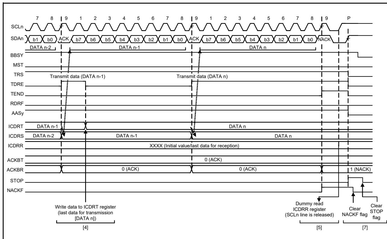
Figure 38.16 Slave Transmit Operation Timing (2)
