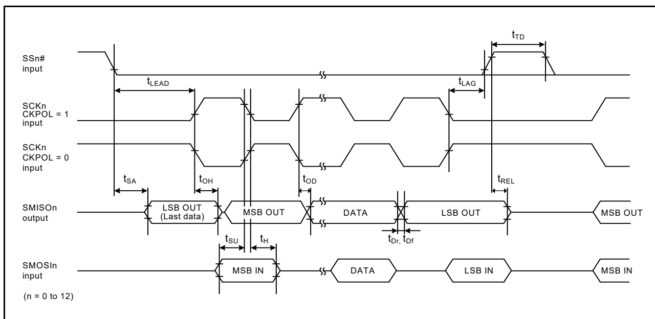
Figure 60.53 Simple SPI Timing (Slave, CKPH = 0)
