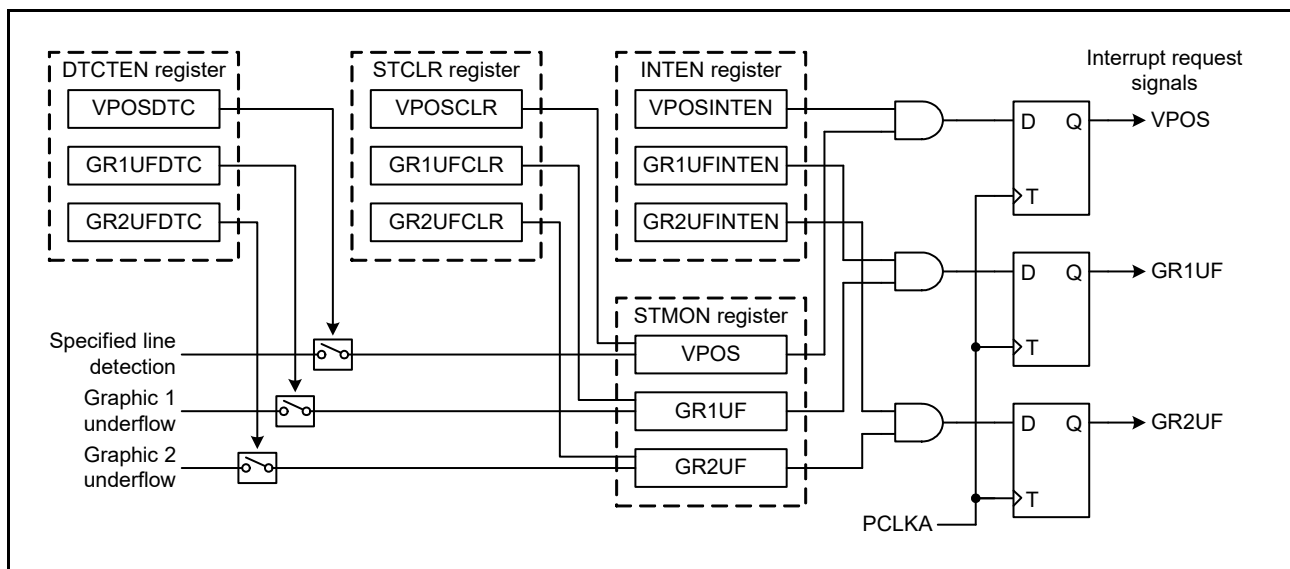
Figure 47.25 Interrupt Request Signal Generating Circuit
