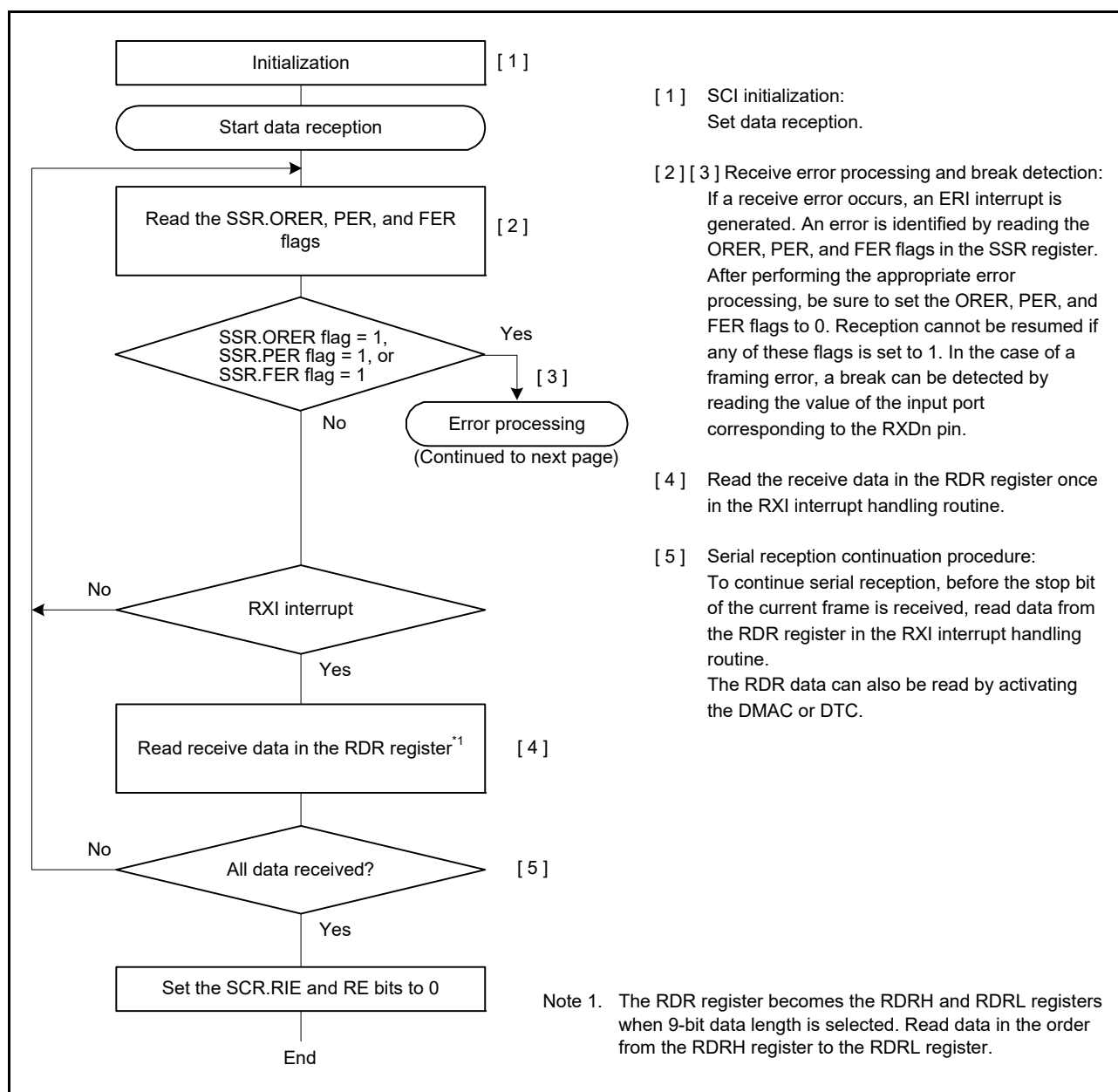
Figure 37.20 Example Flowchart of Serial Reception in Asynchronous Mode (1)
