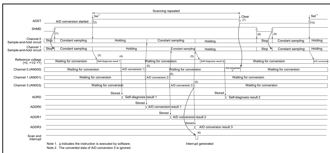
Figure 53.20 Example of Operation in Sequence Scan Mode (Channel-Dedicated Sample-and-Hold Circuits Used: AN000, AN001, and AN003 Selected + Self-Diagnosis, With Constant Sampling Enabled)
