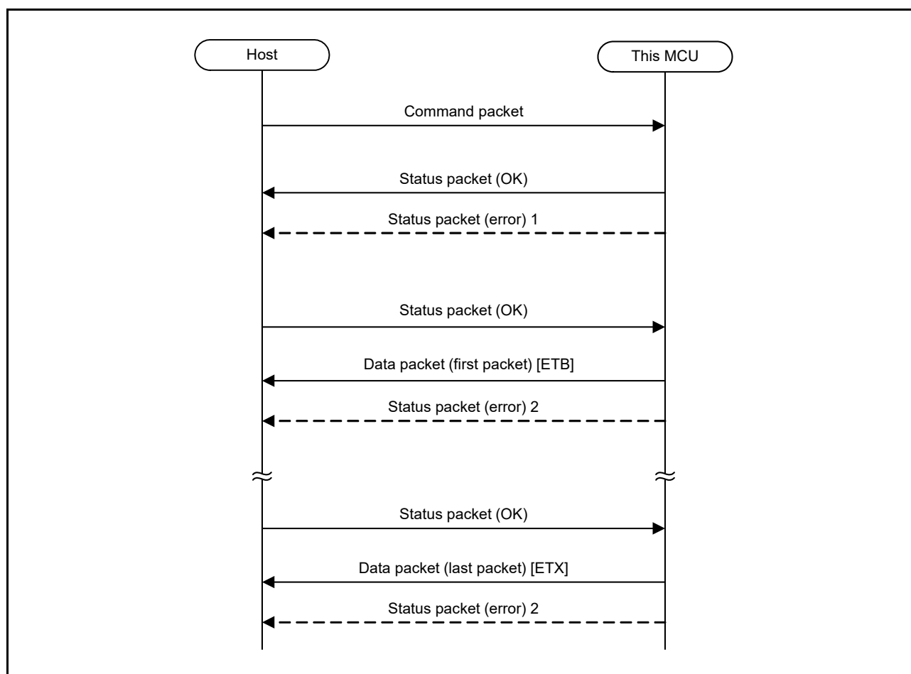
Figure 59.21 Read Command Transfer Sequence
