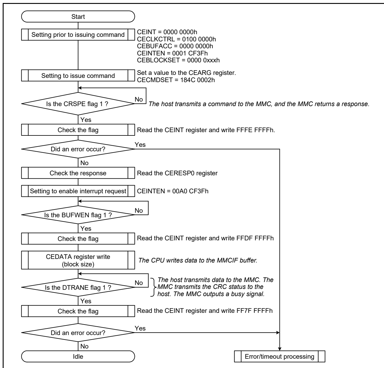
Figure 45.18 Issuing a Single Block Write Command (CMD24)
