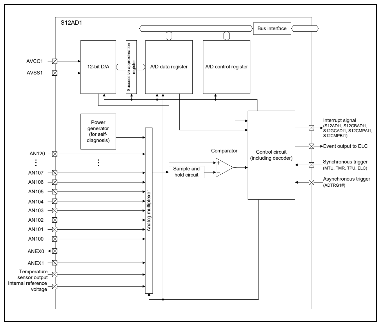
Figure 53.2 Block Diagram of 12-Bit A/D Converter (Unit 1)
