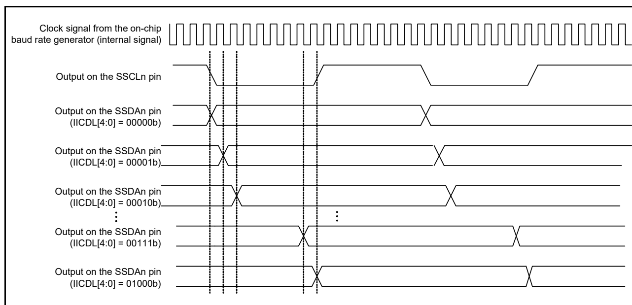
Figure 37.54 Timing of Delays in SSDA Output
