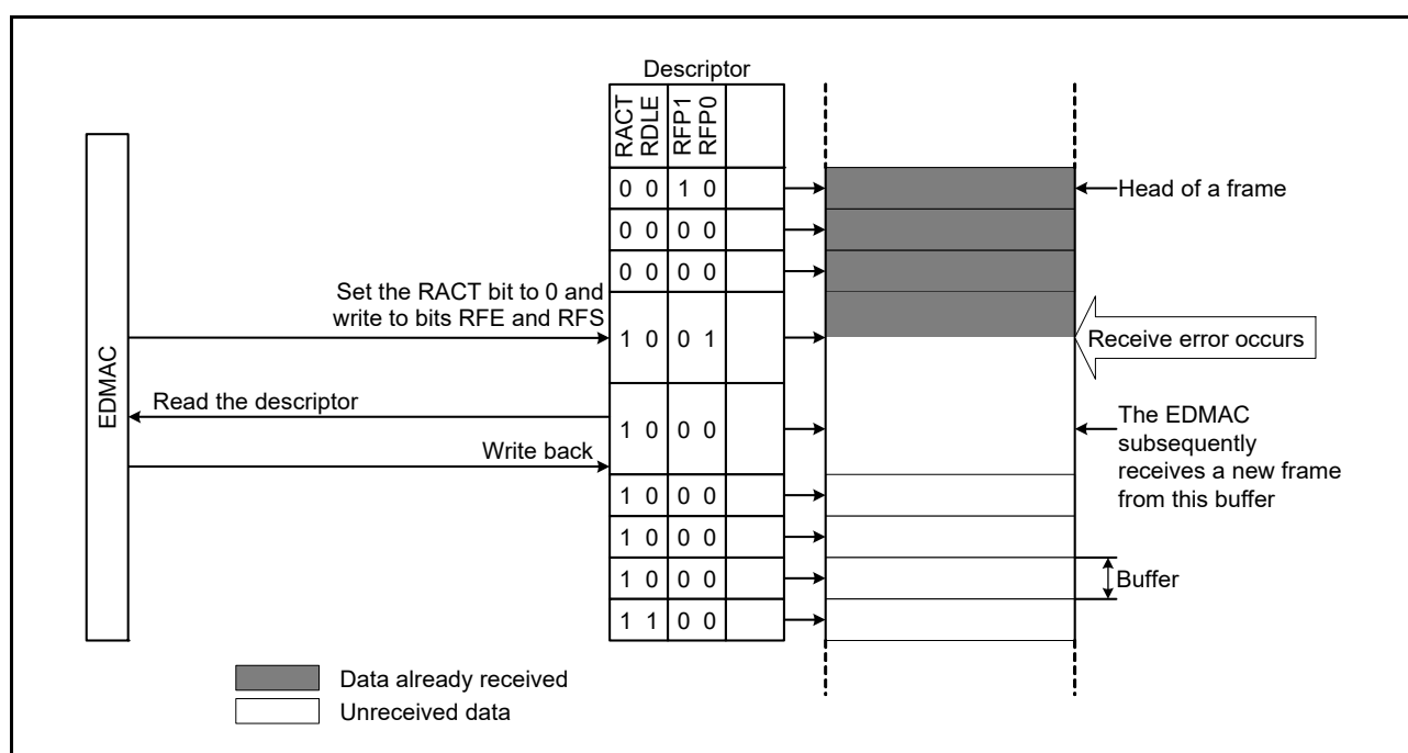
Figure 35.8 EDMAC Operation After a Receive Error Occurs
