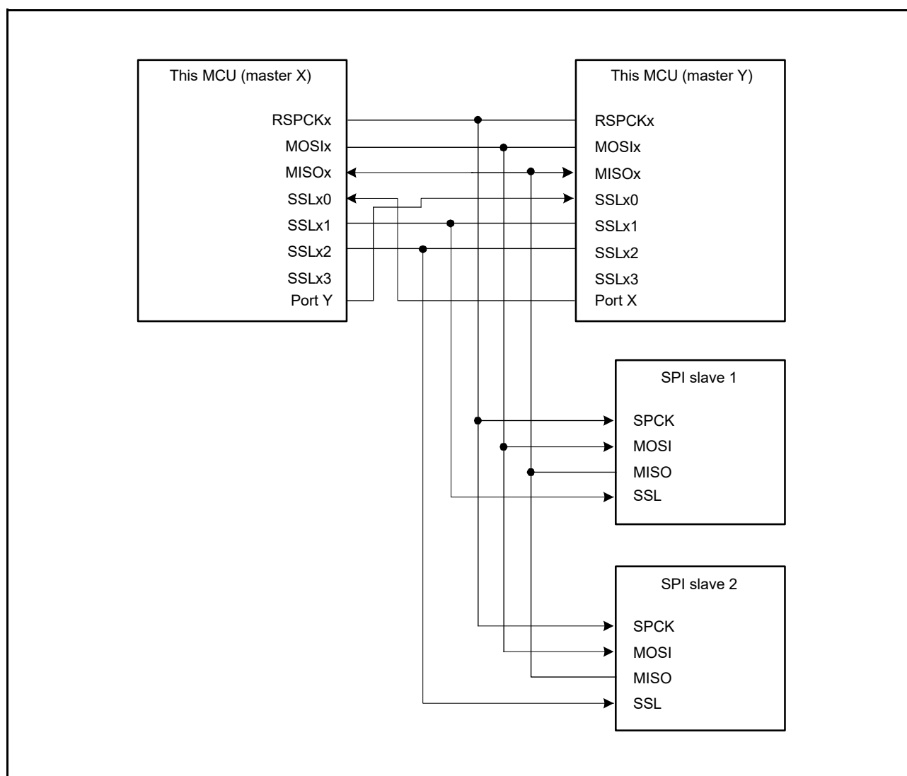
Figure 40.10 Multi-Master/Multi-Slave Configuration Example (This MCU = Master)
