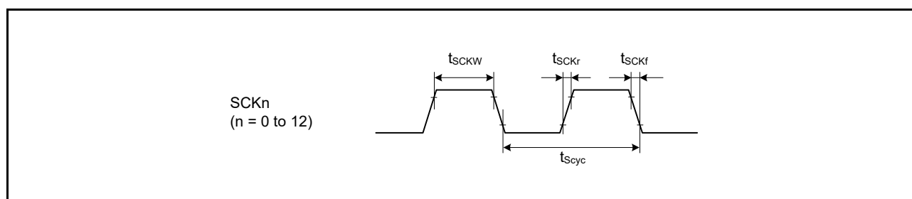
Figure 60.46 SCK Clock Input Timing
