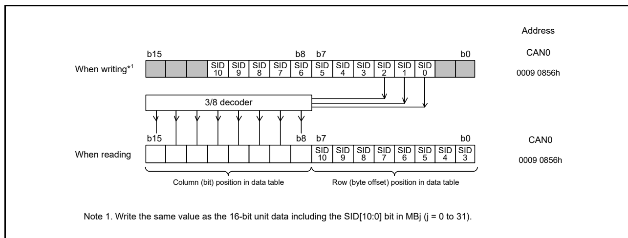
Figure 39.5 Write and Read of AFSR
