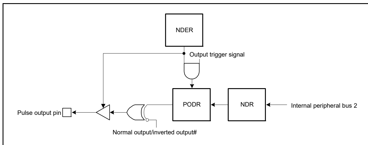
Figure 27.4 Schematic Diagram of PPG
