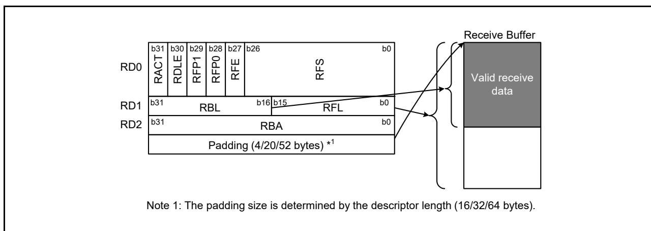
Figure 35.4 Relation between Receive Descriptor and Receive Buffer
