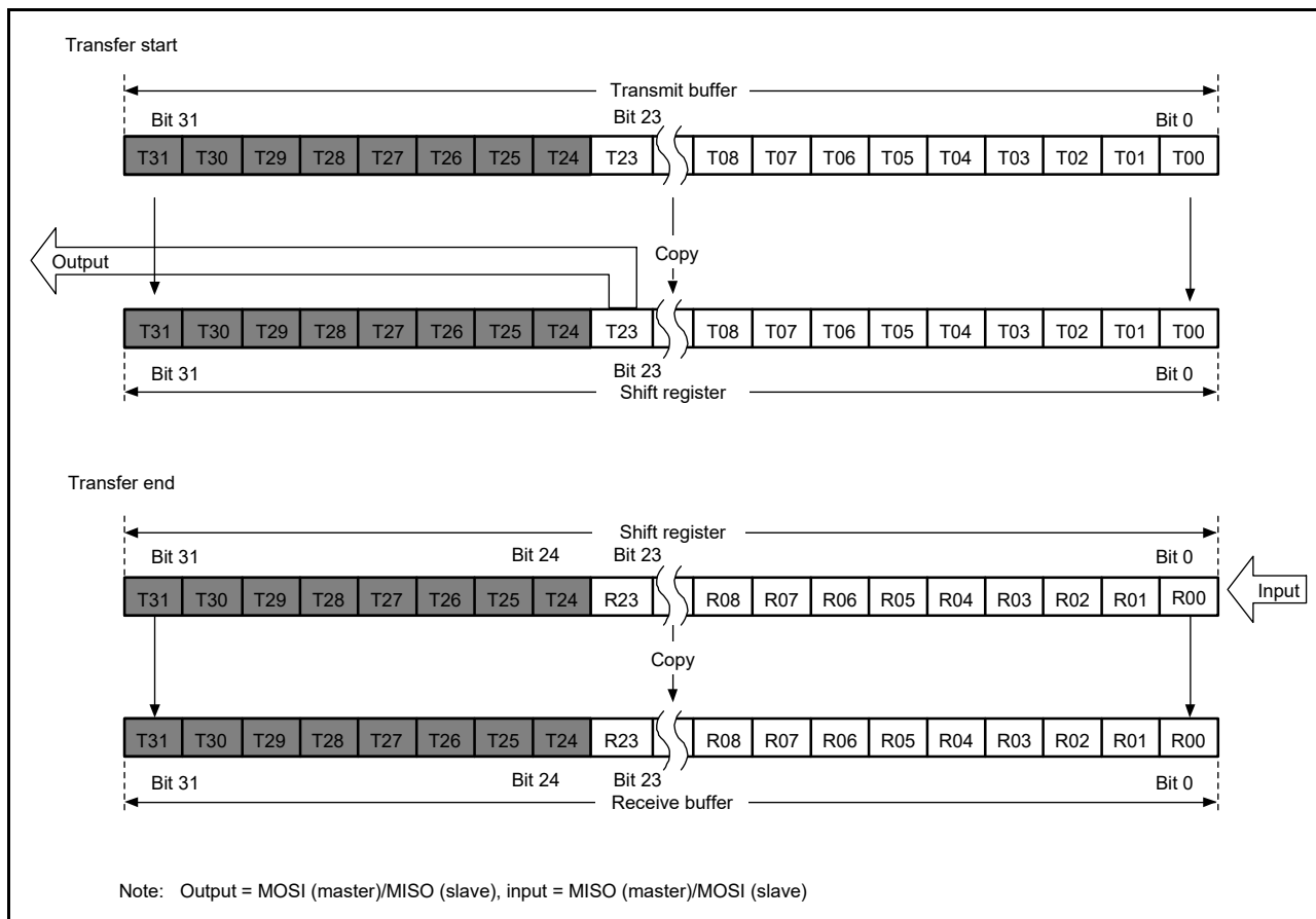
Figure 40.15 MSB First Transfer (24-Bit Data, Parity Disabled)
