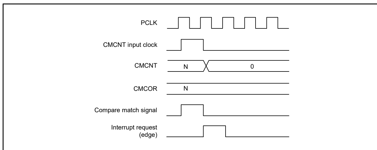
Figure 29.4 Timing of a Compare Match Interrupt
