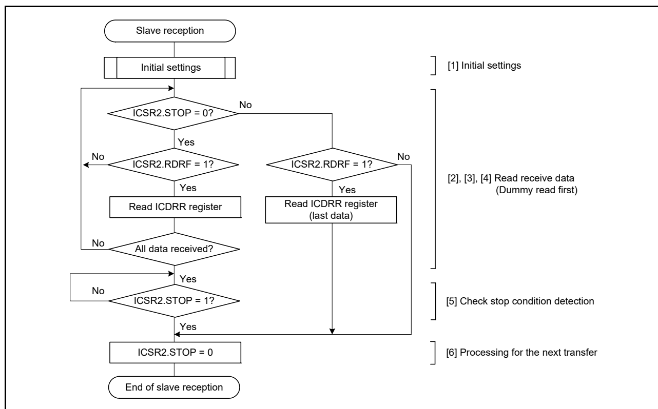
Figure 38.17 Example of Slave Reception Flowchart
