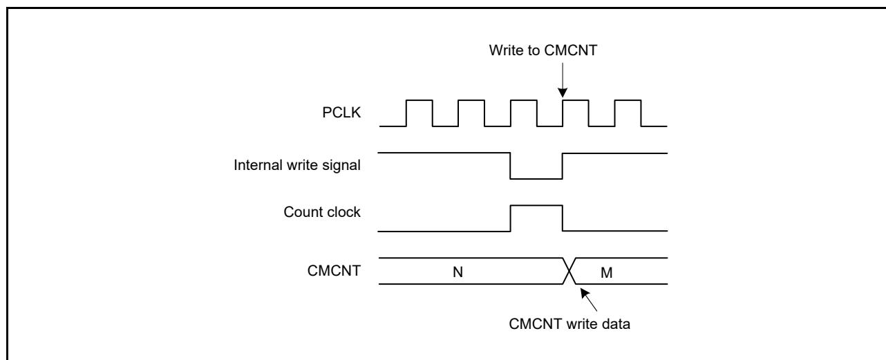
Figure 29.6 Conflict between CMCNT Counter Writing and Incrementing
