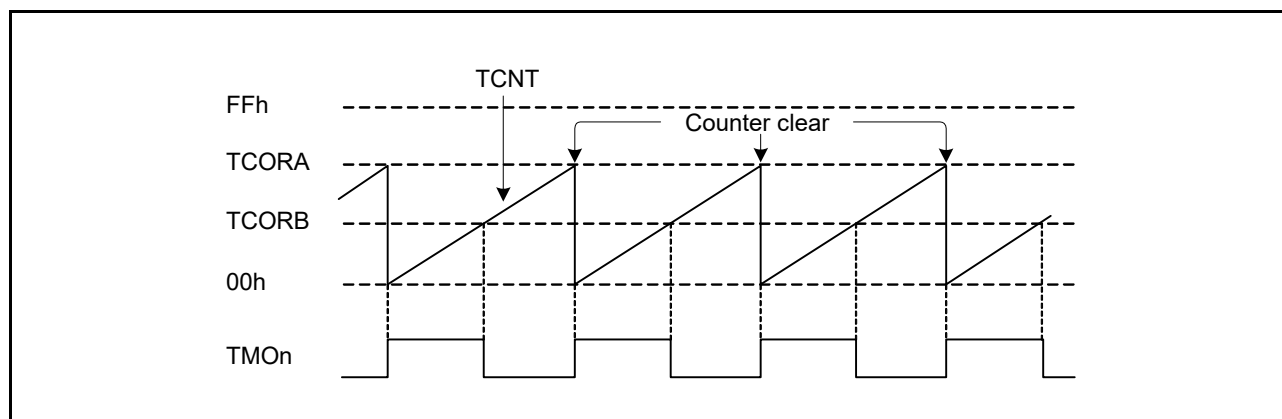
Figure 28.3 Example of Pulse Output (n = 0 to 3)
