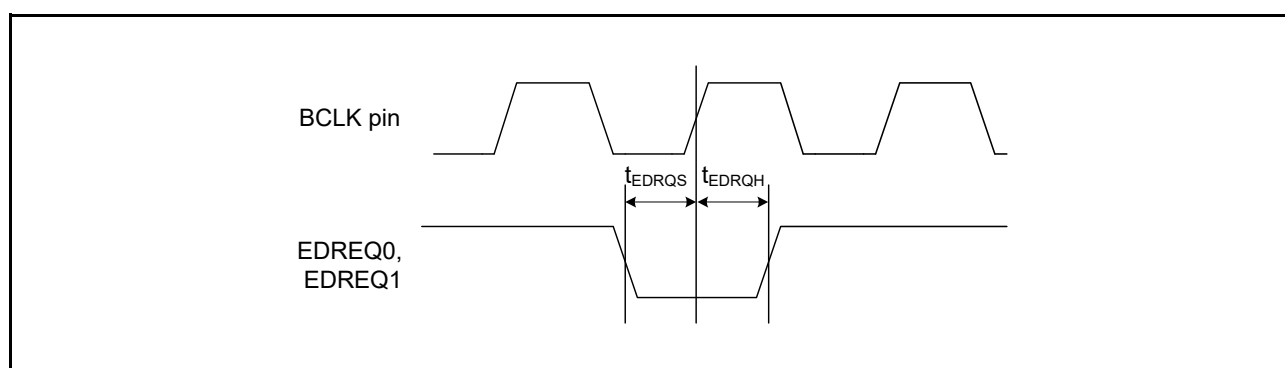
Figure 60.30 EDREQ0 and EDREQ1 Input Timing
