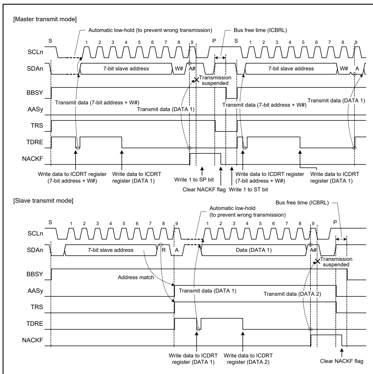
Figure 38.30 Suspension of Data Transmission When NACK is Received (NACKF = 1)
