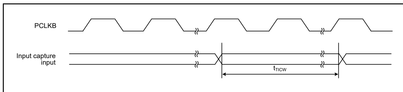
Figure 60.34 TPU Input Capture Input Timing
