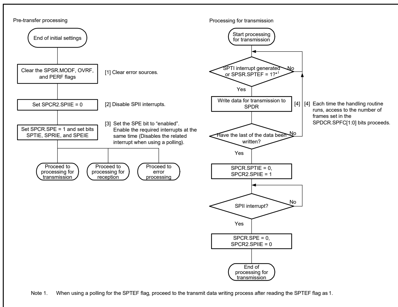
Figure 40.38 Flowchart in Master Mode (Transmission)
