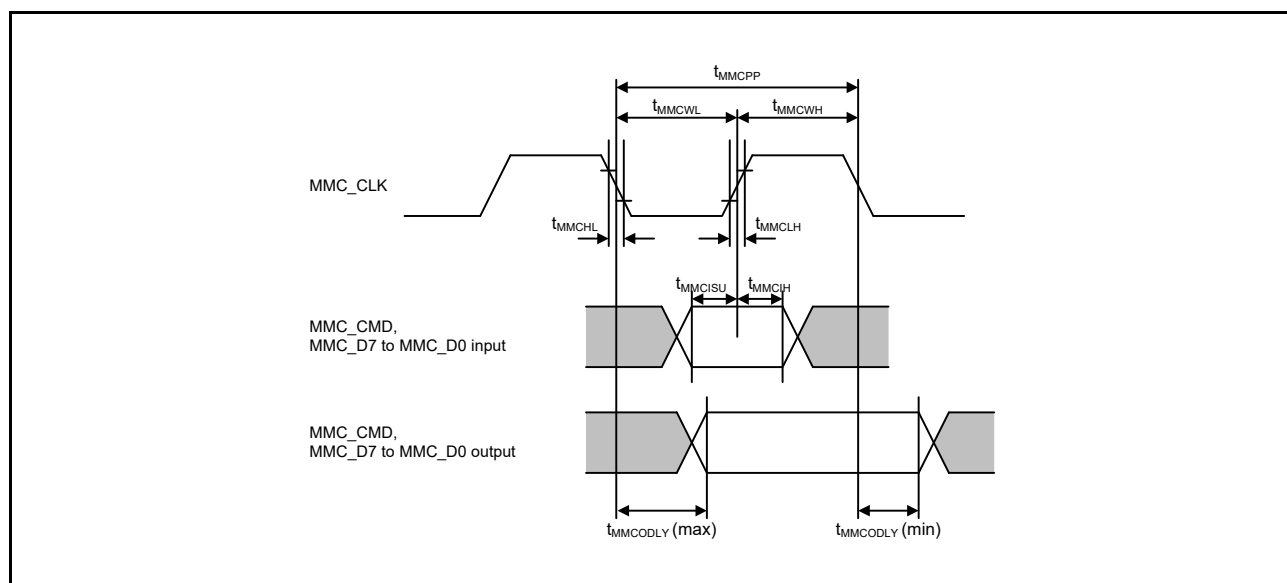
Figure 60.65 MMC Interface
