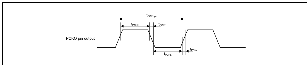
Figure 60.77 PDC Output Clock Timing
