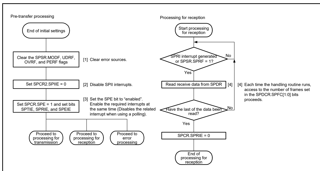
Figure 40.43 Flowchart in Slave Mode (Reception)
