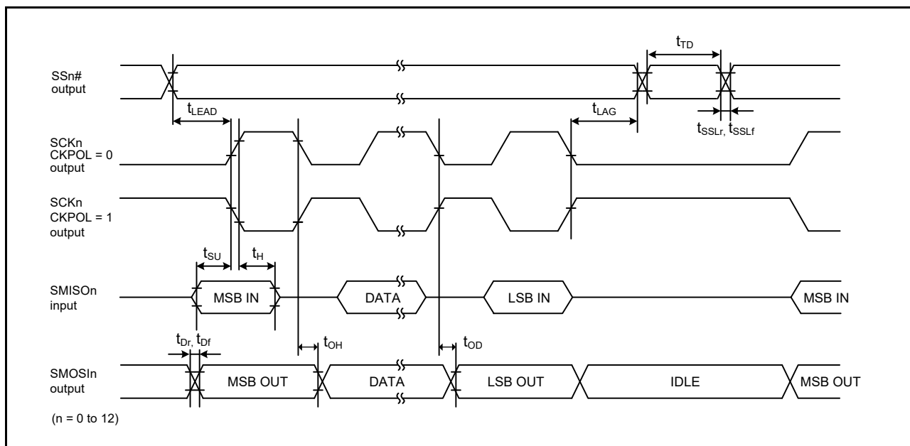
Figure 60.50 Simple SPI Timing (Master, CKPH = 1)
