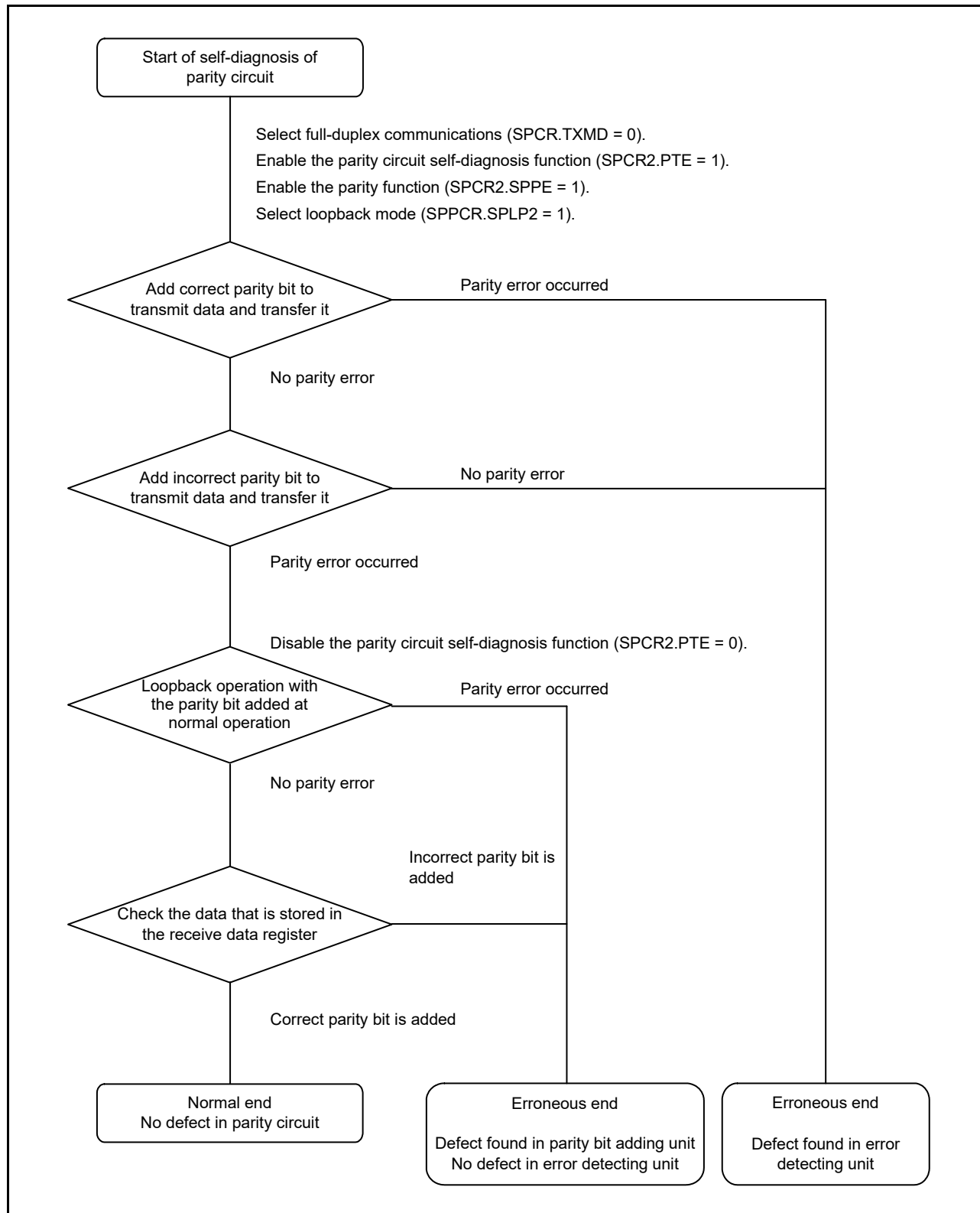
Figure 40.51 Flowchart for Self-Diagnosis of Parity Circuit
