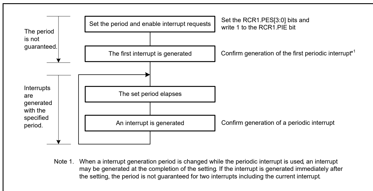
Figure 31.13 Using Periodic Interrupt Function
