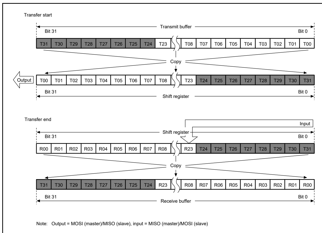
Figure 40.17 LSB First Transfer (24-Bit Data, Parity Disabled)
