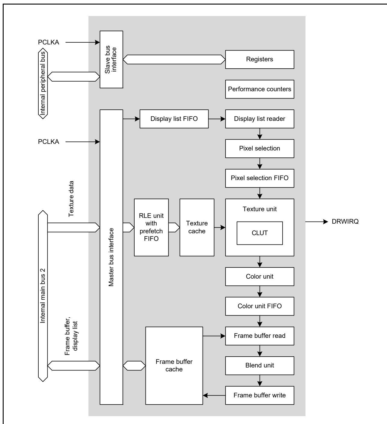
Figure 48.2 Block Diagram of the DRW2D
