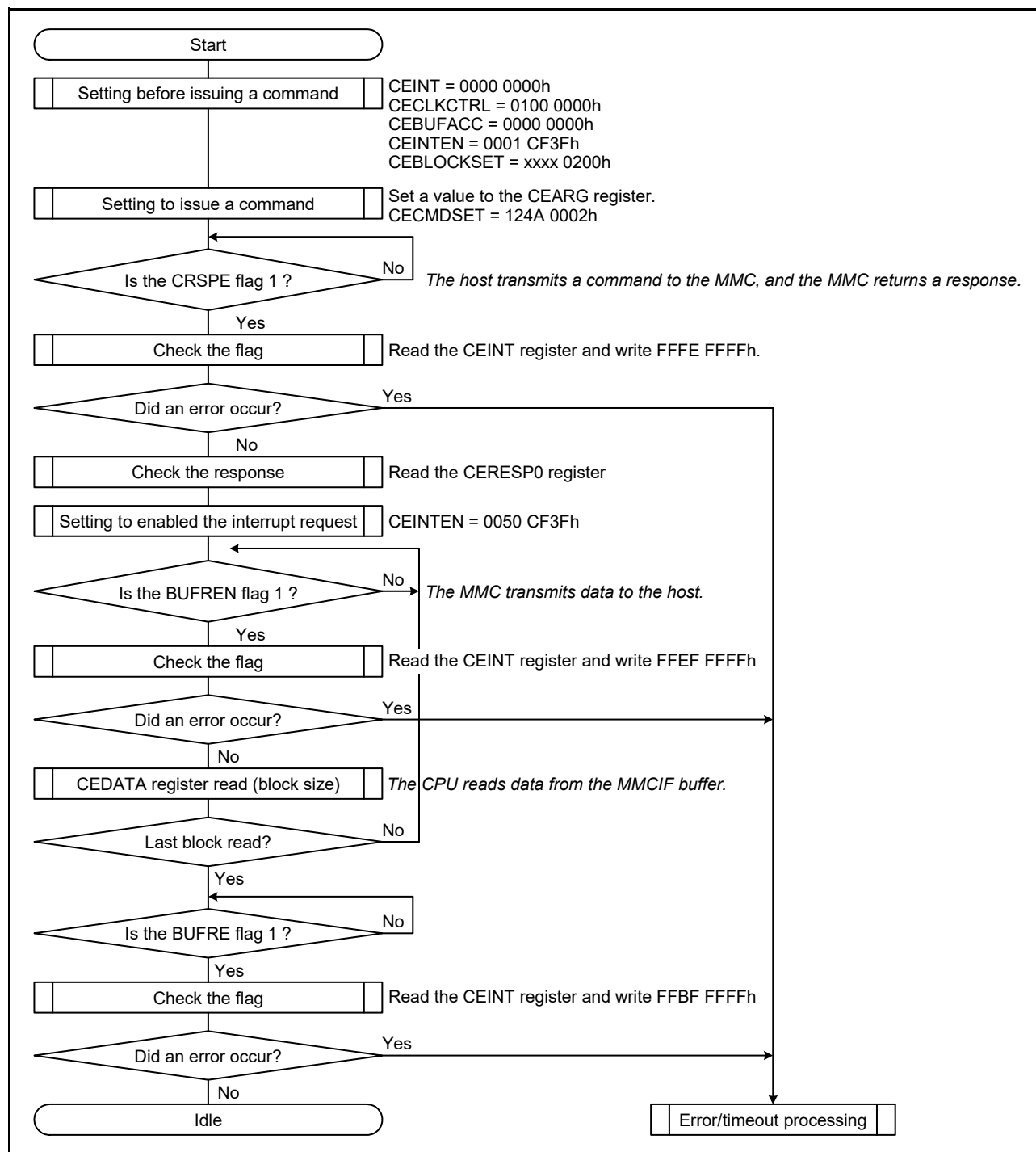
Figure 45.16 Issuing a Multi-Block Read Command (CMD18 Pre-Defined)
