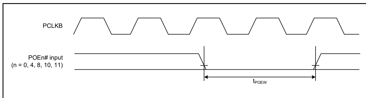
Figure 60.40 POE# Pin Input Timing
