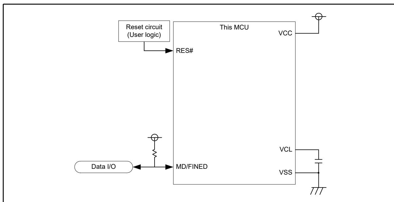
Figure 59.10 Example of Pin Connections in Boot Mode (FINE Interface)
