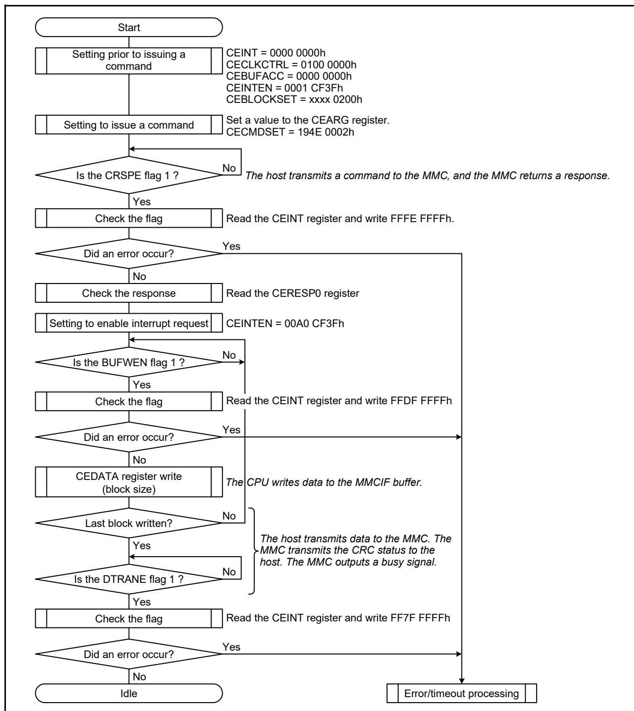
Figure 45.19 Issuing a Multi-Block Write Command (CMD25 Pre-Defined)
