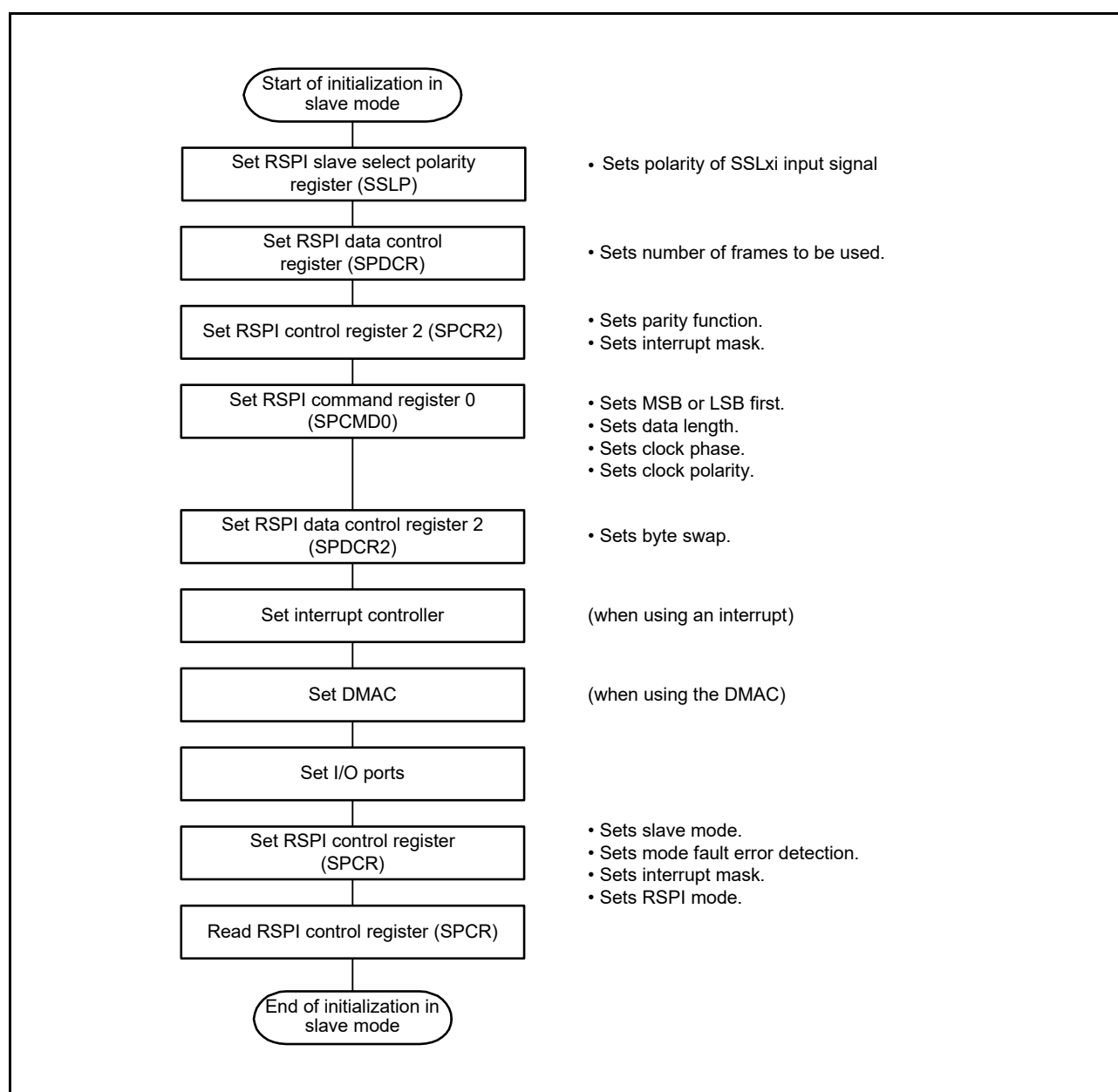
Figure 40.41 Example of Initialization Flowchart in Slave Mode (SPI Operation)
