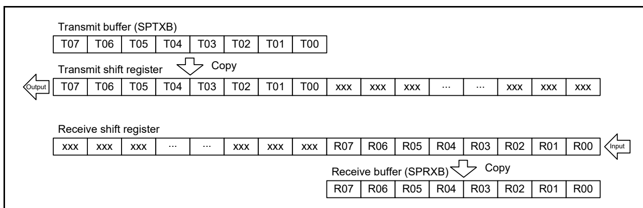
Figure 41.8 MSB First Transfer (8-Bit Data)
