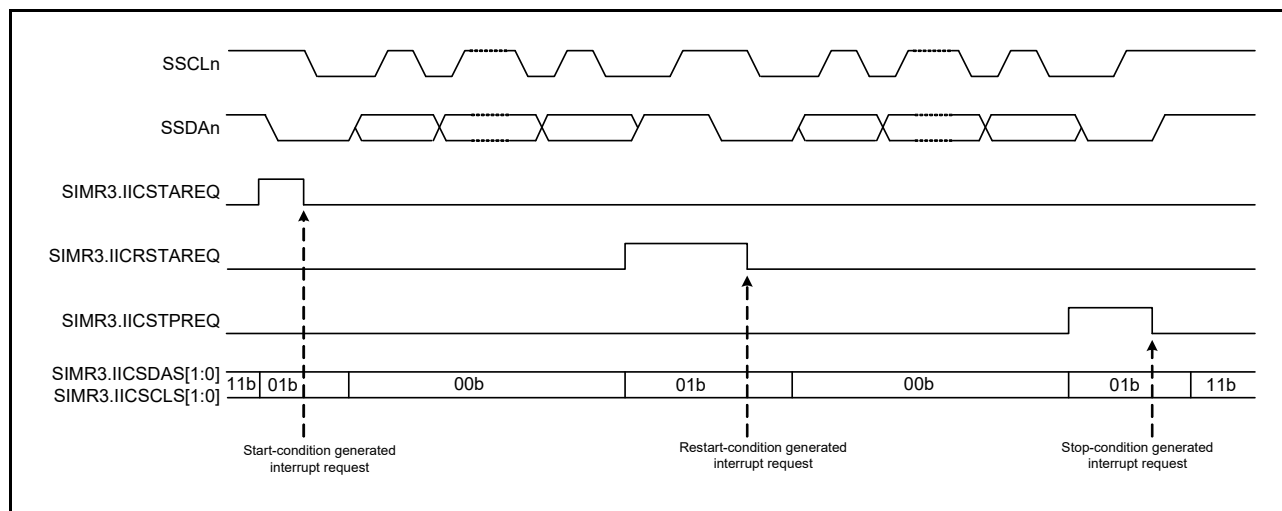
Figure 37.52 Timing of Operations in the Generation of Start, Restart, and Stop Conditions
