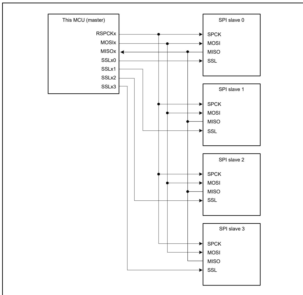
Figure 40.8 Single-Master/Multi-Slave Configuration Example (This MCU = Master)
