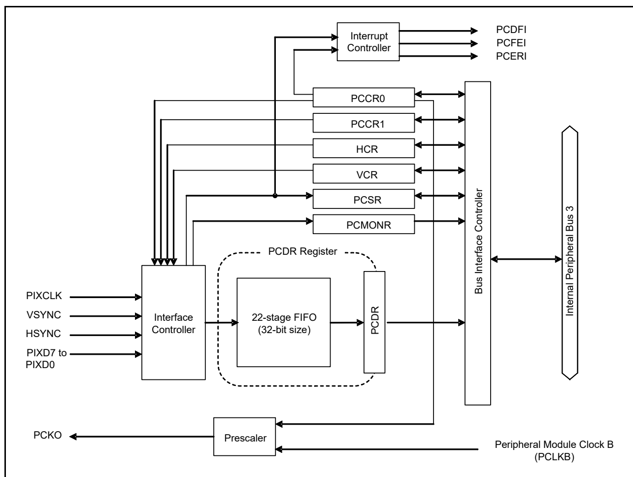
Figure 46.1 Block Diagram of the PDC
