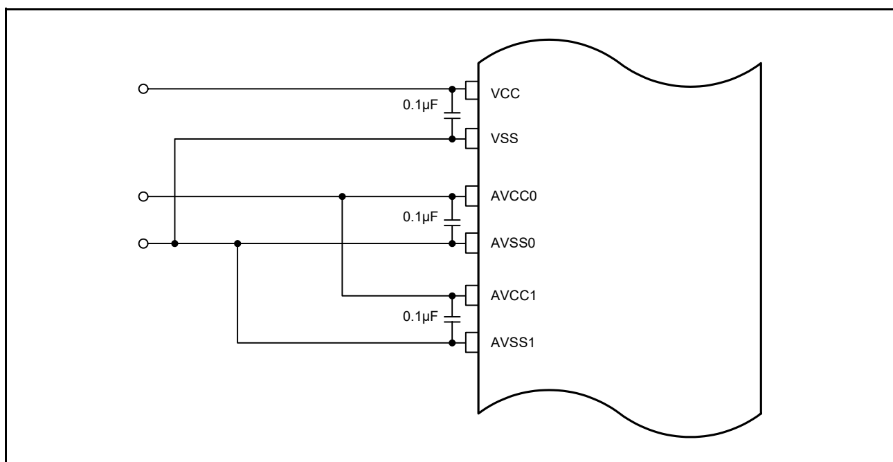
Figure 53.47 Power Supply Pin Connection Example
