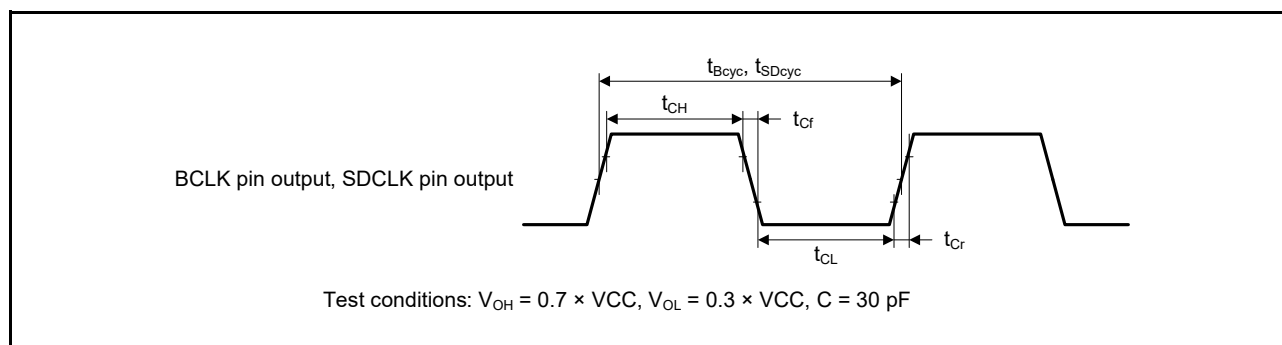
Figure 60.3 BCLK Pin and SDCLK Pin Output Timing
