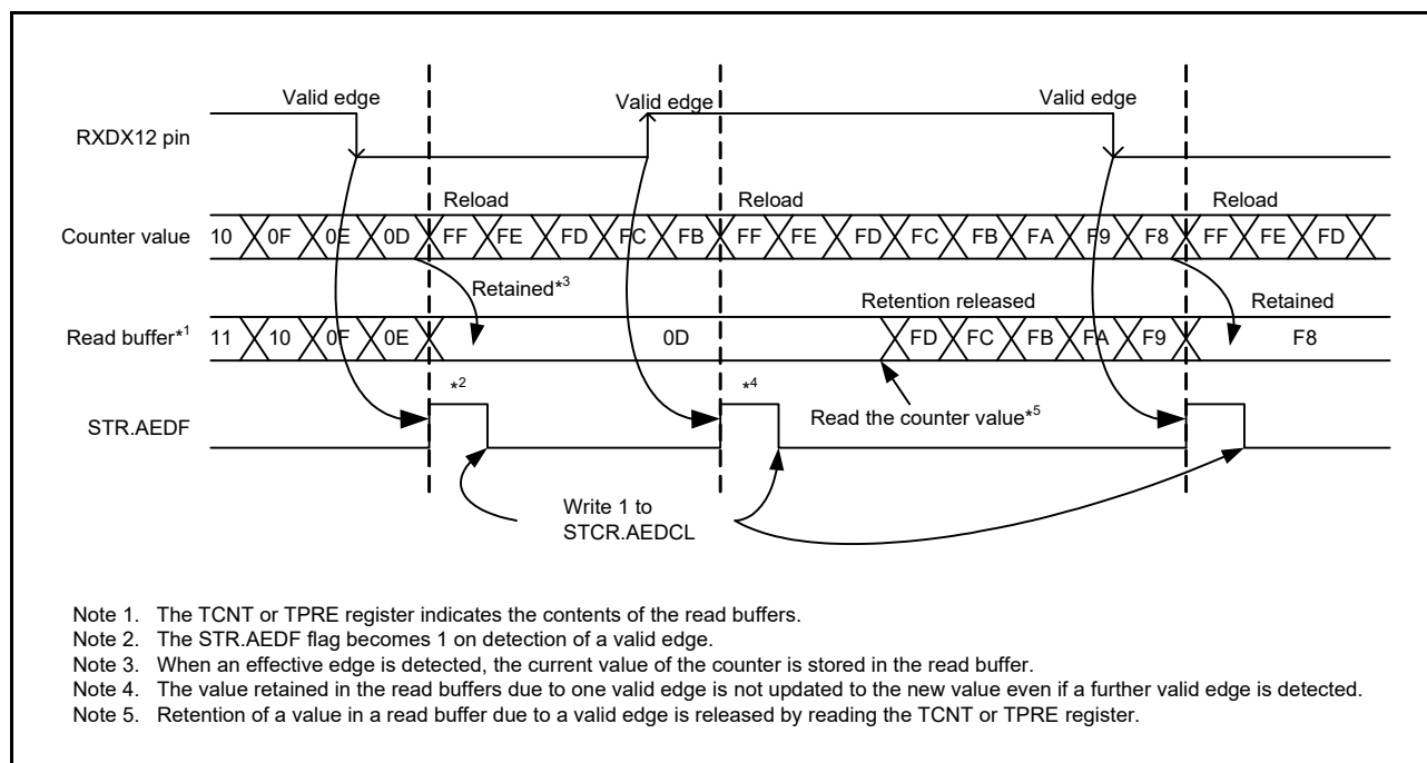
Figure 37.75 Example of Operations for Bit Rate Measurement
