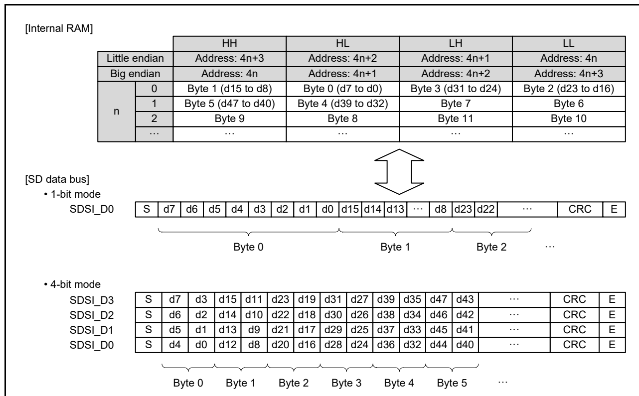
Figure 44.8 Data Format (Swapping the Byte Position)
