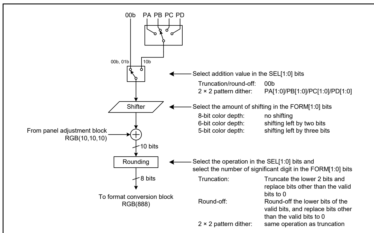
Figure 47.12 Structure of Dithering Block
