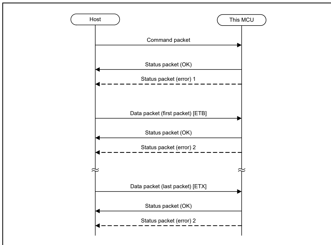
Figure 59.20 Program Command Transfer Sequence
