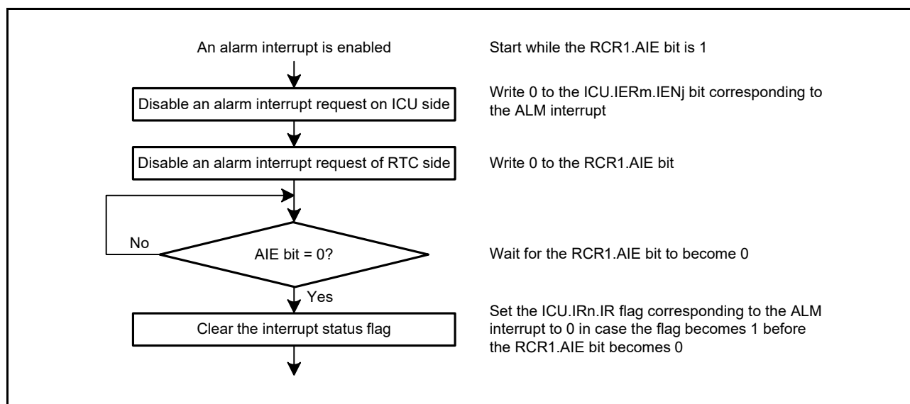
Figure 31.8 Procedure for Disabling Alarm Interrupt Request
