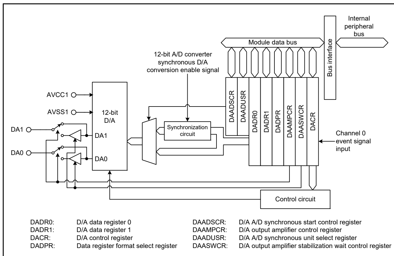
Figure 54.1 Block Diagram of 12-Bit D/A Converter
