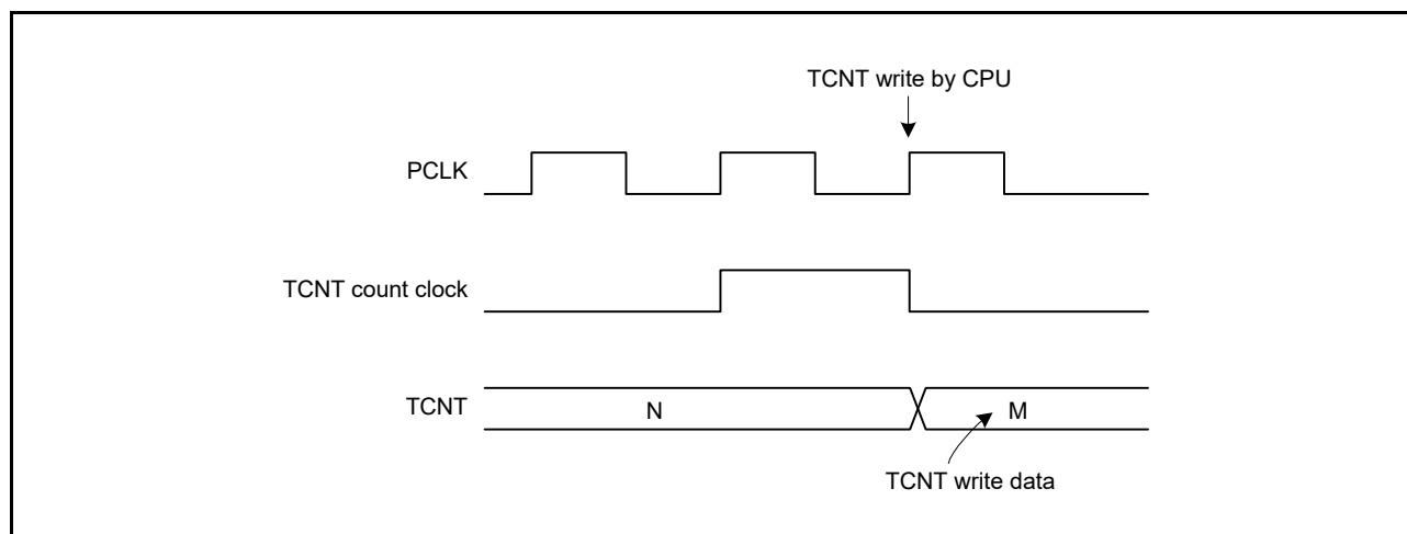
Figure 28.14 Conflict between TCNT Write and Increment
