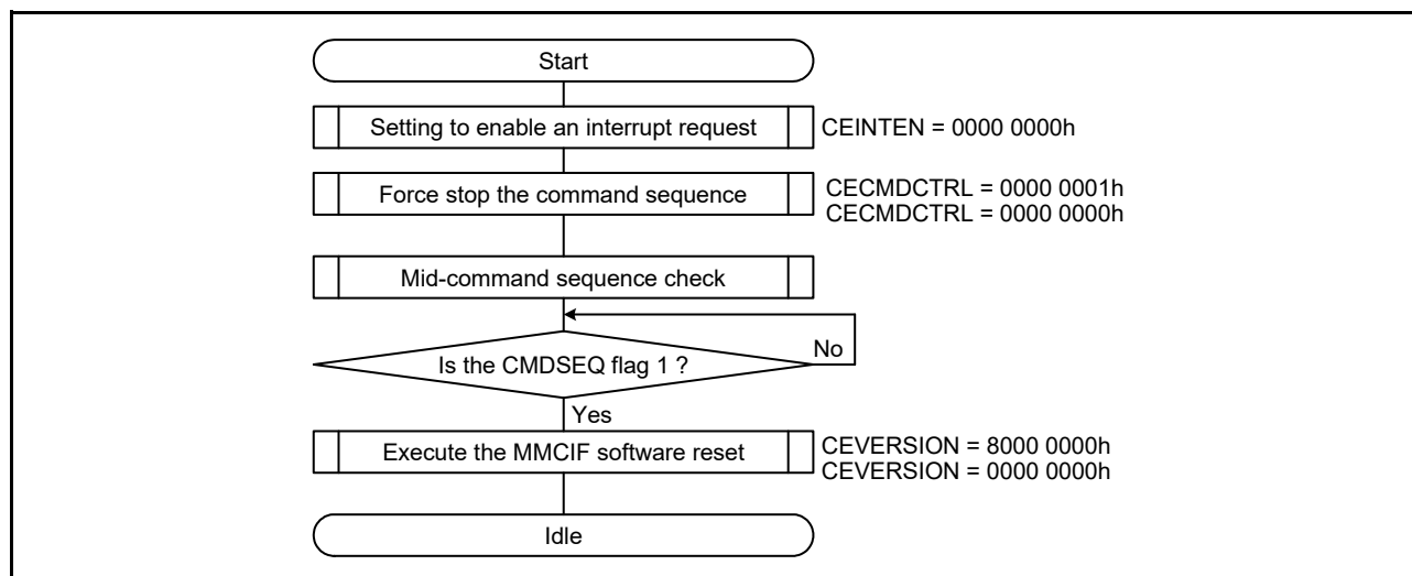
Figure 45.22 Command Sequence Force Stop
