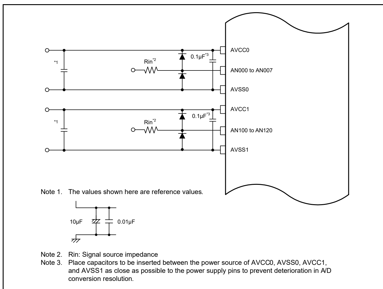
Figure 53.48 Sample Protection Circuit for Analog Inputs
