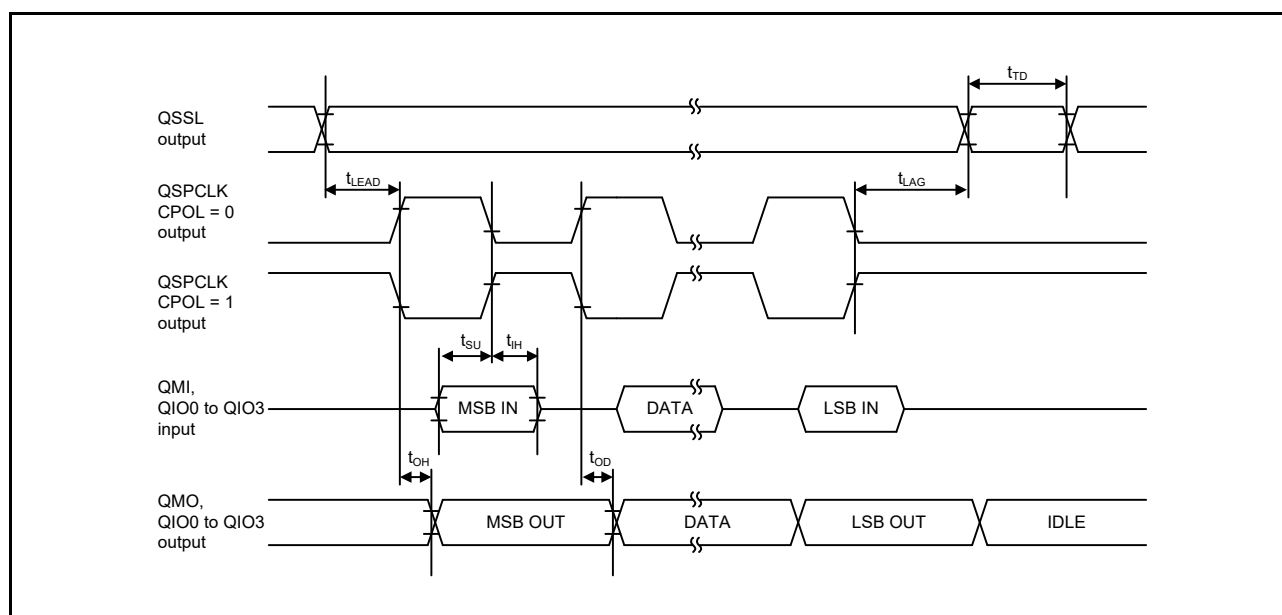
Figure 60.63 Transmit/Receive Timing (CPHA = 1)
