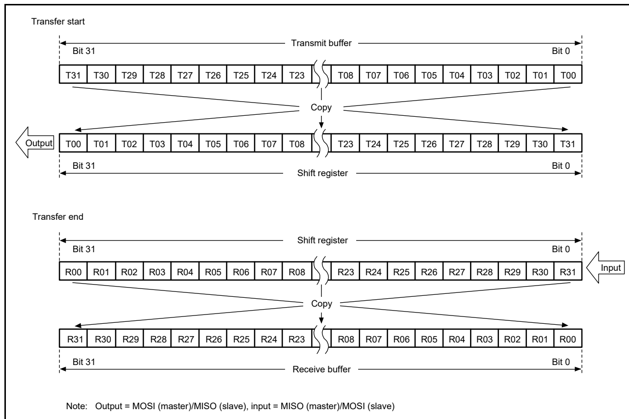
Figure 40.16 LSB First Transfer (32-Bit Data, Parity Disabled)
