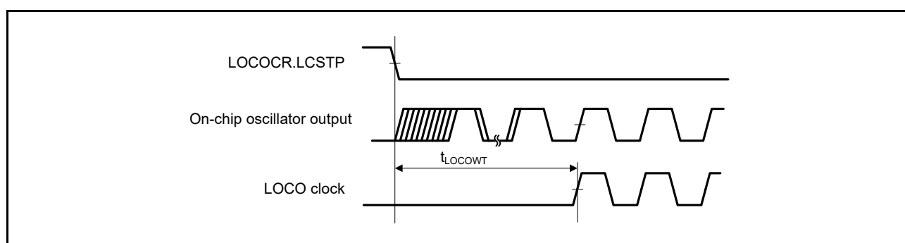
Figure 60.6 LOCO Clock Oscillation Start Timing
