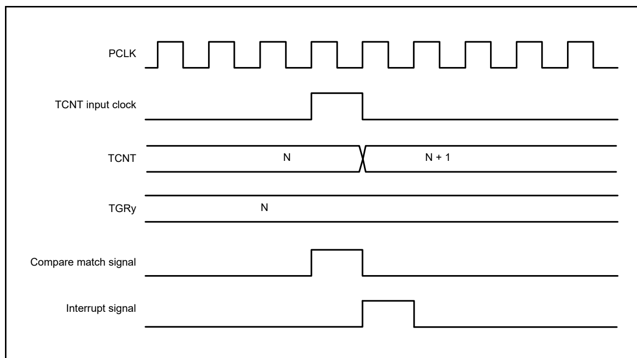
Figure 26.39 TGImy Interrupt Timing (Compare Match)
