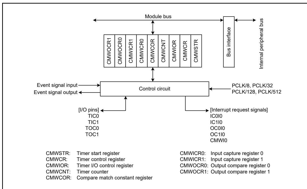
Figure 30.1 CMTW0 Block Diagram
