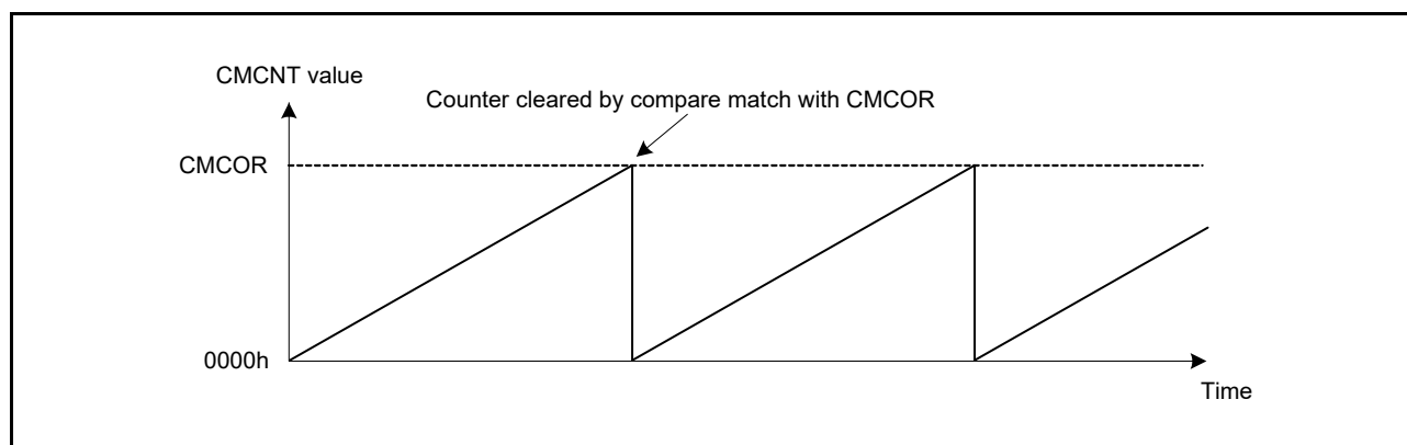
Figure 29.2 CMCNT Counter Operation
