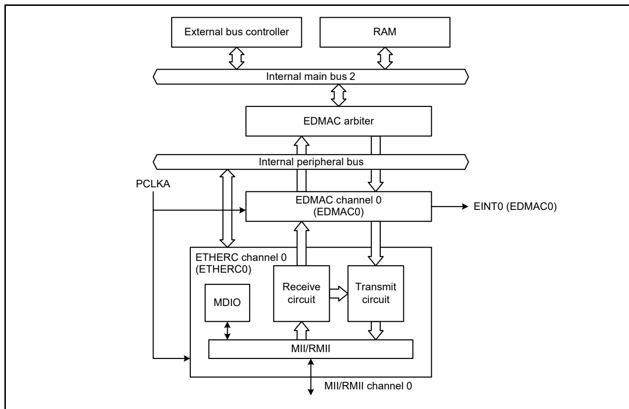
Figure 34.1 ETHERC Configuration
