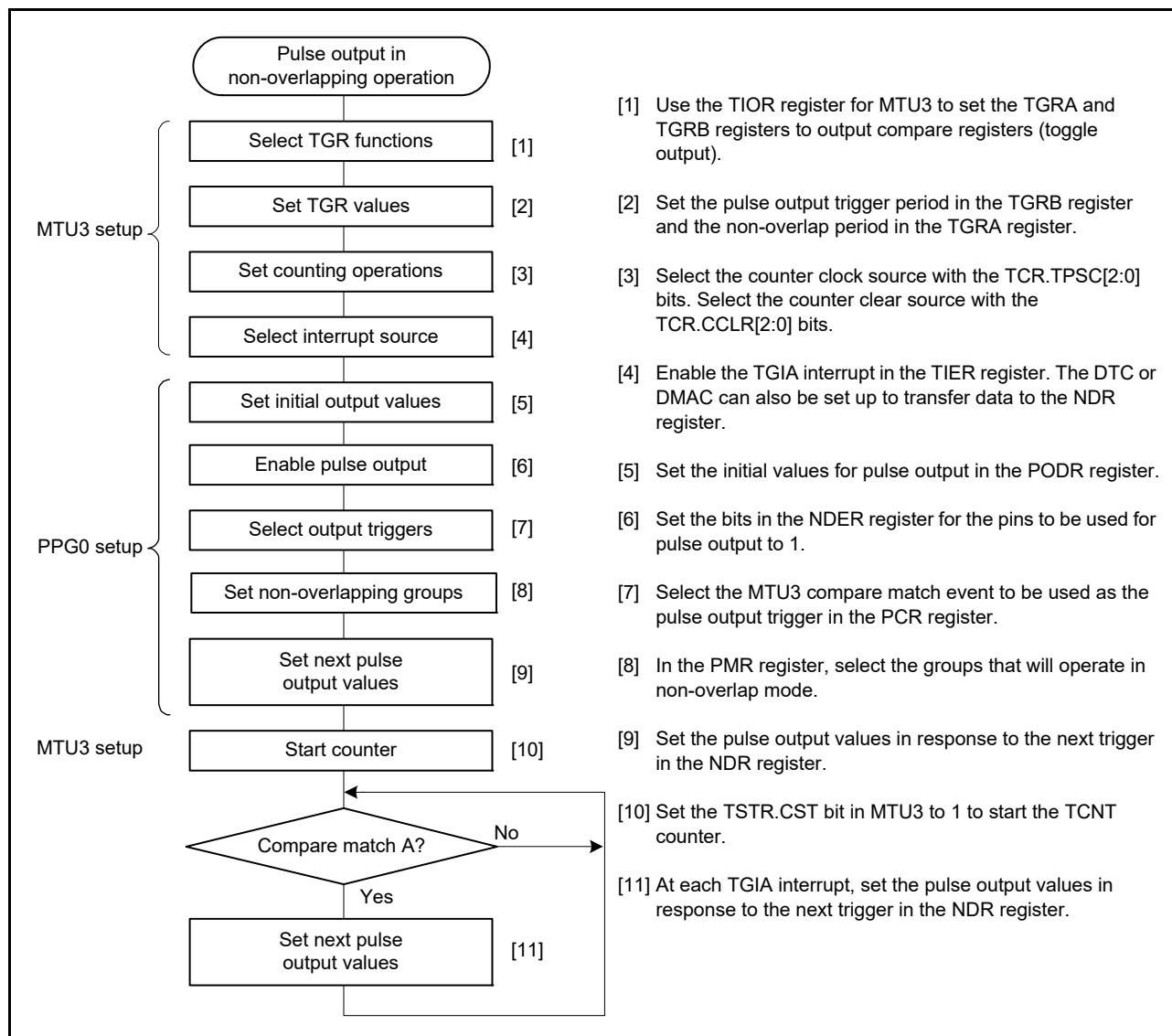
Figure 27.11 Example of Setup Procedure for Pulse Output in Non-Overlapping Operation (PPG0 Setting)
