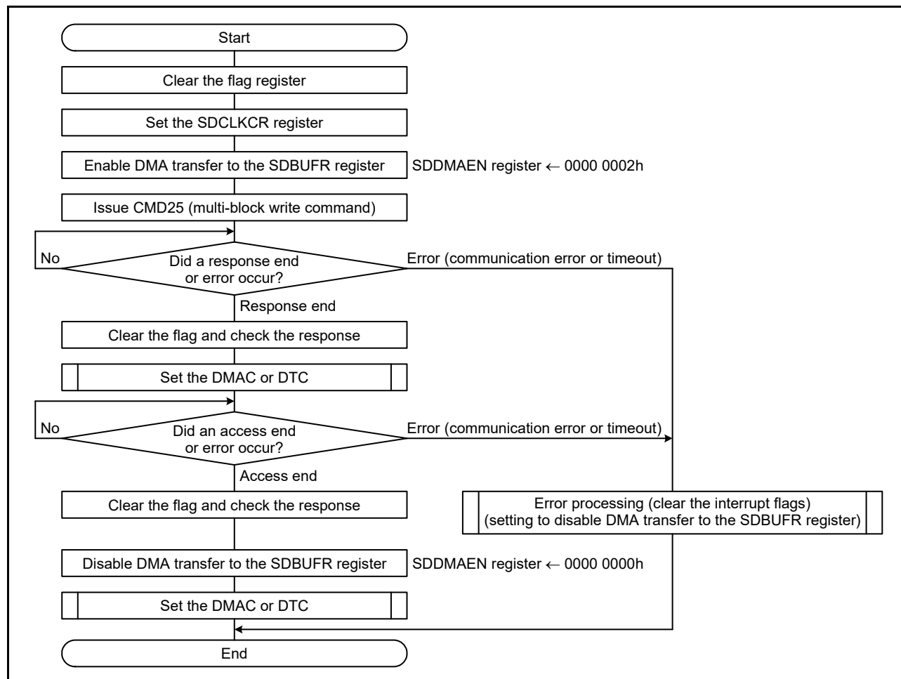
Figure 43.22 DMA Transfer After CMD25 is Issued
