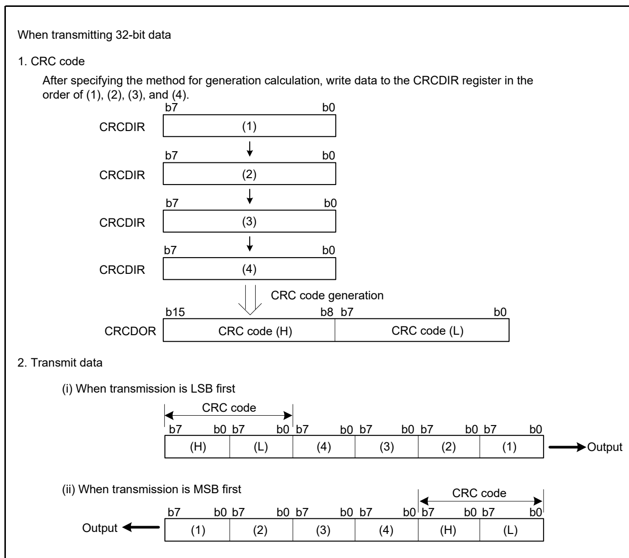
Figure 42.6 LSB First and MSB First Data Transmission
