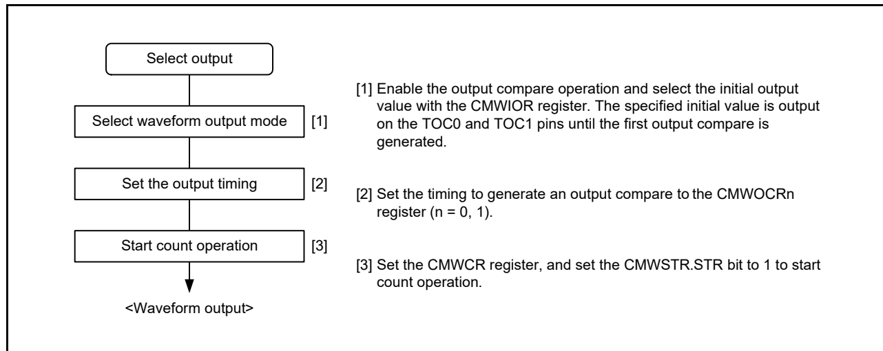
Figure 30.6 Procedure for Setting Output Compare Operation
