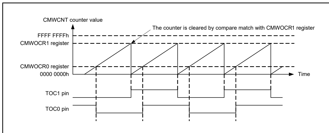
Figure 30.7 Example of Output Compare Operation (Unit 0)
