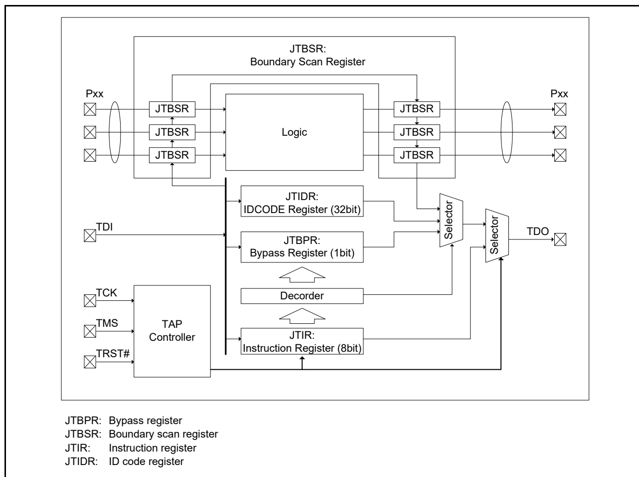
Figure 49.1 Block Diagram of JTAG
