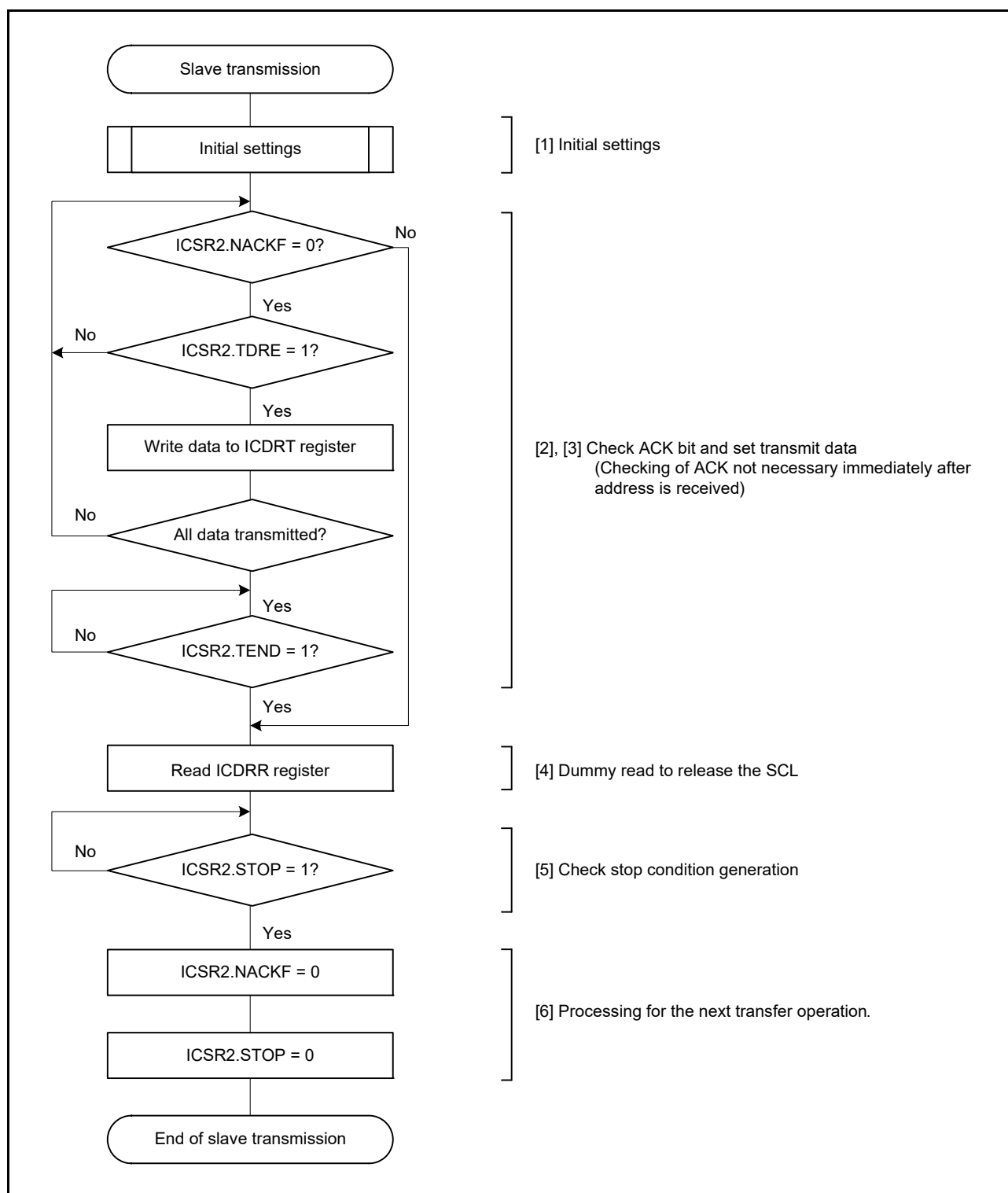
Figure 38.14 Example of Slave Transmission Flowchart
