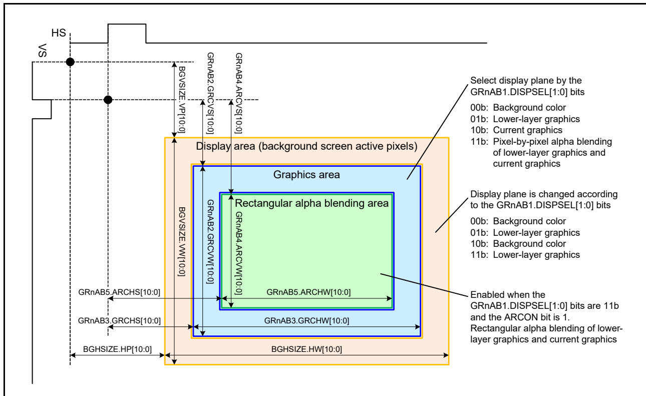
Figure 47.9 Selection of Graphic Display Screen (n = 1, 2)
