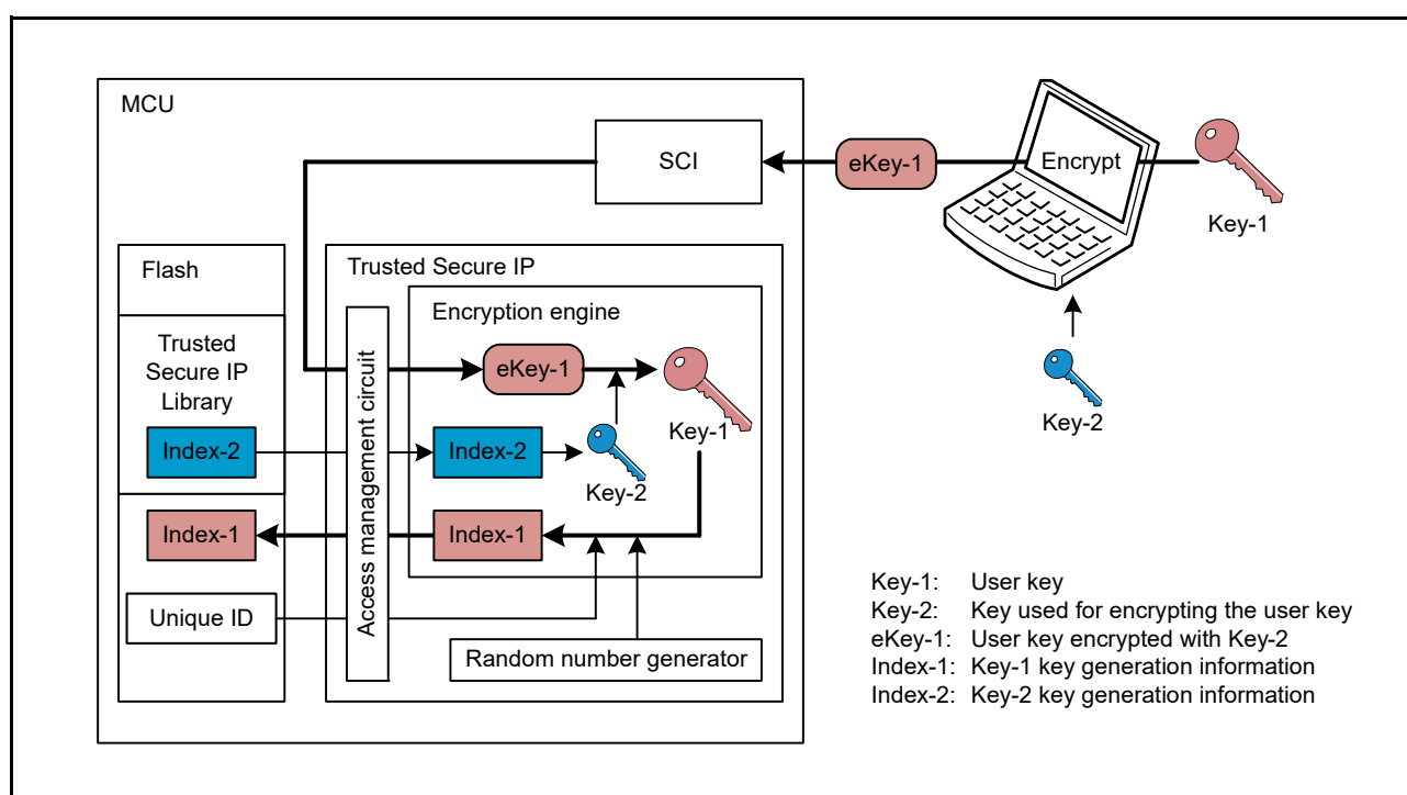
Figure 52.4 Key Installation Process
