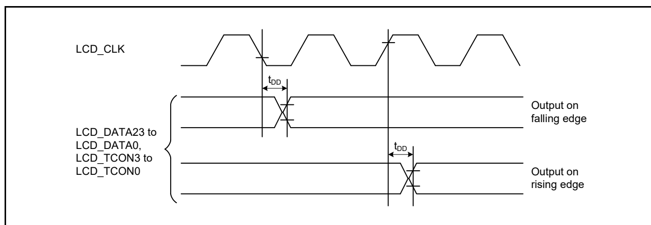
Figure 60.81 LCD Output Data Timing
