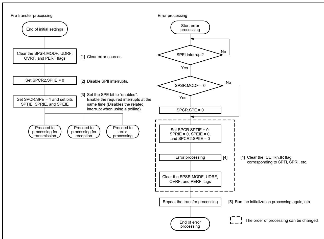
Figure 40.44 Flowchart for Slave Mode (Error Processing)
