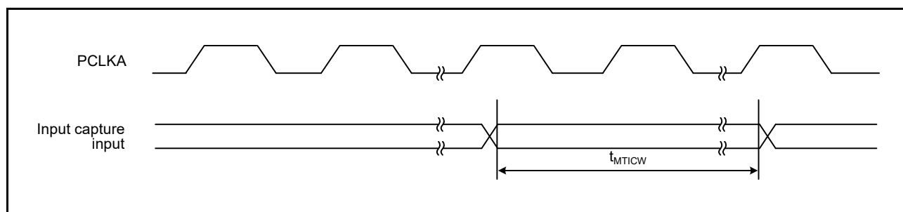
Figure 60.38 MTU3 Input Capture Input Timing
