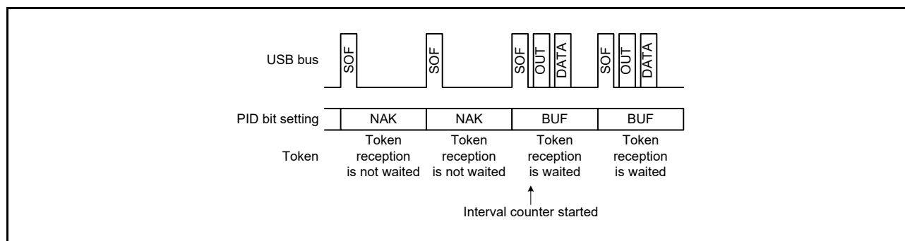
Figure 36.18 Relationship between Frames and Expected Token Reception When IITV[2:0] = 000b
