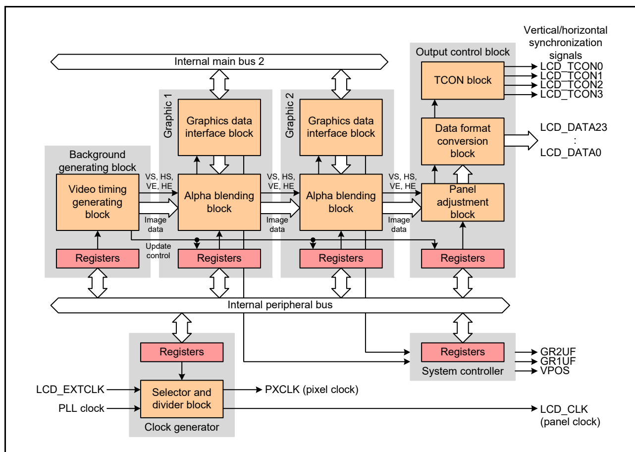
Figure 47.1 GLCDC Block Diagram
