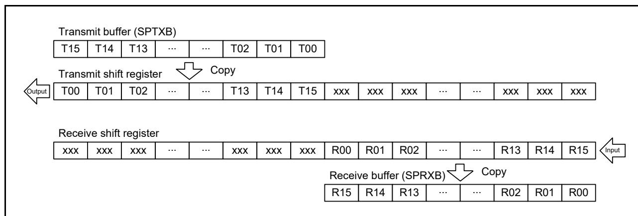
Figure 41.10 LSB First Transfer (16-Bit Data)
