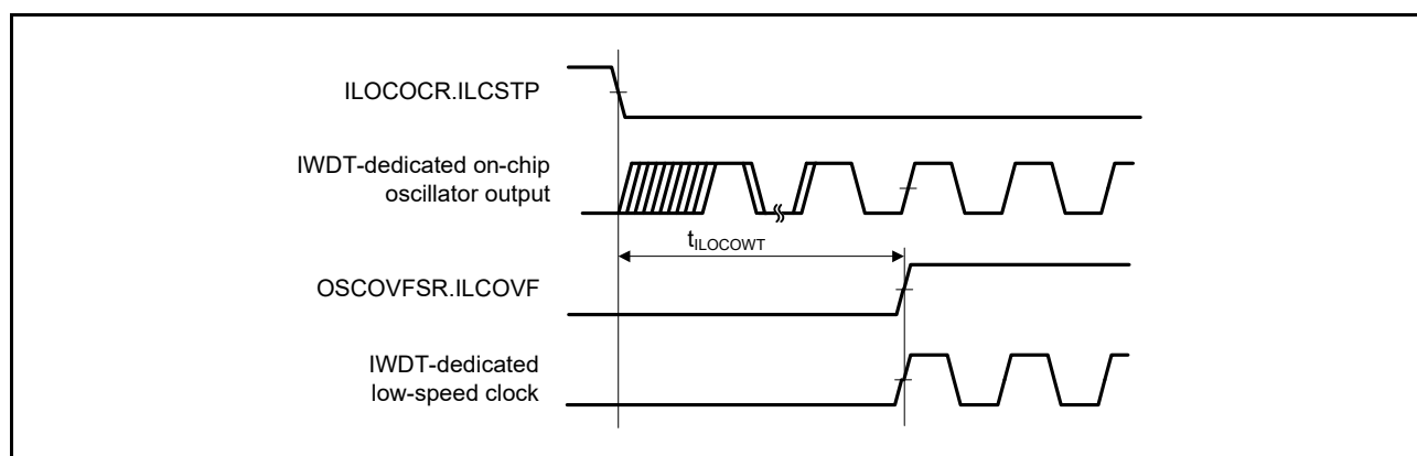
Figure 60.7 IWDT-dedicated Low-Speed Clock Oscillation Start Timing
