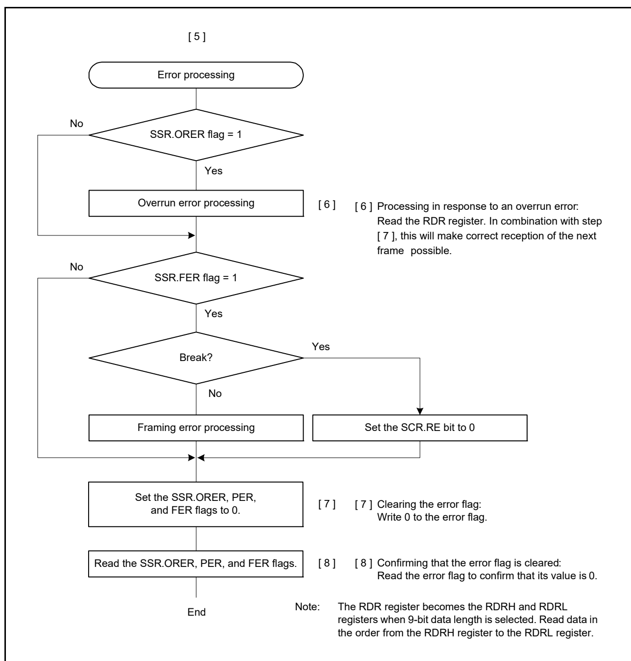
Figure 37.26 Example of Multi-Processor Serial Reception Flowchart (2)
