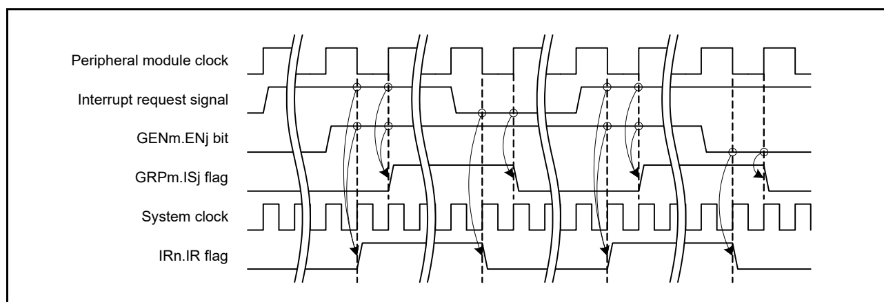
Figure 15.16 Operation Example of Group Interrupt Using Level Detection ( m = \text{BL0, BL1, BL2, AL0, AL1} )
