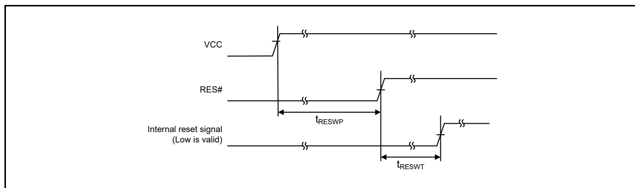
Figure 60.1 Reset Input Timing at Power-On
