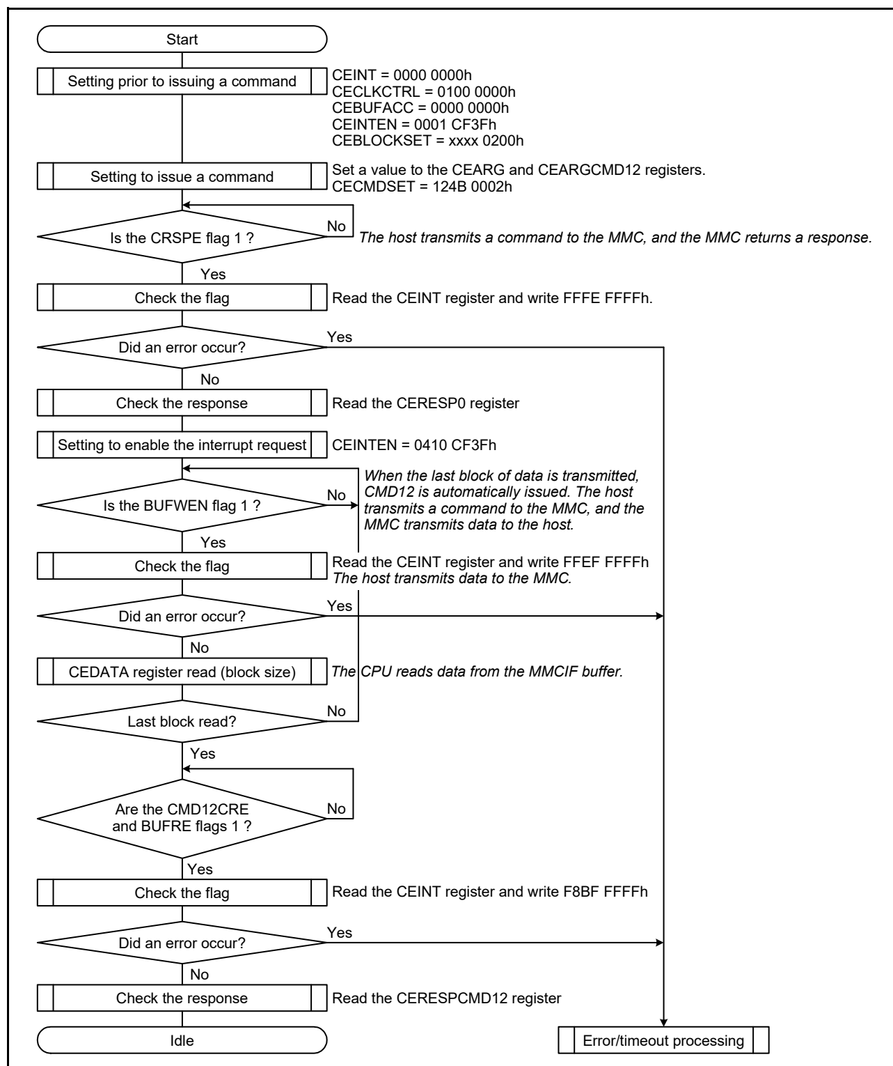
Figure 45.17 Issuing a Multi-Block Read Command (CMD18 Open-Ended)
