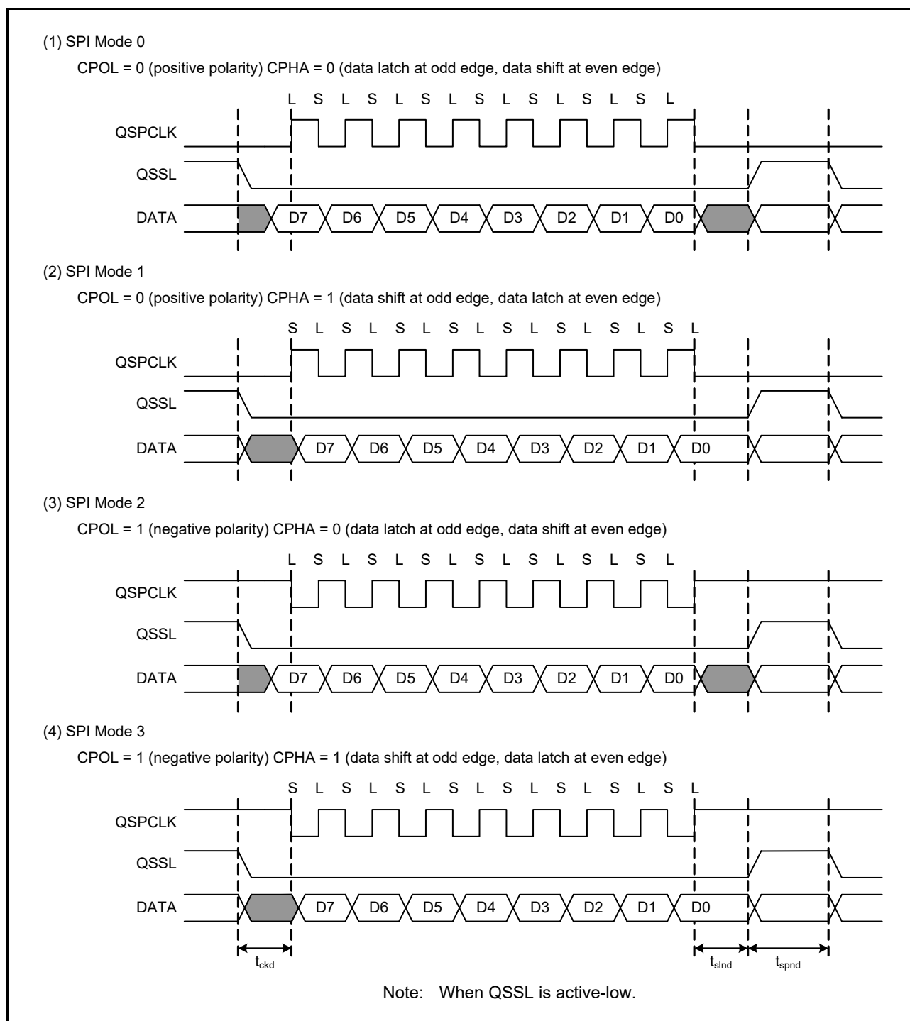
Figure 41.2 Clock Setting and Transfer Timing
