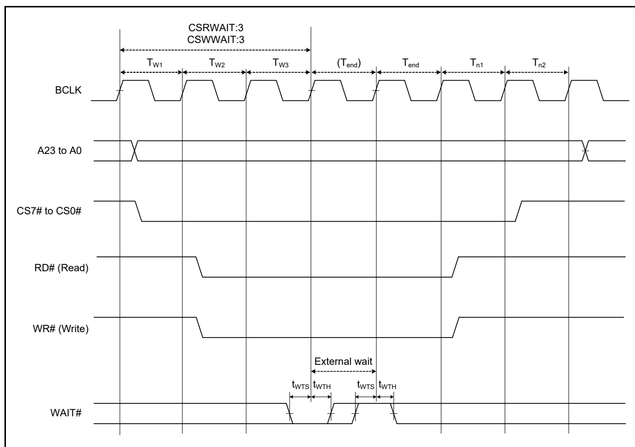
Figure 60.22 External Bus Timing/External Wait Control
