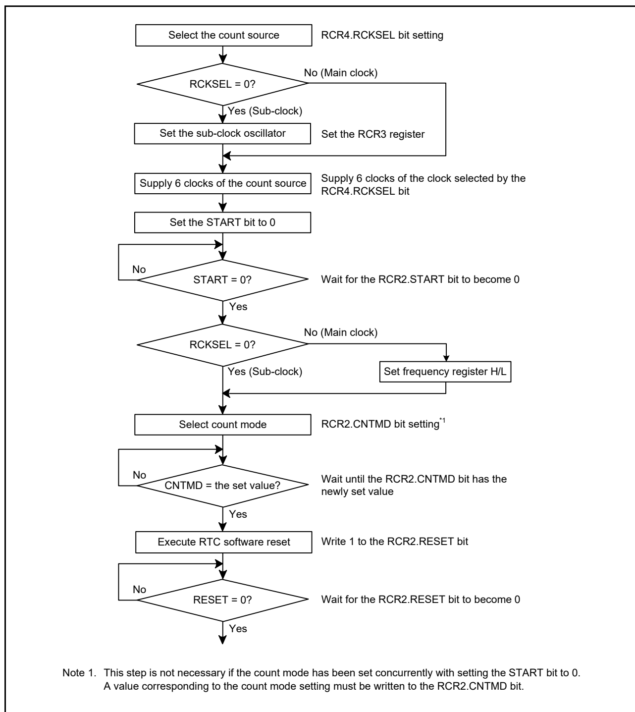
Figure 31.3 Clock and Count Mode Setting Procedure
