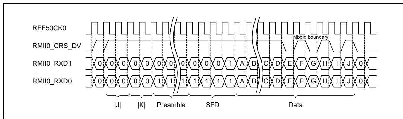
Figure 34.12 RMII Frame Receive Timing During Normal Reception
