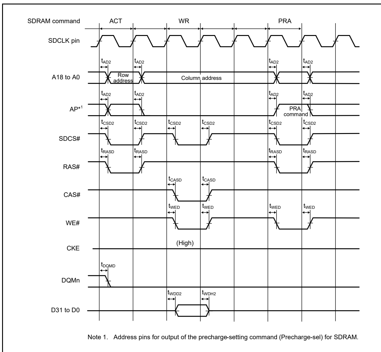
Figure 60.24 SDRAM Space Single Write Bus Timing
